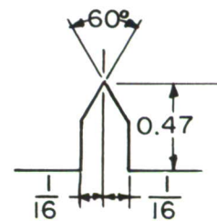
NOTCH DETAIL
