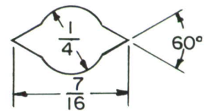
NOTCH DETAIL
