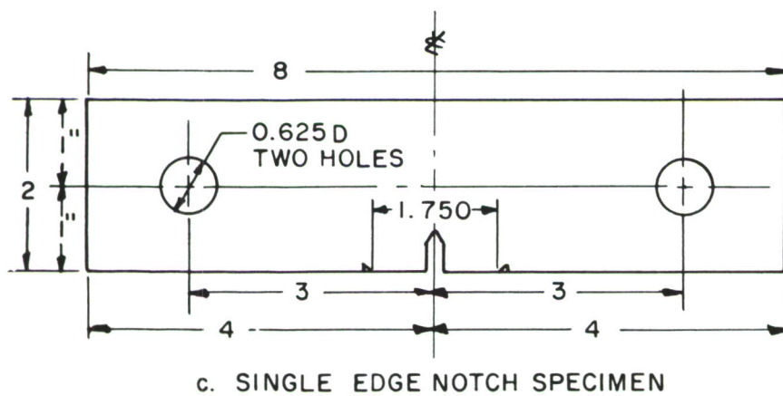
Figure 2. Test Specimens
