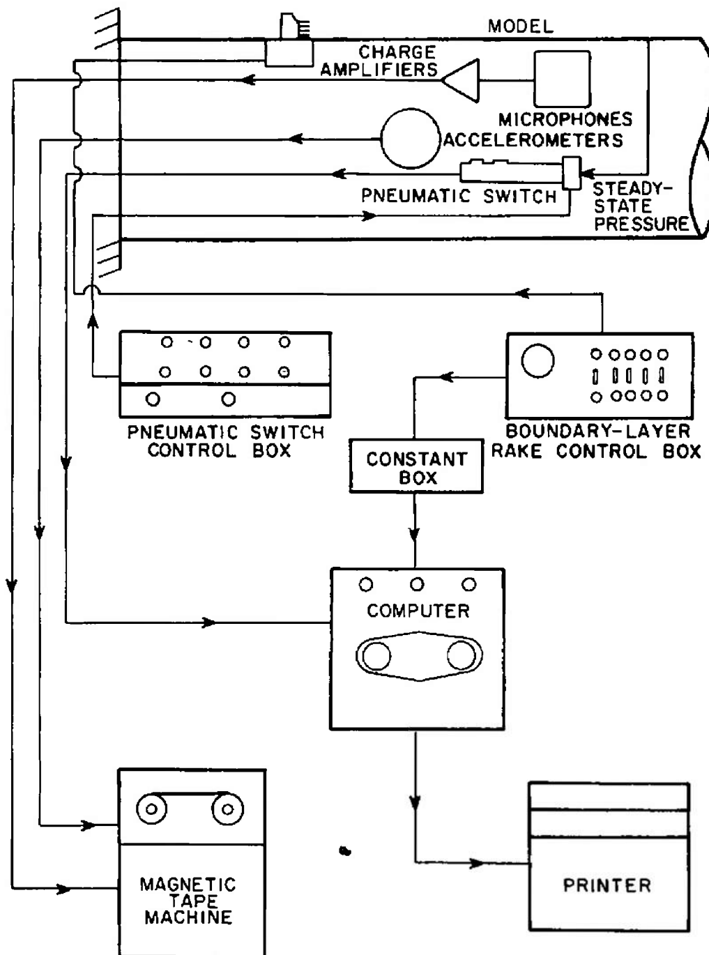
Fig. 5 Instrumentation Arrangement
