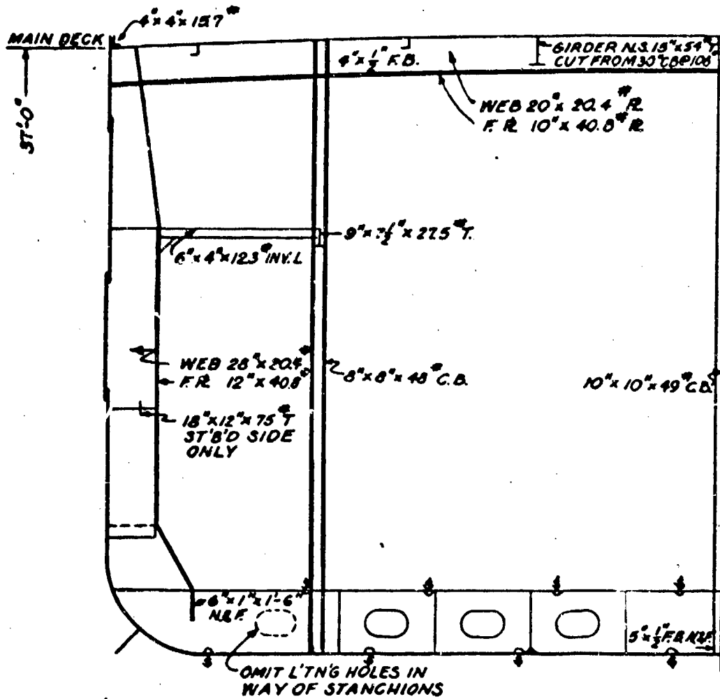
FRAME 78 LOOKING AFT
