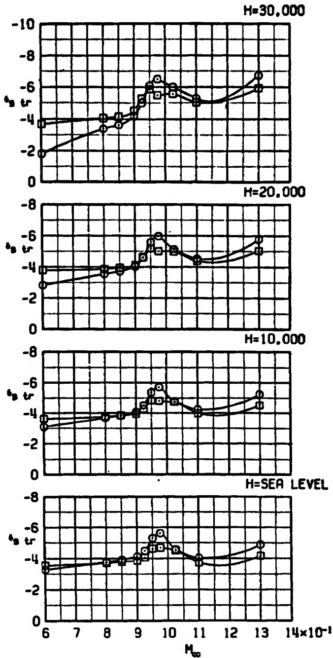
Figure 35. The effect of the Oneway RPV store on trim stabulator angle.
