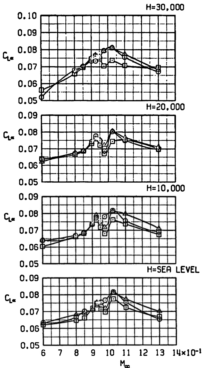
Figure 33. The effect of the PF Modular Weapons stores on the lift-curve slope at trim.
