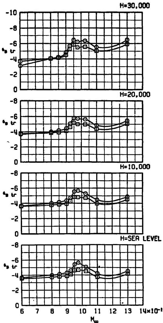
Figure 20. The effect of the Stubby HOBOS store on trim stabilator angle.
