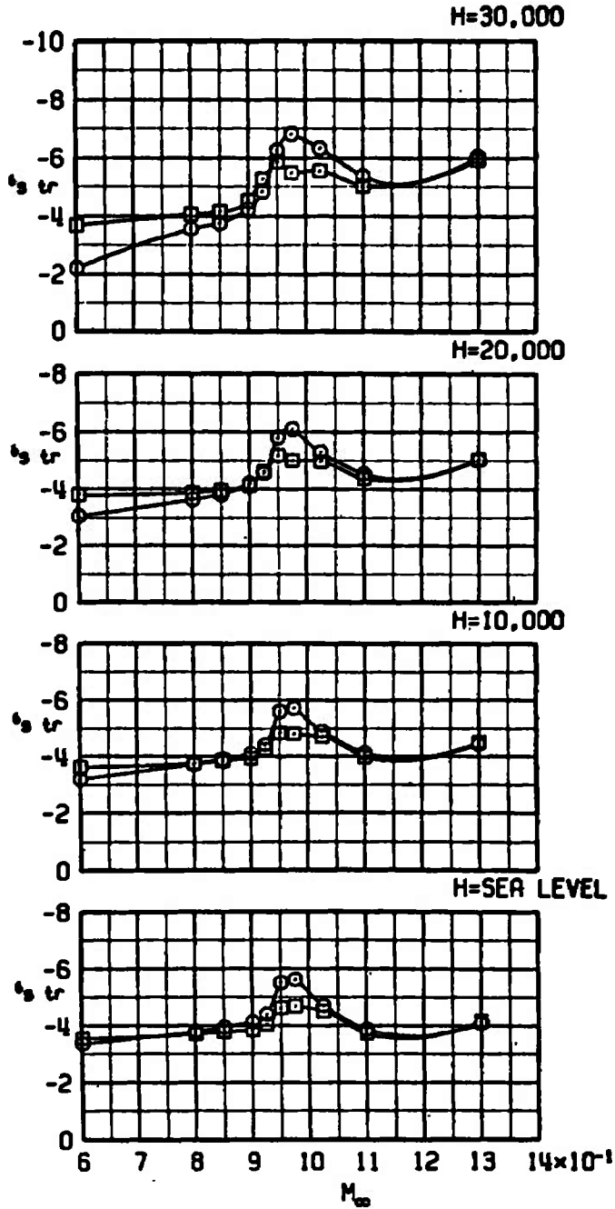
Figure 40. The effect of the ERV store on trim stabilator angle.
