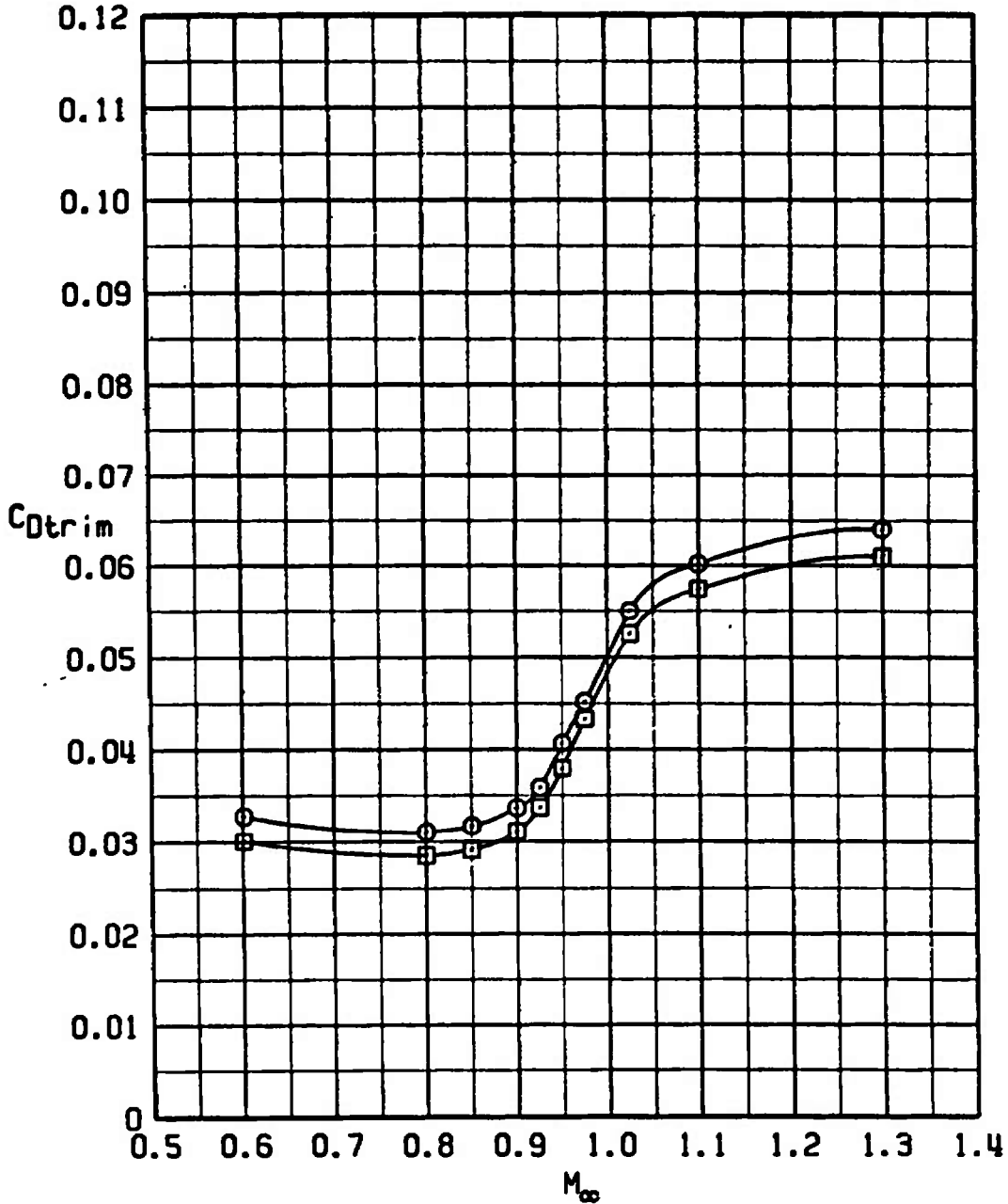
Figure 49. The effect of the TCTV store on trim drag.
