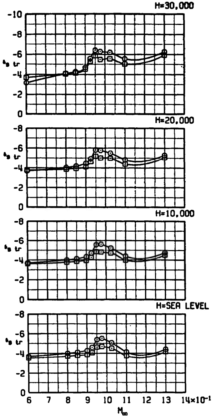
Figure 25. The effect of the TCTV store on trim stabilator angle.
