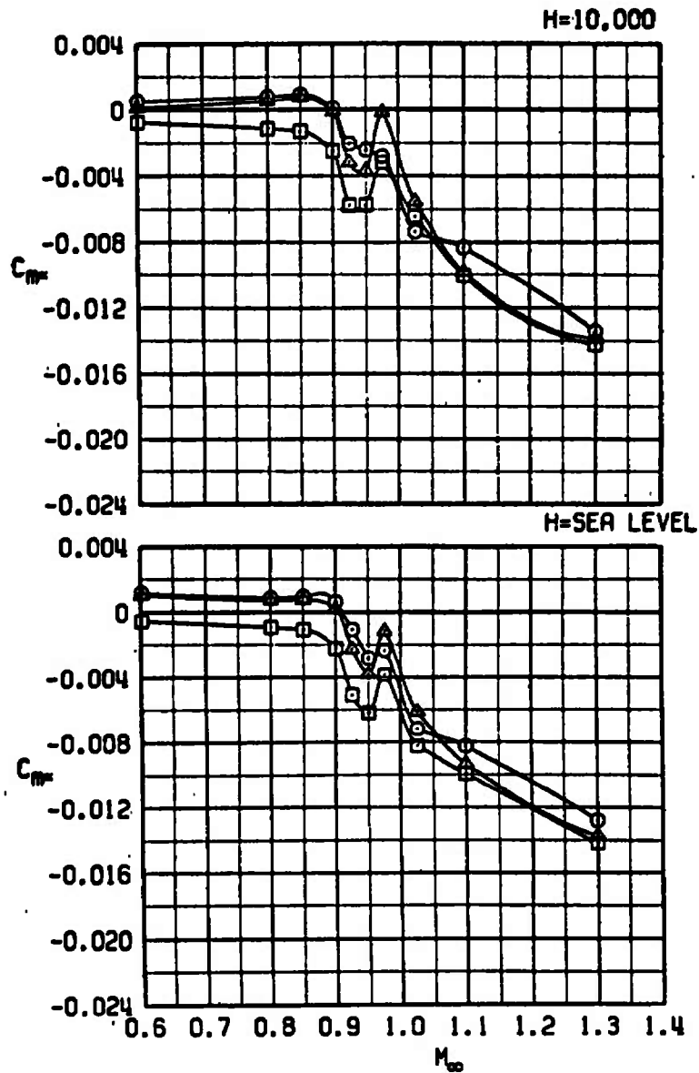
Figure 32. The effect of the PF Modular Weapons stores on the slope of the pitching-moment coefficient versus angle-of-attack curve at trim.
