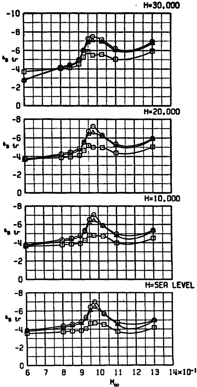
Figure 30. The effect of the PF Modular Weapons stores on trim stabilator angle.
