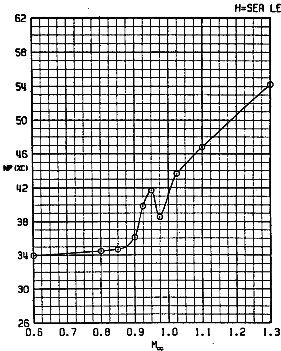
Figure 9. Neutral-point location as a function of Mach number and altitude for configuration 21.
