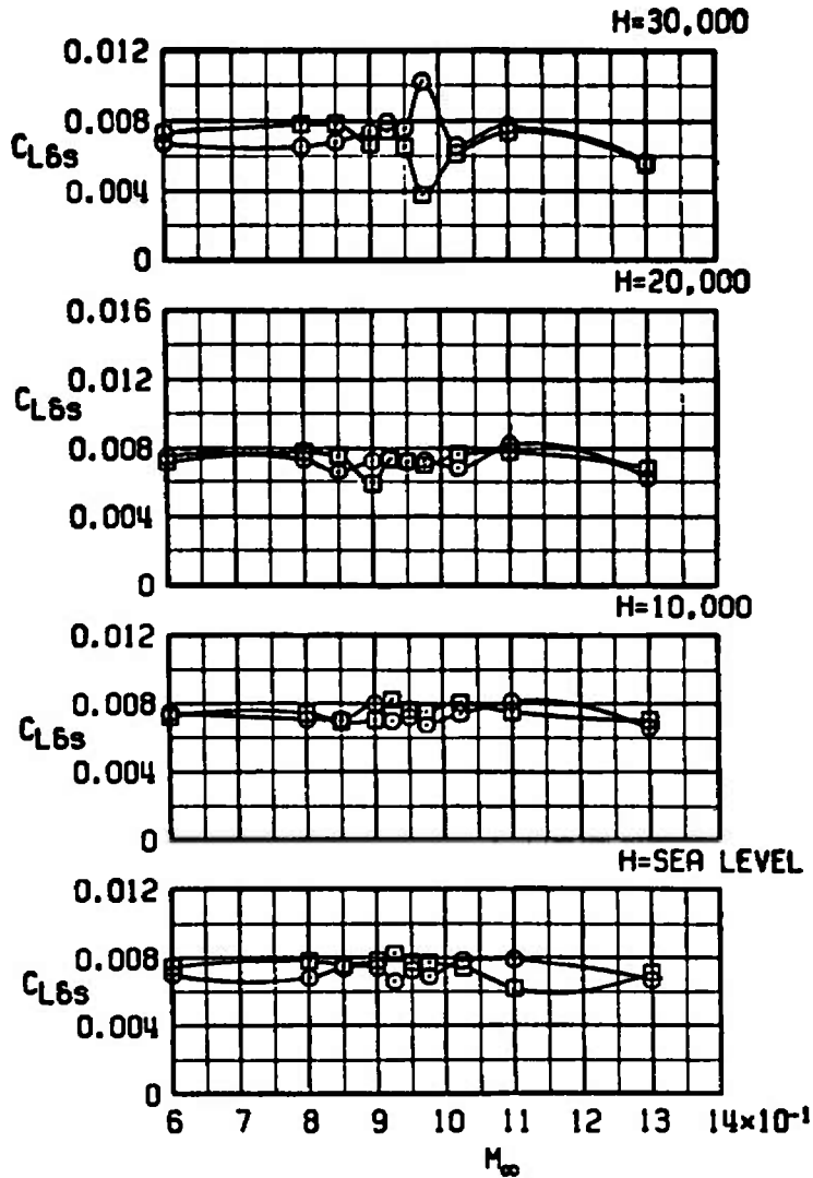
b. Stabilator lift effectiveness Figure 59. Concluded.
