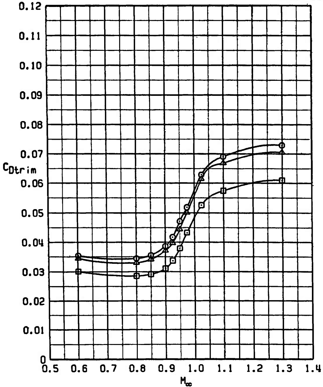
Figure 50. The effect of the PF Modular Weapons stores on trim drag.
