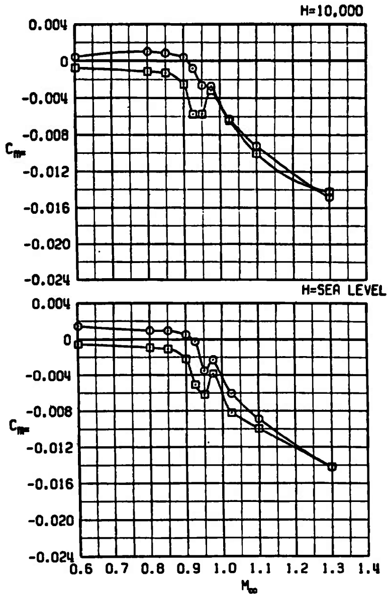
Figure 42. The effect of the ERV store on the slope of the pitching-moment coefficient versus angle-of-attack curve at trim.
