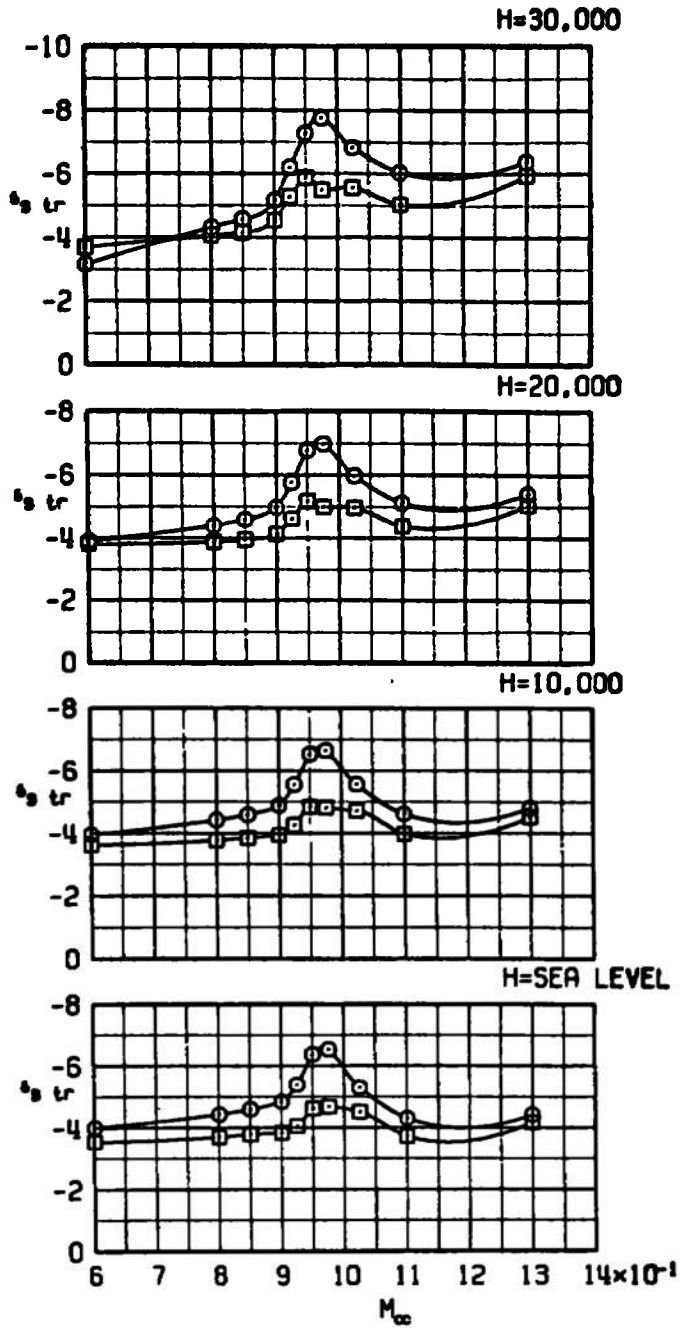
Figure 15. The effect of the SOM store on trim stabilator angle.
