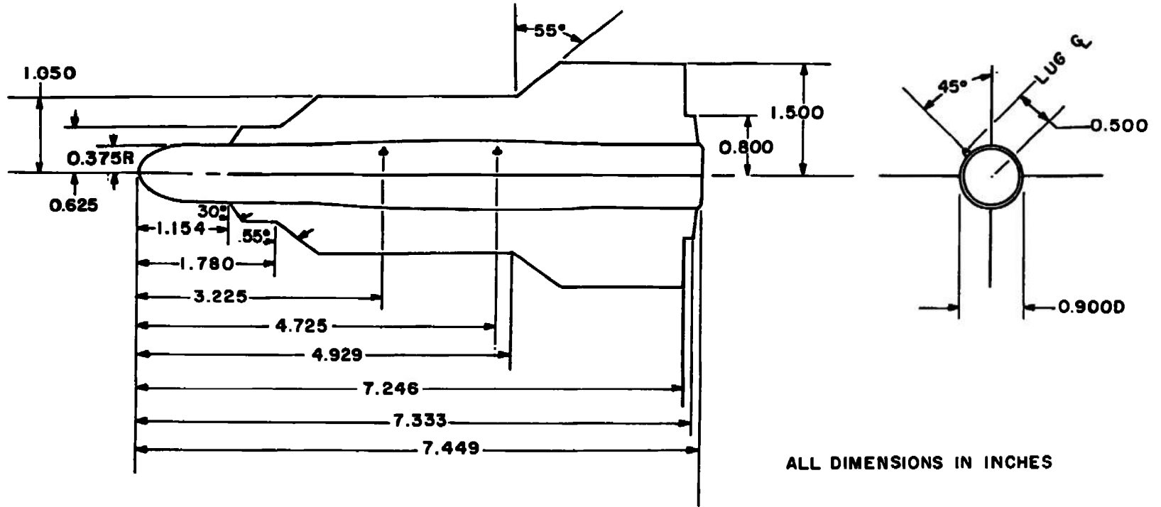
c. Tactical Control Test Vehicle (TCTV) Figure 6. Continued.
