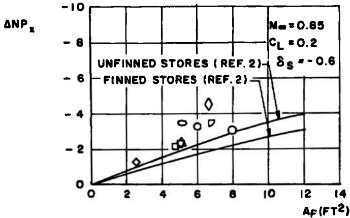
a. Wing-mounted store frontal area correlation
