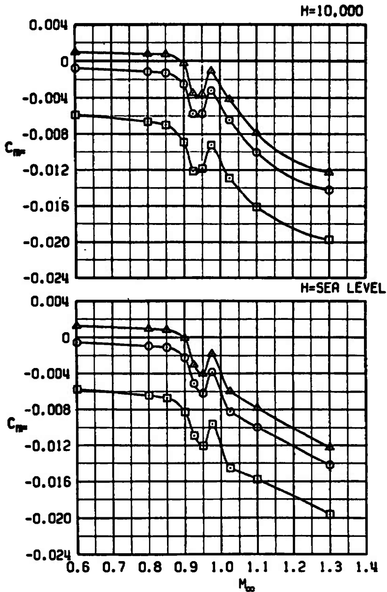
Figure 10. Slope of pitching-moment coefficient versus angle-of-attack curve at trim as a function of Mach number, altitude, and cg location for configuration 21.
