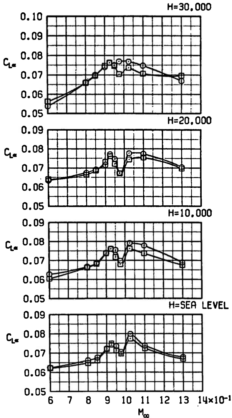
Figure 28. The effect of the TCTV store on the lift-curve slope at trim.
