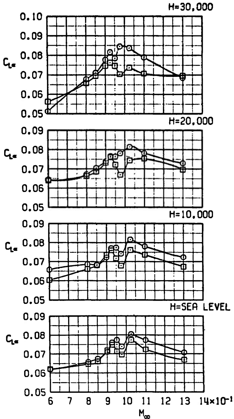
Figure 38. The effect of the Oneway RPV store on the lift-curve slope at trim.
