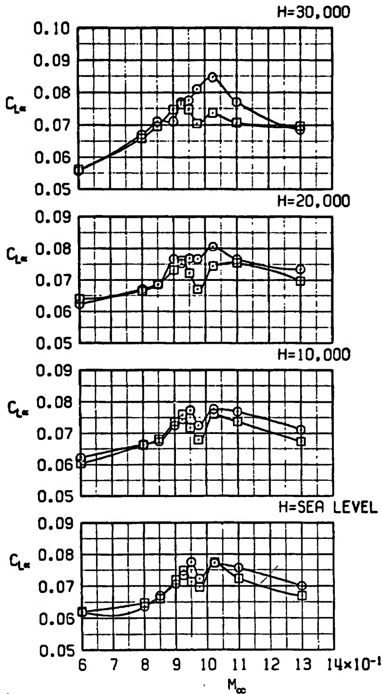
Figure 43. The effect of the ERV store on the lift-curve slope at trim.
