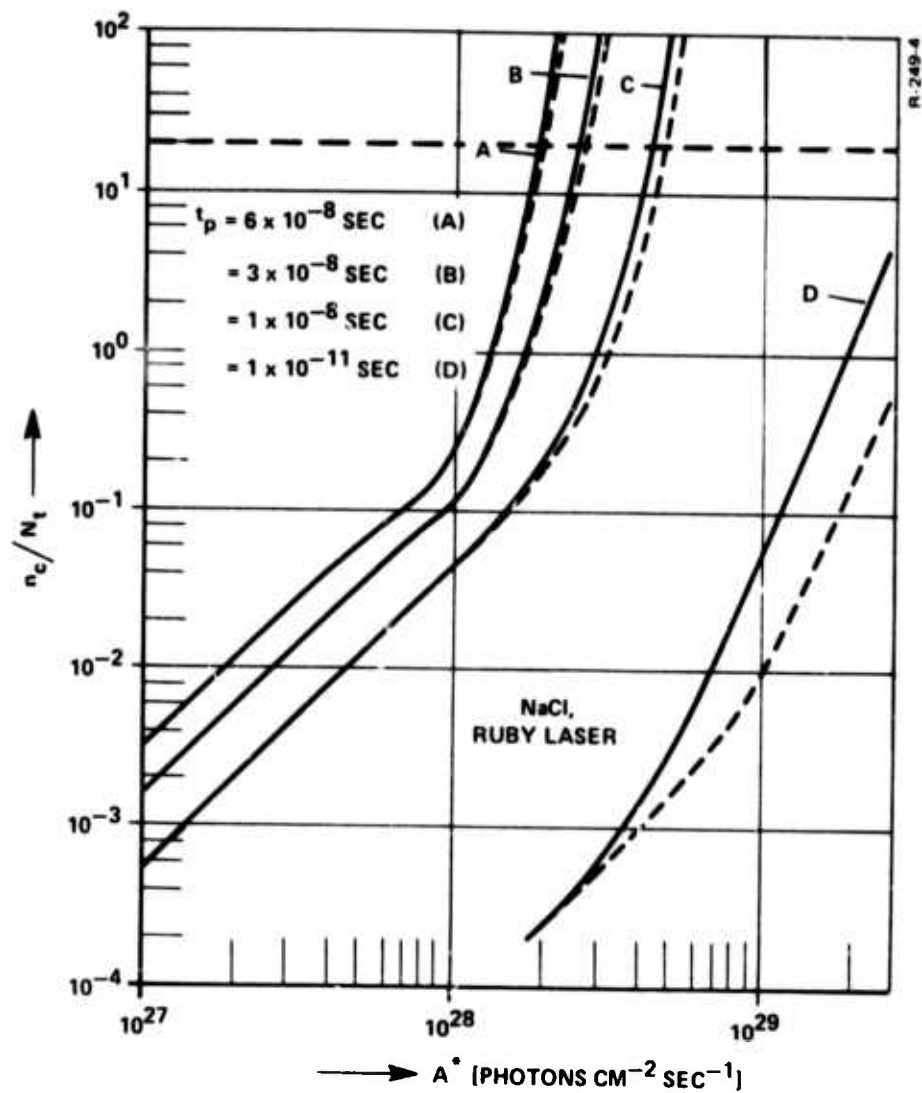
Figure 3 - Normalized concentration n_c/N_t of free electrons in NaCl containing 5 \times 10^{15} \text{ cm}^{-3} \text{Cl}^- -vacancies as a function of laser peak flux A^* for ruby laser pulses of several different pulse lengths t_p .
