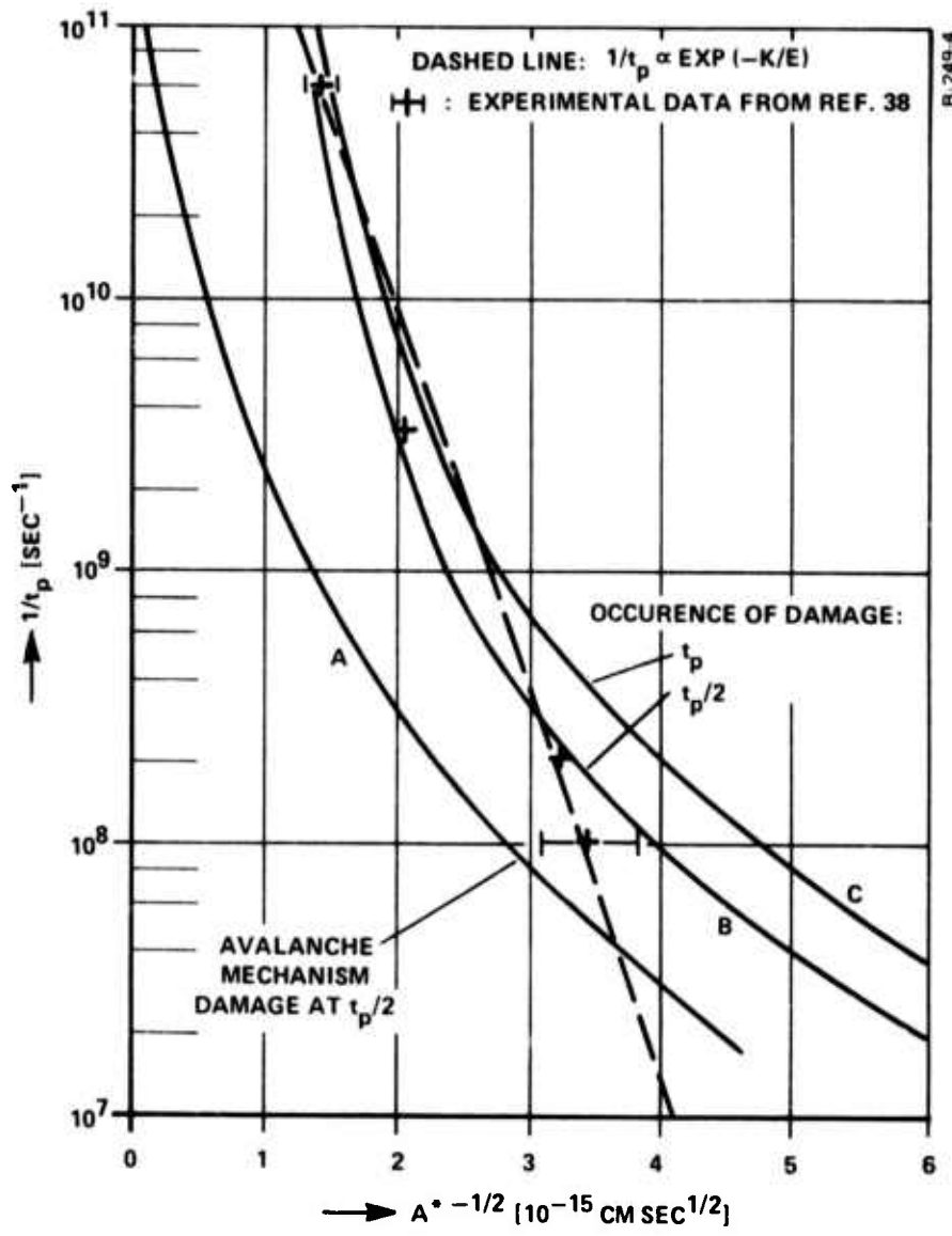
Figure 5 - Dependence of the intrinsic damage threshold on the ruby laser pulse duration for NaCl; damage criterion: n_c = 1 \times 10^{18} \text{ cm}^{-3} A. Avalanche ionization only [ \omega_i from equation (14)], damage at t = t_p/2 B. Avalanche and multiphoton, damage occurs at t = t_p/2 C. Avalanche and multiphoton, damage occurs at t = t_p For B and C: \sigma_5 = 0.5 \times 10^{-141} \text{ cm}^{10} \text{ sec}^4 , standard sample Note: The experimental data were obtained at the Nd-frequency, however, the results for the ruby frequency are practically identical. 40
