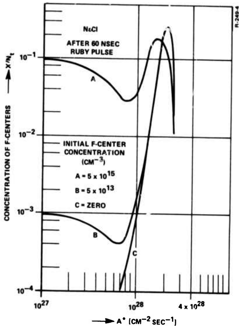
Figure 8 - Laser induced concentration of F-center in a NaCl crystal containing 5 \times 10^{16} \text{ Cl}^- -vacancies as a function of the ruby laser peak plus for various initial F-center densities. In this case, the damage thresholds are (in 10^{28} \text{ cm}^{-2} \text{ sec}^{-1} ):
