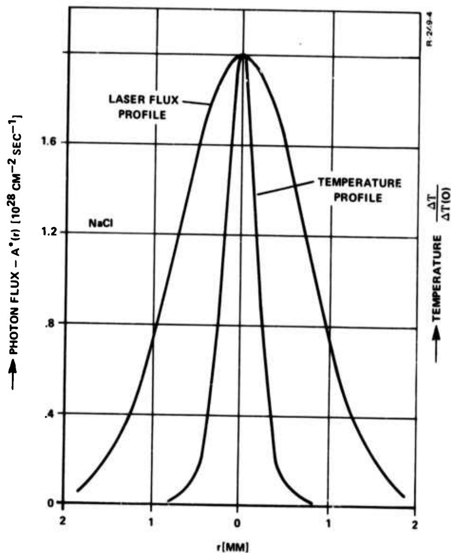
Figure 10 - Laser flux profile and normalized temperature profile of the standard NaCl crystal that was exposed at room temperature to a 60 nsec TEM 00 mode ruby laser pulse having a peak flux A^* = 2 \times 10^{28} photons per cm 2 and sec. The temperature increase \Delta T at the center of the pulse was 390.4°C.
