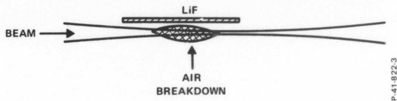
Figure 16 - Exoelectron images of a LiF single crystal that was placed parallel to the axis of the laser beam waist so that the air breakdown spark occurred in front of the crystal as shown schematically.
