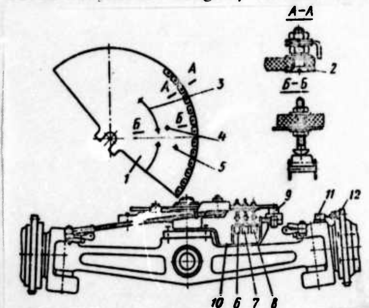
Fig. 3: General view and details of measuring device.
