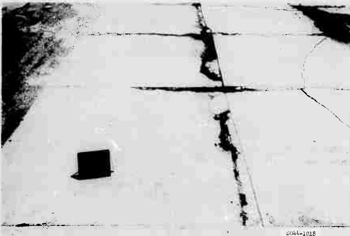
Figure A49. Subitem 5a, lane 2, rigid pavement test section, after 950 coverages by 240-kip twin-tandem assembly
