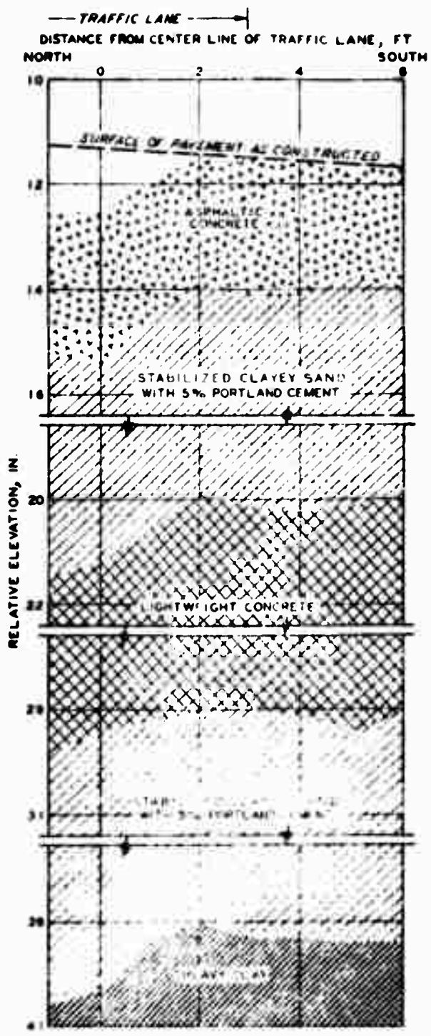
Figure 10. Cross-section profile of subgrade, base, flexible pavement test section, Station 1+50 after 140 passages of 10-ton single-wheel assembly
