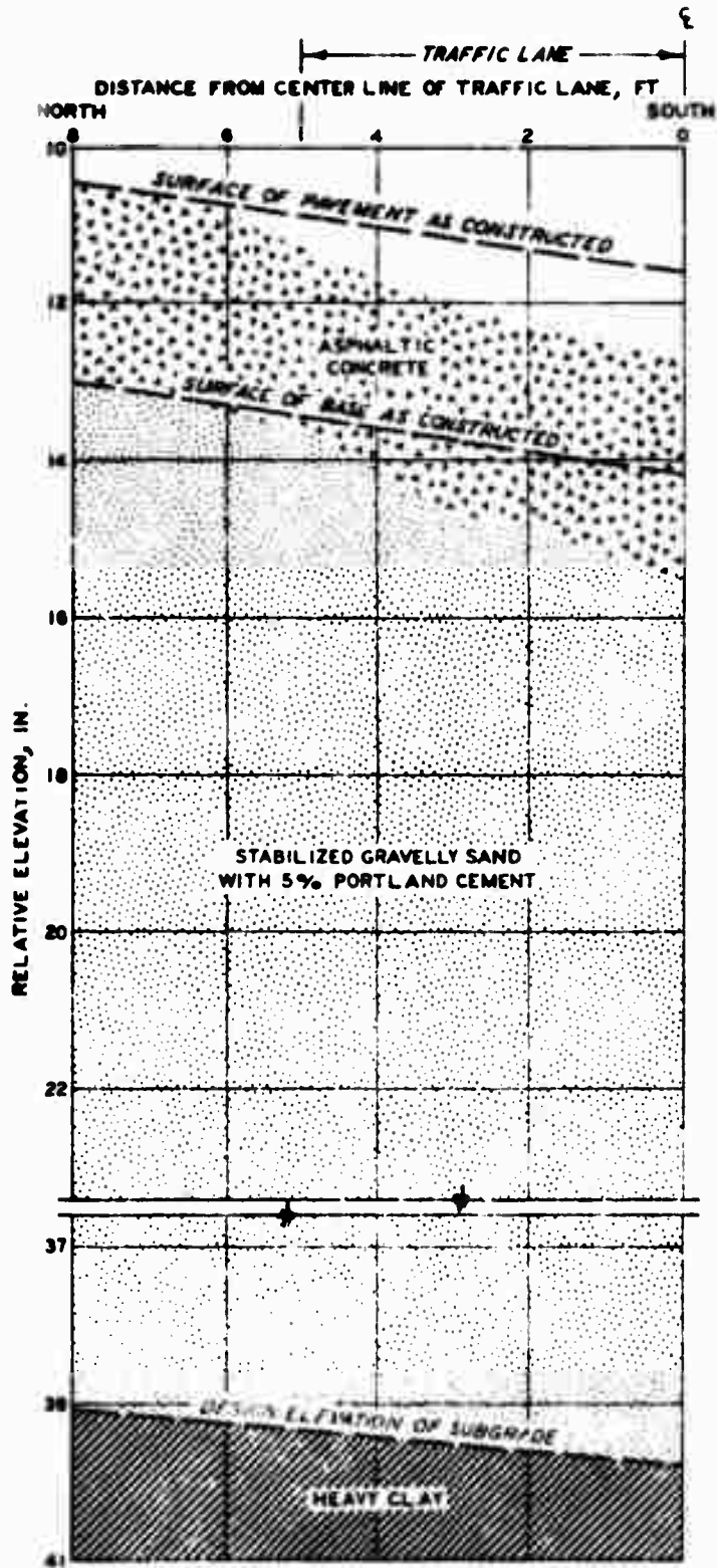
Figure 175. Test pit profile of item 3, lane 1, flexible pavement test section. Station 1+04 after 7820 coverages of 200-kip twin-tandem assembly
