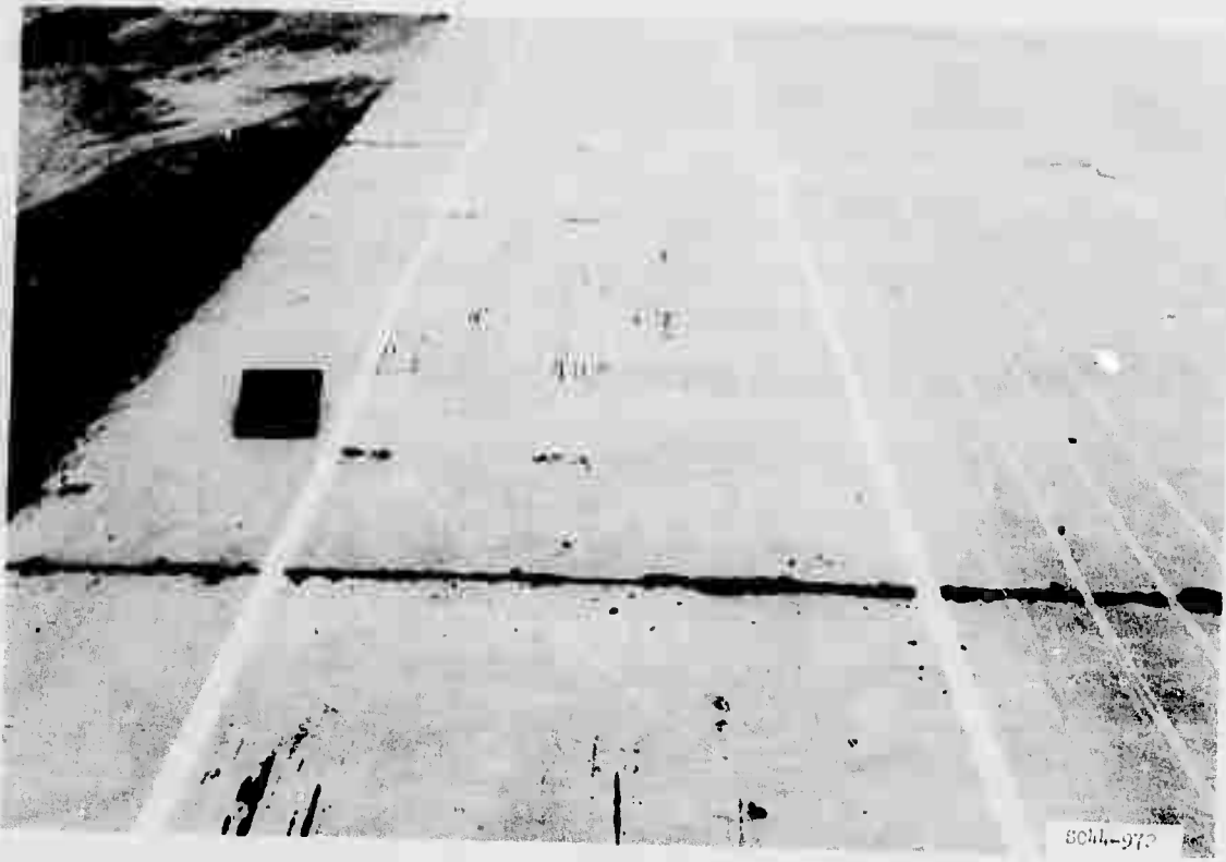
Figure A44. Item 4, lane 2, rigid pavement test section, prior to traffic
