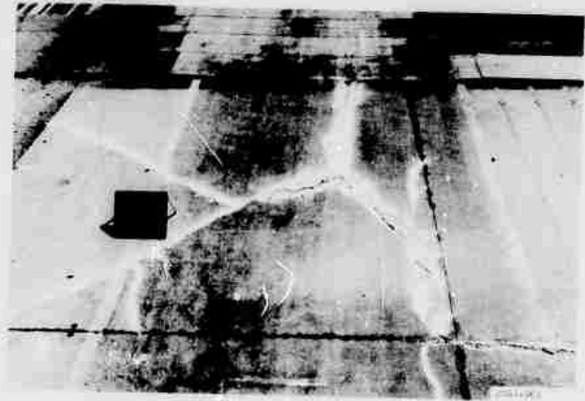
Figure A56. Subitem 5d, lane 2, rigid pavement test section, after 200 coverages by 240-kip twin-tandem assembly
