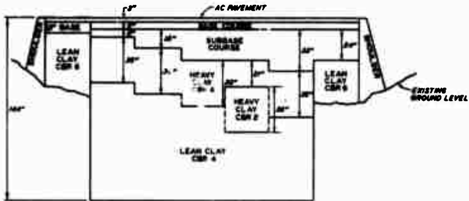
SECTION A-A FLEXIBLE PAVEMENT TEST SECTION
