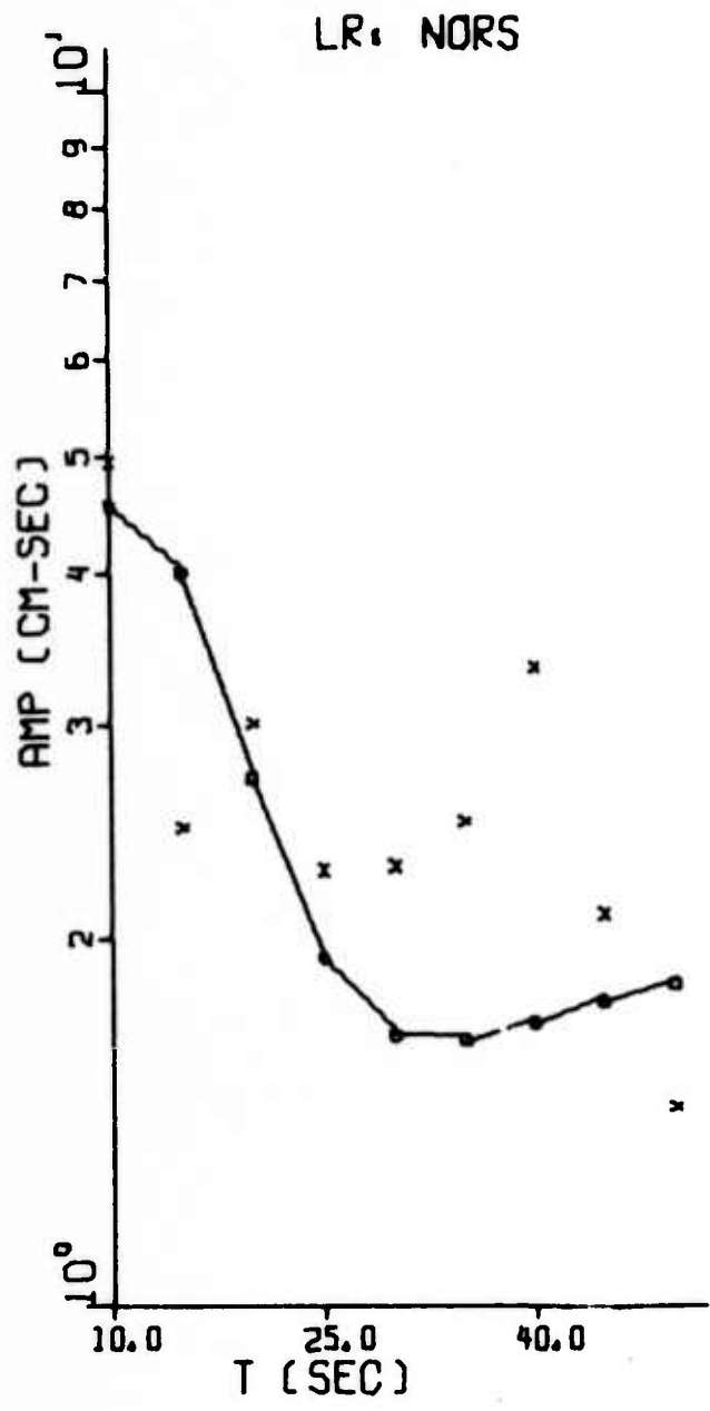
FIGURE III-5 AMPLITUDE SPECTRA LX*TURN3*003
