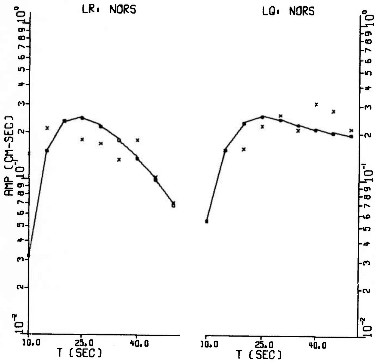
FIGURE III-9 AMPLITUDE SPECTRA LX+CENAP+50
