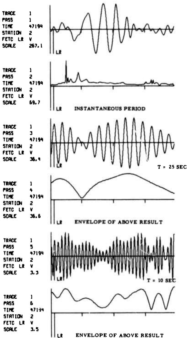
FIGURE C-1 NARROW BAND FILTER ANALYSIS
