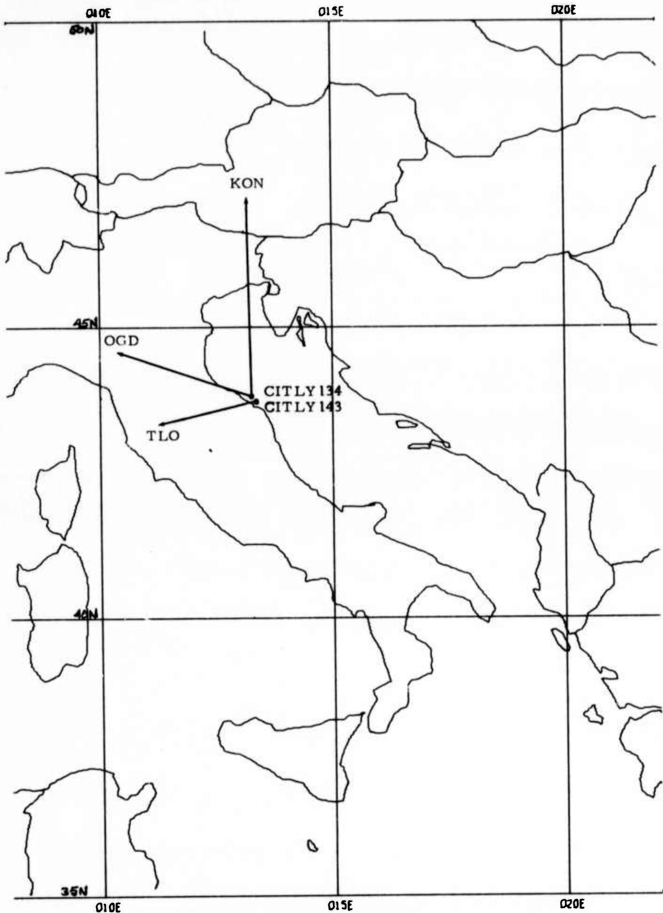
FIGURE D-1 LOCATIONS OF TWO, LOW MAGNITUDE ITALIAN EVENTS RECORDED AT THREE VLPE STATIONS D-2
