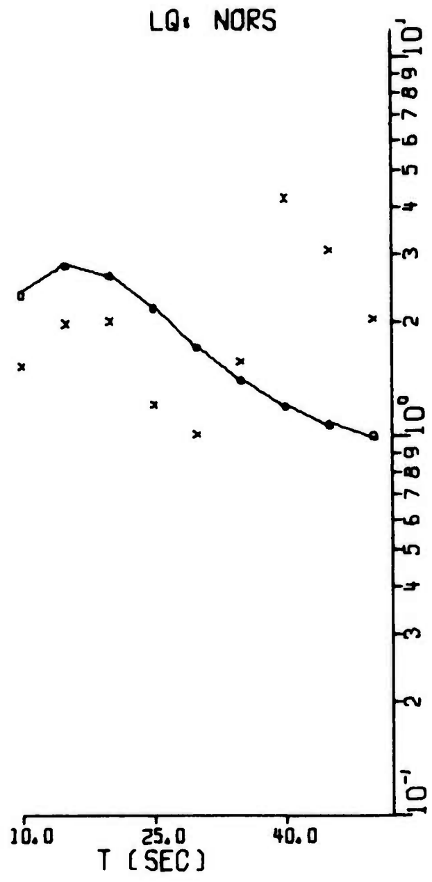
FIGURE III-5 AMPLITUDE SPECTRA LX*TURN3*003
