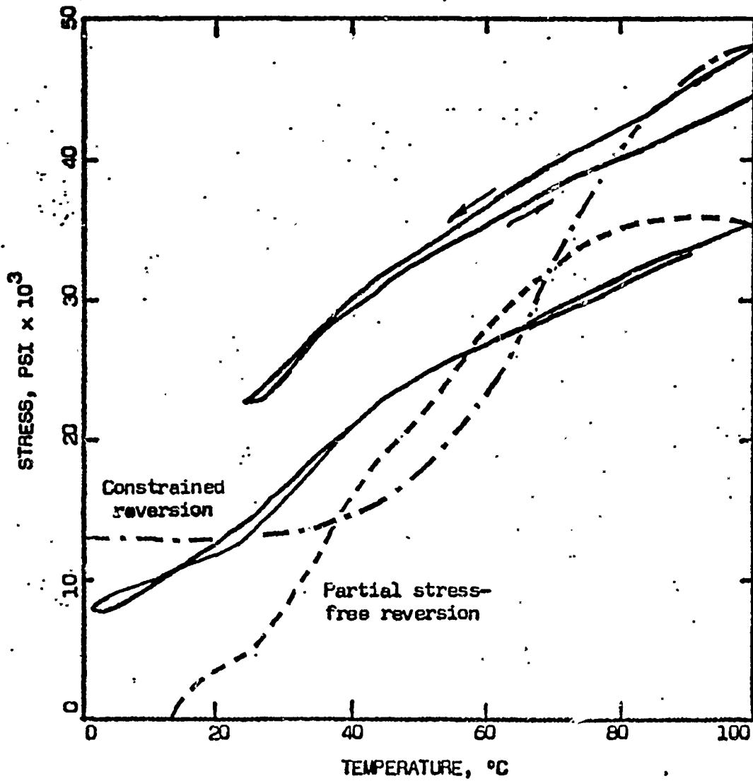
FIGURE 21. Reversion-stress recovery after cooling below the A_f . True stress vs true temperature.
