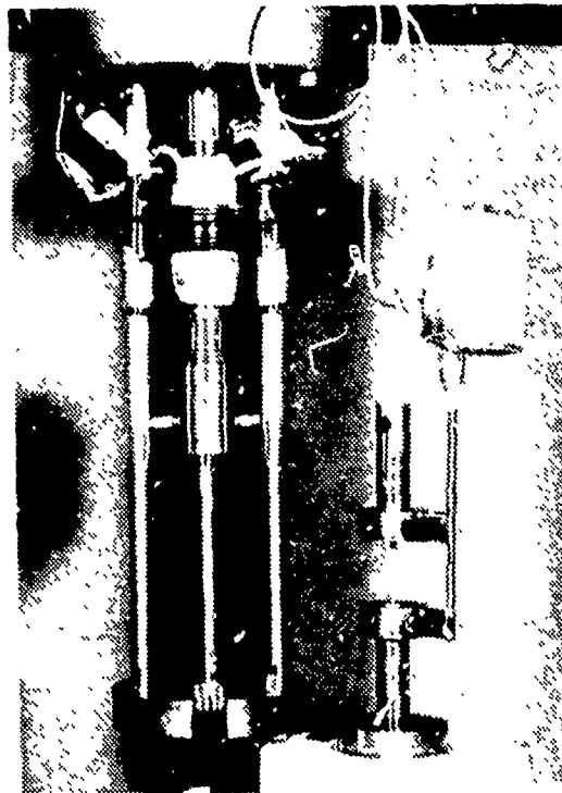
FIGURE 6. The testing rig with grip assembly and specimen ready to be installed.
