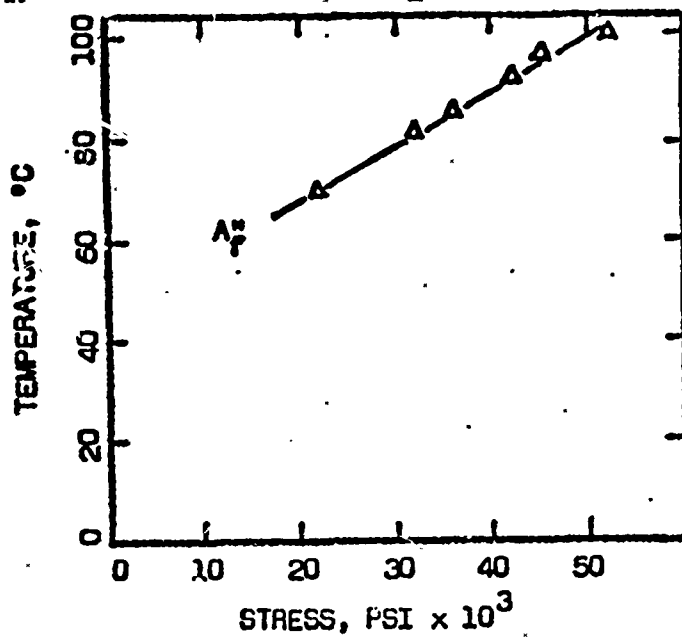
FIGURE 13. Increases in the transformation temperature due to increasing internal stress during constrained stress reversion. Temperature vs external stress.
