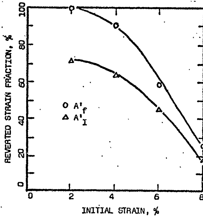
FIGURE 18. The fraction of the initial strain reverted at A'_I and A'_f vs the initial strain.
