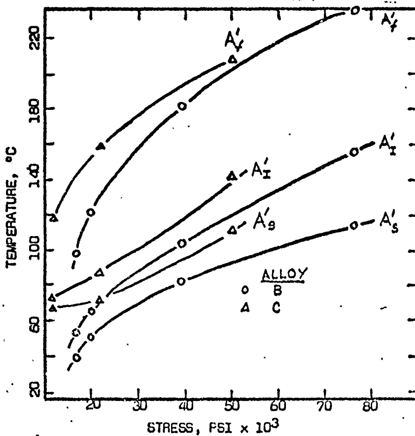
FIGURE 14. Increases in the transformation temperatures due to constant external stress during strain reversion. Temperature vs external stress (from data of Reference 2).
