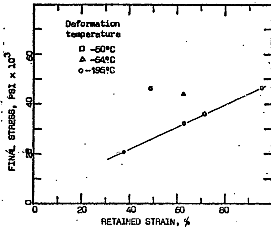
FIGURE 11. Increasing reversion stress due to greater strain retained in the specimen. Final true stress vs strain retained.
