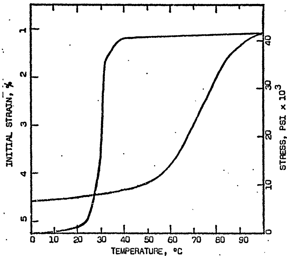
FIGURE 12. Comparison of the transformation temperatures for stress-free reversion and constrained stress reversion. Percent retained strain vs temperature to the left, and reversion stress vs temperature to the right.
