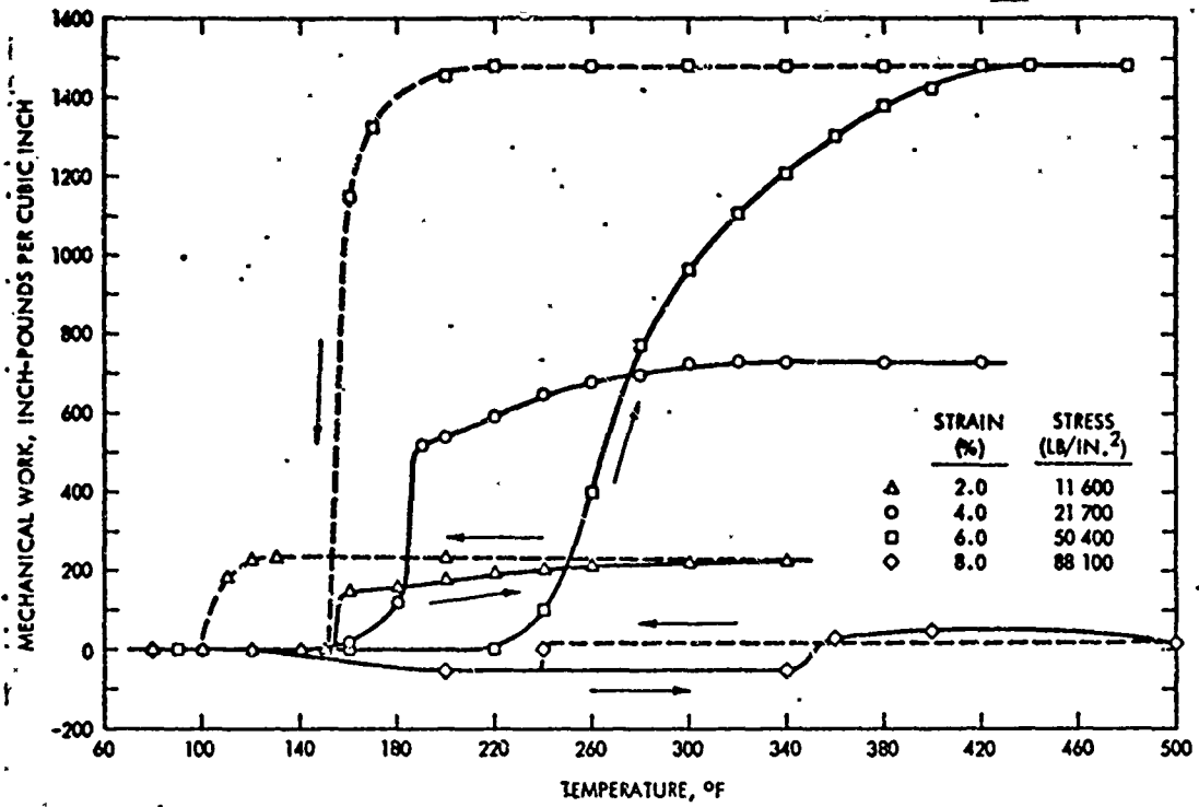
FIGURE 17. Mechanical work performed during strain reversion of alloy C. Specific work vs temperature.
