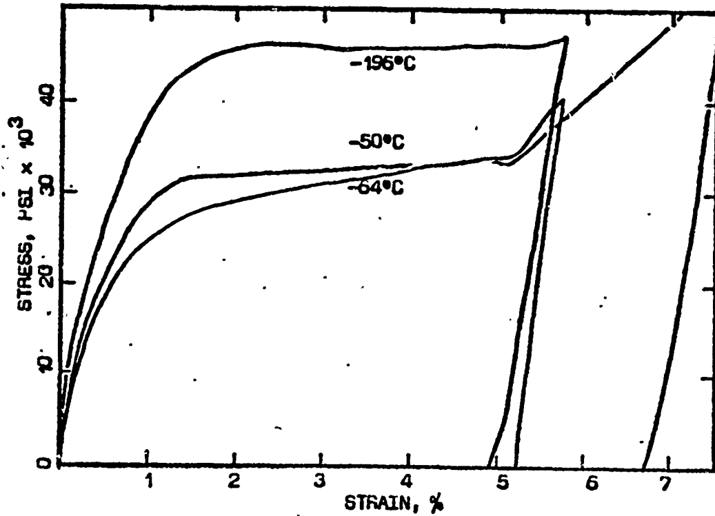
FIGURE 8. True stress vs true strain for martensitic NiTi at various temperatures below M_f .
