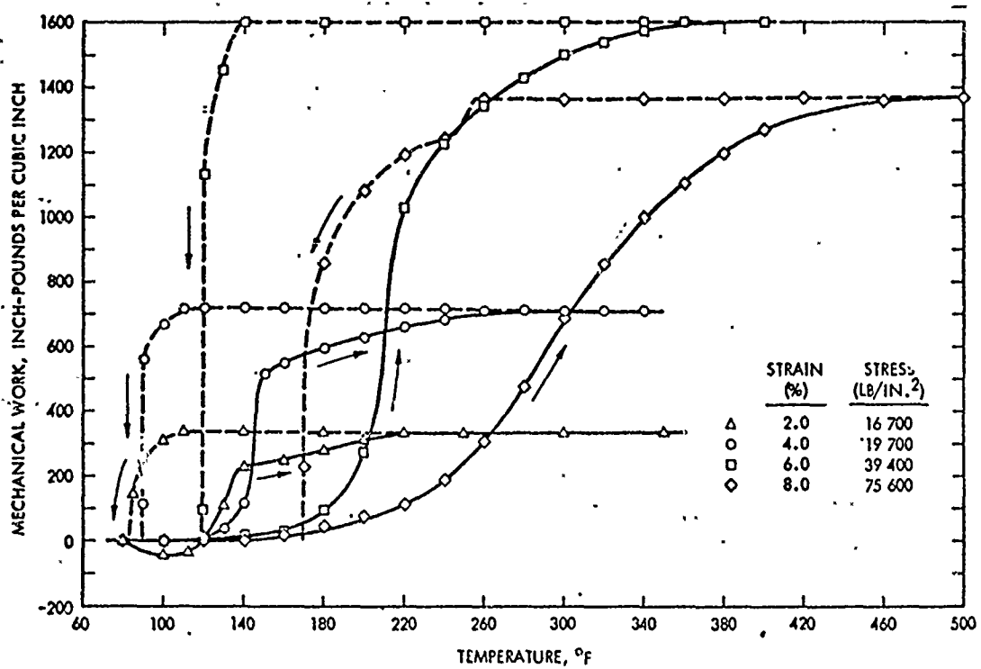
FIGURE 16. Mechanical work performed during strain reversion of alloy B. Specific work vs temperature.
