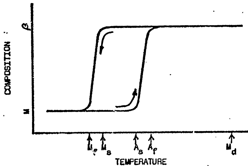
FIGURE 2. The thermal hysteresis curve for the stress-free transformations of thermal martensite and austenite.
