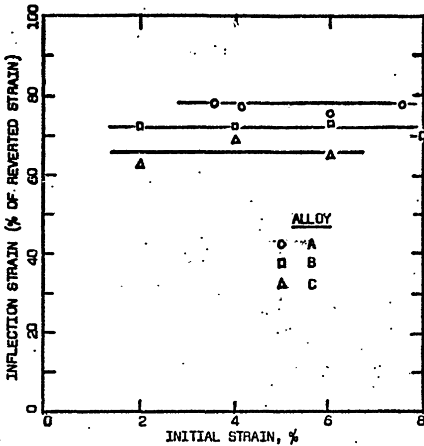
FIGURE 19. The occurrence of A'_I as a fraction of the total reverted strain in three alloys. Percent of reverted strain prior to the inflection vs the initial strain.
