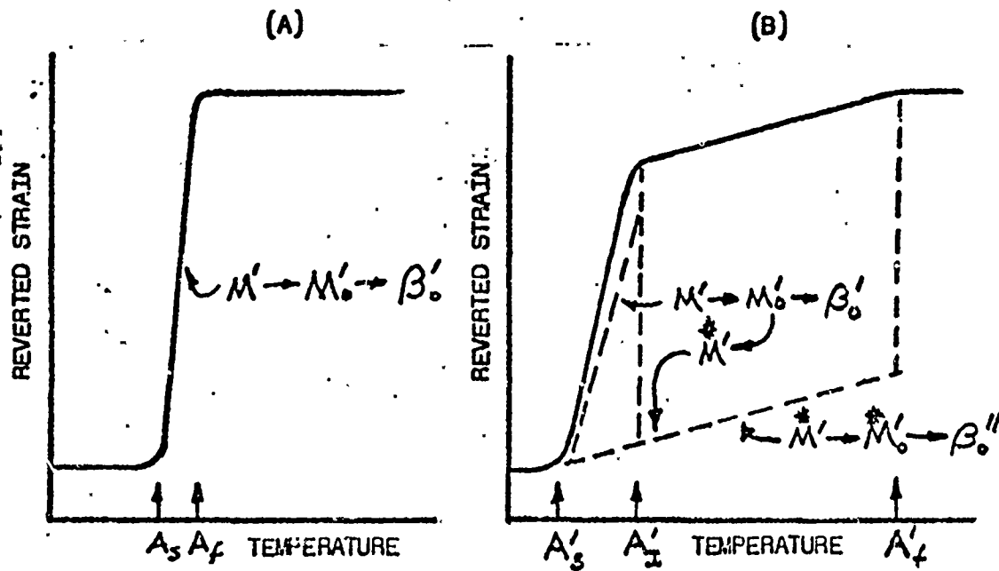
FIGURE 20. Schematic model of a reversion process (hypothetical): a. reverted stress-free, b. stress-reverted with an inflection point.
