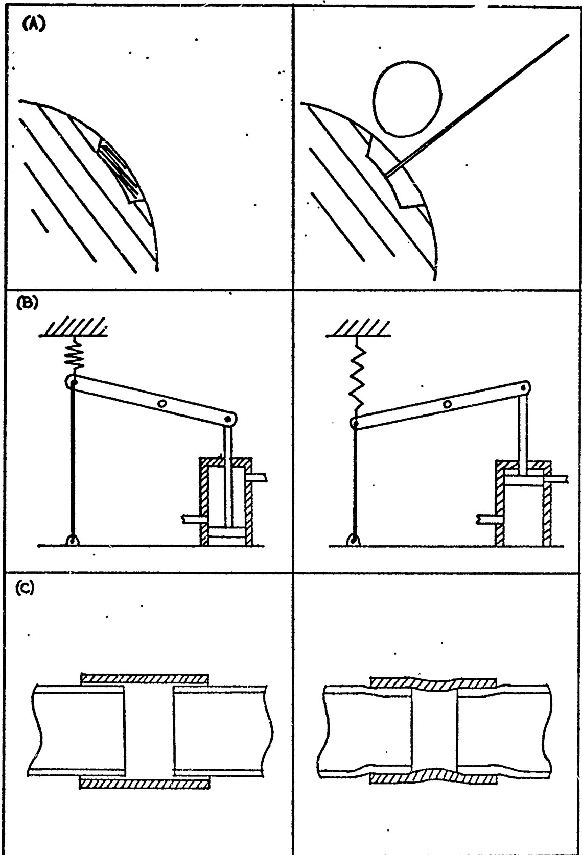
FIGURE 3. Selected applications of the shape-memory effect: (A) shape recovery, (B) mechanical work, (C) constraining stress.
