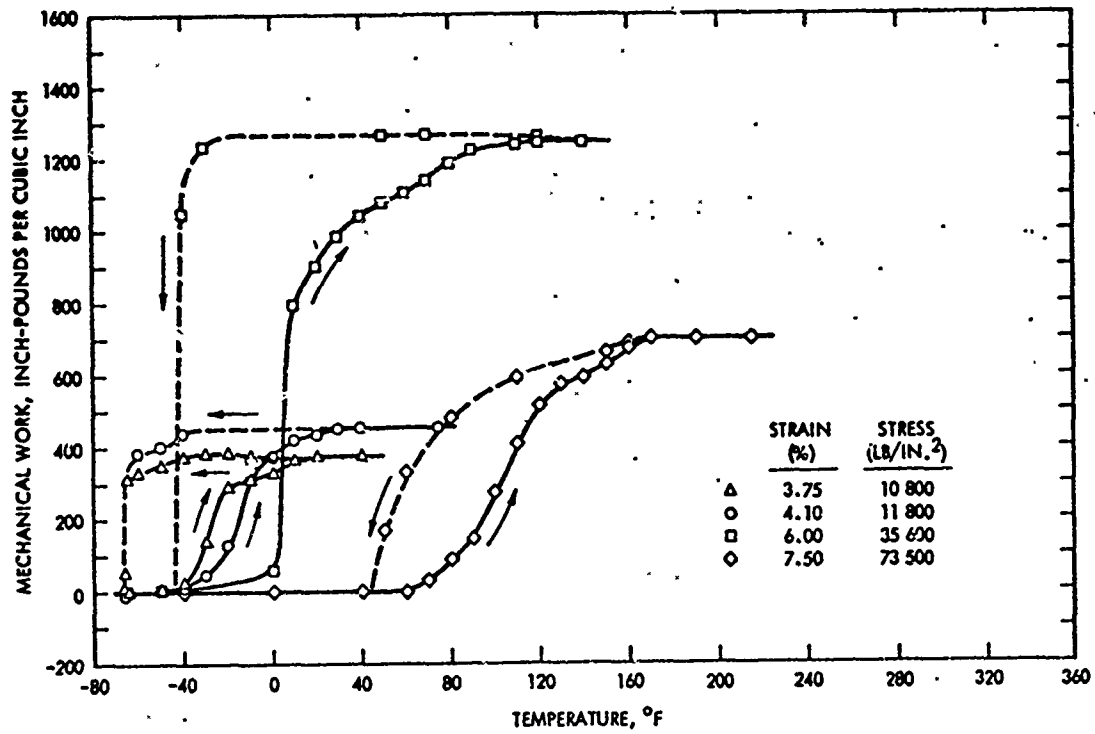
FIGURE 15. Mechanical work performed during strain reversion of alloy A. Specific work vs temperature.
