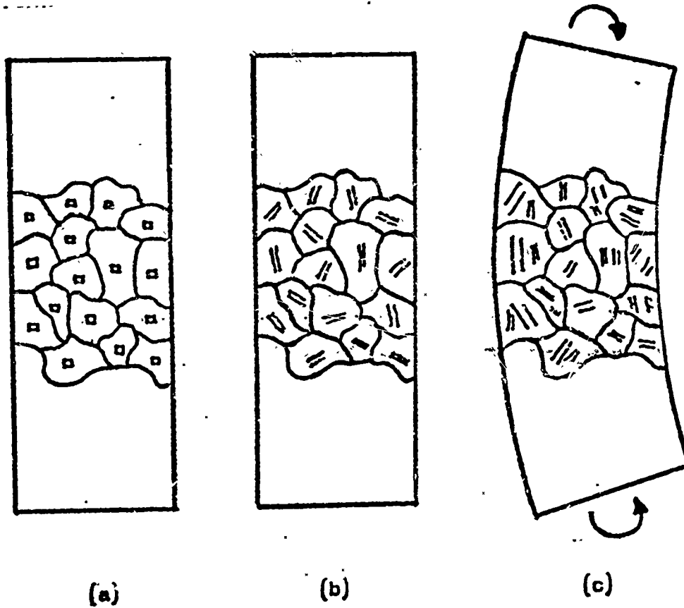
FIGURE 1. Schematic representation of the formation of deformation martensite from thermal martensite.
