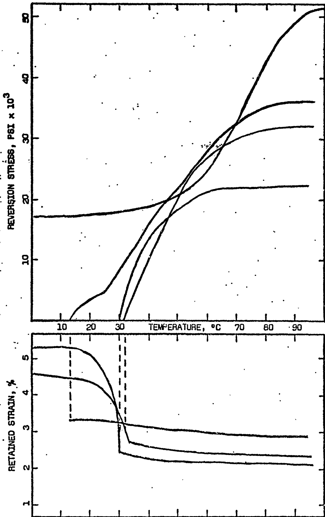
FIGURE 10. Comparison of the reversion stress for partial loss of initial strain. True stress and true strain vs specimen temperature.
