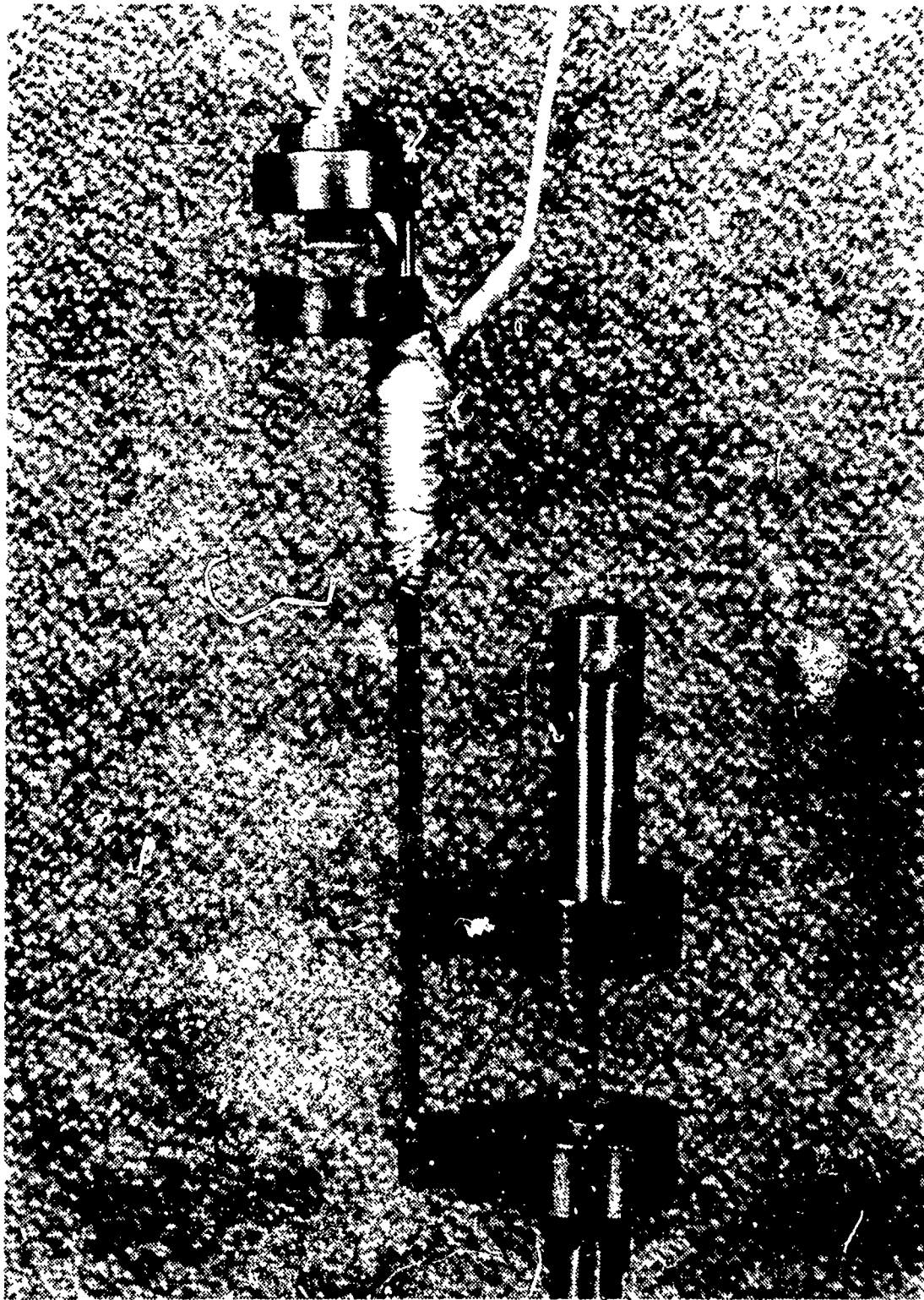
FIGURE 4. The serrated grip assembly with the proximeter extensometer mounted.
