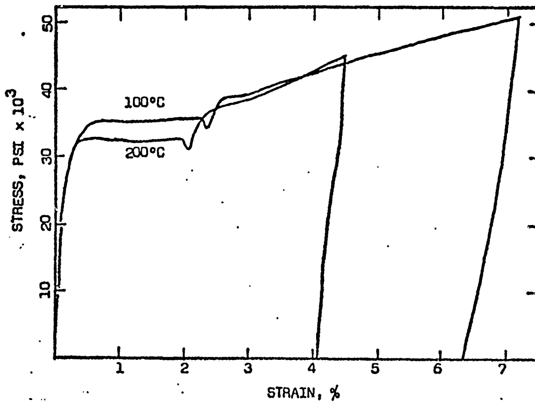
FIGURE 9. True stress vs true strain for austenitic NiTi at two temperatures above the M_d .
