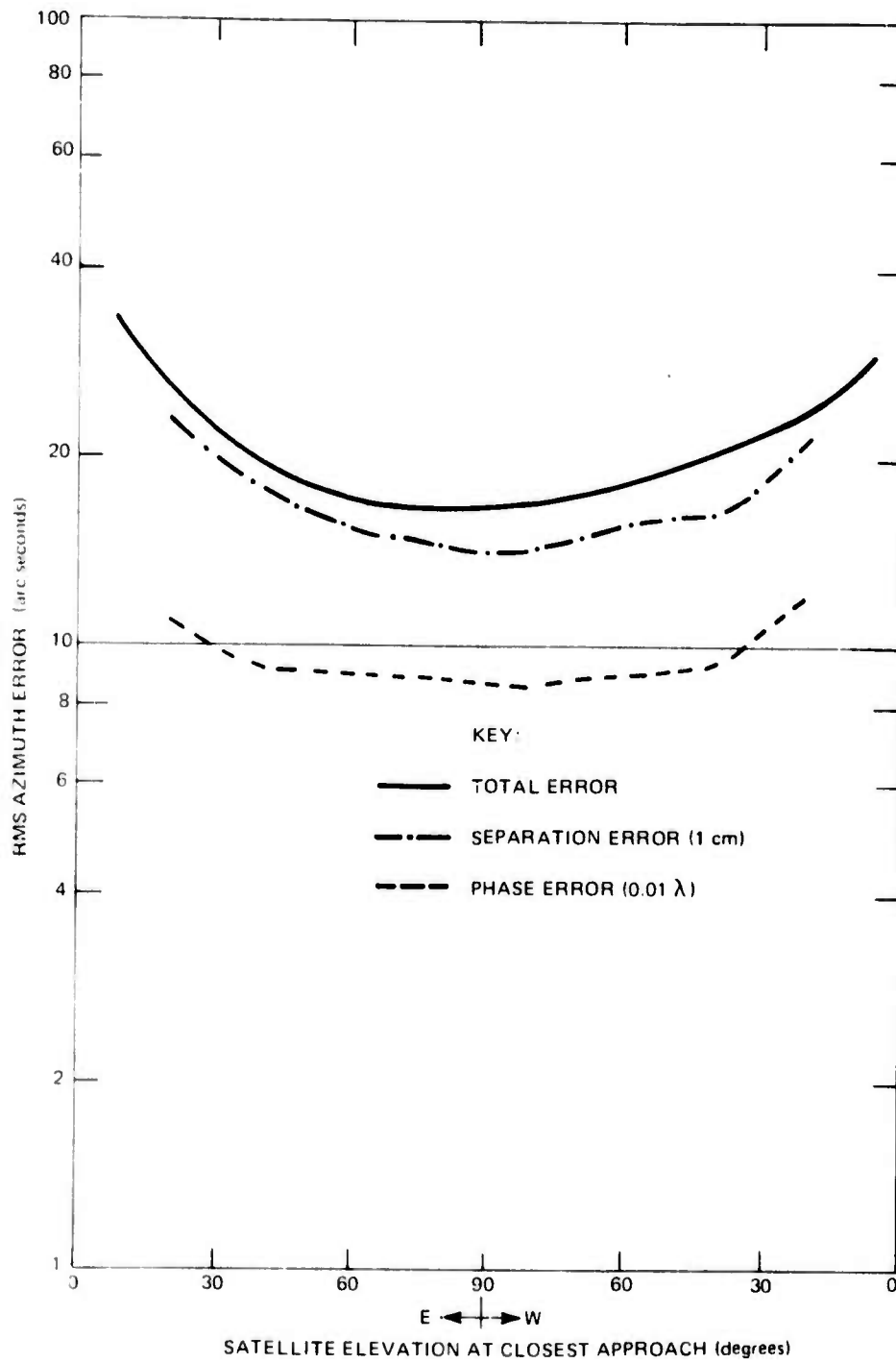
Fig B 3 RMS AZIMUTH ERROR FOR SATELLITE PASSES OVER APL (AZ = 60°)
