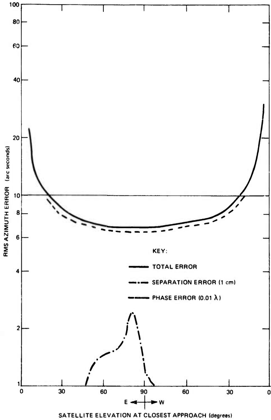
Fig. B-4 RMS AZIMUTH ERROR FOR SATELLITE PASSES OVER APL (AZ = 90°)
