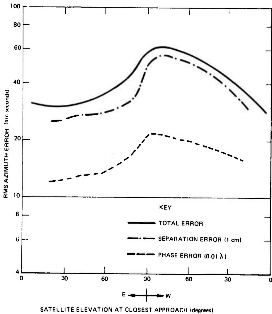
Fig. B-2 RMS AZIMUTH ERROR FOR SATELLITE PASSES OVER APL (AZ = 30°)
