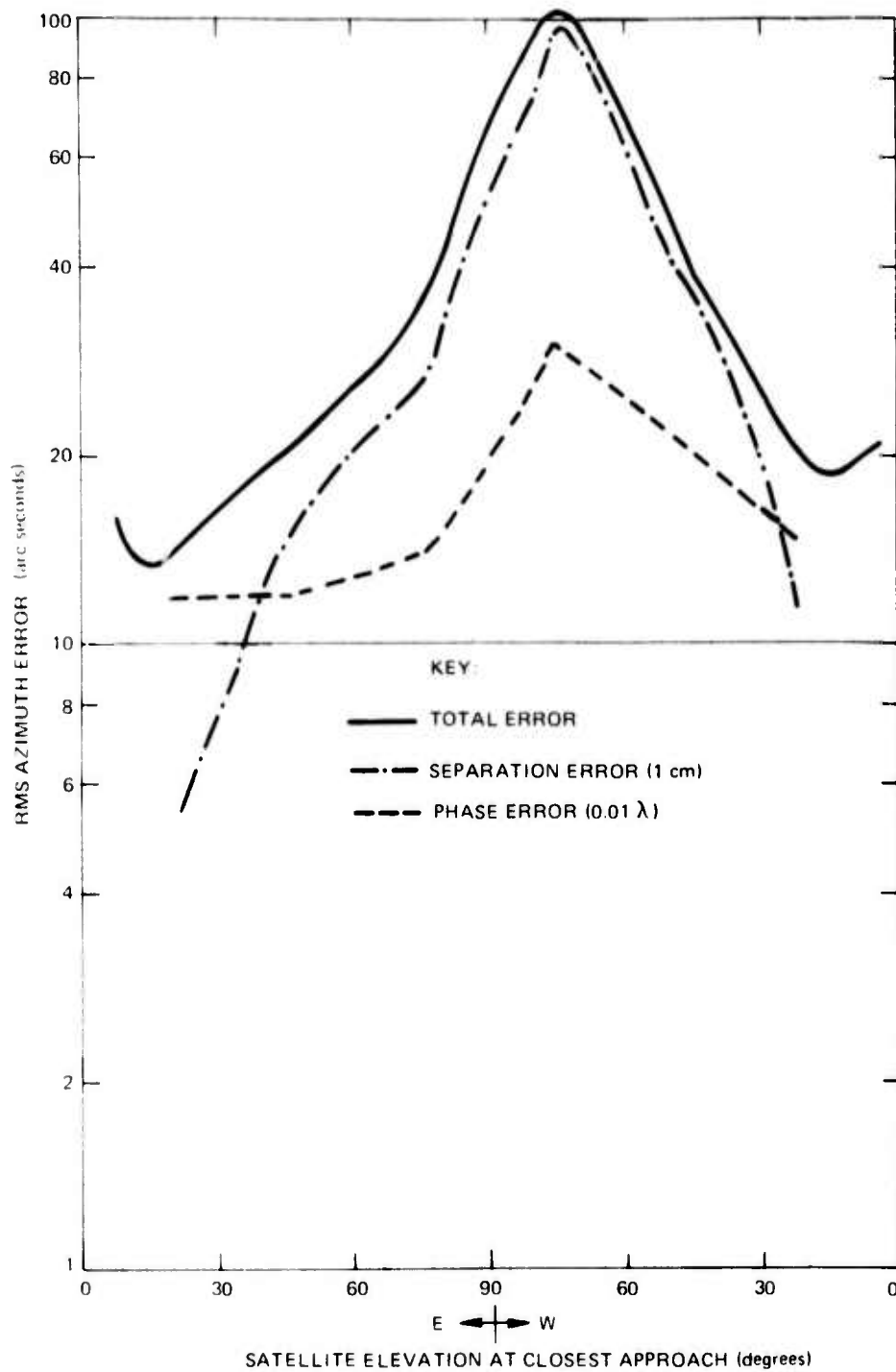
Fig B 1 RMS AZIMUTH ERROR FOR SATELLITE PASSES OVER APL ( AZ = 0^\circ )
