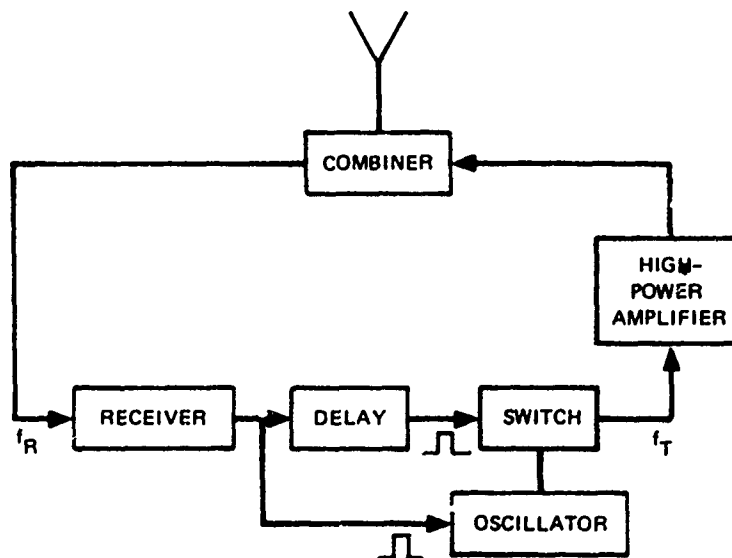
FIGURE VII-14 HIGH-POWER BEACON TRANSPONDER
