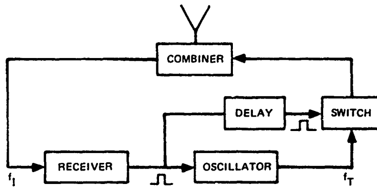
FIGURE VII-13 MEDIUM-POWER BEACON TRANSPONDER
