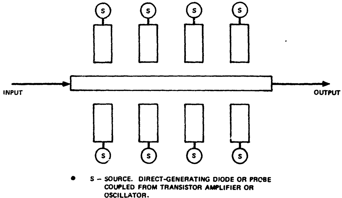
FIGURE VII-8 ITERATIVE POWER-COMBINER SCHEME FOR AMPLIFIERS AND OSCILLATORS
