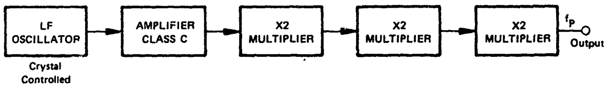
(a) CRYSTAL-CONTROLLED OSCILLATOR/VARACTOR MULTIPLIER COMBINATION
