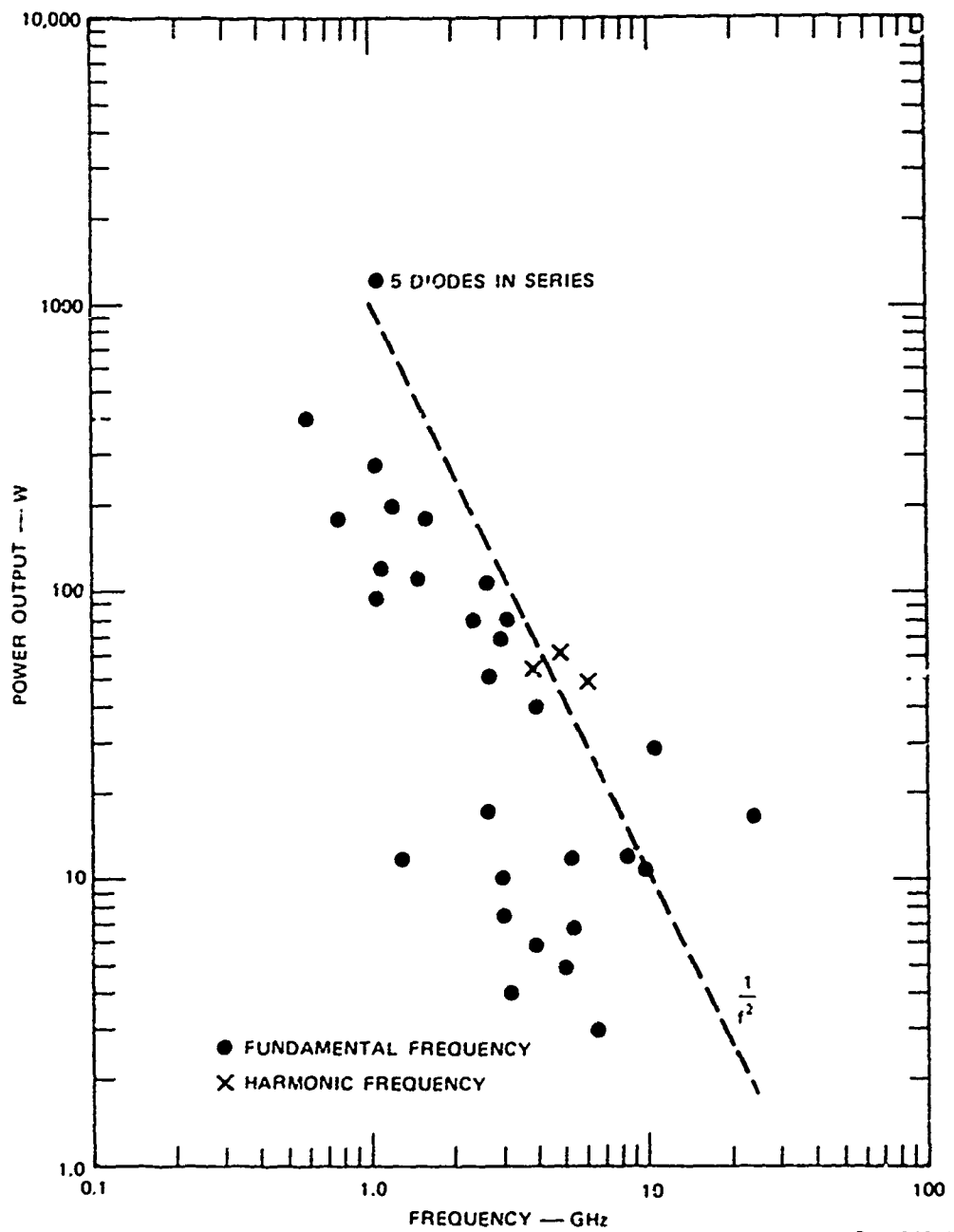
FIGURE VI-2 PERFORMANCE OF TRAPATT DIODES — 1973
