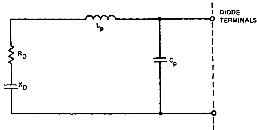
FIGURE V-3 IMPATT DIODE PACKAGE EQUIVALENT CIRCUIT
