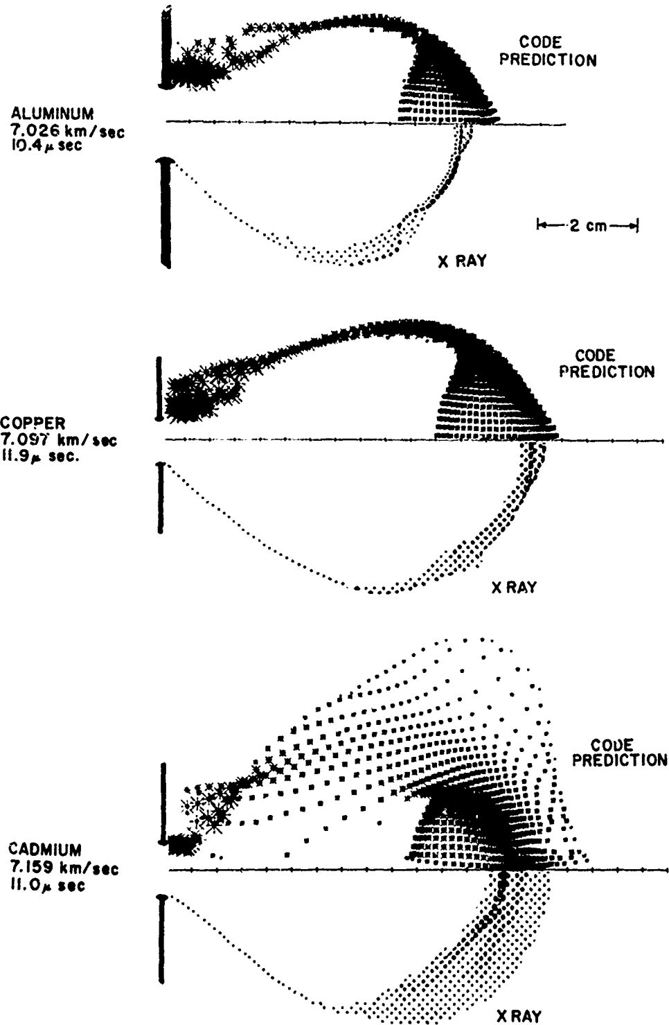
Figure 7. Comparisons of Observed Material Distributions of Debris Clouds With Computer Predictions.
