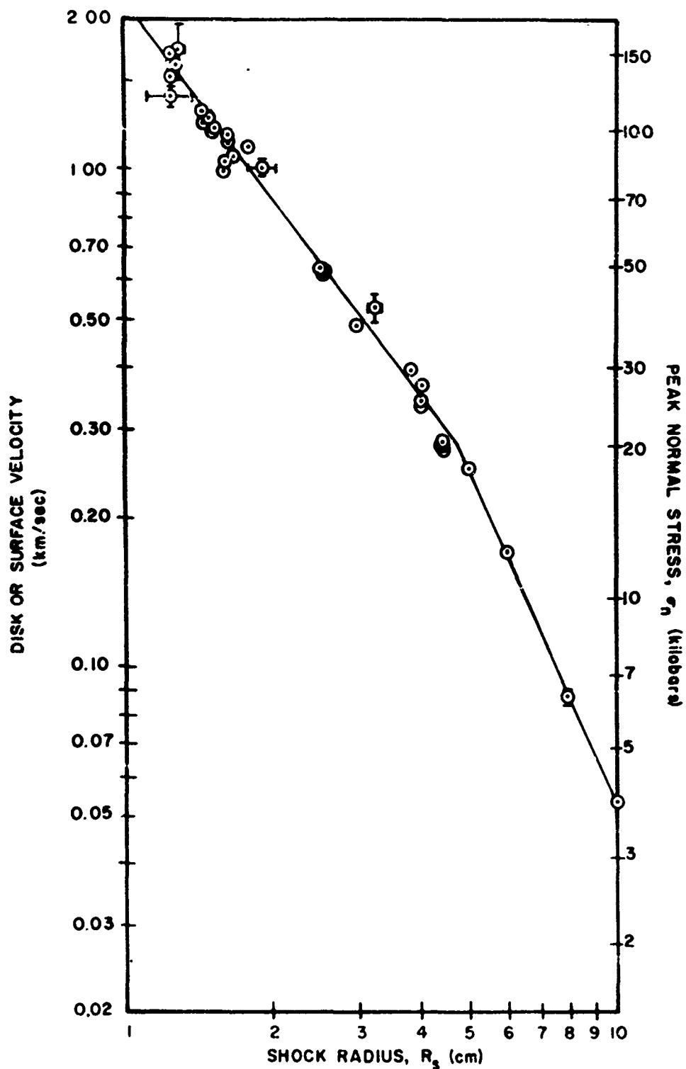
Figure 21. Typical Results of Peak Shock Wave Pressure Experiments Showing Peak Pressure vs. Depth Into Target for 1100 A. Aluminum Targets.
