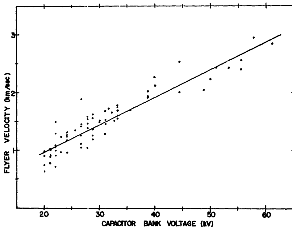
Figure 25. Flyer Velocity vs. Charging Voltage of the High Voltage Bank.
