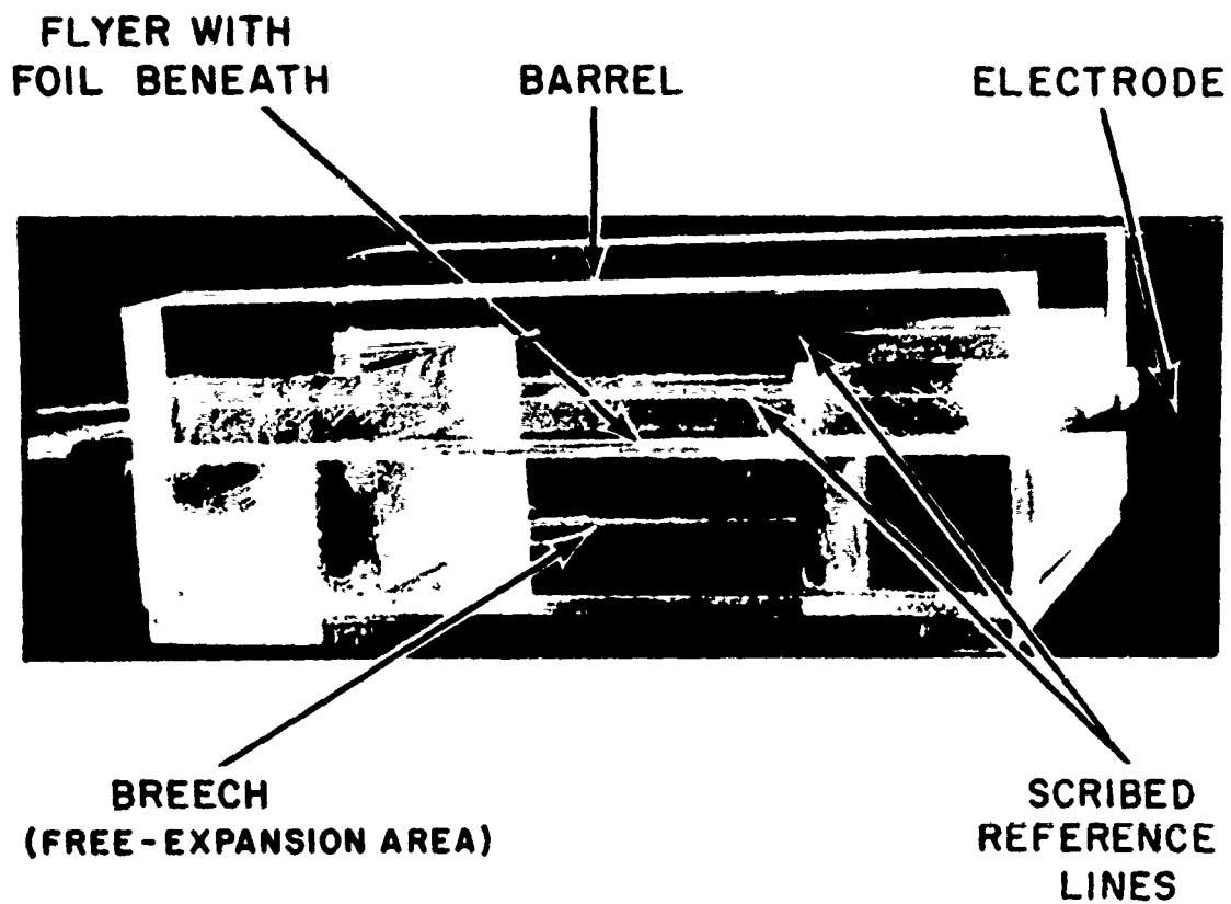
Figure 30. Intermediate Velocity Transducer (RIFL).
