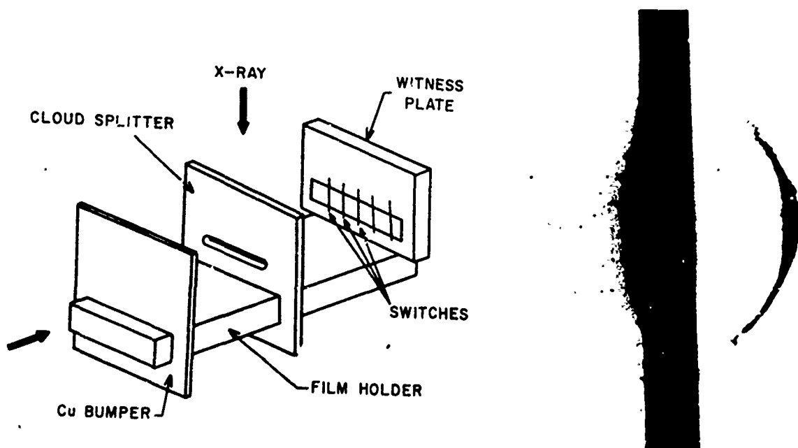
Figure 6. Experiment for Dissecting Debris Cloud to Determine Material Distribution.
