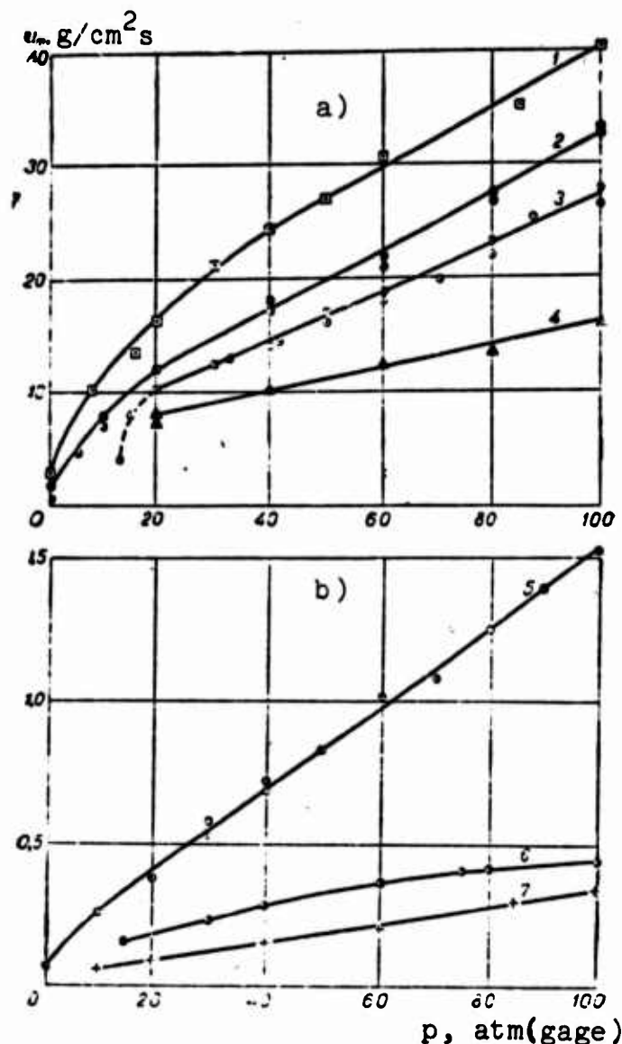
The dependence of the combustion rate of salts of tetraamine copper (II), on the pressure. a) rapid-burning anions: 1 - BrO 3 - , 2 - ClO 3 - , ClO 4 - , 4 - MnO 4 - ; b) slow-burning salts of anions: 5 - NO 3 - , 6 - NO 2 - , 7 - IO 3 - .
