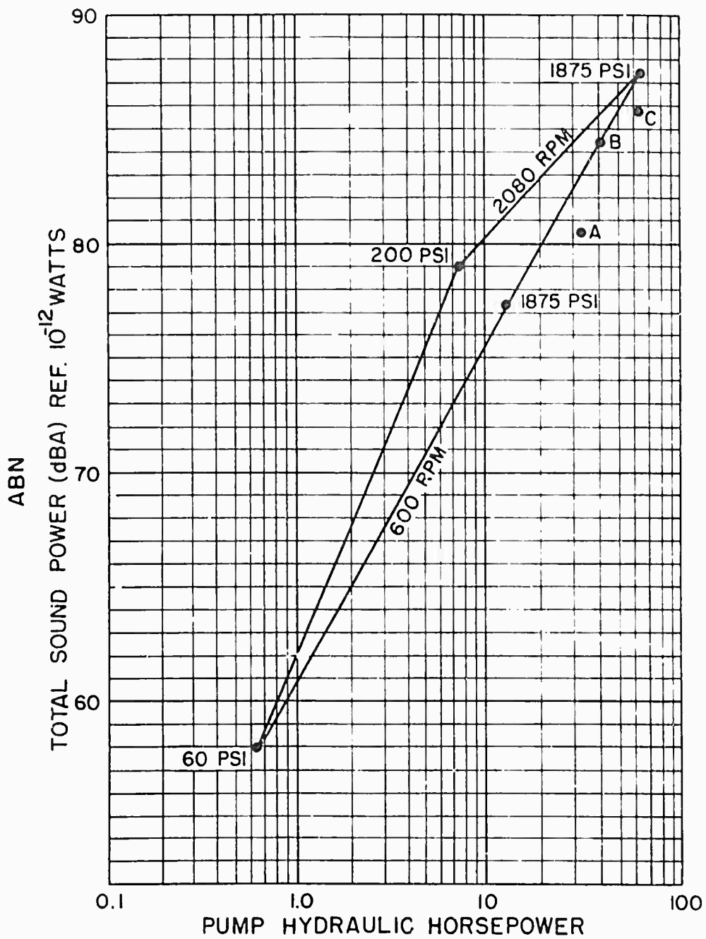
Fig. 4-1. ABN levels for pump group 5R714 for military D7F(DV29) tested as received. Pressures shown are the same for both pump outputs. Point (A) 2080 RPM, shaft side pump 200 PSI, end pump 1875 PSI; point (B) 2080 RPM, shaft side pump 1875 PSI, end pump 200 PSI; point (C) 2080 RPM, 1875 PSI with relief valve loading. All other points use needle valve load.
