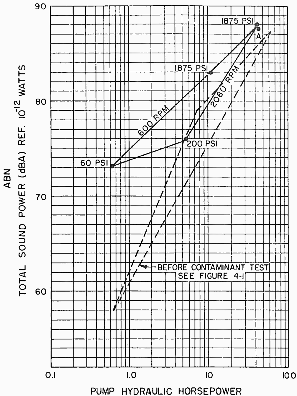
Fig. 4-4. ABN levels for pump group 5R714 after contaminant test. Pressures shown are the same for both pump outputs, Point (A) 2080 RPM, 1875 PSI, with relief valve loading. All other points use needle valve load.
