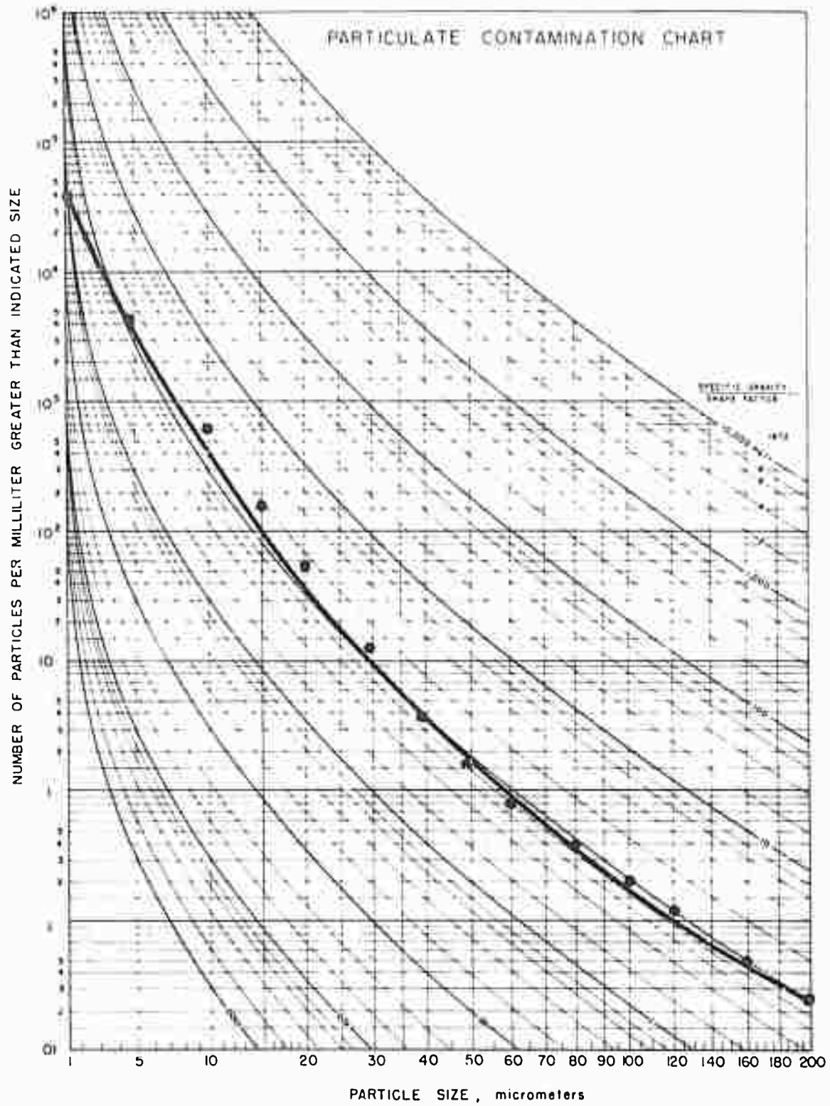
Fig. 4-3. Contaminant Tolerance Profile of Pump Group 5R714 for 1000 Hour Life.
