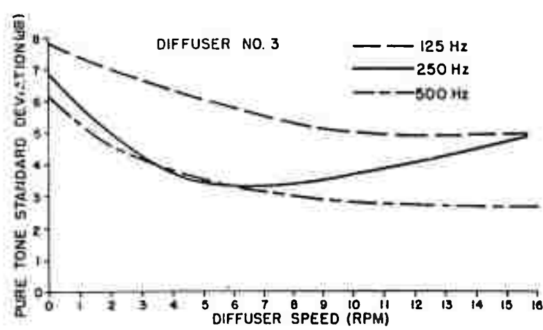
Fig. 3-1. Pure Tone Standard Deviation in OSU-FPRC Reverberant Facility for Each of Three Diffusers Operating Separately at Various Speeds.
