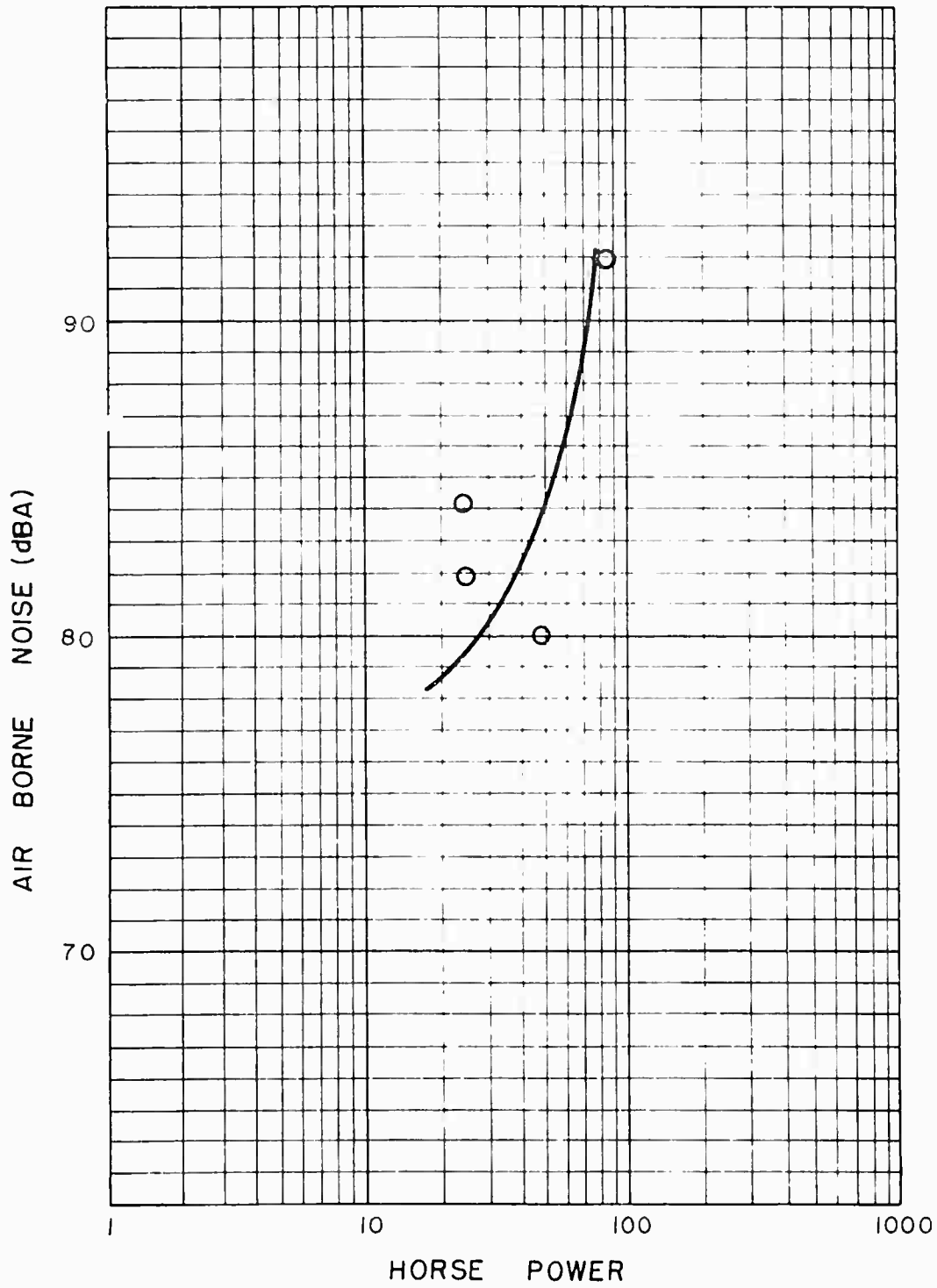
Fig. 6-1. Airborne Noise Level Versus Horsepower for Valve 2.
