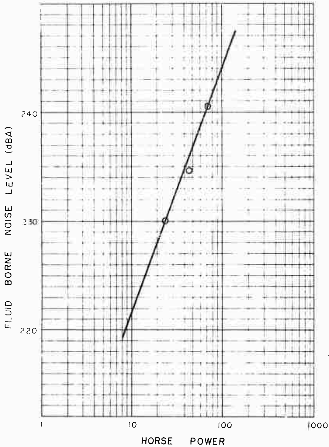
Fig. 6-4. Fluid-Borne Noise Levels Versus Horsepower for Valve 2.
