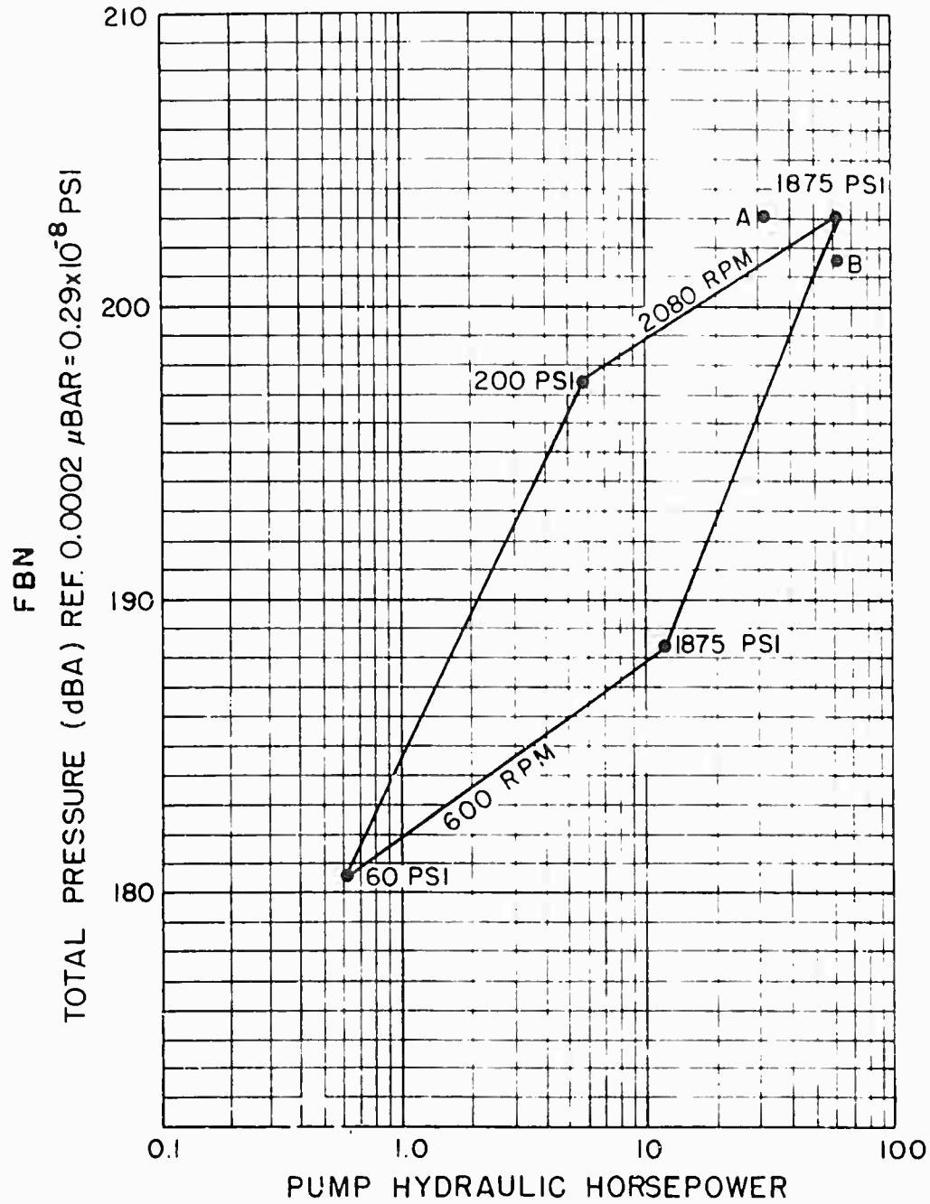
Fig. 4-2. FBN levels for pump group 5R714 tested as received. FBN measurements are for end pump of pump group. Pressures shown are the same for both pump outputs, Point (A), 2080 RPM, 1875 PSI, end pump, 200 PSI shaft pump. Point (B), 2080 RPM, 1875 PSI with relief valve loading. All other points use needle valve load.
