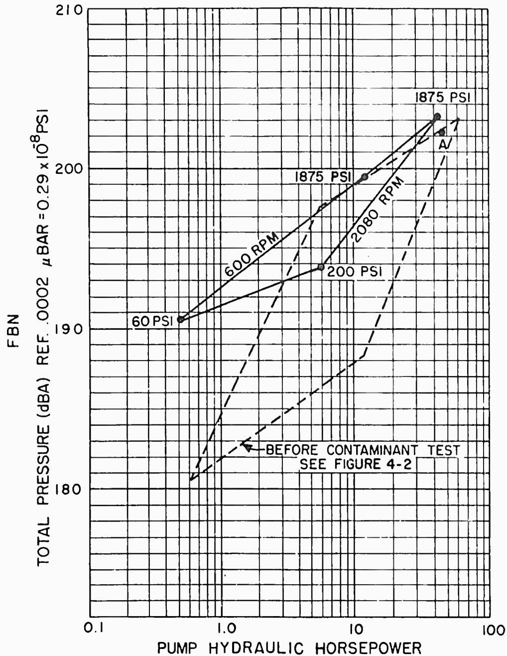
Fig. 4-5. FBN levels for pump group 5R714 after contaminant test. FBN measurements are for end pump of pump group. Pressures shown are the same for both pump outputs Point (A) 2080 RPM, 1875 PSI with relief valve loading. All other points use needle valve load.
