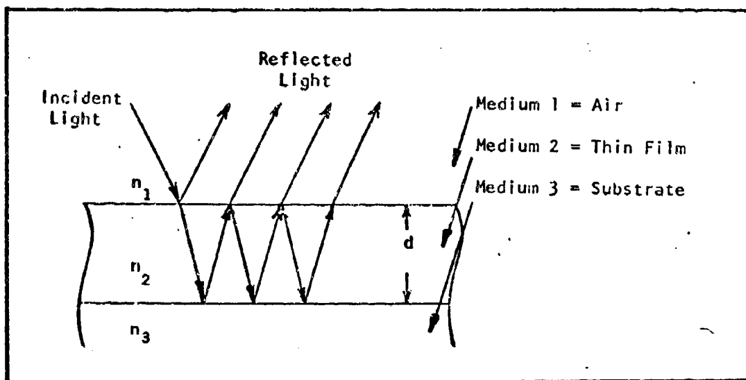
Fig. 4. Three Media Model Used in Interference Fringe Analysis
