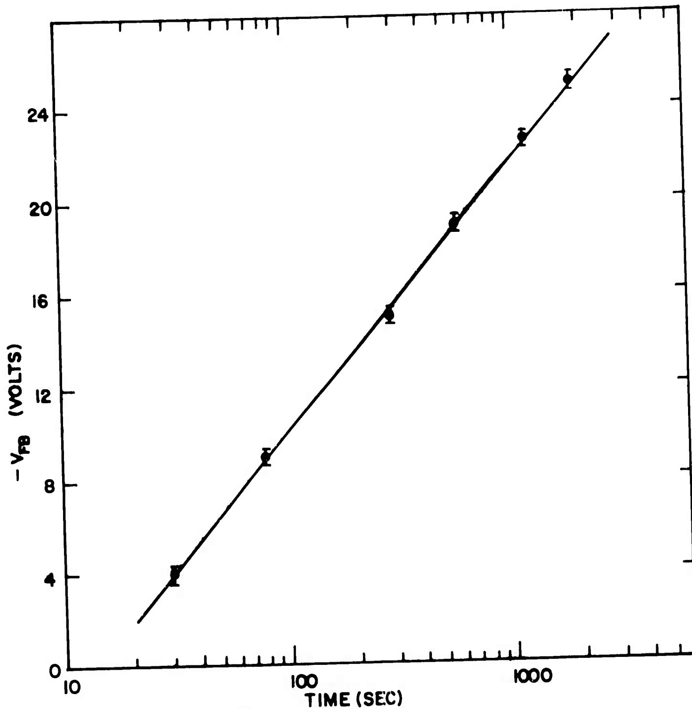
FLAT - BAND VOLTAGE SHIFT vs TIME DUE TO HOLE INJECTION FROM Si INTO \text{SiO}_2 (NEGATIVE CORONA)
