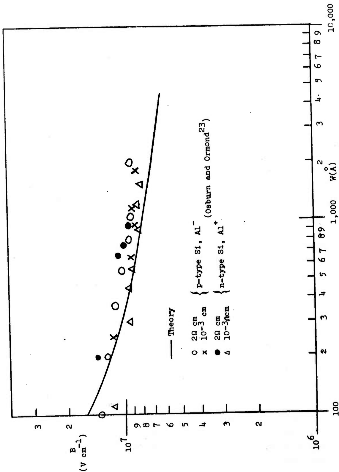
Fig. 50. Dependence of Breakdown Field on Film Thickness (Al-SiO 2 -Si Structure)
