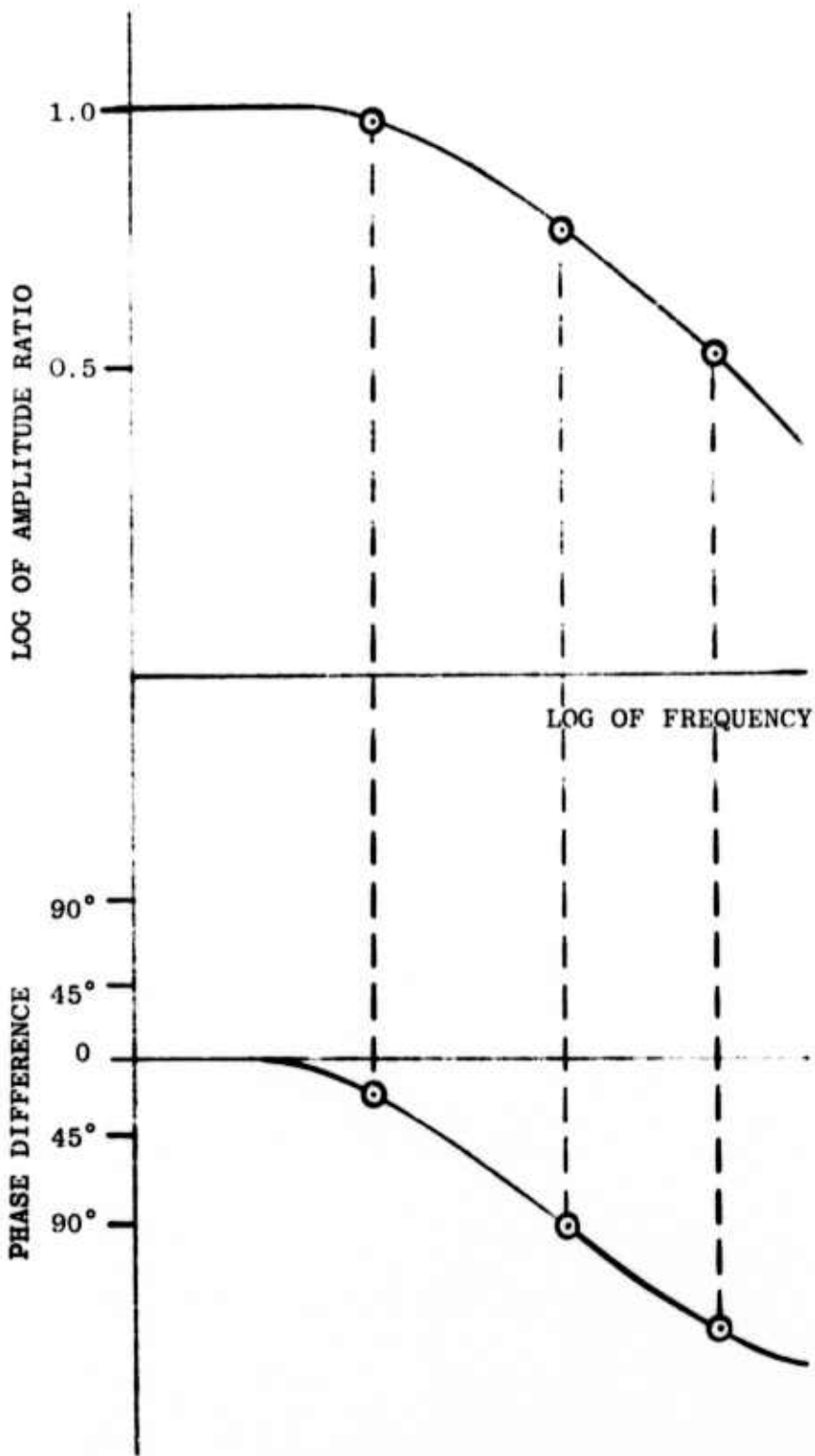
Figure 2. Typical bode plot of human tracking performance, showing amplitude ratio and phase difference at three frequencies.
