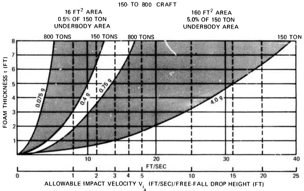
Figure 19b - 0.5- and 5-Percent Underbody Involvement
