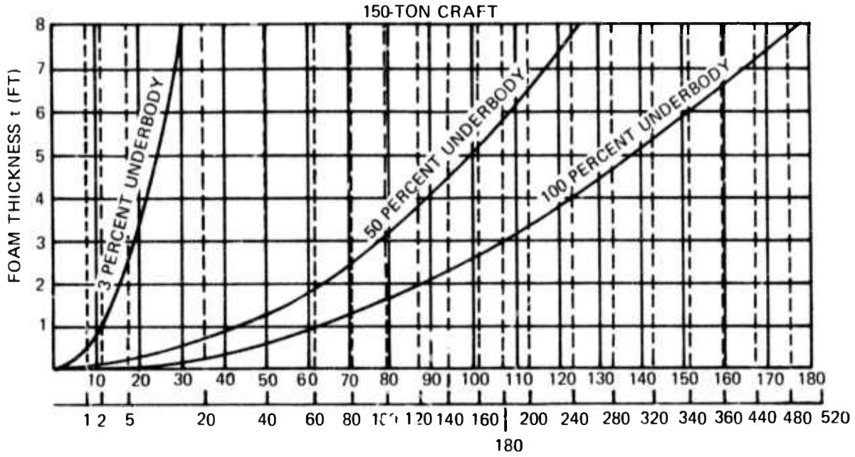
Figure 19 - Foam Thickness Necessary to Sustain Various Vertical Impact Velocities without Bottoming as a Function of Underbody Area Contact
