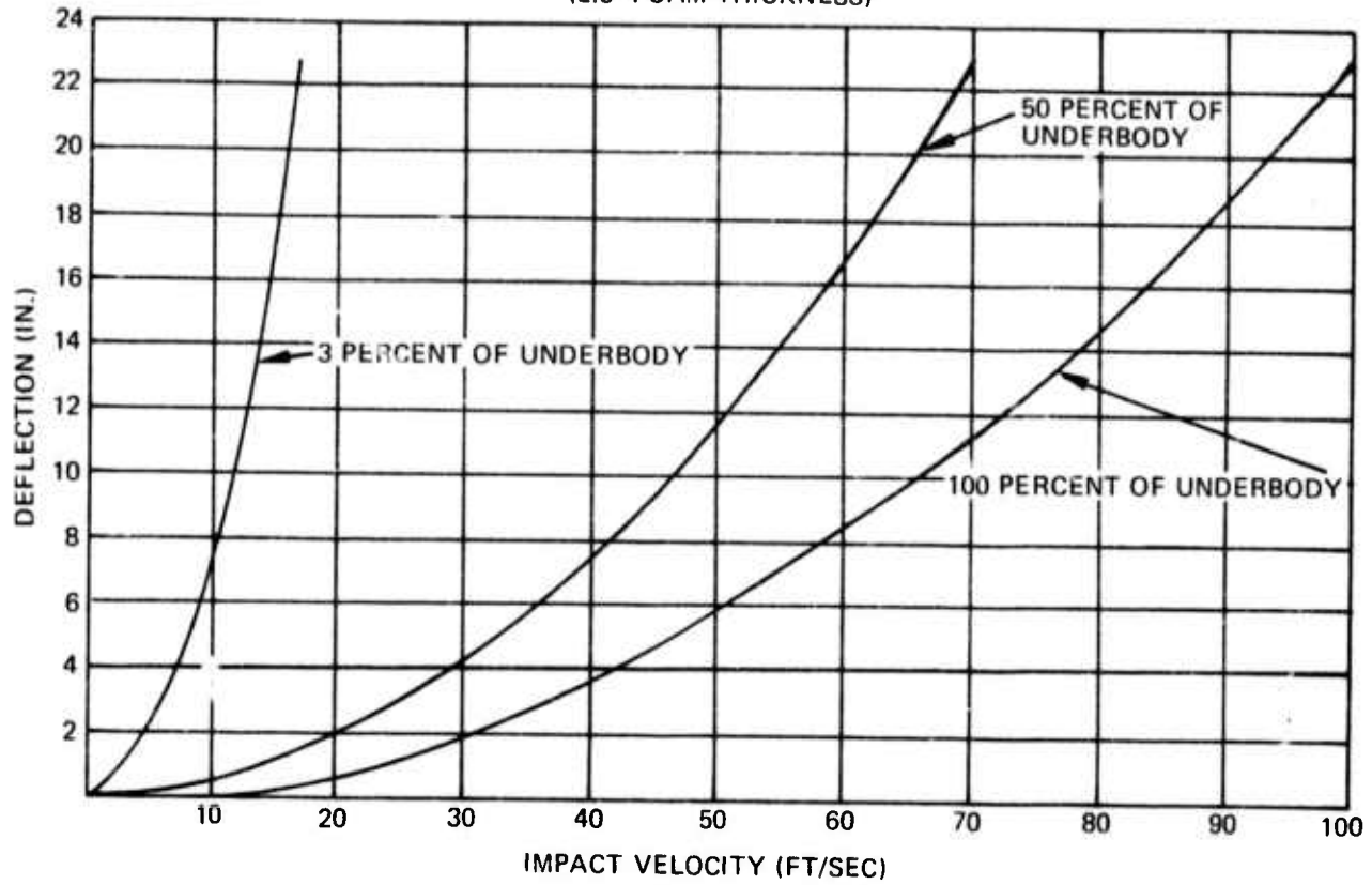
Figure 21 - Deflection versus Impact Velocity as a Function of Underbody Area Involvement
