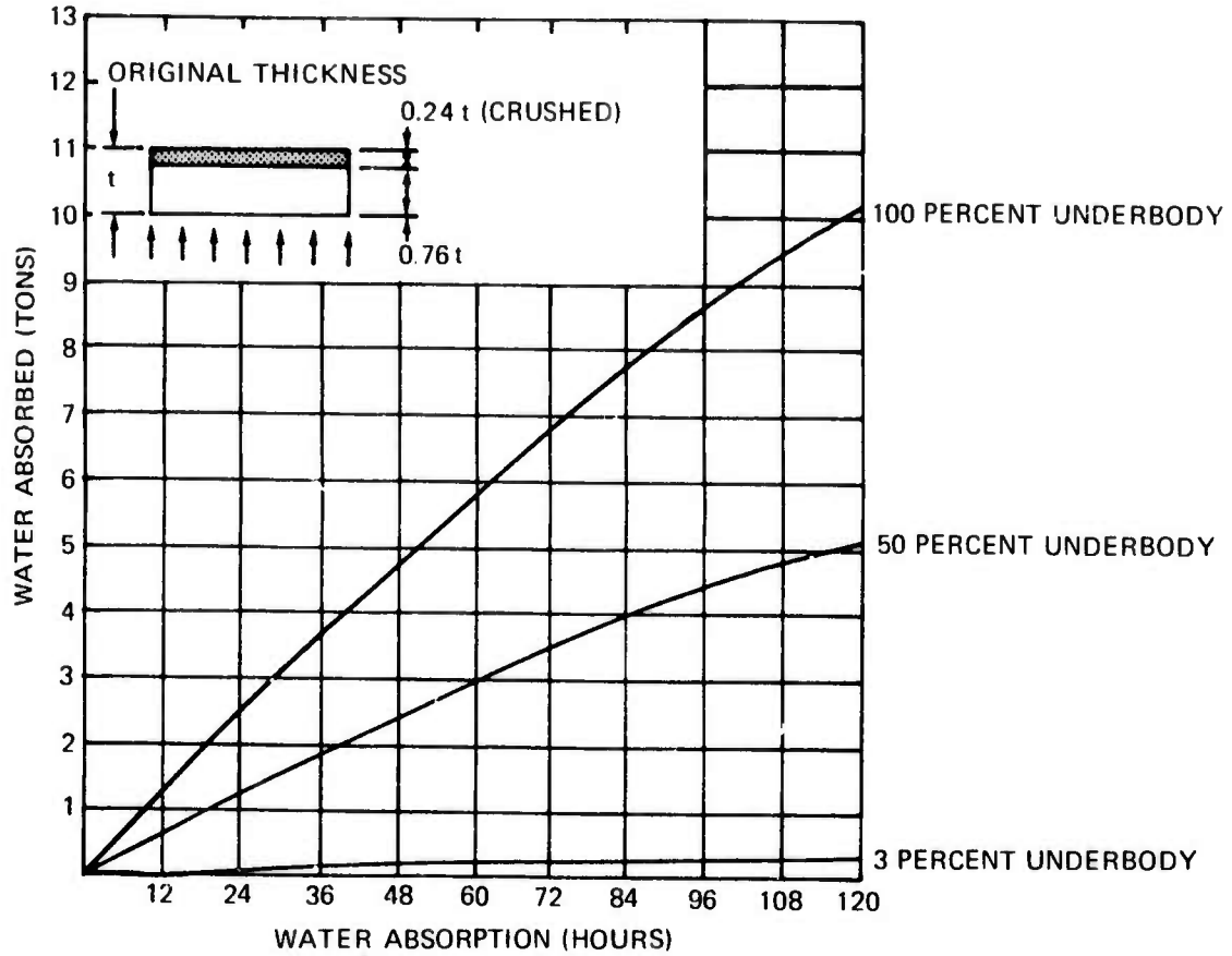
Figure 20 - Water Absorbed by Crushed Foam as a Function of Underbody Area Involvement
