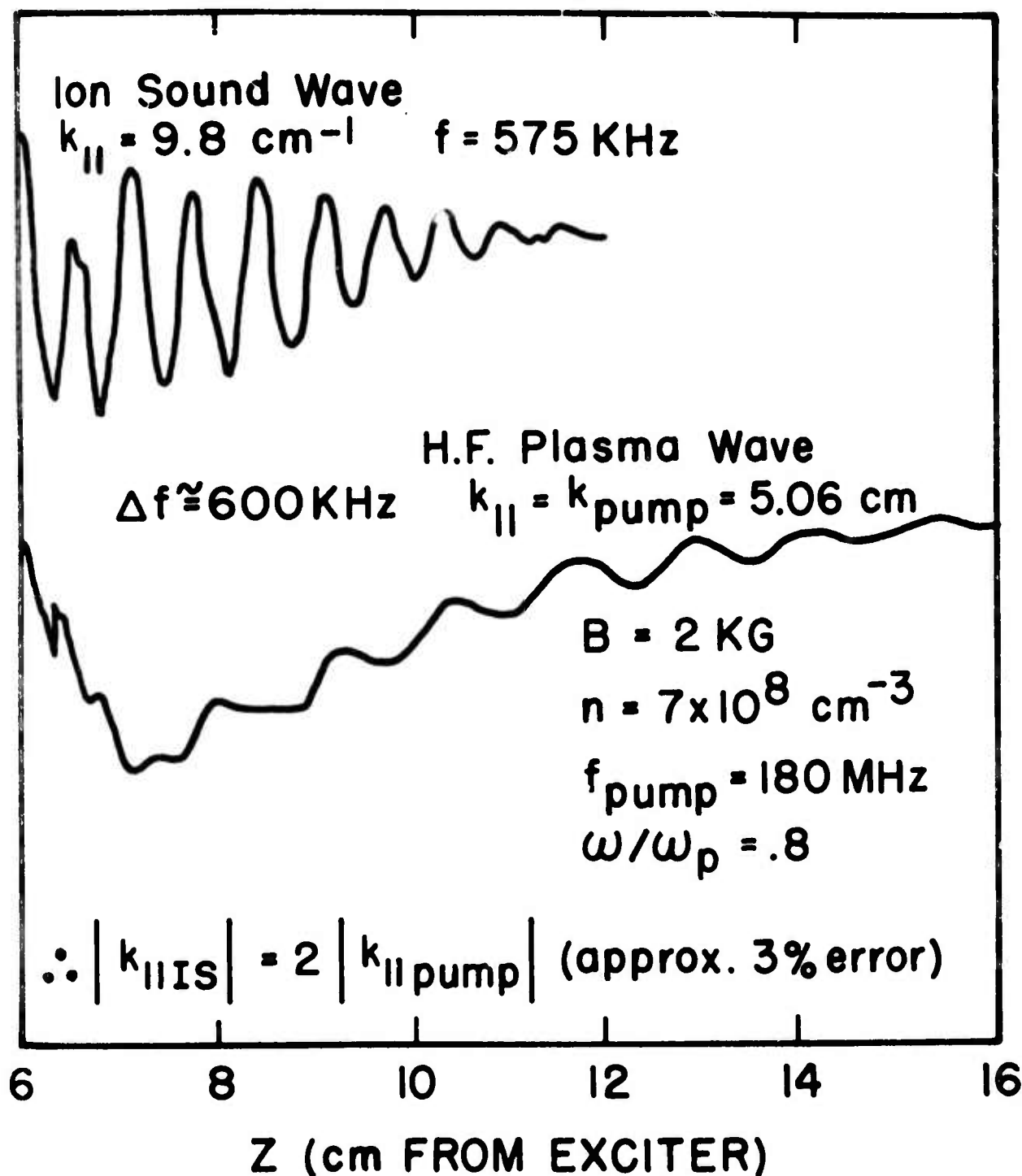
Fig. 3. Typical wavelength measurements, showing momentum conservation.
