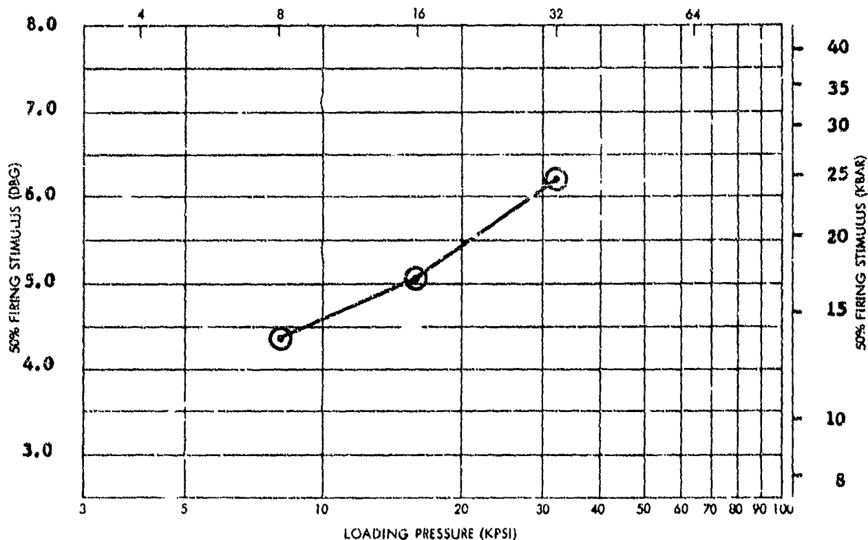
SMALL SCALE GAP TEST (SSGT) DATA BDX/ST-AC (96.7/3.3)
