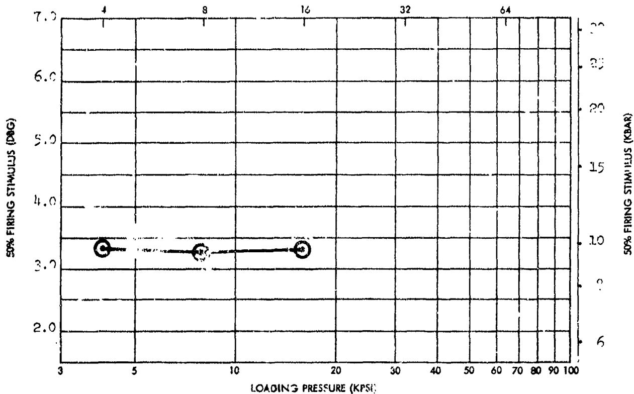
SMALL SCALE GAP TEST (SSGT) DATA PETT/DATE (50/50)
