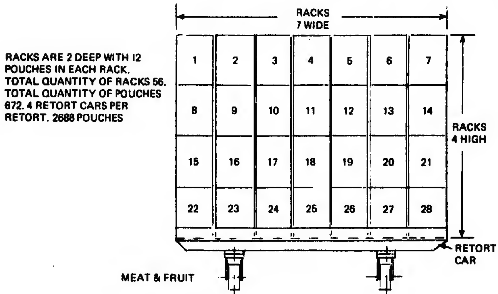
FIGURE 5 Retort Car Patterns
