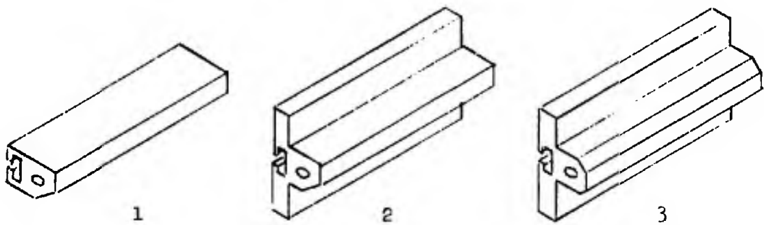
FIGURE 2 Bottom Heat Sealing Bar Configurations
