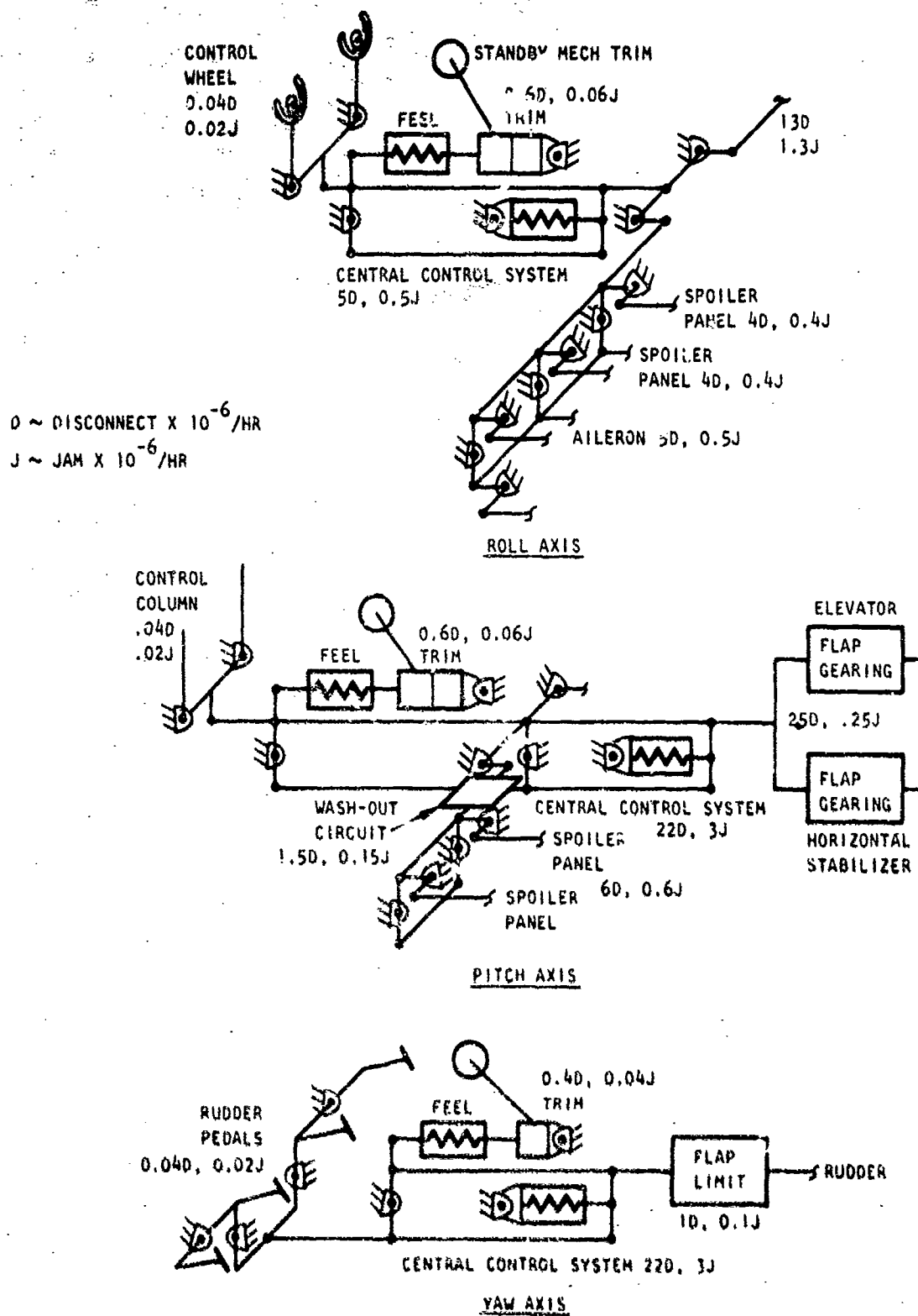
Figure 5. Single Mechanical Control System
