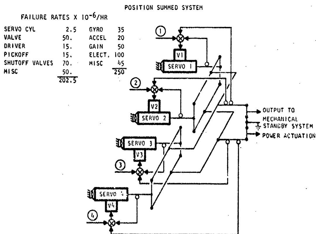
Figure 12. Fly-by-Wire Servo Systems
