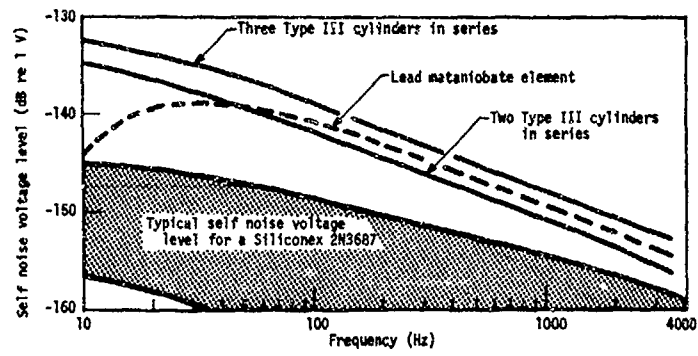
Fig. F-2. Maximum acceptable FET self noise for various acoustic elements.
