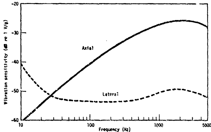
Fig. 9. Vibration sensitivity of a lead metaniobate disk.
