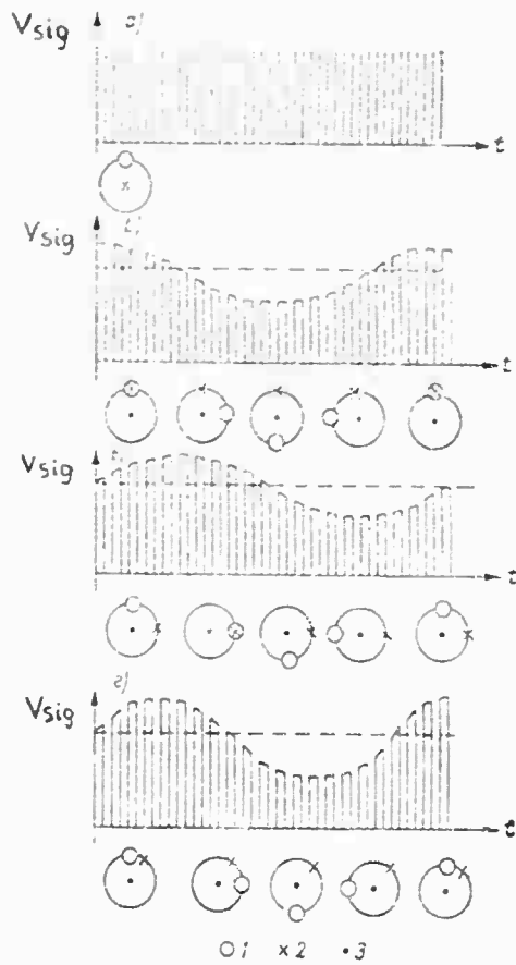
Fig. 9.36. Change in the phase of the envelope of the received signals a) object on axis of antenna; b) object shifted up along elevation angle; c) object shifted right along azimuth; d) object shifted along azimuth and elevation angle; 1) beam axis; 2) object; 3) antenna axis
