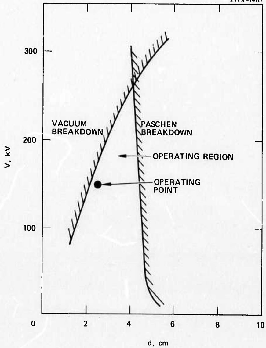
Fig. 4. Low pressure breakdown voltage in the plasma cathode accelerating region as a function of the gap width, d .
