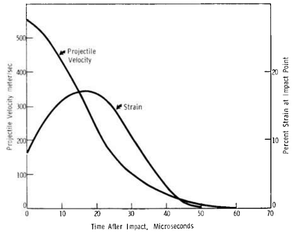
FIG. 8. Strain at impact point and projectile velocity vs time after impact.
