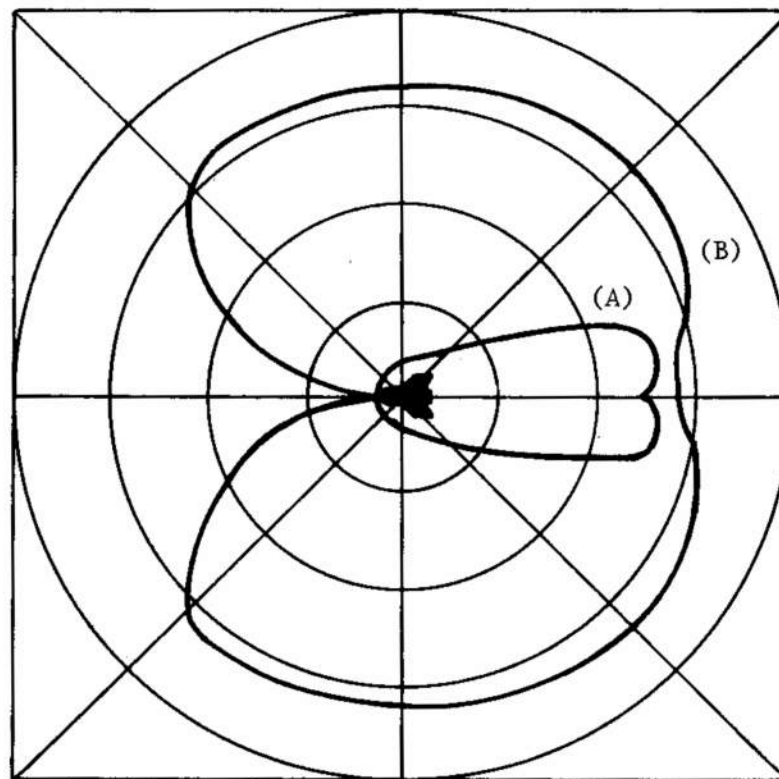
(A) UNDER MILITARY POWER, (B) WITH AFTERBURNER
