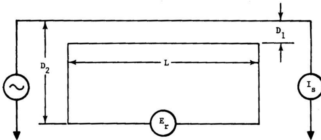
FIGURE 3-179. Schematic Illustrating Electromagnetic Coupling Parameters
