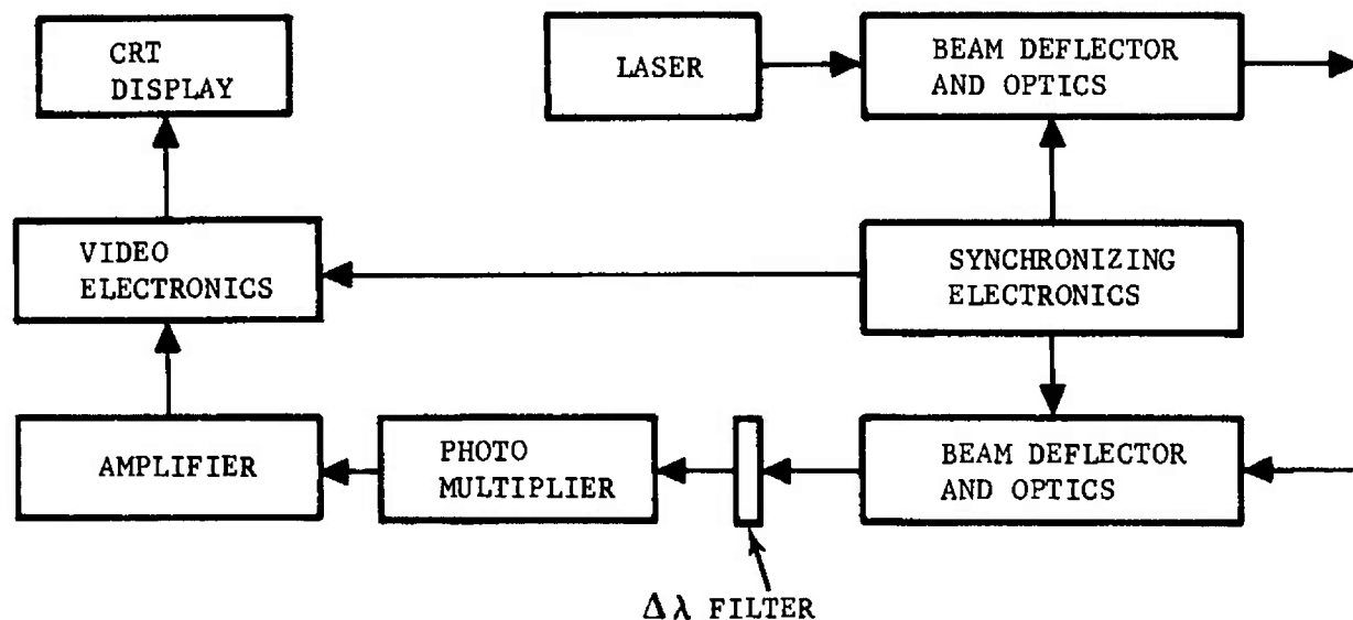
FIGURE 5-25. System Block Diagram
