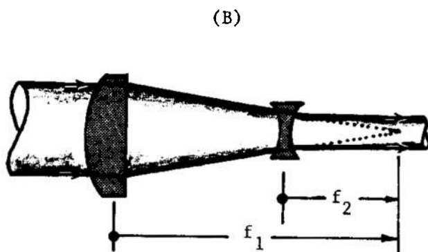
GALLILEAN TELESCOPE
