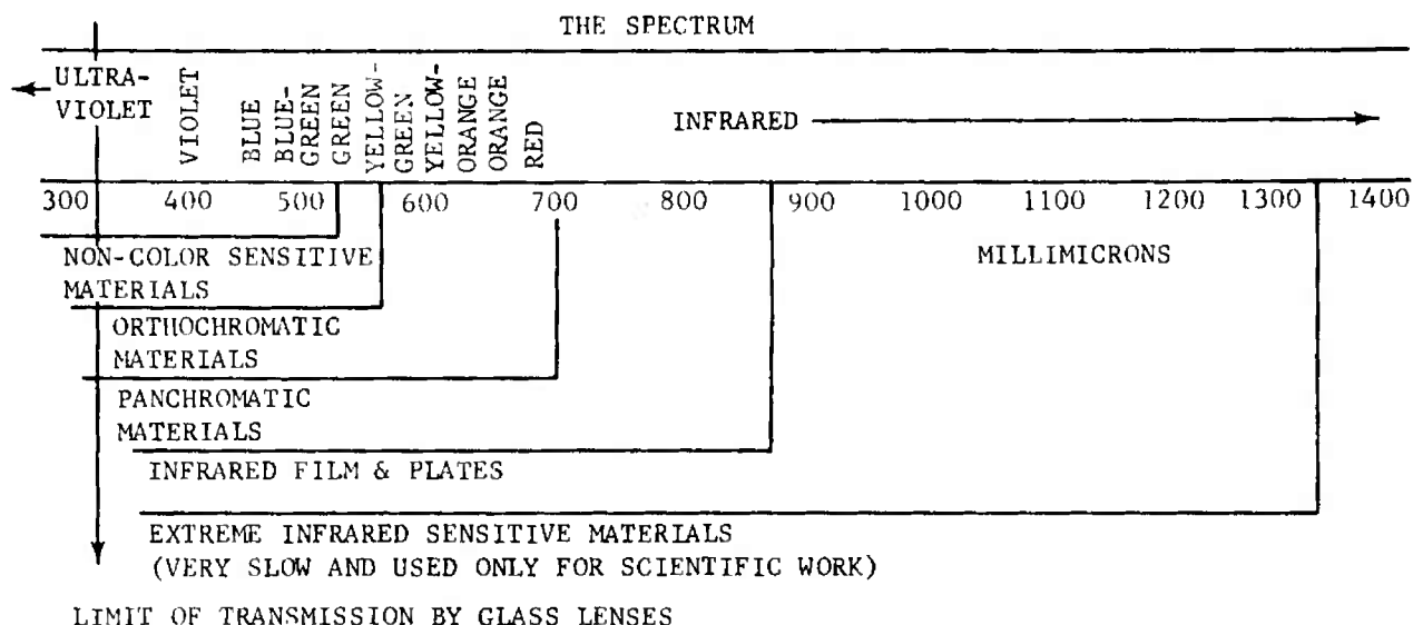
(A) THE SPECTRAL RANGE OF PHOTOGRAPHIC SENSITIVITY
