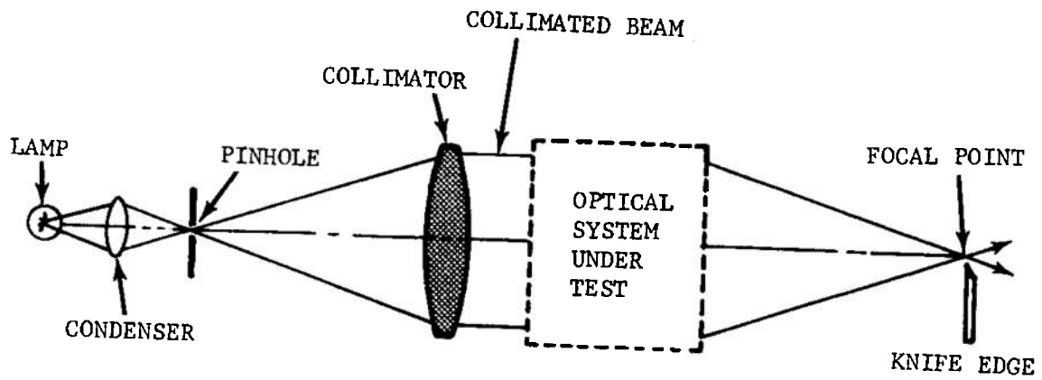
(A) KNIFE-EDGE TEST SETUP FOR COMPLEX OPTICAL SYSTEM
