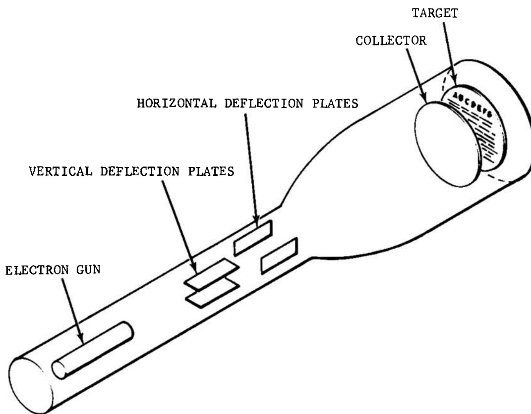
FIGURE 3-122. Monoscope Tube
