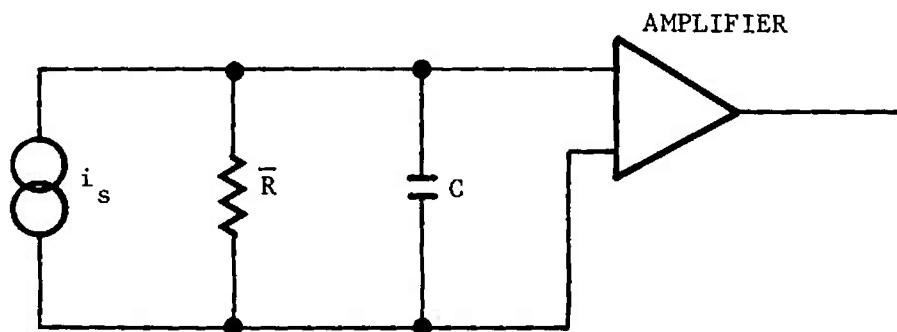
FIGURE 3-76. Equivalent Circuit Illustrating Detector-associated Capacitance
