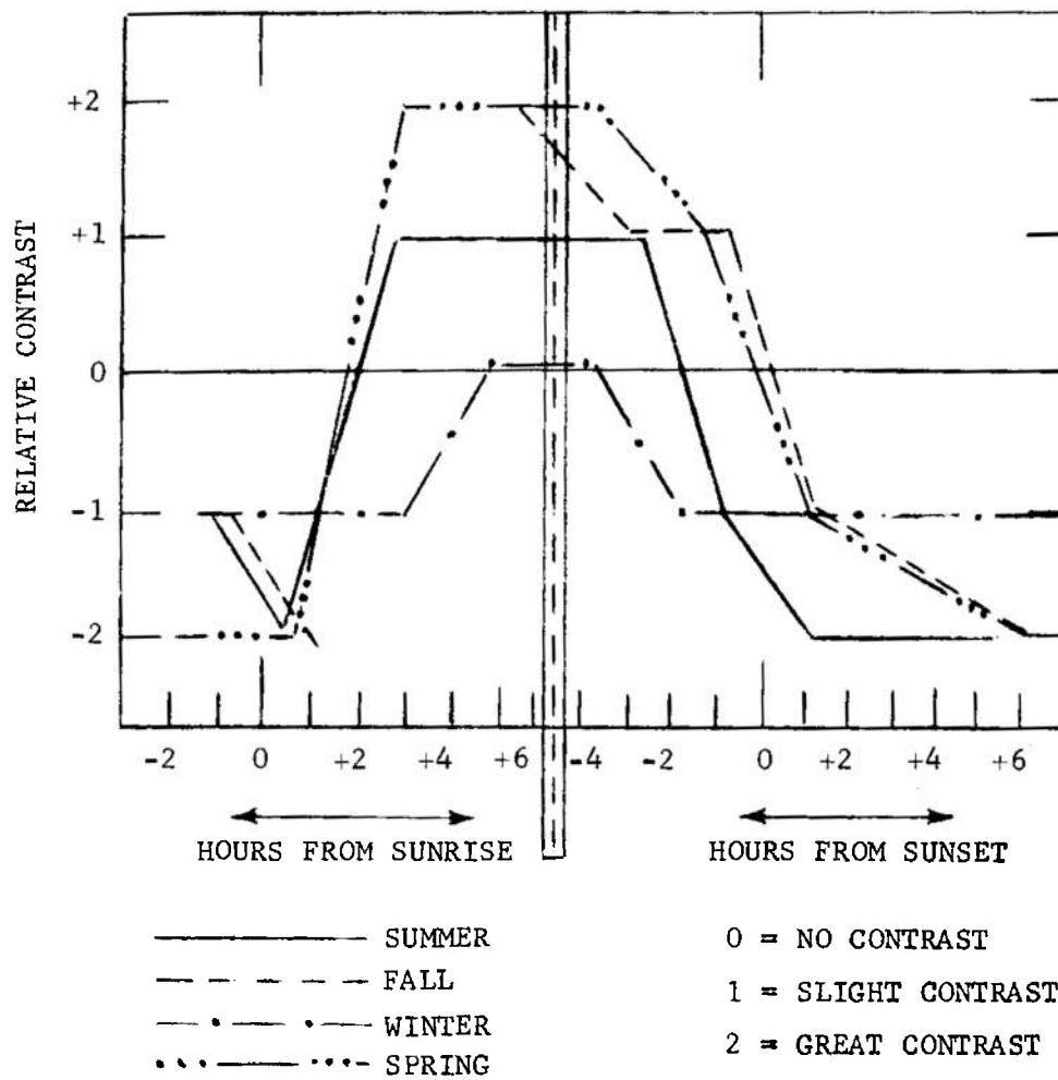
FIGURE 2-31. Relative Contrast of Wooden Catwalk Atop a Dam to the River Upstream from the Dam
