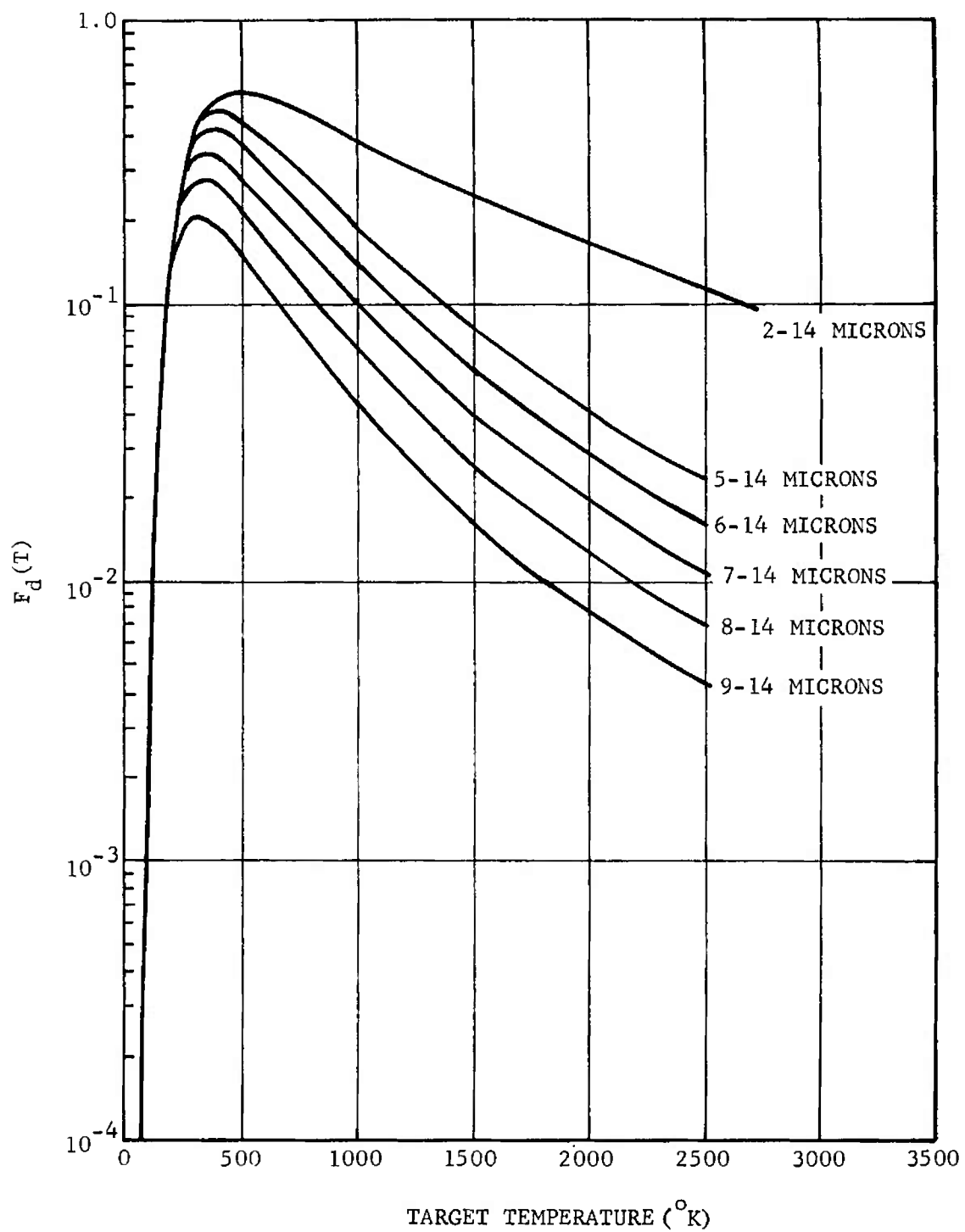
FIGURE 2-49. Detector Response Fraction F_d(T) for Ge:Hg Detectors As a Function of Spectral Band and Target Temperature
