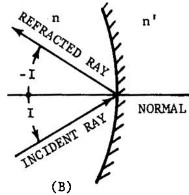
REFLECTION OF A RAY AT AN INTERFACE BETWEEN MEDIA OF DIFFERENT INDICES
