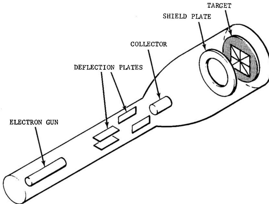
FIGURE 3-121. Matricon Tube
