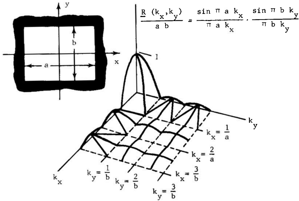
FIGURE 3-91. Spatial Filter Amplitude Response of Rectangular Detector
