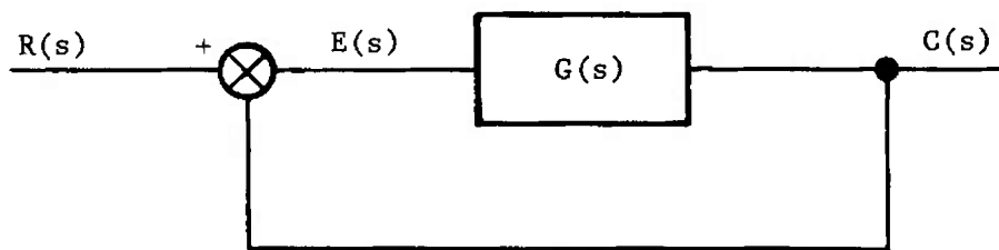
FIGURE 3-155. Servo Loop Diagram
