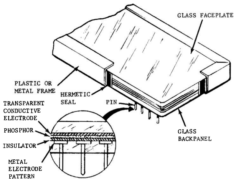
FIGURE 3-134. Exploded View of All-glass EL Readout Panel and Sectional View of Metal-glass Unit
