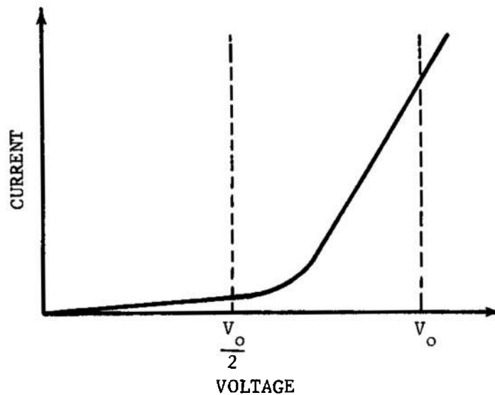
FIGURE 3-137. Voltage-current Curve for Nonlinear Resistor
