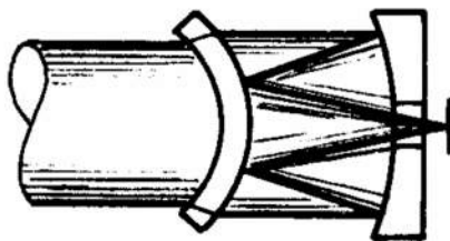
CASSEGRAINIAN SYSTEM COMBINED WITH MENISCUS CORRECTOR
