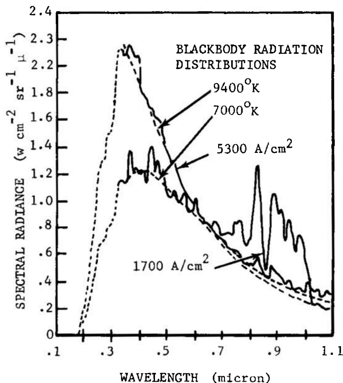
FIGURE 3-50. Spectral Radiant Energy of FZ-47A Flashtube Normalized to Input Power. Spectral Resolution Equal to 0.01 Micron
