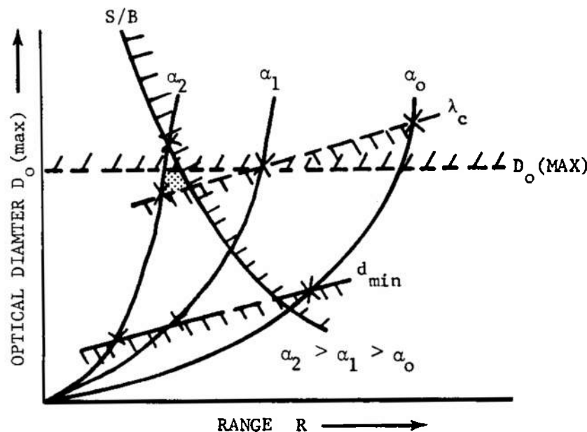
FIGURE 5-14. Constraints on System Aperture Selection
