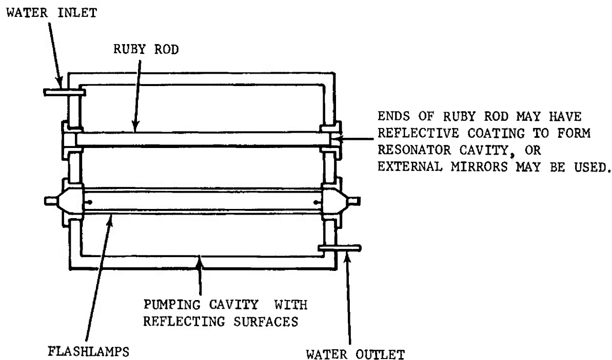
FIGURE 3-52. Outline of Solid-state Laser
