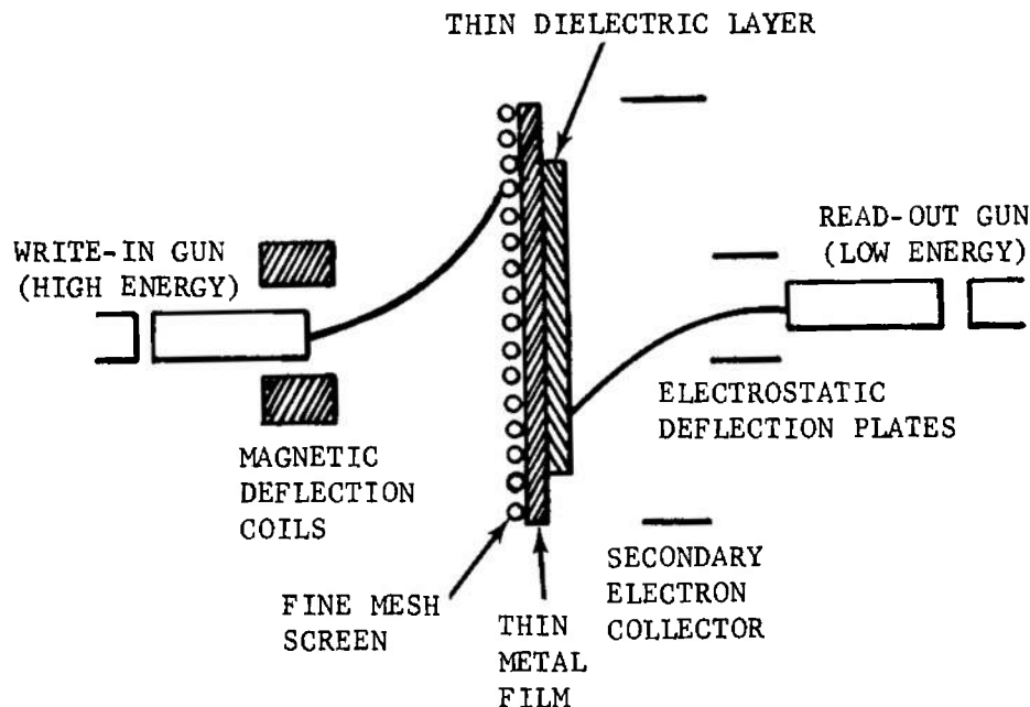
FIGURE 3-120. Typical Scan-conversion Tube
