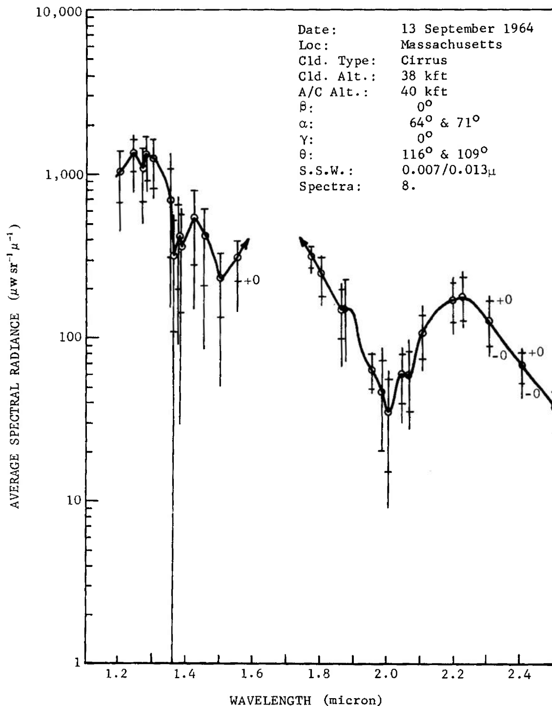
FIGURE 2-35. Typical 1.2- to 2.5-micron Cirrus Cloud Spectrum
