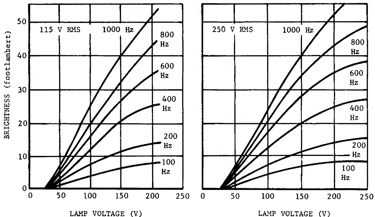
FIGURE 3-136. Brightness vs Voltage With 60% Transmission Glass for Both Metal-glass and All-glass EL Readout Panels at 115 and 250 V rms, Respectively
