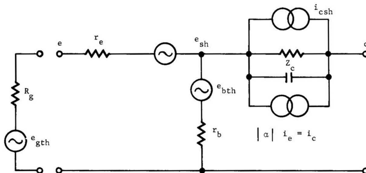
FIGURE 3-96. Classic Conventional Transistor Noise-equivalent Circuit
