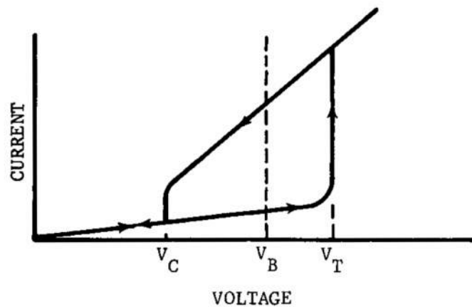
FIGURE 3-138. CdSe Hysteresis Curve
