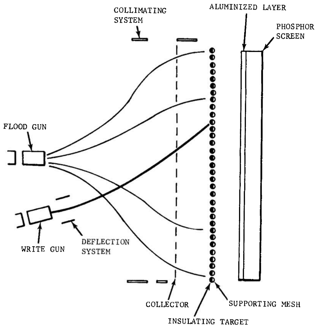
FIGURE 3-119. Display Storage Tube
