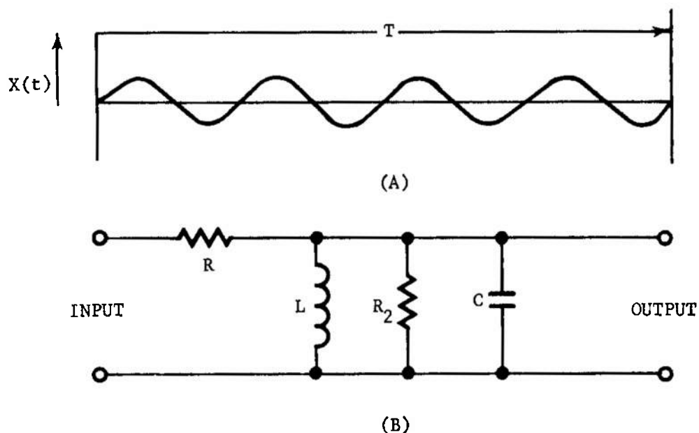
FIGURE 3-109. Input Sinusoidal Pulse Train and Second-order Filter
