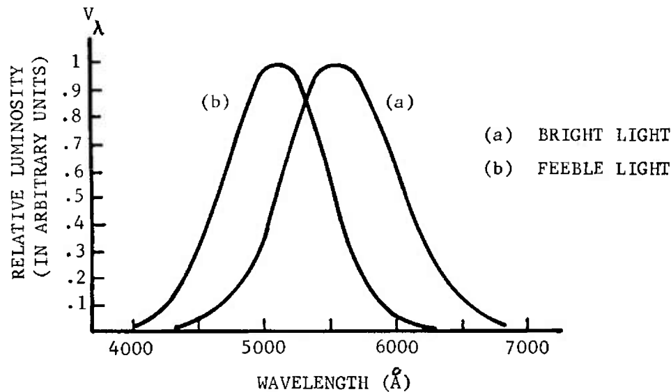
FIGURE 3-112. Standard Luminosity Curve for the Average Human Eye
