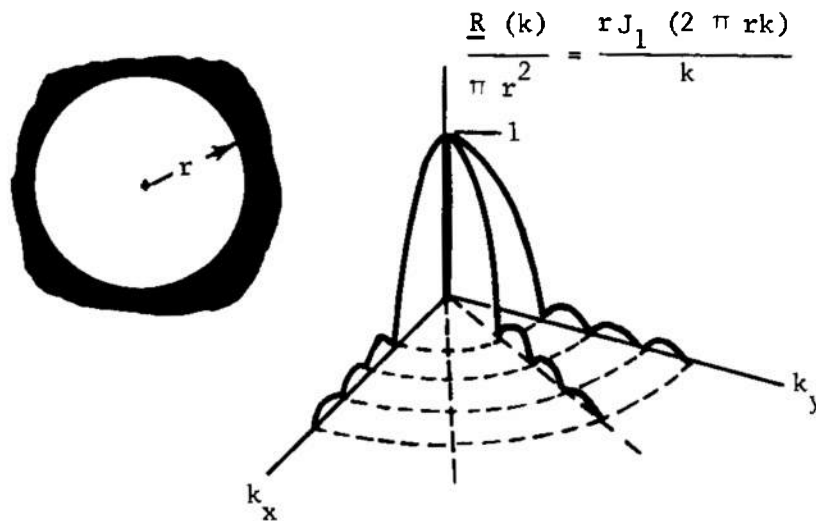
FIGURE 3-93. Spatial Amplitude Response of Circular Detector
