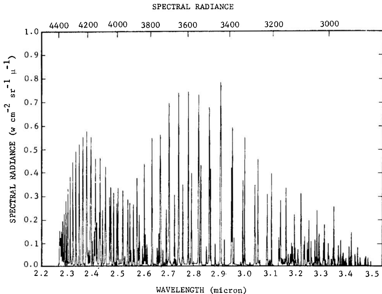
FIGURE 2-63. Emission Spectrum of HF for 0.5 cm-atm at 2640°K
