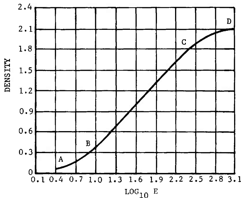
FIGURE 3-129. Typical Characteristic Curve of a Photographic Emulsion
