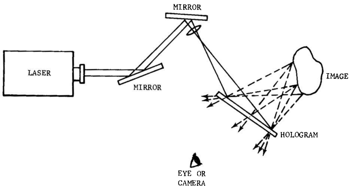
FIGURE 3-132. Reconstruction of a Hologram
