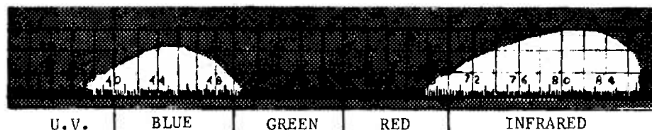
(B) SPECTRAL SENSITIVITY OF KODAK INFRARED MATERIALS, NAMELY, KODAK INFRARED FILM (IN SHEETS) AND KODAK INFRARED FILM (IN MAGAZINES)
