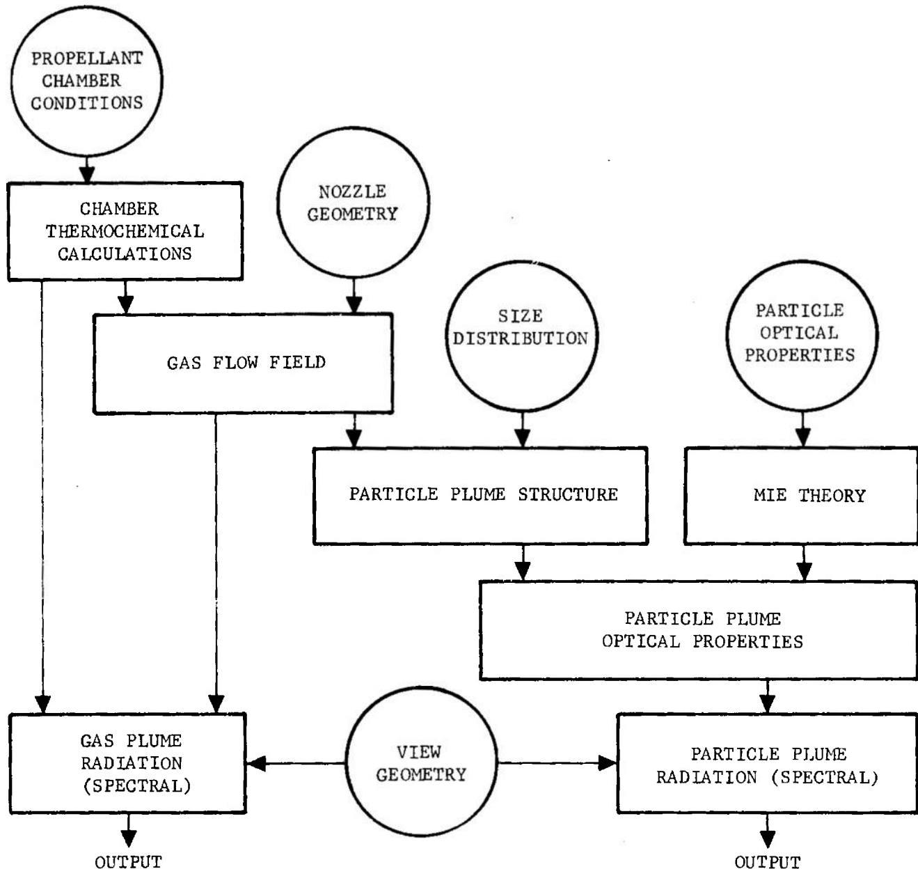
FIGURE 2-54. Flow Chart for Plume Radiation Calculations
