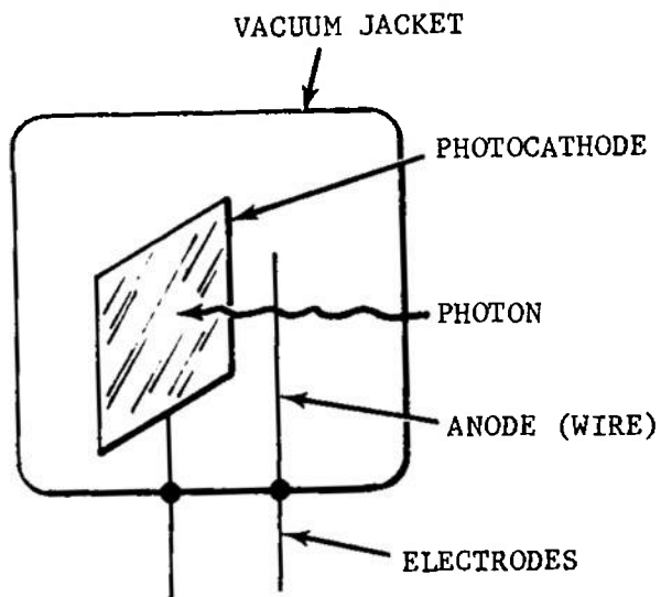
(A) VACUUM PHOTODIODE
