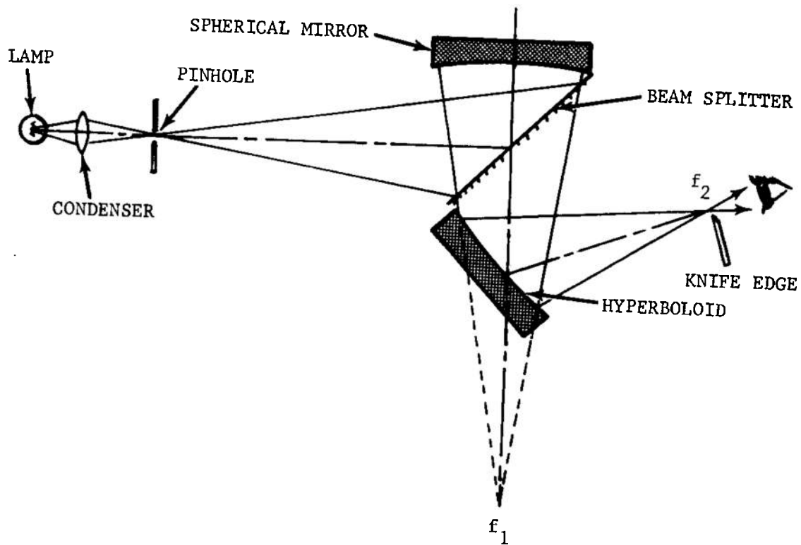
(B) KNIFE-EDGE TEST SETUP FOR HYPERBOLOIDAL MIRROR
