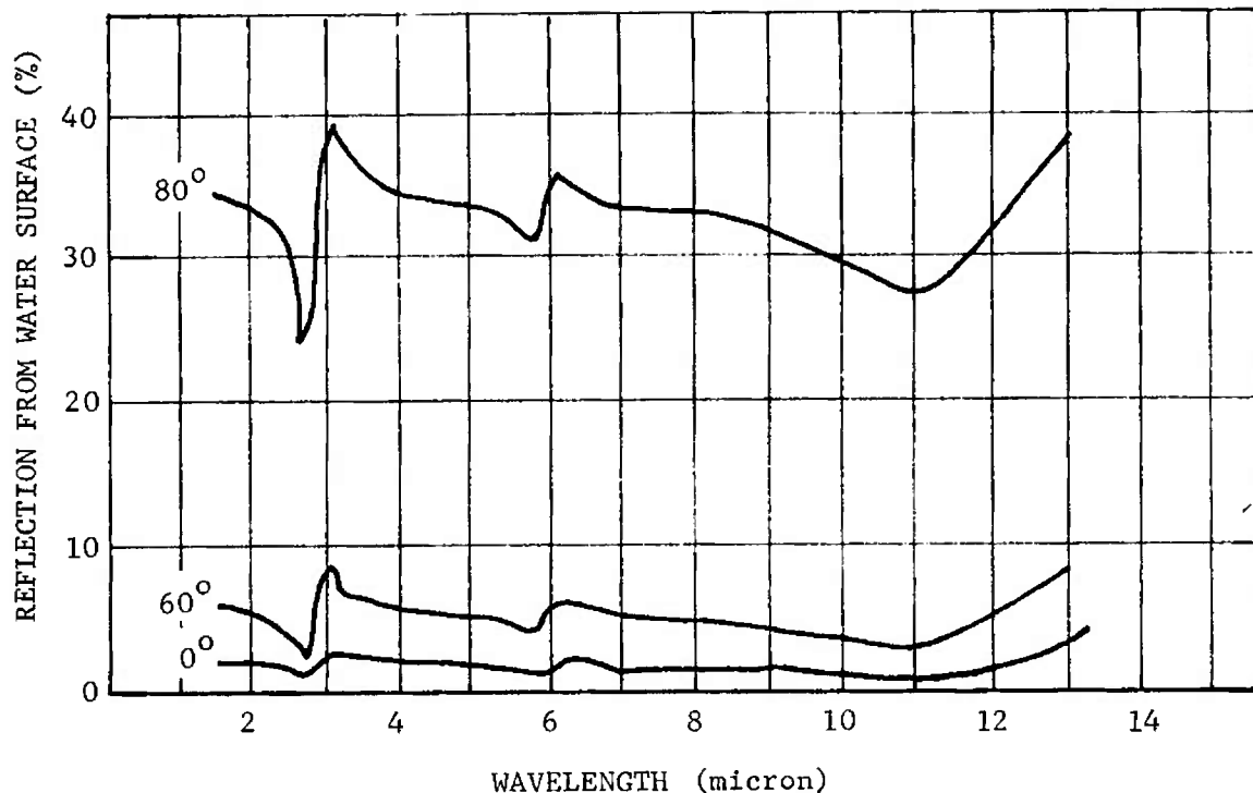
FIGURE 2-34. Reflectance of a Water Surface at 0^\circ , 60^\circ , and 80^\circ Angle of Incidence
