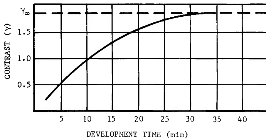
FIGURE 3-130. Typical Variation of Gamma With Development Time
