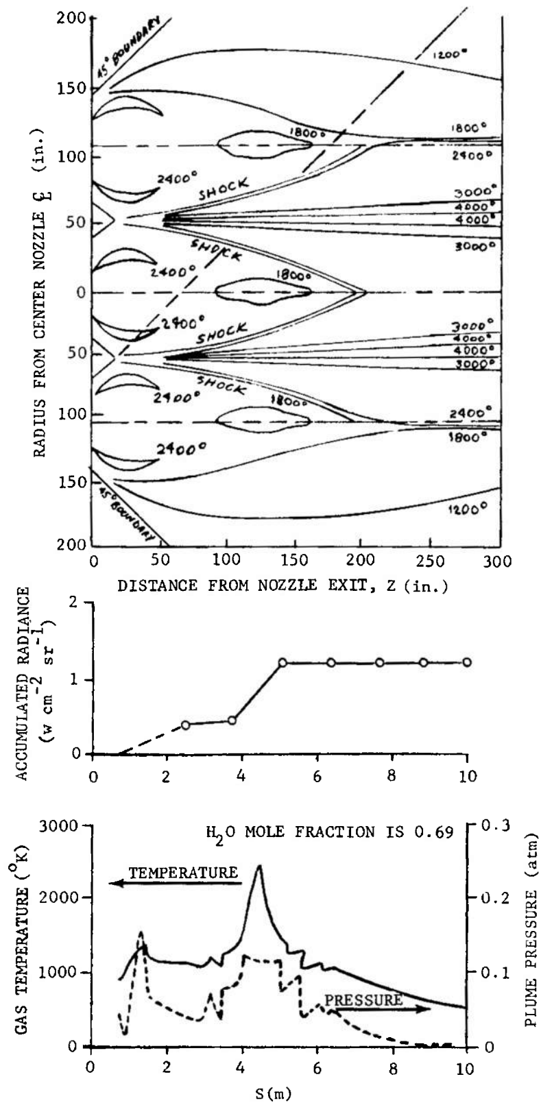
FIGURE 2-57. Typical Line-of-sight Variations on the Saturn S-II Stage
