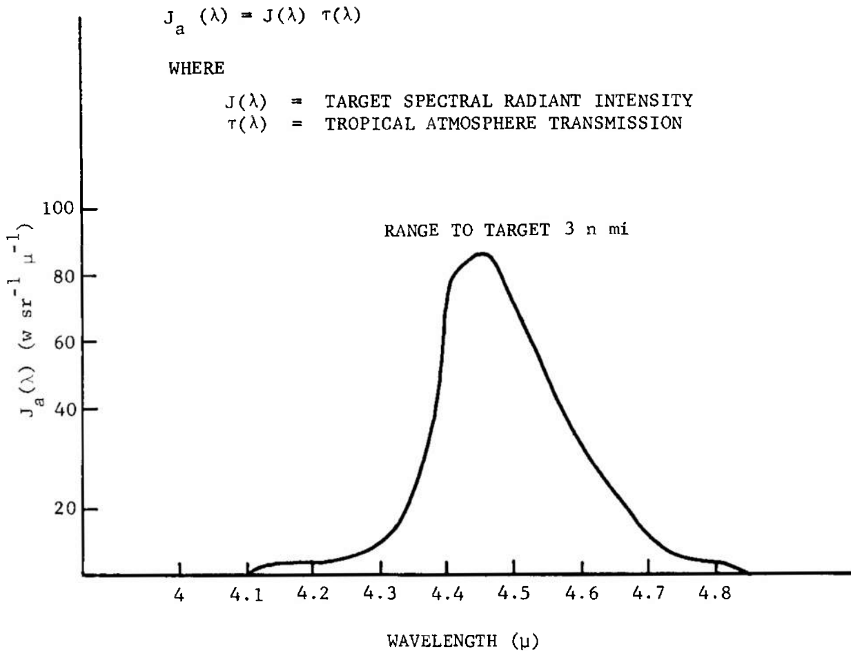
FIGURE 5-22. Apparent Target Intensity
