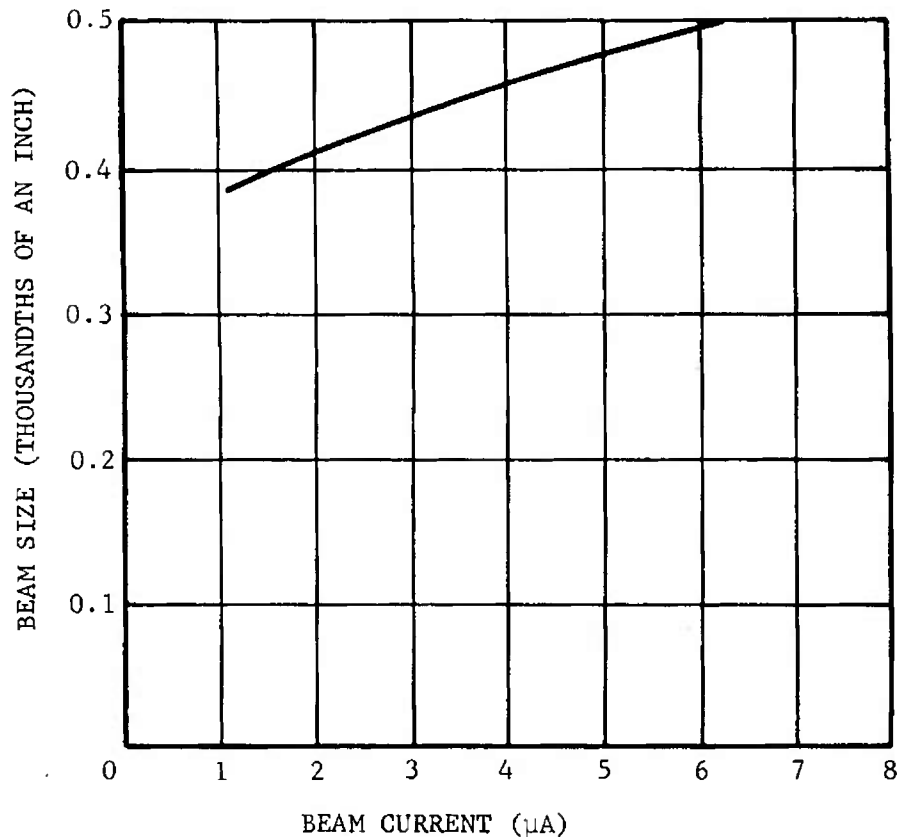
FIGURE 3-115. Spot Size for Several Beam Currents
