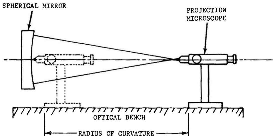
FIGURE 3-39. Setup for Determining the Curvature of Concave Spherical Mirrors
