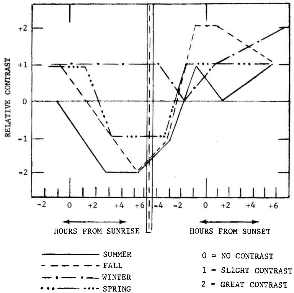
FIGURE 2-30. Relative Contrast of Deciduous Trees to Short Grass
