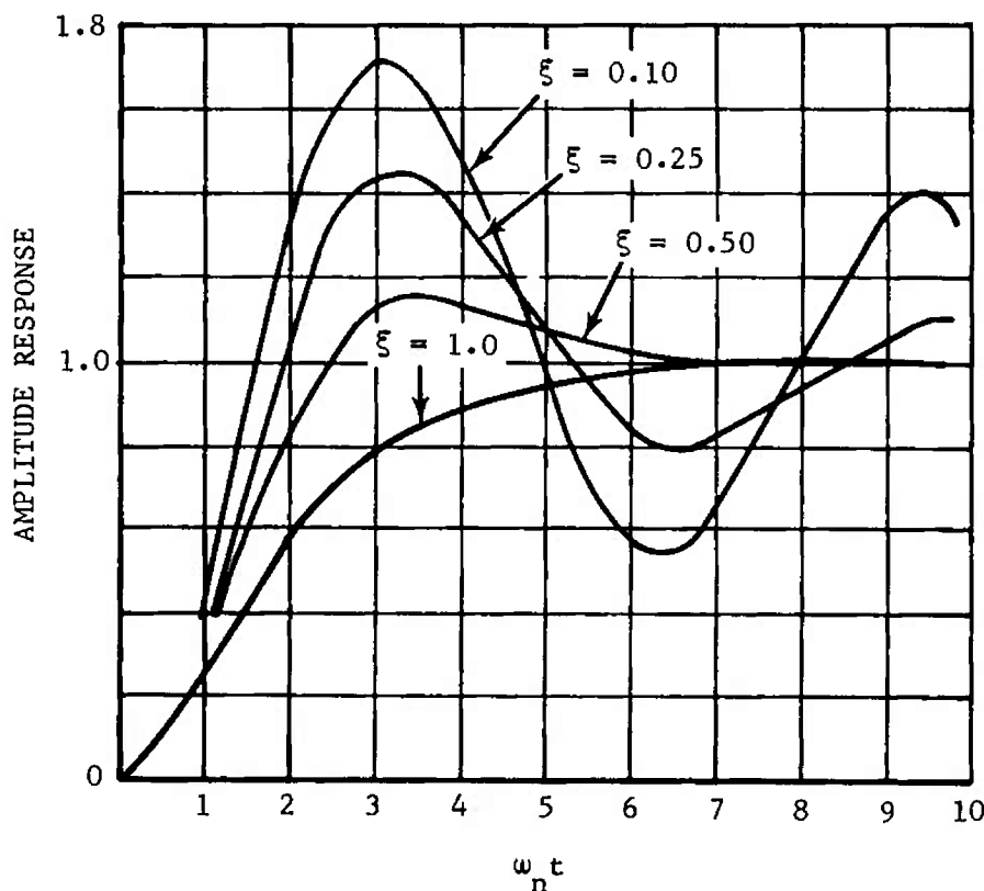
FIGURE 3-157. Servo Response of \frac{\omega_n^2}{s^2 + 2\xi\omega_n s + \omega_n^2} to Unit Step Input for Various Damping Factors
