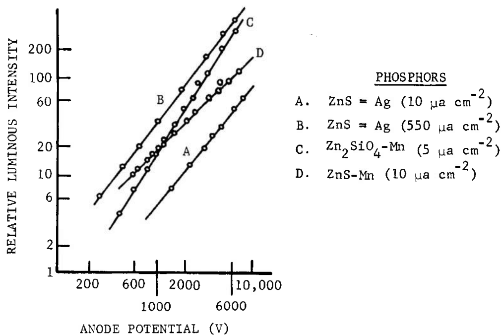
FIGURE 3-116. Variation of Luminous Intensity With Anode Potential
