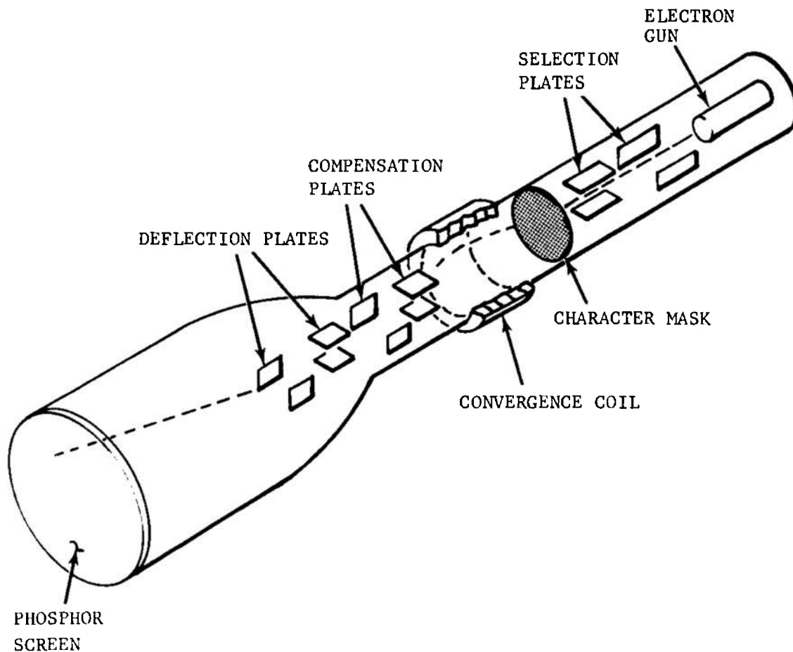
FIGURE 3-123. Shaped-beam Tube
