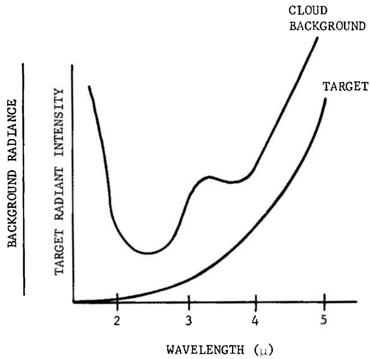
FIGURE 5-7. Sample Spectral Signature of Target and Background
