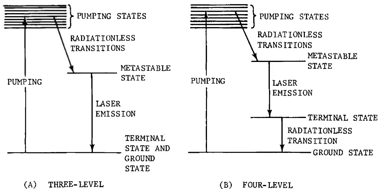
FIGURE 3-51. Simplified Laser Energy-level Diagram
