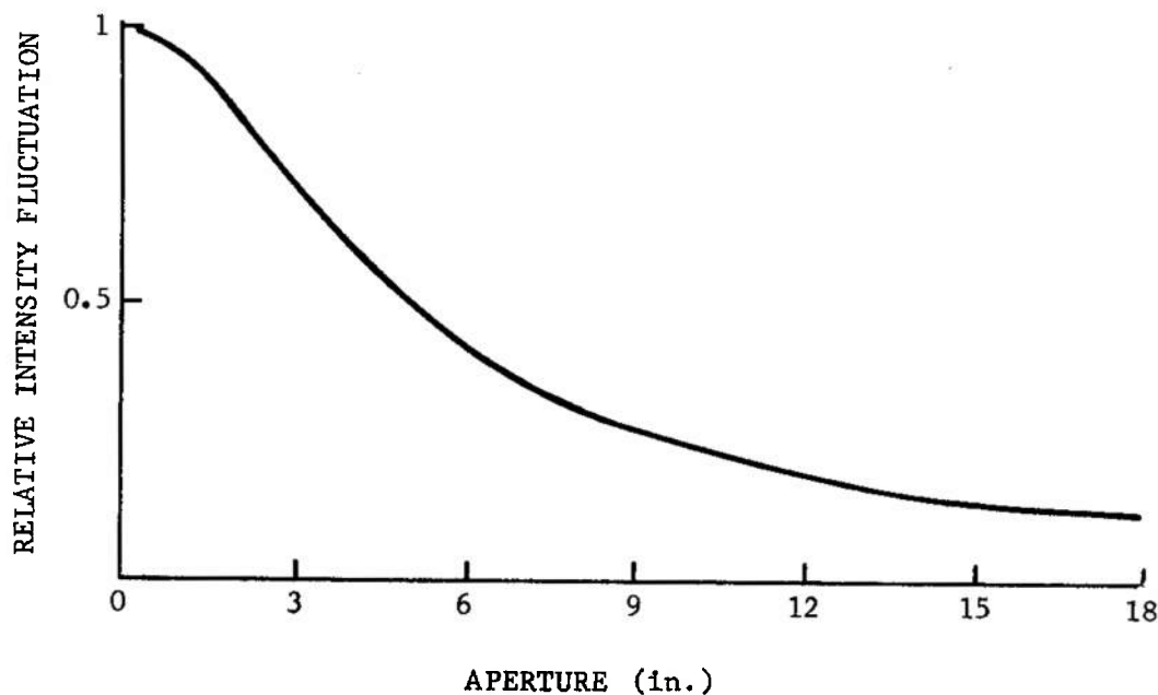
FIGURE 2-18. Scintillation vs Telescope Aperture
