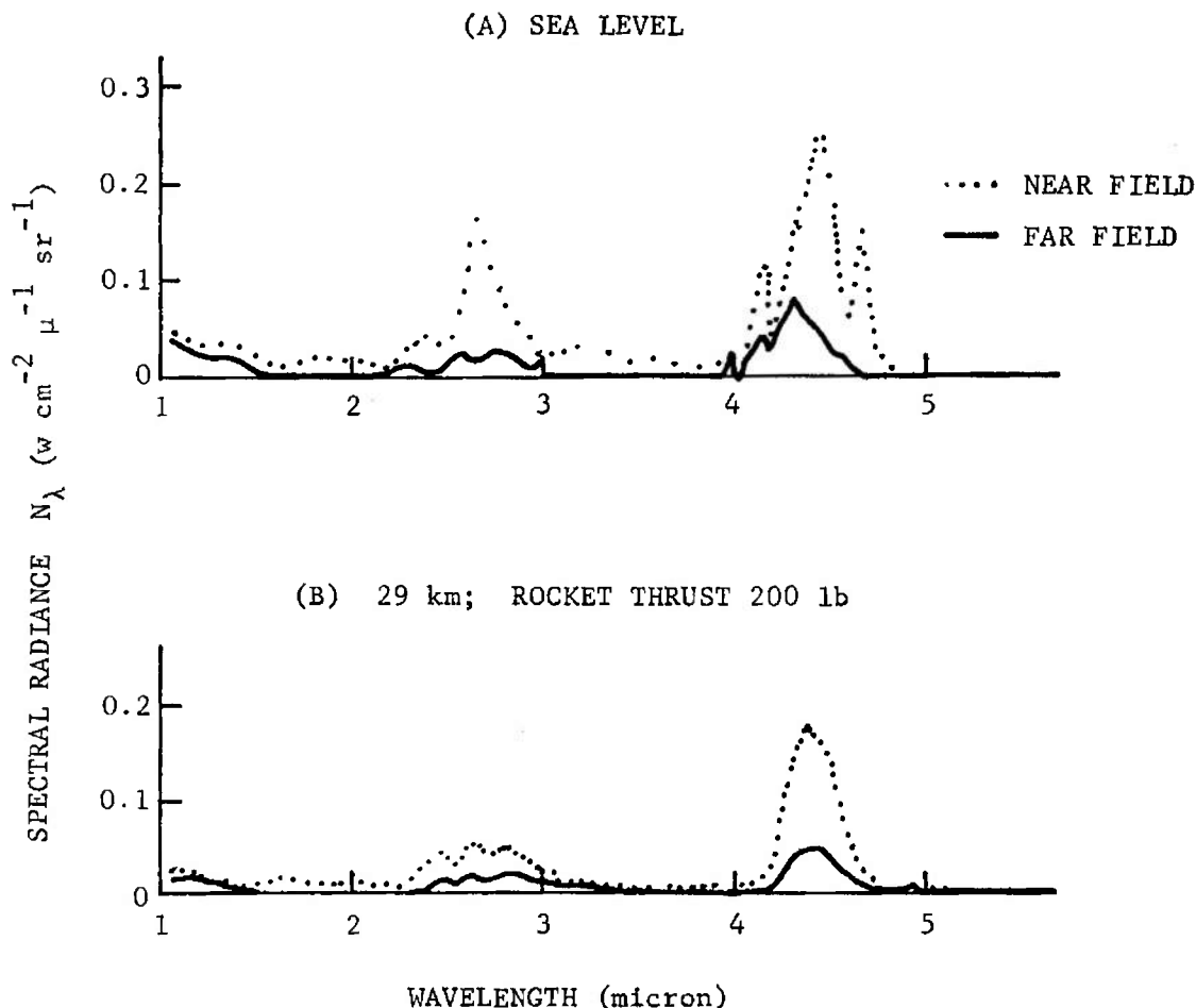
FIGURE 2-66. Spectral Radiance of Solid Propellant Rocket
