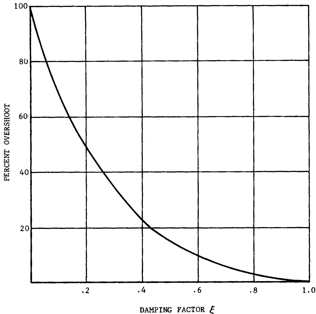
FIGURE 3-158. Overshoot vs Damping Factor for Second-order System
