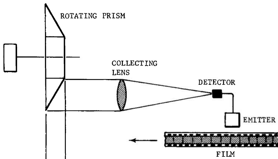
FIGURE 5-18. Line Scanning Technique
