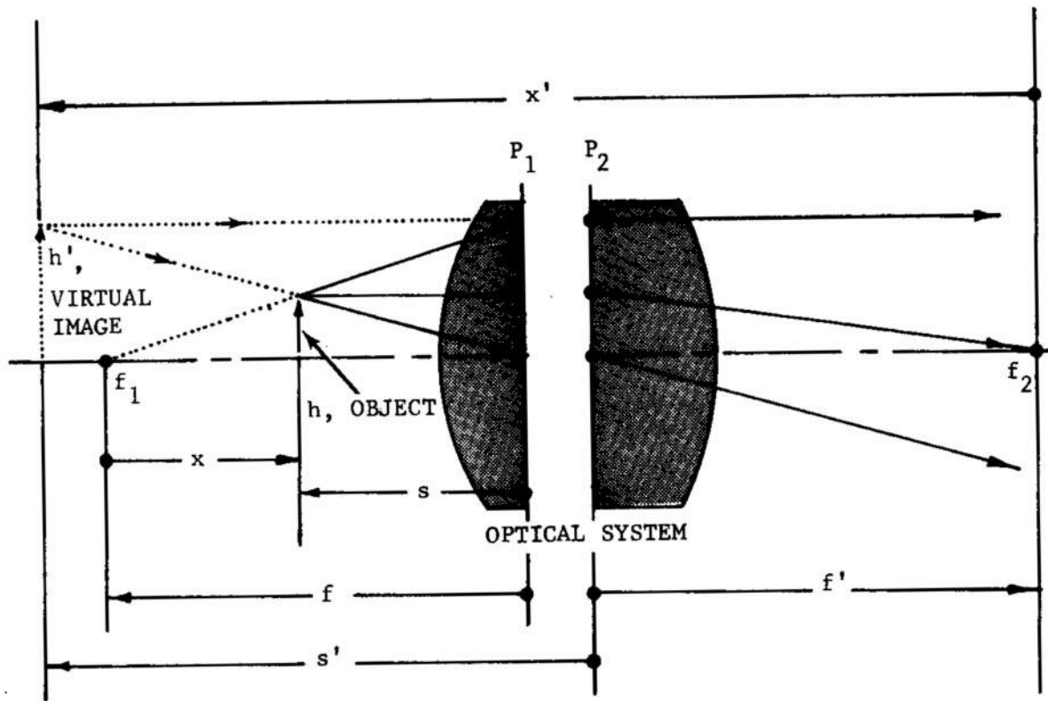
FIGURE 3-15. Virtual Image Formation by an Optical System
