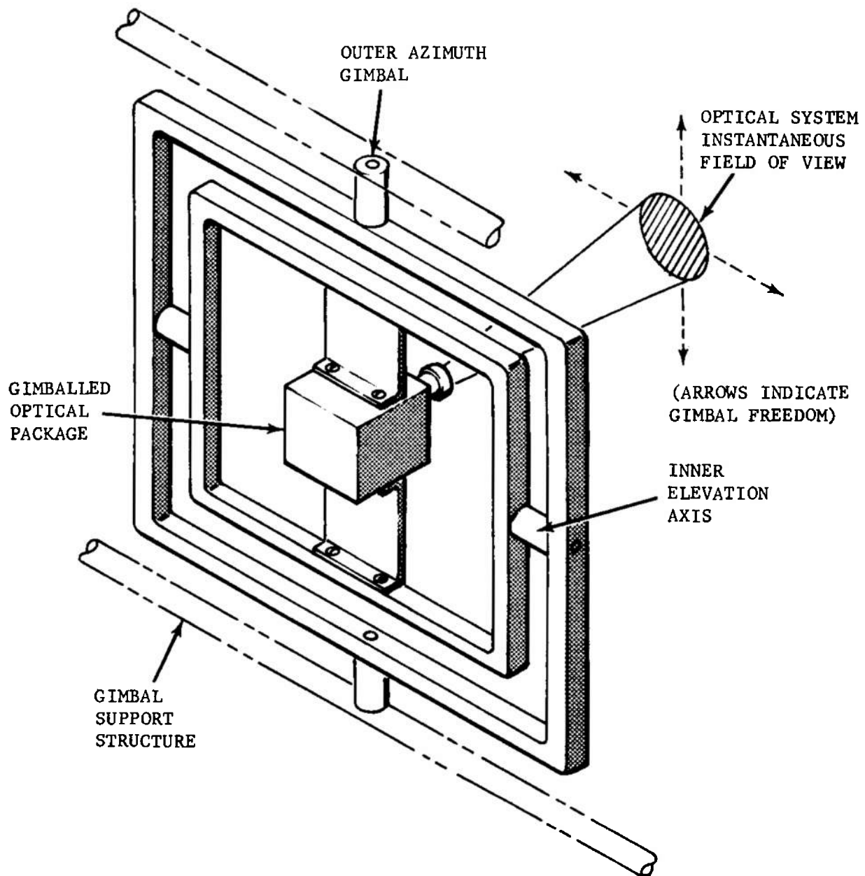
FIGURE 3-149. Conceptual Layout of Two-axis Gimbal Assembly
