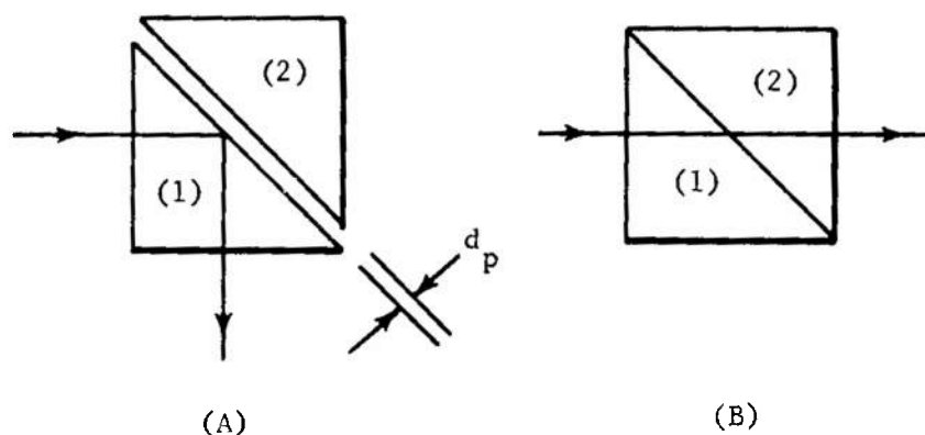
FIGURE 3-54. Frustrated-Internal-Reflection Modulator
