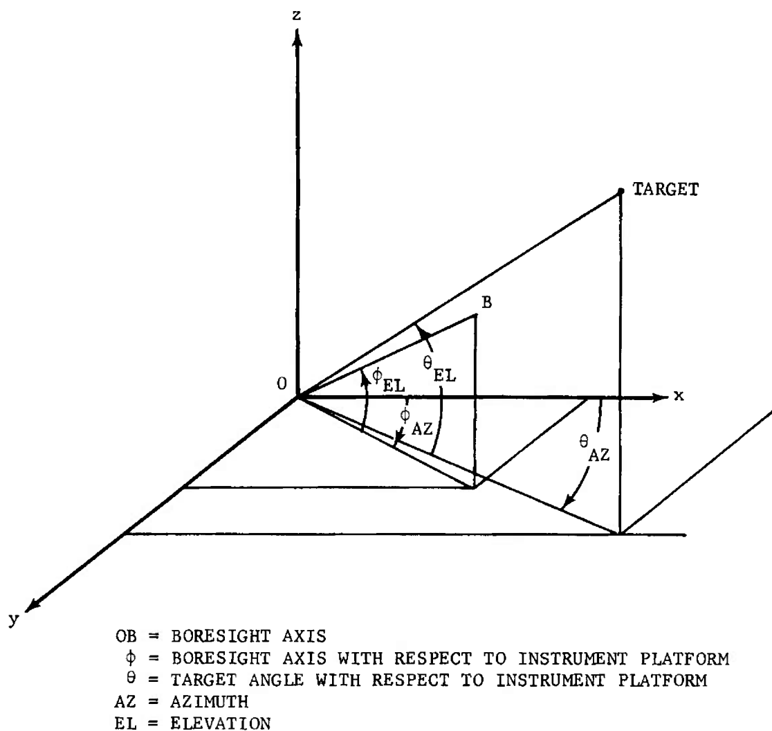
FIGURE 3-151. Relationship of Gimbal and Target Coordinates
