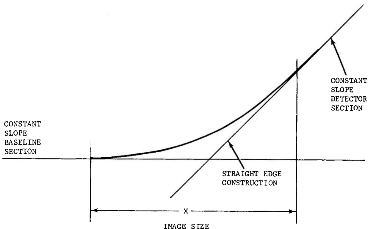
FIGURE 3-147. Section of Knife-edge Recording Characteristic Curve
