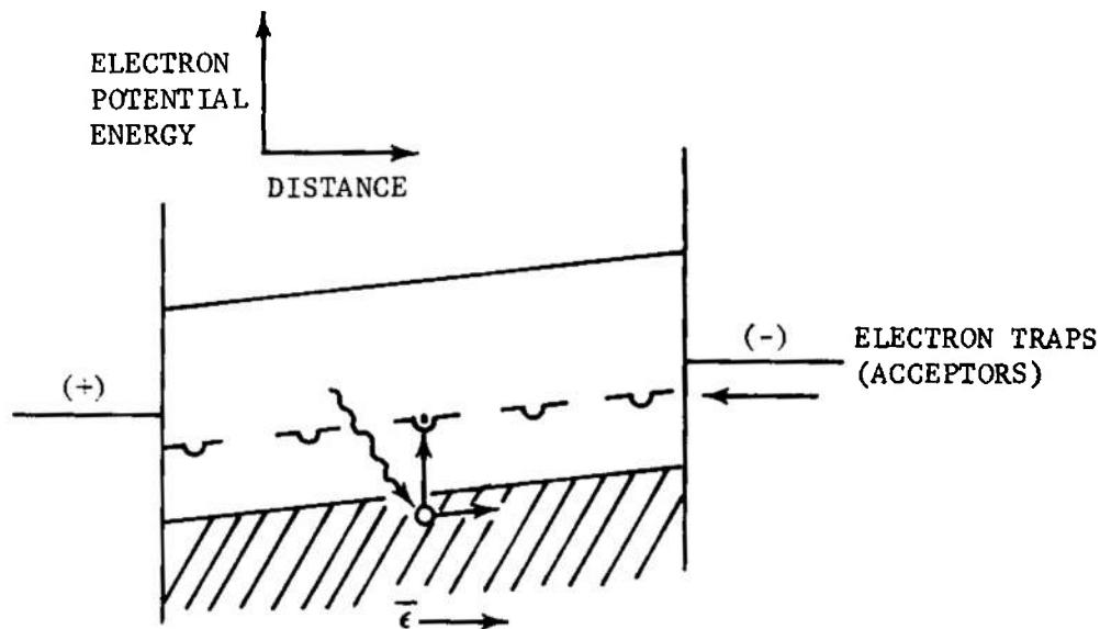
FIGURE 3-64. Semiconductor (P-type Extrinsic Detector) With Acceptors
