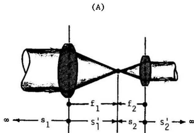
ASTRONOMICAL TELESCOPE
