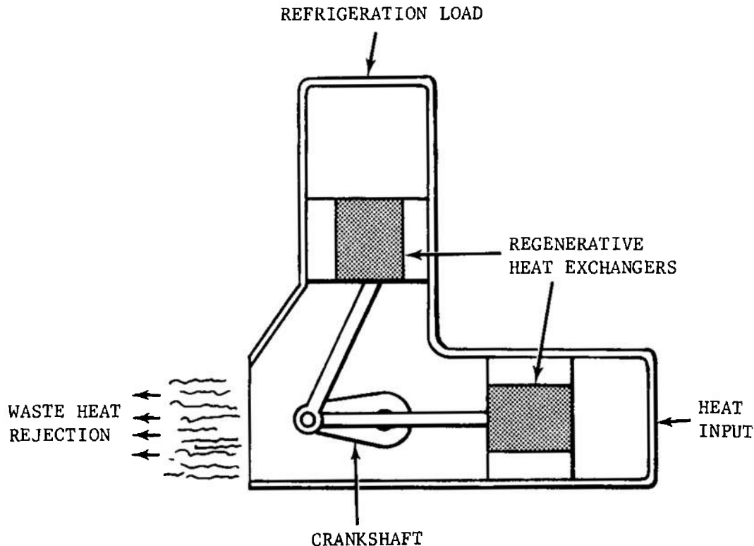
FIGURE 3-89. Vuilleumier Cycle Cooling System
