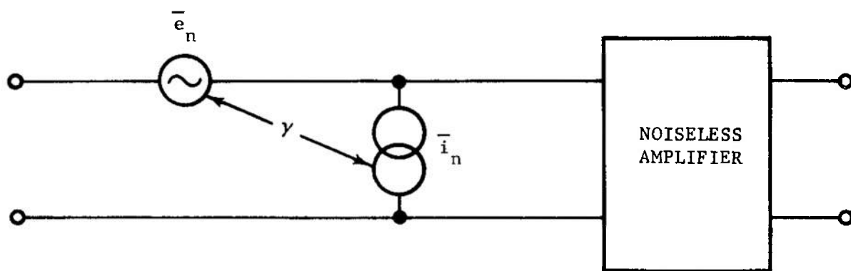
FIGURE 3-99. \bar{e}_n, \bar{i}_n Noise Equivalent Circuit
