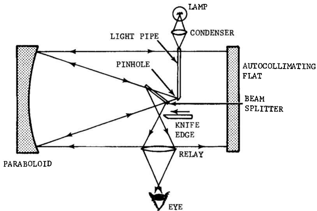
(B) KNIFE-EDGE TEST SETUP FOR PARABOLOIDAL MIRROR
