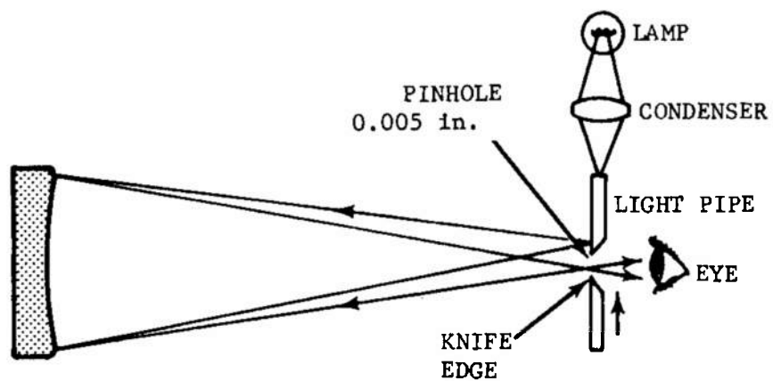
(A) KNIFE-EDGE TEST SETUP FOR SPHERICAL MIRROR
