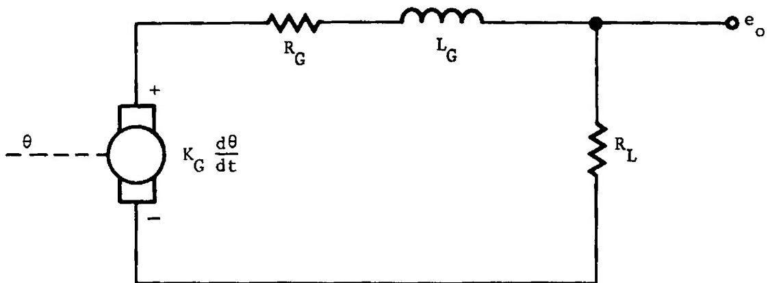
FIGURE 3-160. Equivalent Circuit of Tachometer Generator
