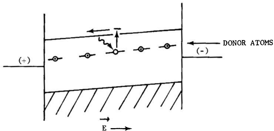
FIGURE 3-63. Semiconductor (N-type Extrinsic Detector) With Donors
