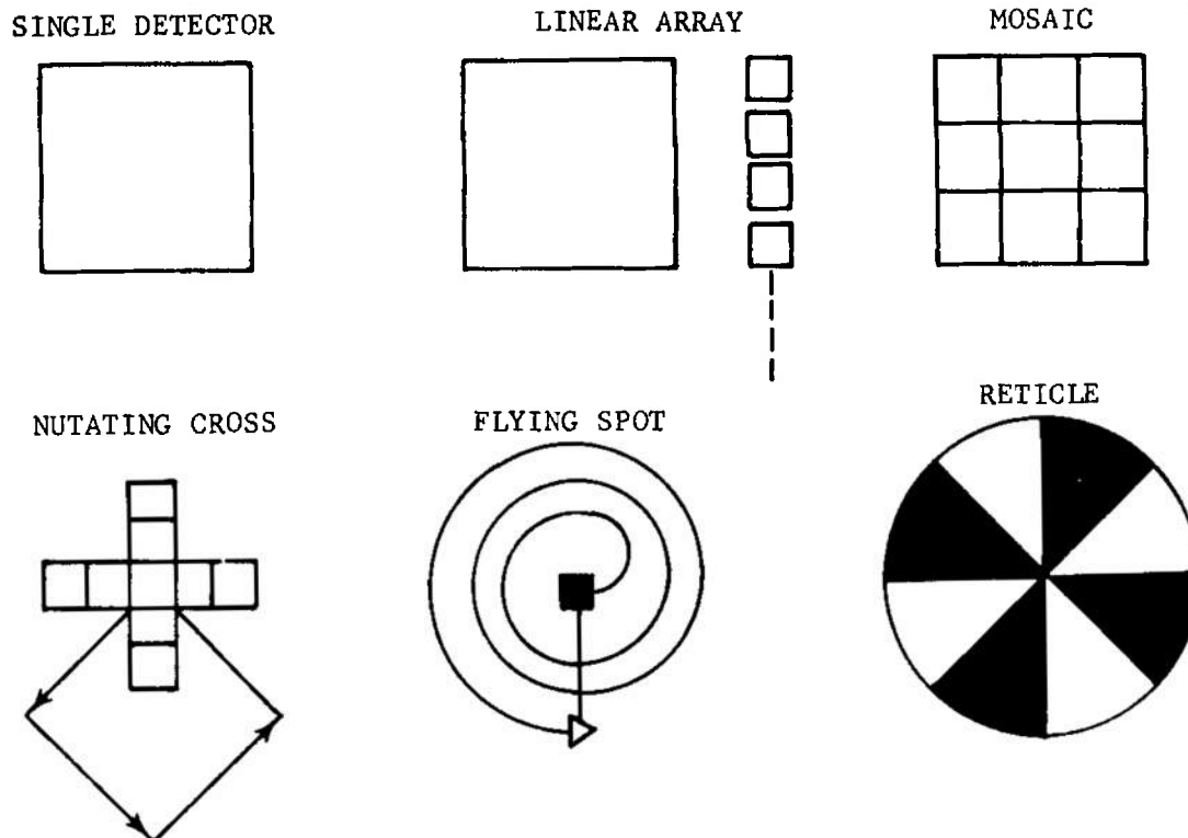
FIGURE 5-17. Basic Scan Modes
