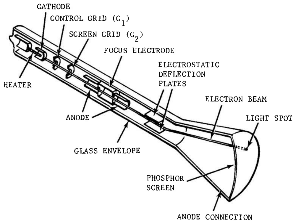
(A) ELECTROSTATIC FOCUS AND DEFLECTION CRT
