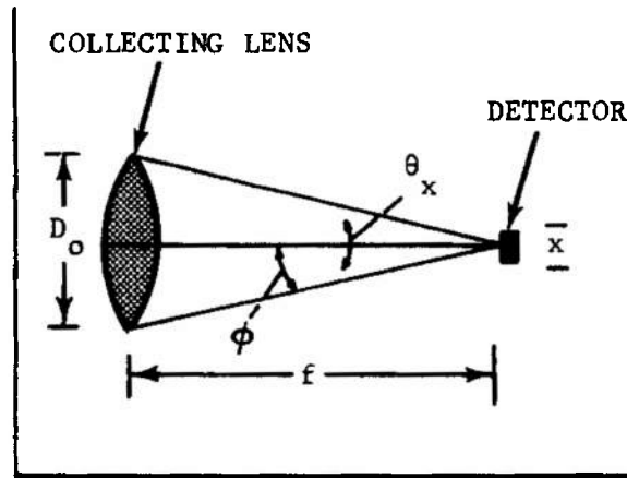
FIGURE 5-13. Optical Diagram
