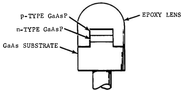
(A) INDIVIDUAL GaAsP Diode
