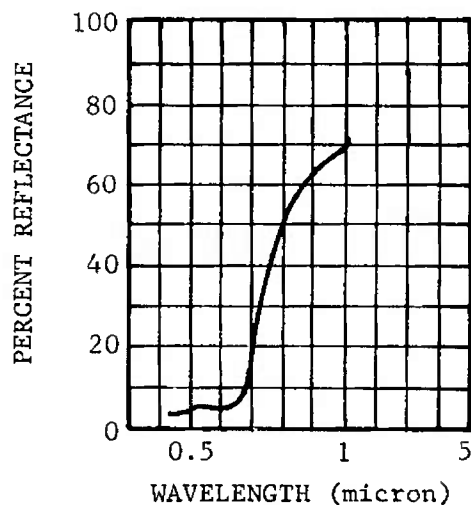
FIGURE 2-70. Reflectance from Typical Uniform Cloth
