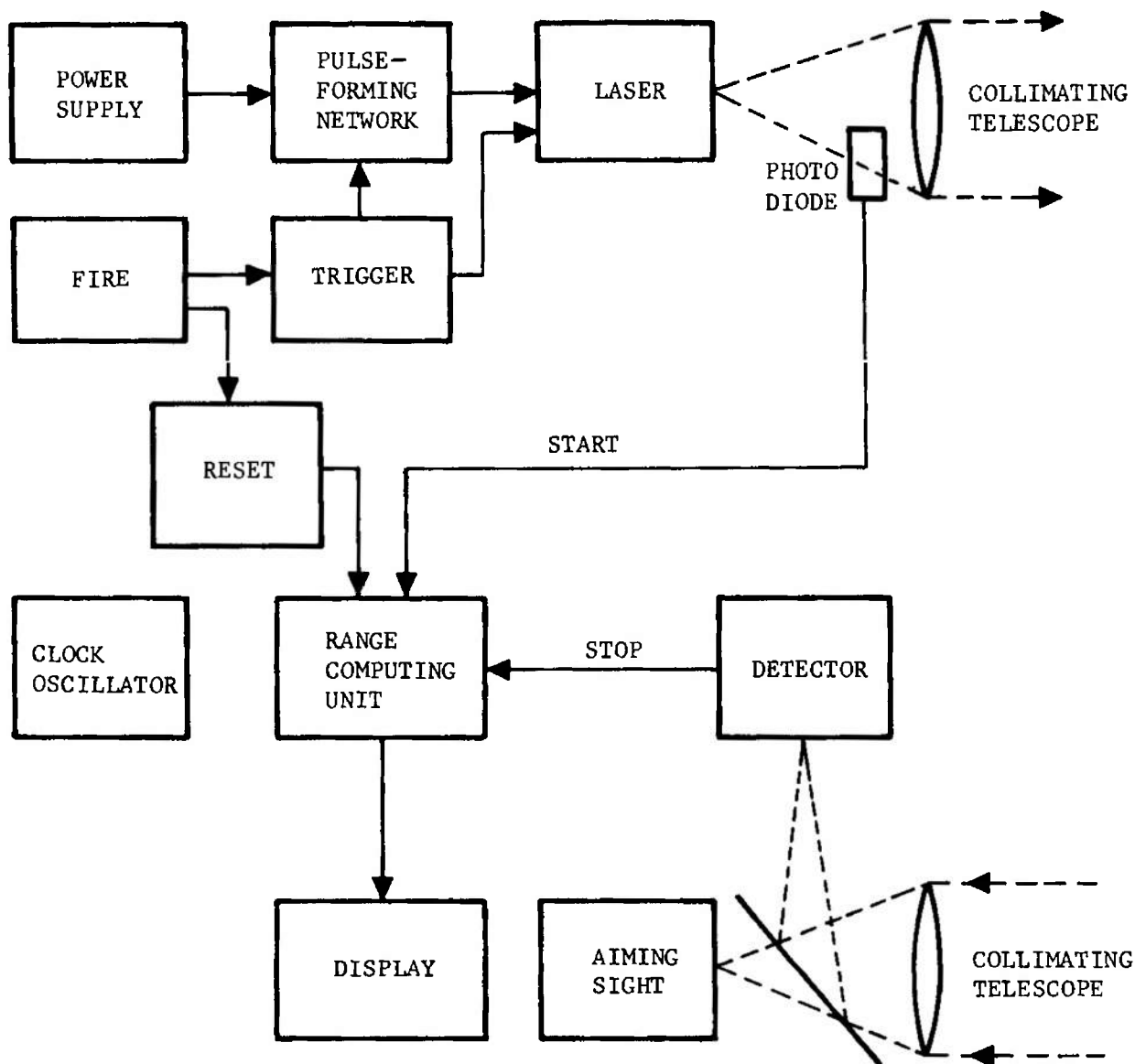
FIGURE 4-7. Typical Laser Rangefinder Block Diagram
