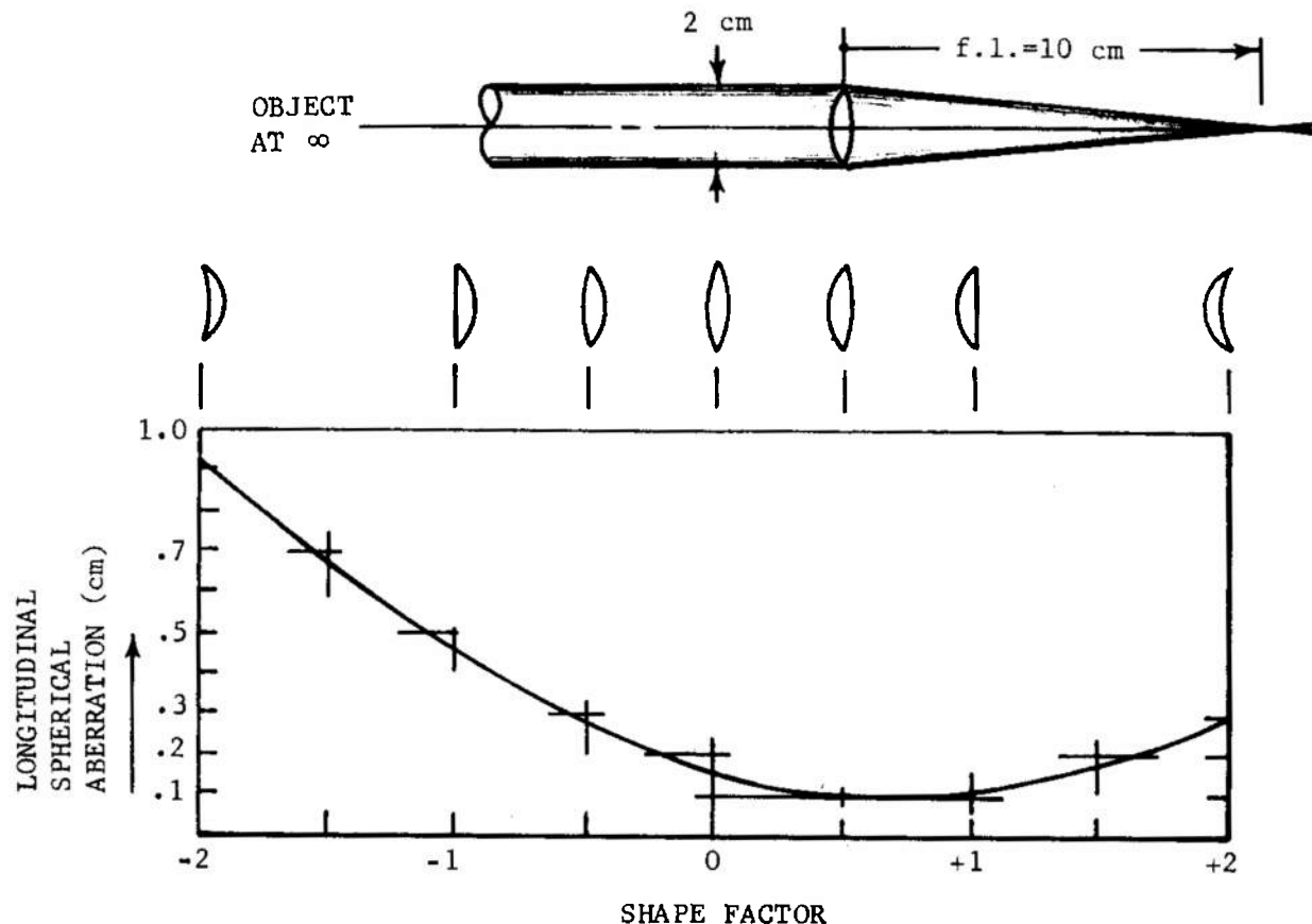
FIGURE 3-26. Lens Bending for Minimum Spherical Aberration
