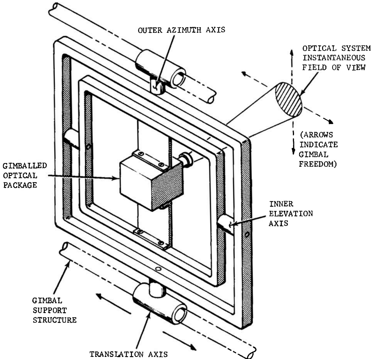
FIGURE 3-150. Conceptual Layout of Three-axis Gimbal Assembly
