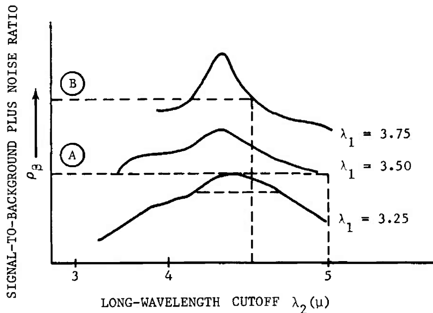
FIGURE 5-11. Signal-to-background Plus Noise Ratio for Various Upper and Lower Wavelength Cutoffs
