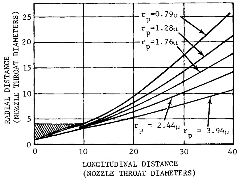
FIGURE 2-58. Limiting Particle Streamlines in the Near Field
