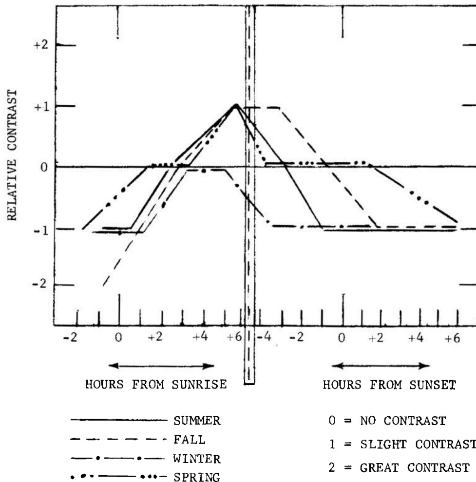
FIGURE 2-32. Relative Contrast of a Small Asphalt-surfaced Concrete Bridge to an Asphalt Roadway
