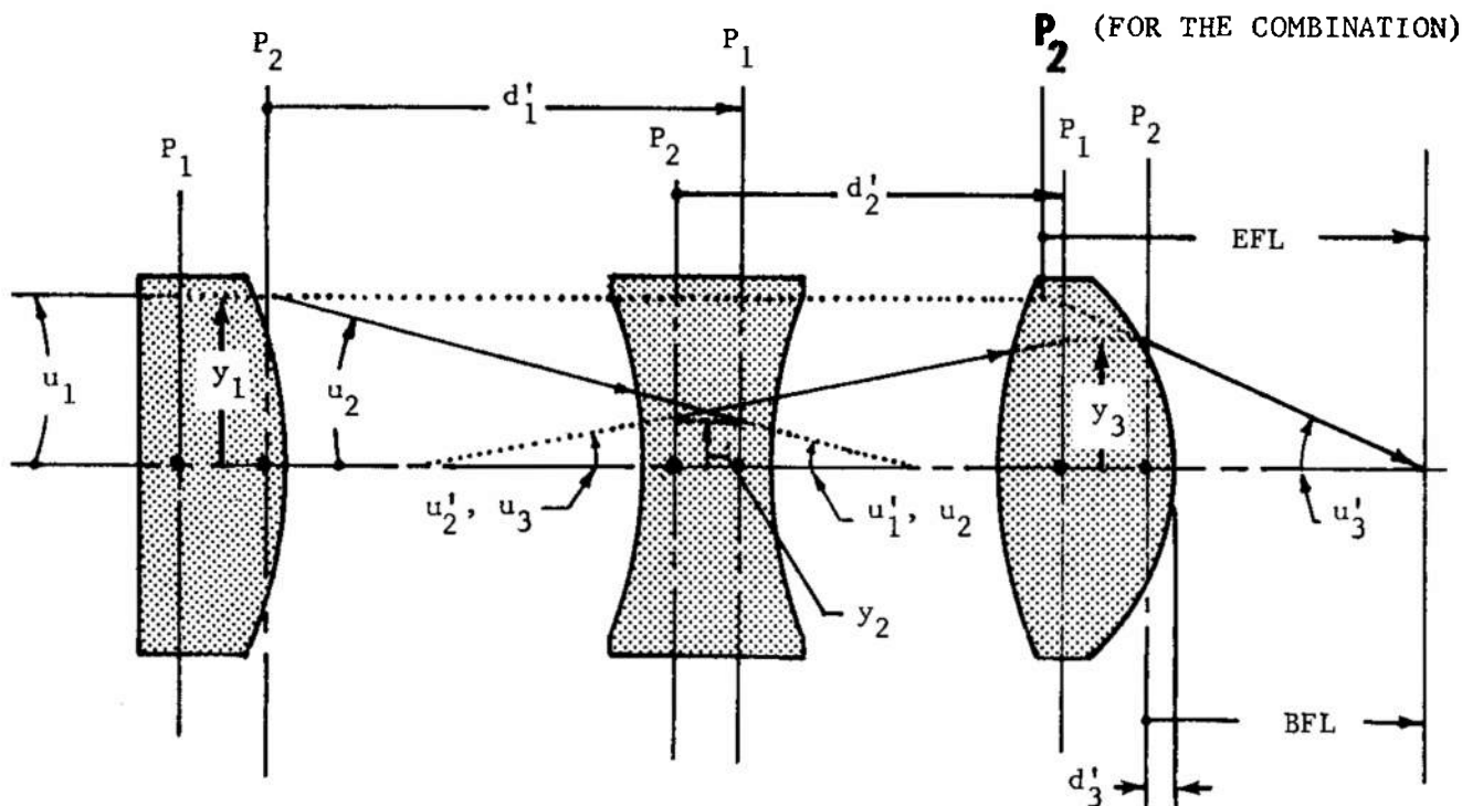
FIGURE 3-12. System Cardinal Points by Ray Tracing
