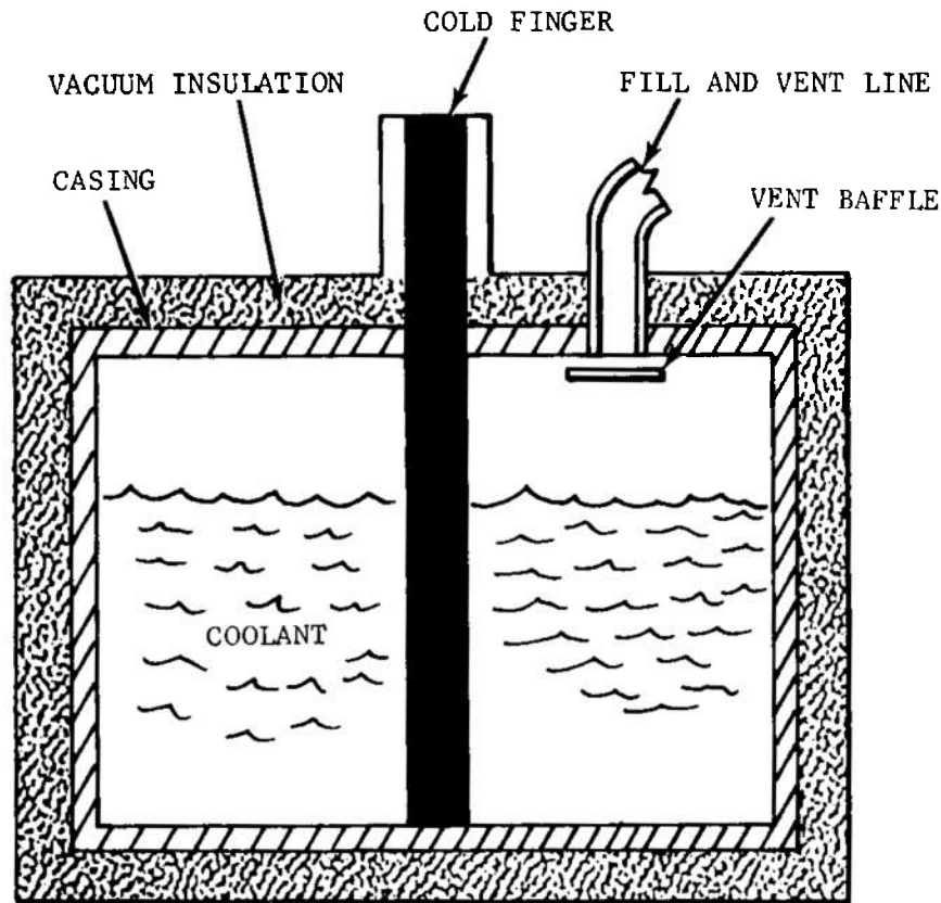
FIGURE 3-79. Liquid Cryogen Cooling System
