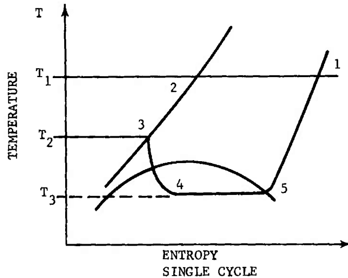
FIGURE 3-84. Joule-Thomson Closed Cycle System Temperature-entropy Diagram
