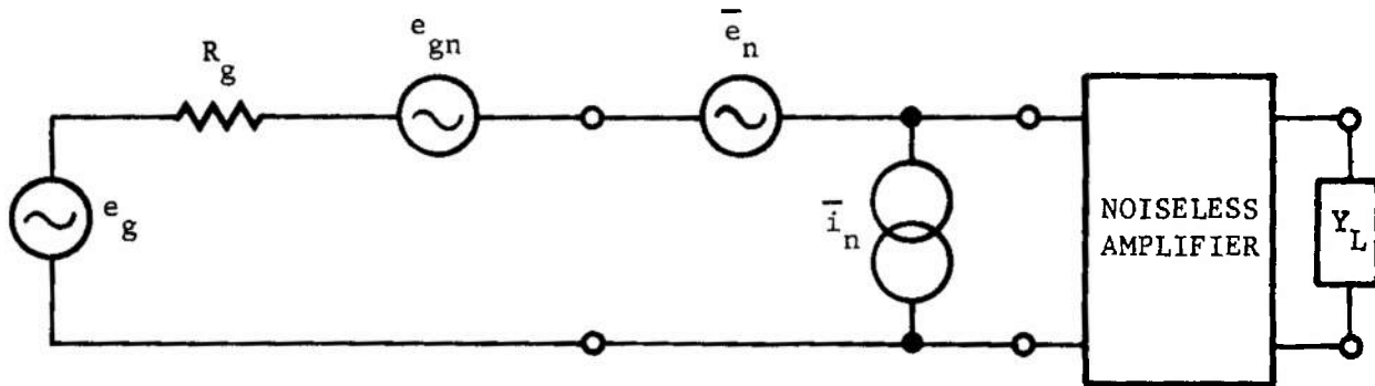
FIGURE 3-100. \bar{e}_n, \bar{i}_n Approach Noise Figure Computational Model
