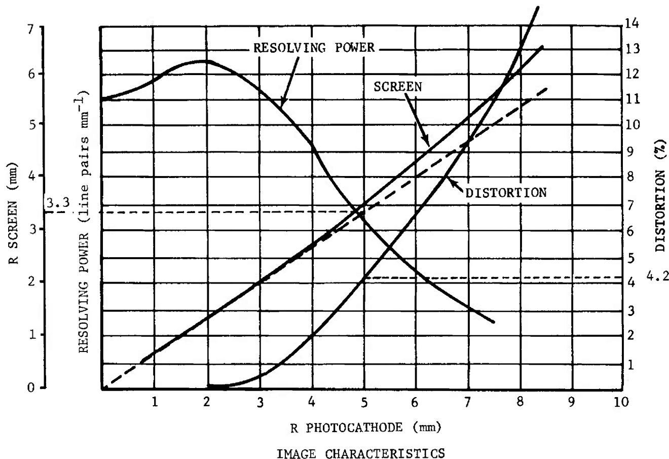
FIGURE 3-127. Image Quality of Image Converter Tube in Terms of Distortion
