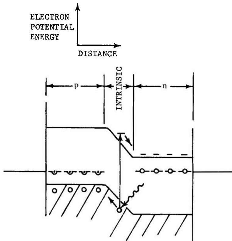
FIGURE 3-65. P-n Junction (Photovoltaic Detector)
