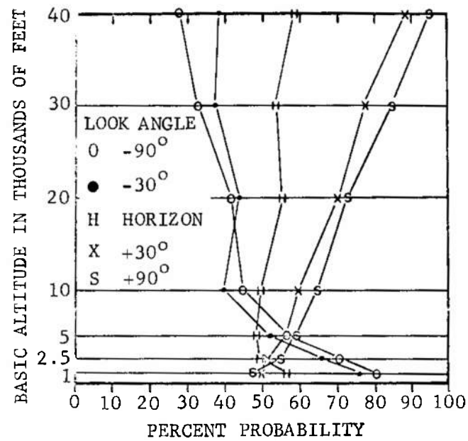
FIGURE 2-38. Probability of Clear Lines-of-sight over Northern Hemisphere for All Seasons Combined
