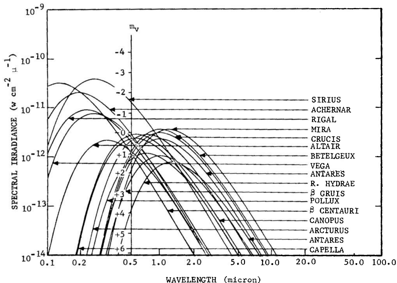
FIGURE 2-41. Spectral Irradiance of the Brightest Visual and Red Stars As a Function of Wavelength
