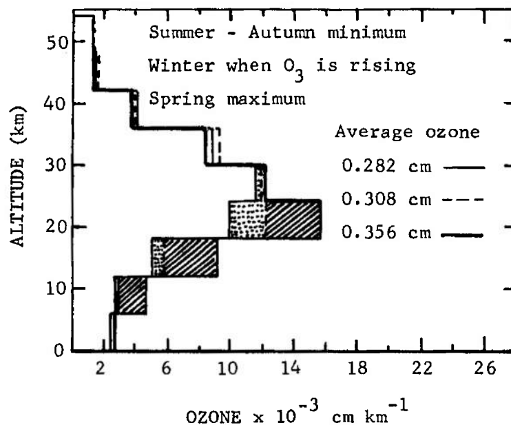
FIGURE 2-7. Seasonal Variation of the Vertical Distribution of Ozone
