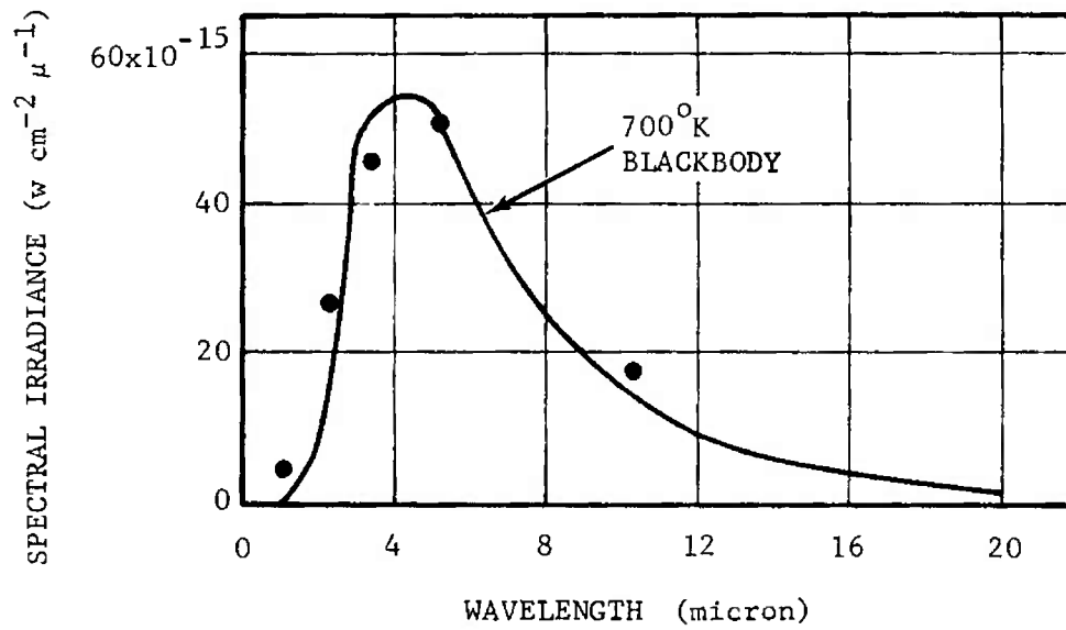
FIGURE 2-45. Spectral Irradiance of the Cygnus Infrared Star As a Function of Wavelength
