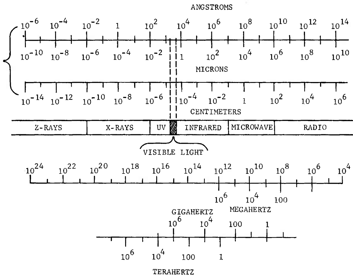
FIGURE 2-21. The Electromagnetic Spectrum
