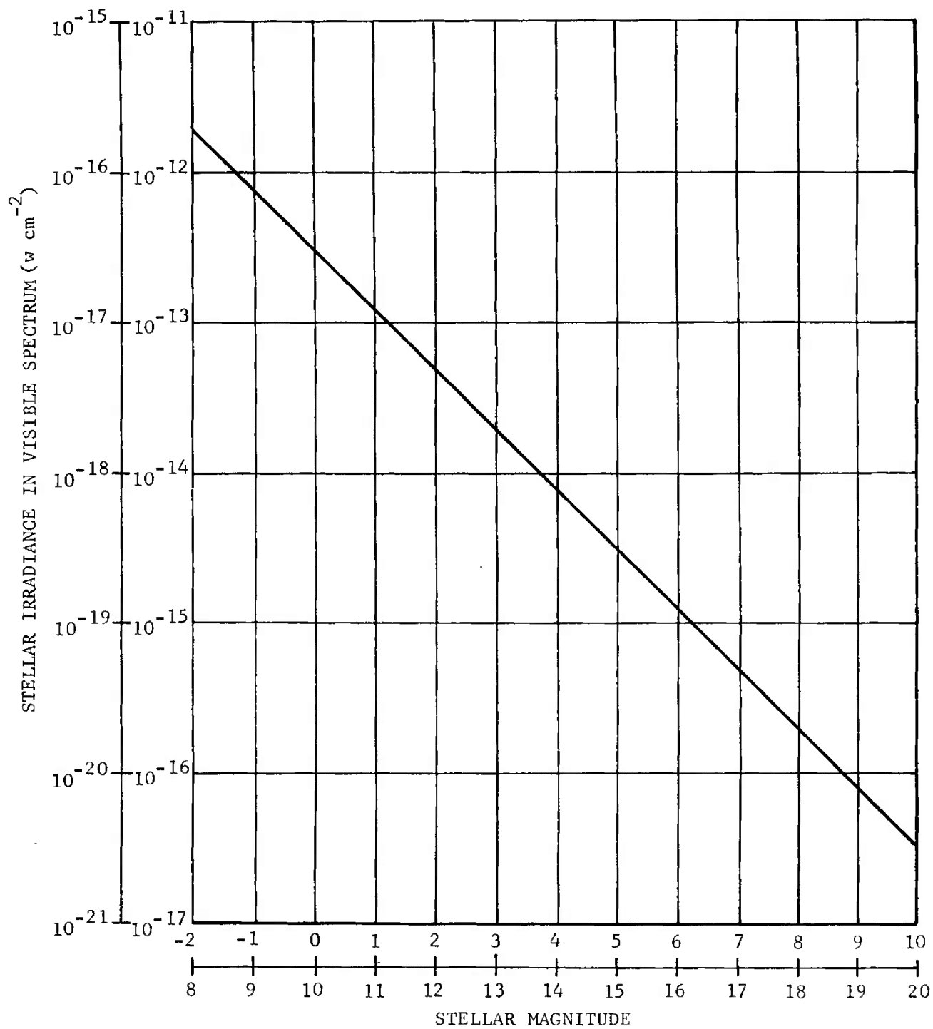
FIGURE 2-46. Stellar Irradiance As a Function of Visual Magnitude
