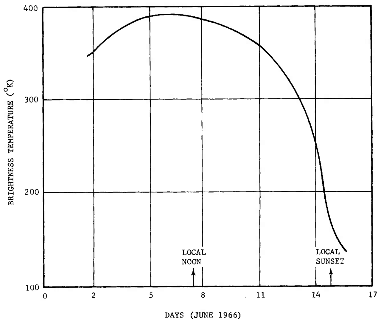
FIGURE 2-51. Lunar Temperature Measured by Surveyor I
