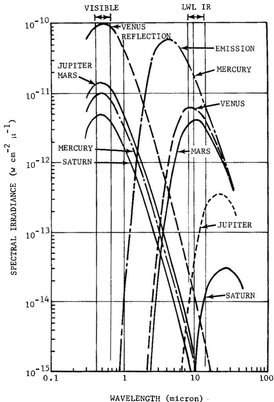
FIGURE 2-42. Major Planet Solar Reflection and Emission
