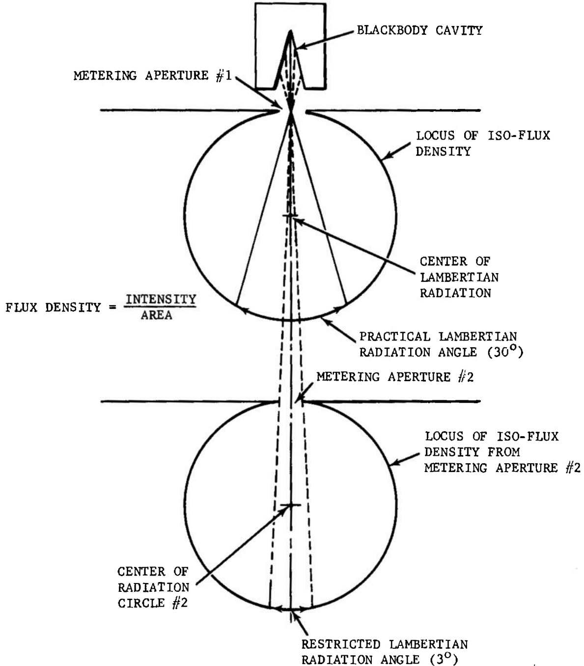
FIGURE 3-145. Lambertian Radiation
