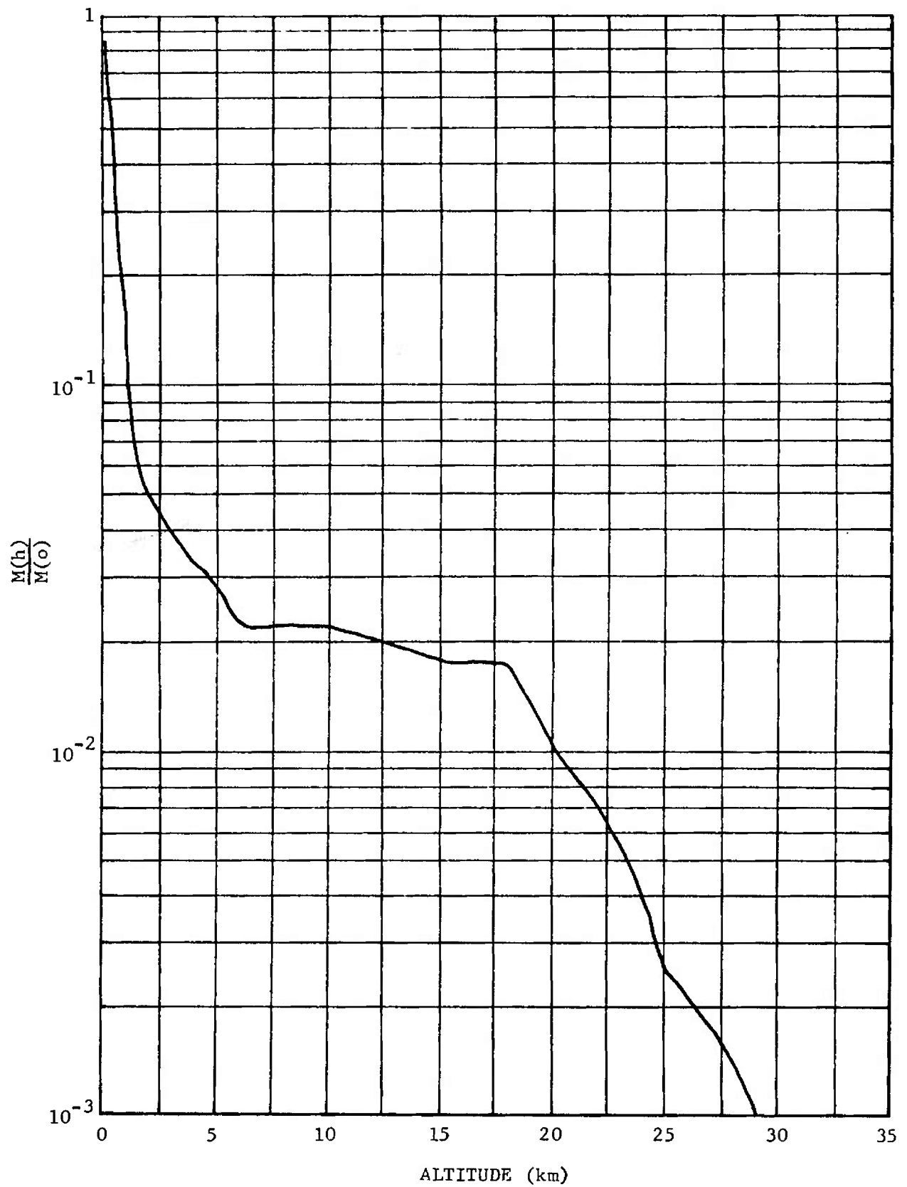
FIGURE 2-17. Normalized Particle Density as a Function of Altitude
