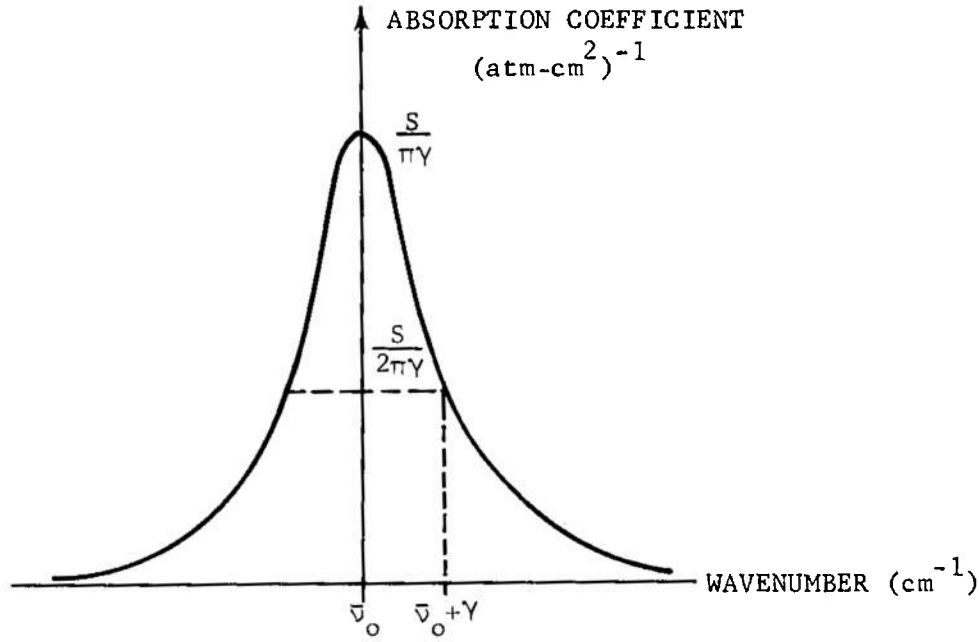
FIGURE 2-10. Lorentz Line Shape
