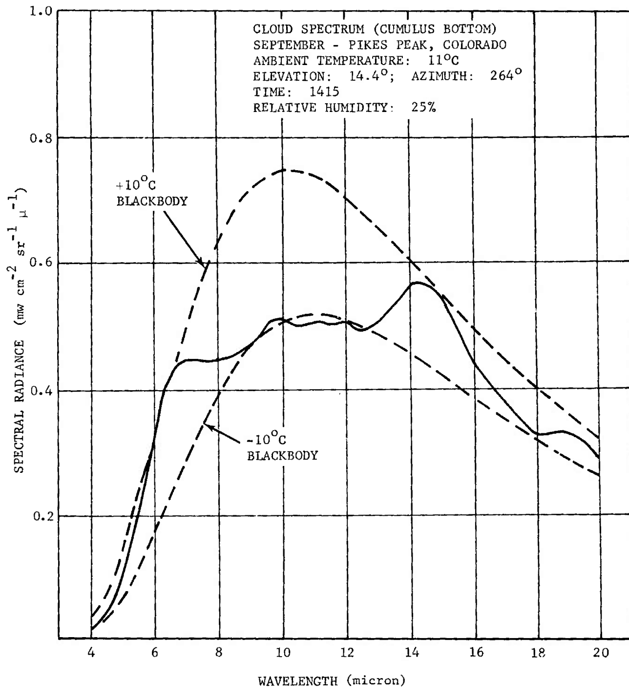
FIGURE 2-37. Cloud Spectrum
