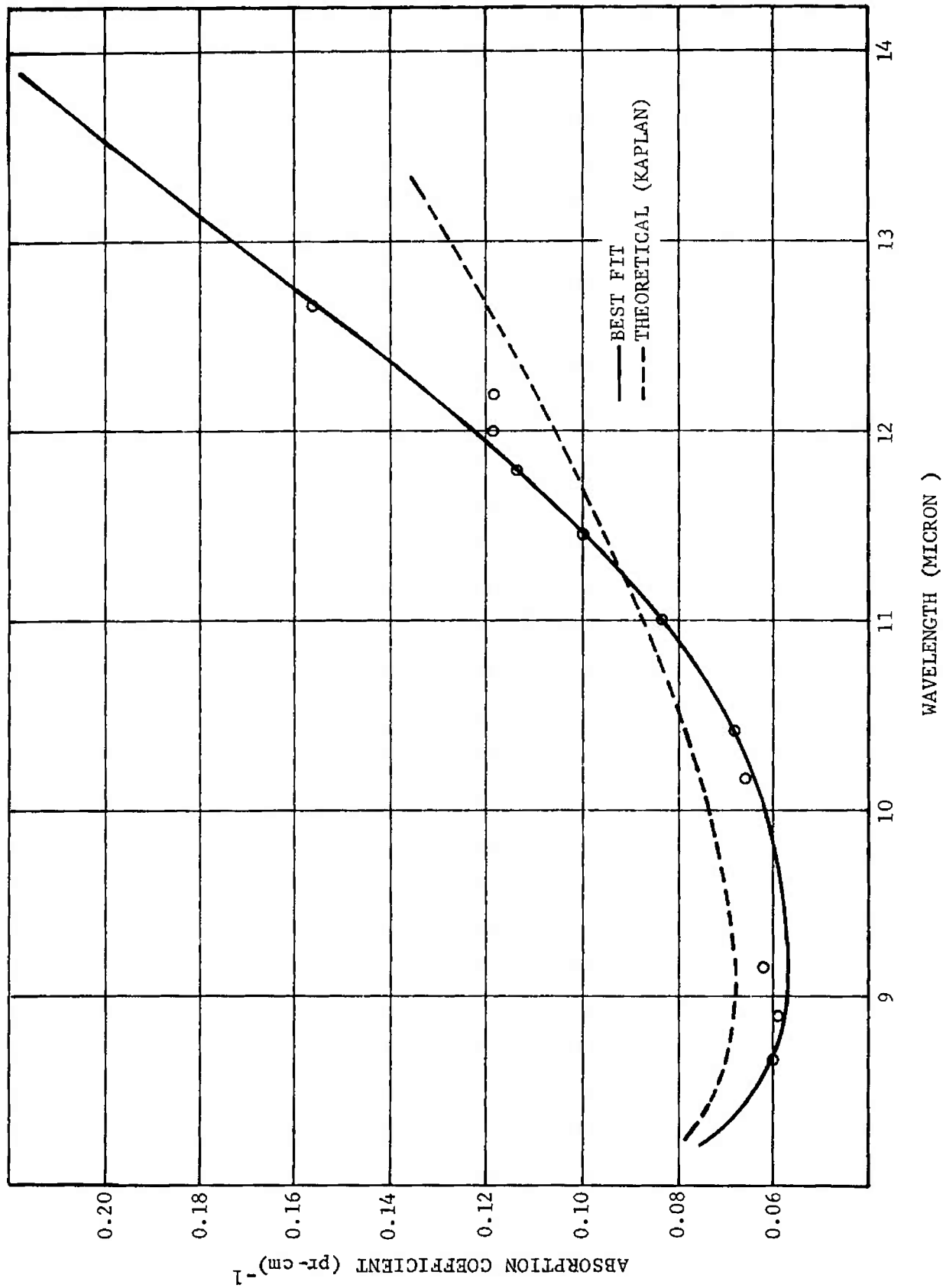
FIGURE 2-13. Variation of Continuum Absorption Coefficient vs Wavelength
