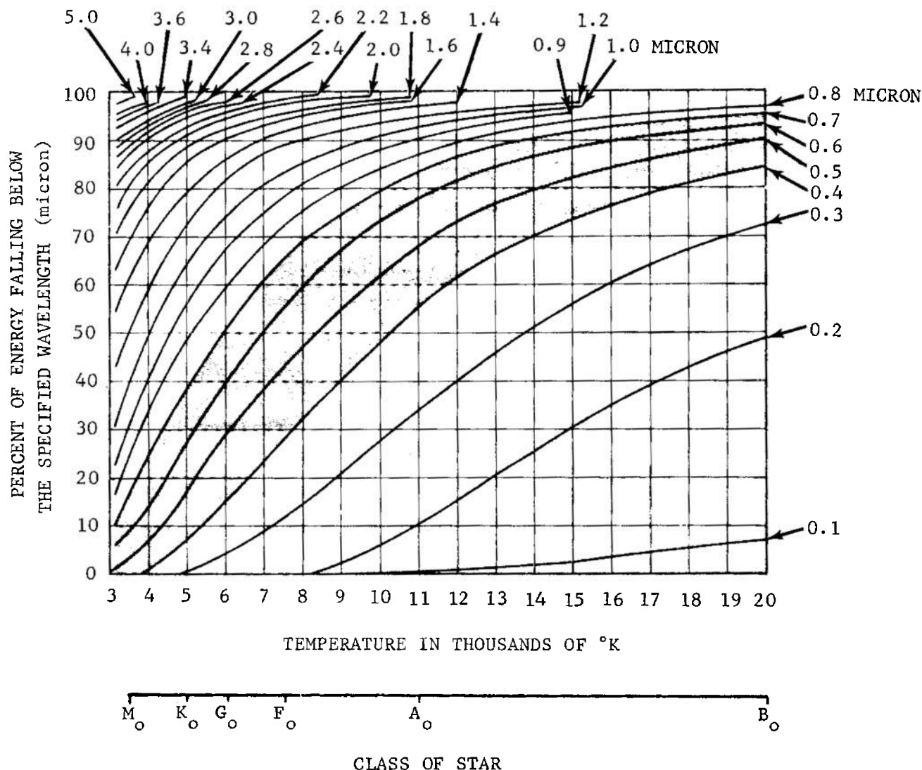
FIGURE 2-48. Relative Spectral Distribution of Stellar Radiation As a Function of Star Class
