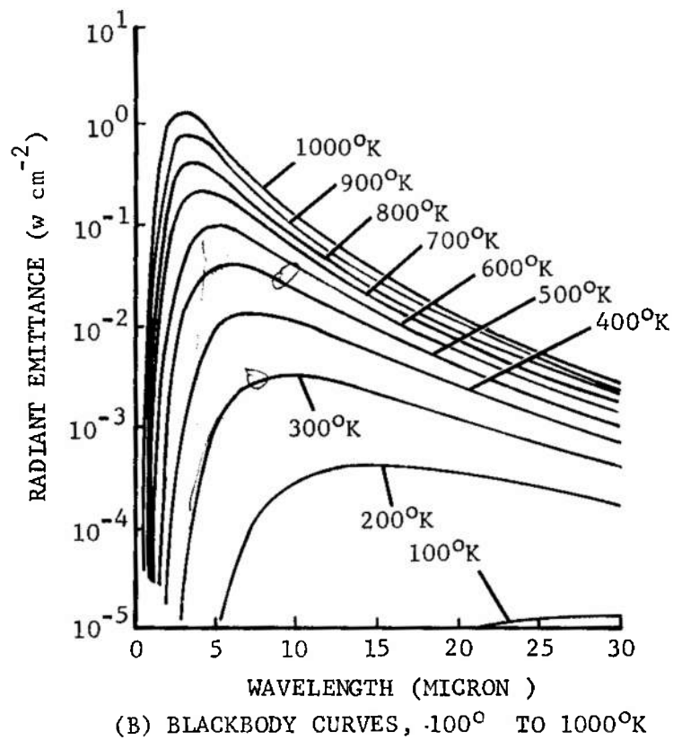
FIGURE 2-3. Blackbody Curves
