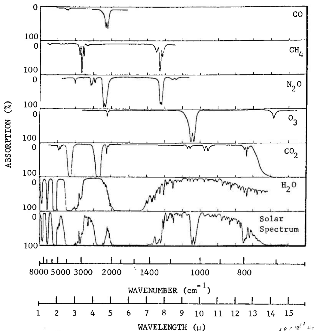
FIGURE 2-6. The Near-infrared Spectra of Solar Irradiation and of CO, CH 4 , N 2 O, O 3 , CO 2 , and H 2 O
