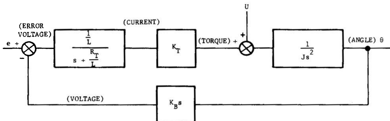
FIGURE 3-159. Block Diagram of dc Torque Motor
