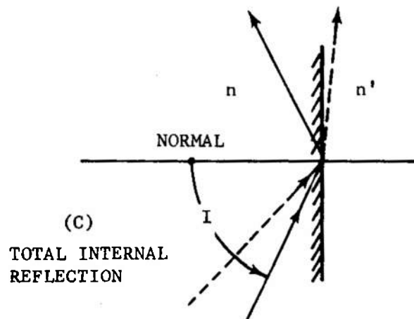
FIGURE 3-20. Geometrical Presentation of Refracted and Reflected Rays
