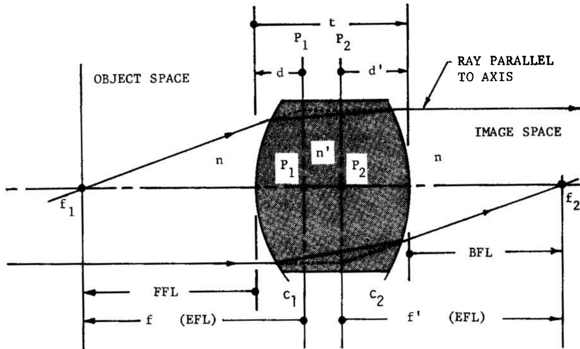
FIGURE 3-11. Cardinal Points for Double-surface Thick Lens Element
