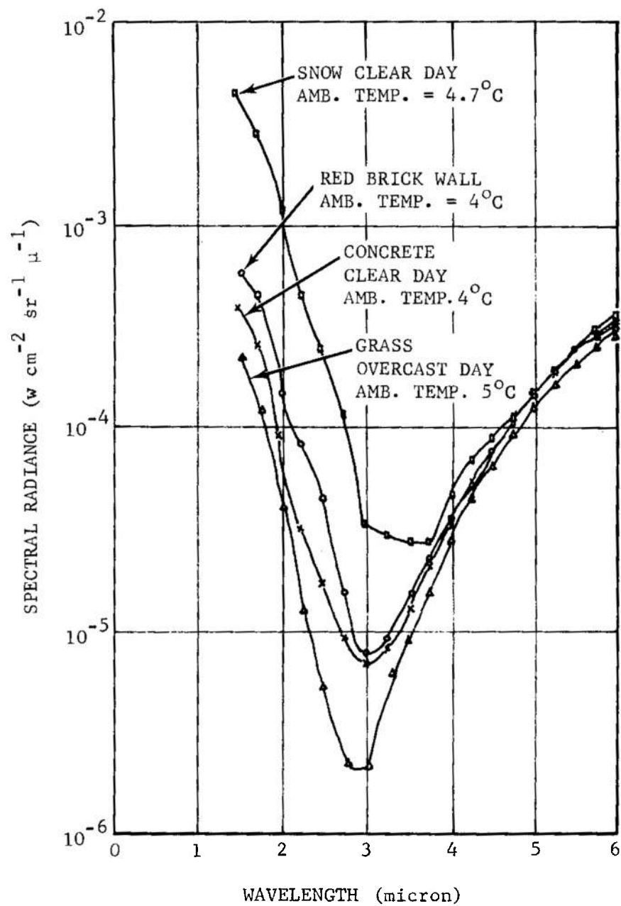
FIGURE 2-29. Daytime Spectral Radiance of Miscellaneous Targets
