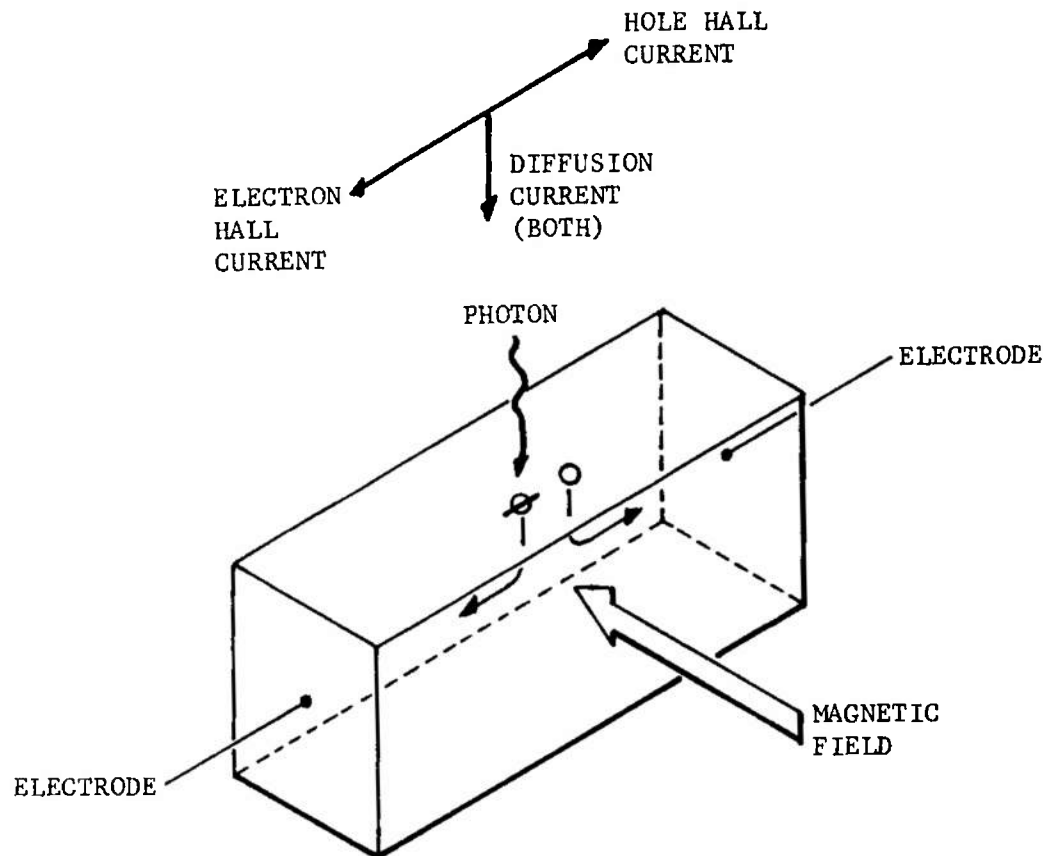
FIGURE 3-66. Photo-induced Hall Effect (Photoelectromagnetic Detector)
