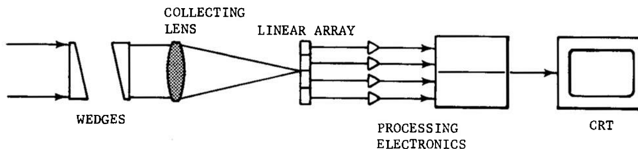
FIGURE 5-19. Scanning Image System
