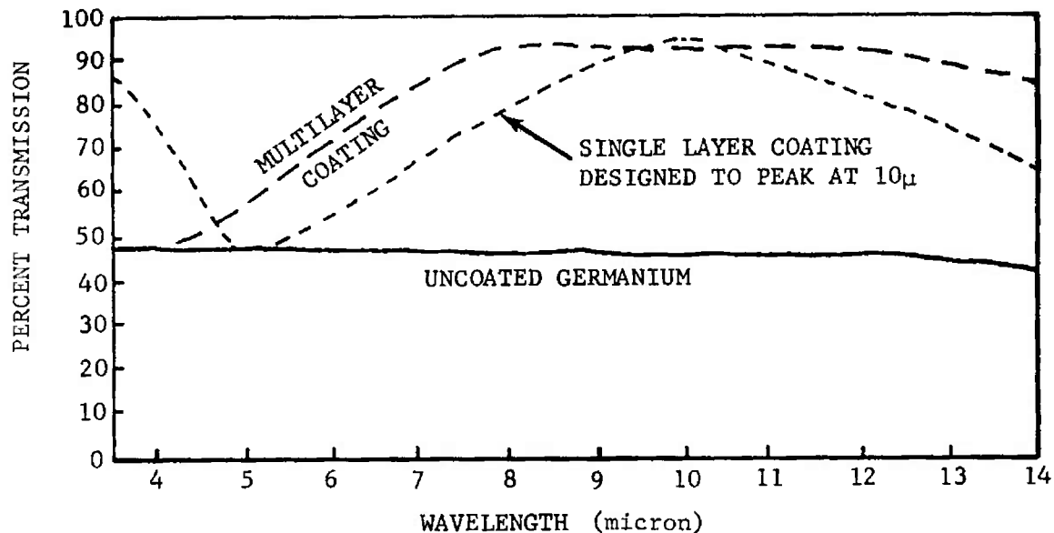
FIGURE 3-4. Effects of Anti-reflection Coatings on Ge Transmission
