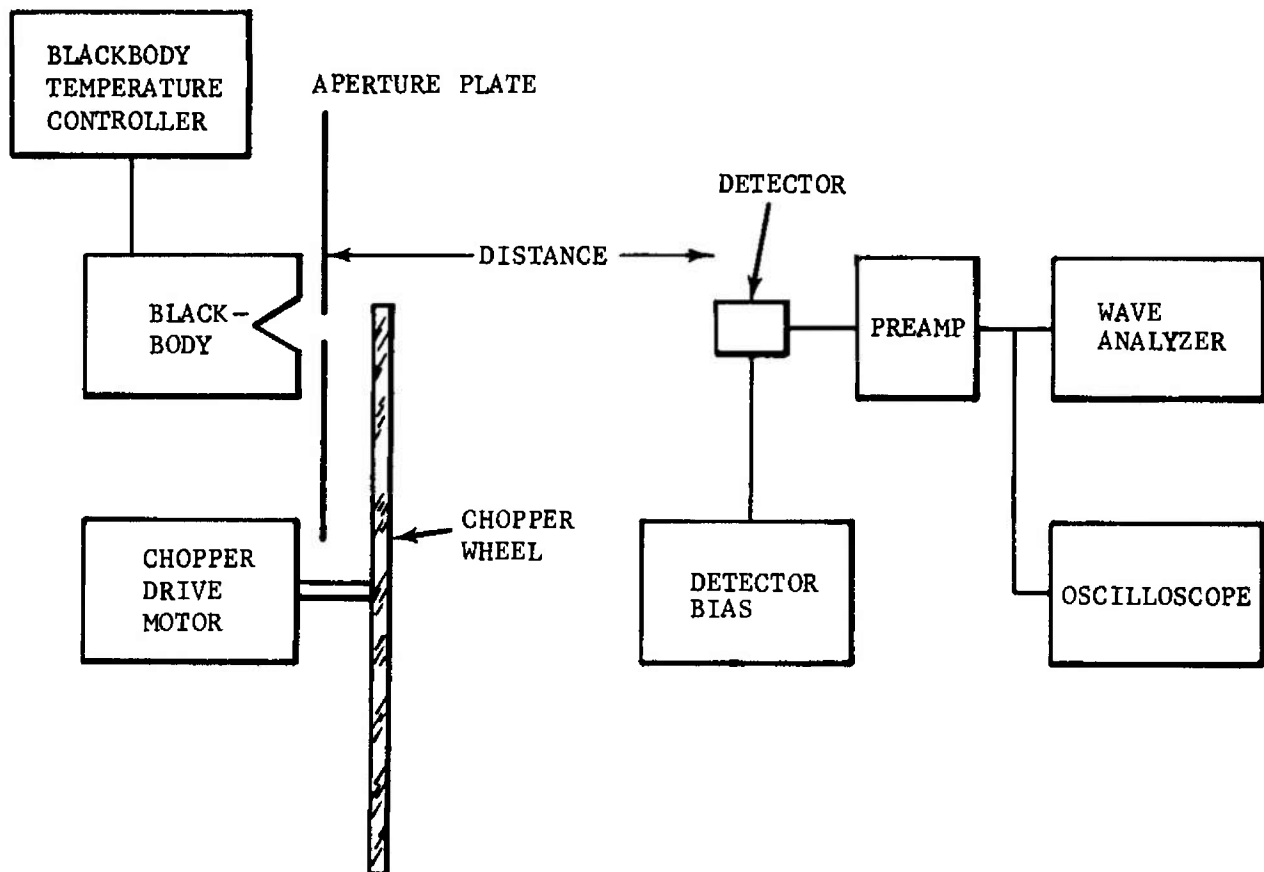
FIGURE 3-71. Block Diagram of D^* Measurement Apparatus
