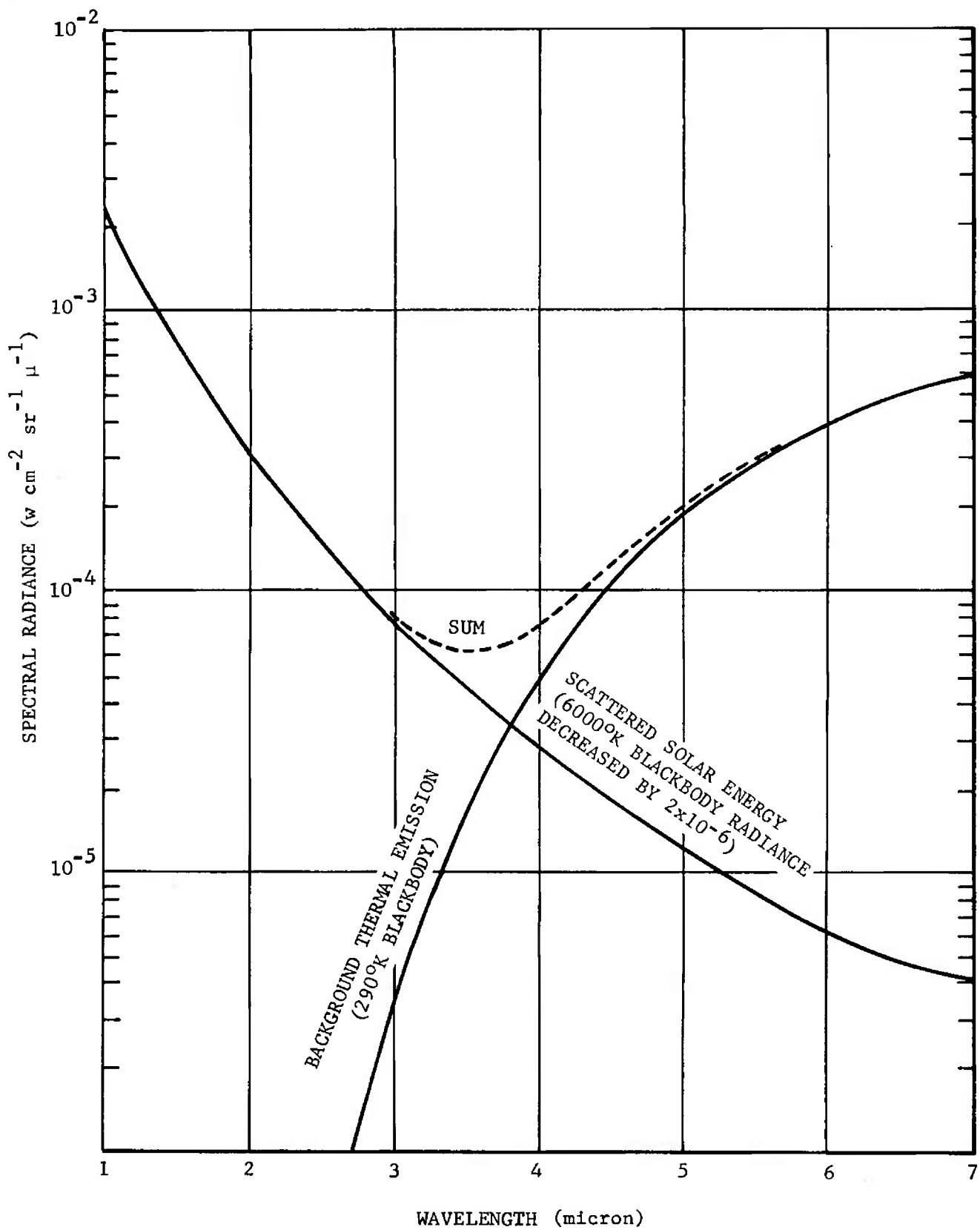
FIGURE 2-25. Idealized Background Spectrum
