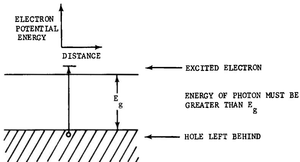
FIGURE 3-61. Electron Excited by a Photon
