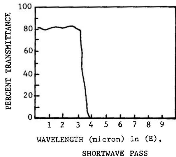
FIGURE 3-7. Typical Spectrophotometric Filter Curves
