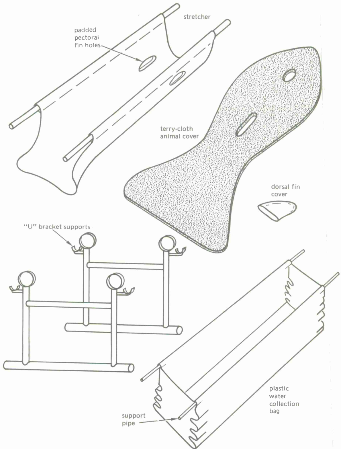
Figure 5.11. Disassembled parts of "U bracket" transport device.
