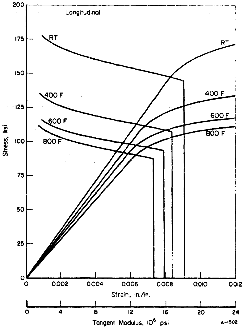
FIGURE 44. TYPICAL COMPRESSIVE STRESS-STRAIN AND TANGENT-MODULUS CURVES FOR SOLUTION-TREATED AND ACED Ti-6Al-2Zr-2Sn-2Mo-2Cr PLATE (LONGITUDINAL)
