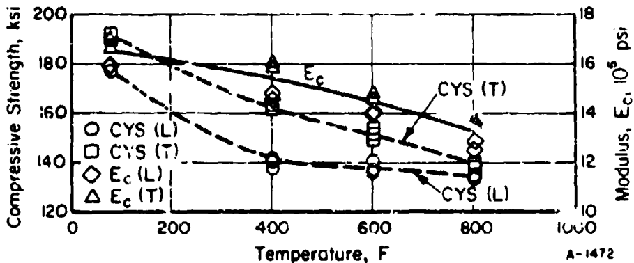
FIGURE 37. EFFECT OF TEMPERATURE ON THE COMPRESSIVE PROPERTIES OF SOLUTION-TREATED AND AGED Ti-8Mo-8V-2Fe-3Al SHEET
