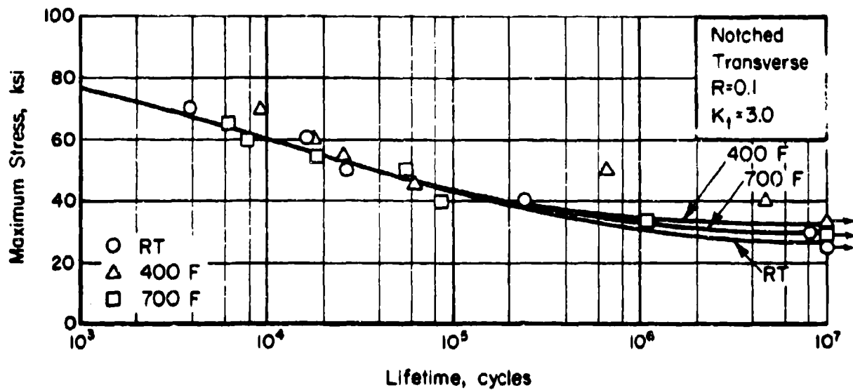
FIGURE 56. AXIAL LOAD FATIGUE BEHAVIOR OF NOTCHED ( K_t = 3.0 ) SOLUTION-TREATED AND AGED Ti-6Al-6V-2Sn ISOTHERMAL DIE FORGINGS (TRANSVERSE)
