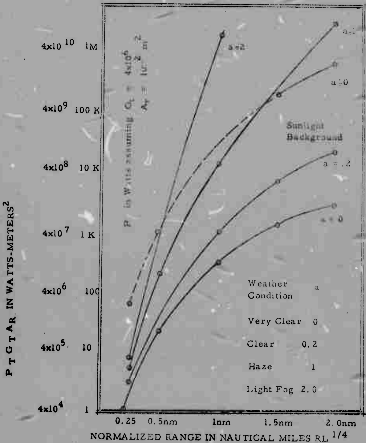
LASER RADAR RANGE, plotted for varying weather conditions, falls off sharply during haze and light fog. Left ordinate is a product of peak transmitter gain and receiving aperture area, parameters which can be traded in laser radar design. The second ordinate is peak transmitter power.
