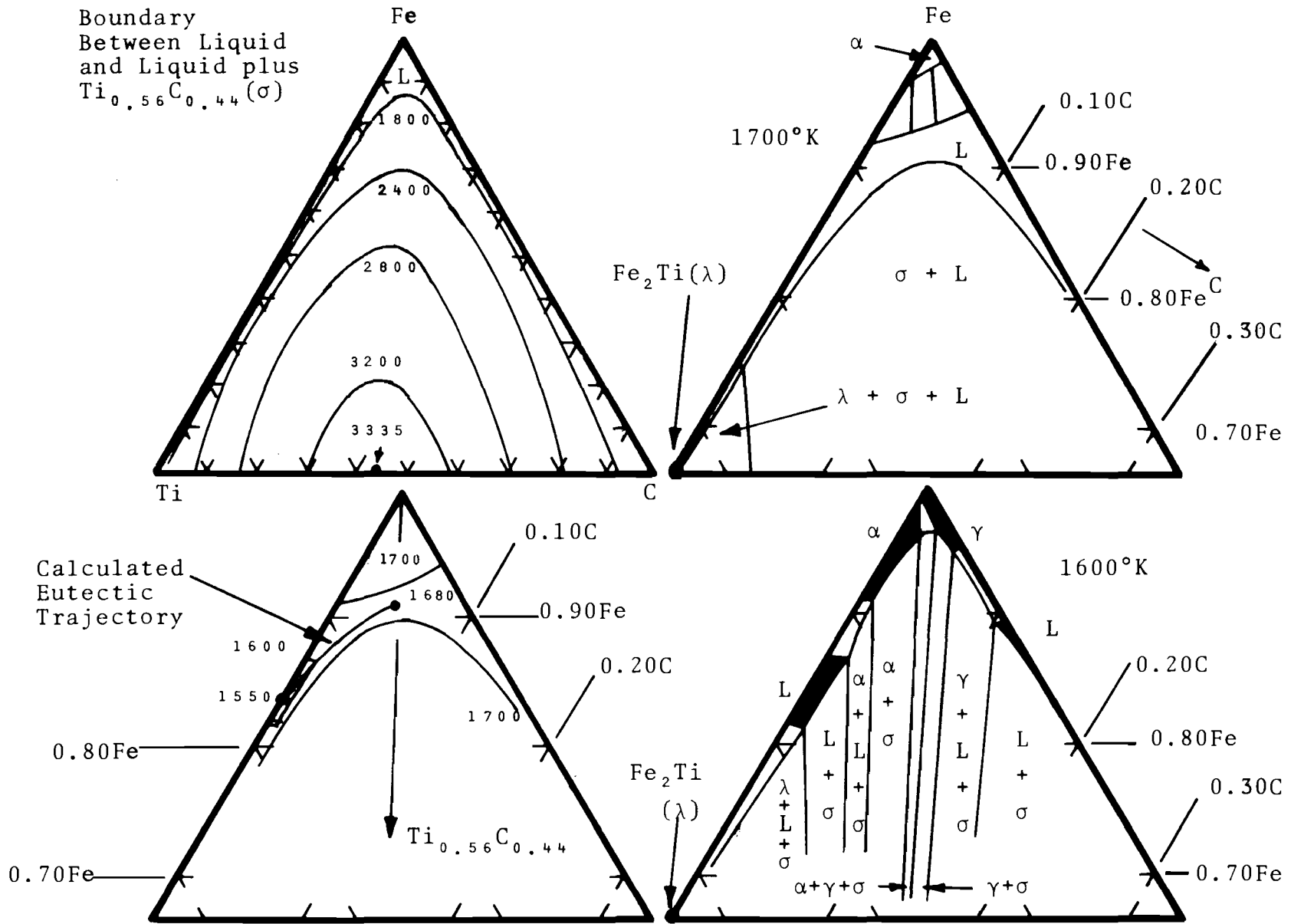
Figure 39 Calculated Liquidus in the Fe- Fe_2Ti -TiC region of the Fe-C-Ti System.
