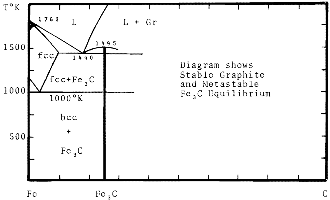
Figure 38 Calculated Phase Diagram for the Fe-C System.
