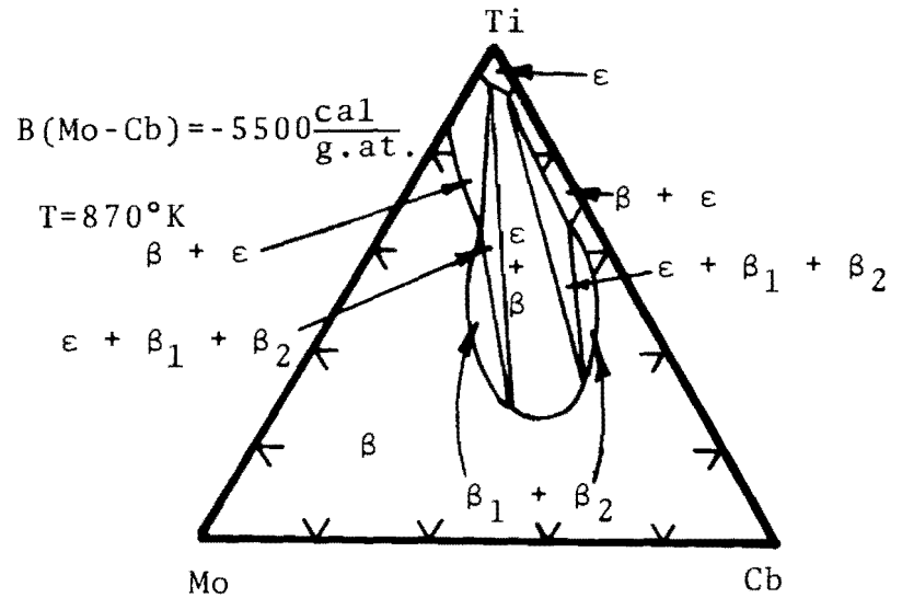
Figure 14 Calculated BCC/(BCC + HCP) Phase Boundaries in the Ti-Cb-Mo System. Observed Boundary at 870°K shown in the upper right corner
