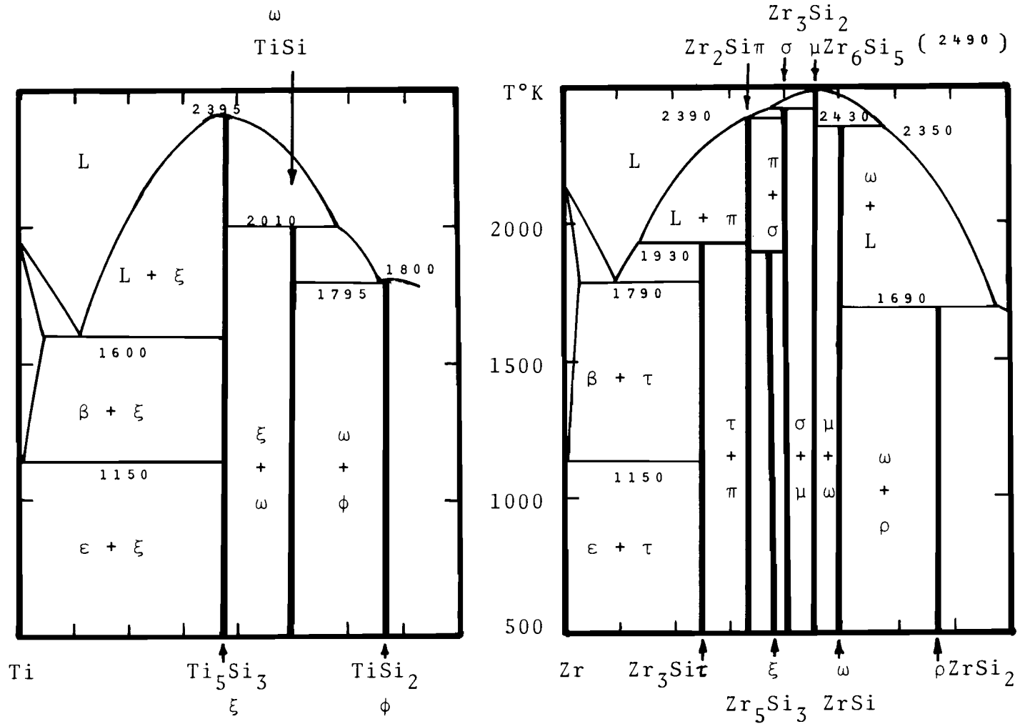
Figure 4. Calculated Partial Ti-Si and Zr-Si Phase Diagrams
