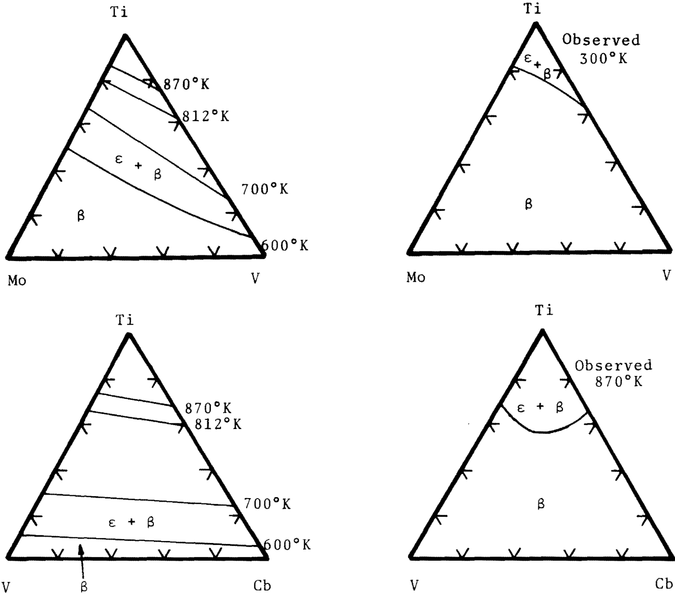
Figure 13 Calculated and Observed BCC/(HCP + BCC) Phase Boundaries in the Ti-V-Mo and Ti-Cb-V Systems
