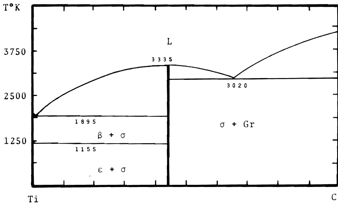
Figure 37. Calculated Phase Diagram for the Ti-C System.
