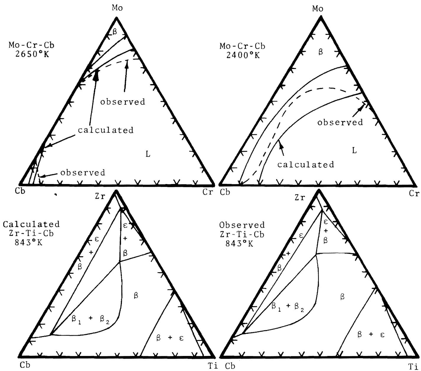
Figure 29 Calculated and Observed Isothermal Sections in Mo-Cr-Cb and Zr-Ti-Cb.
