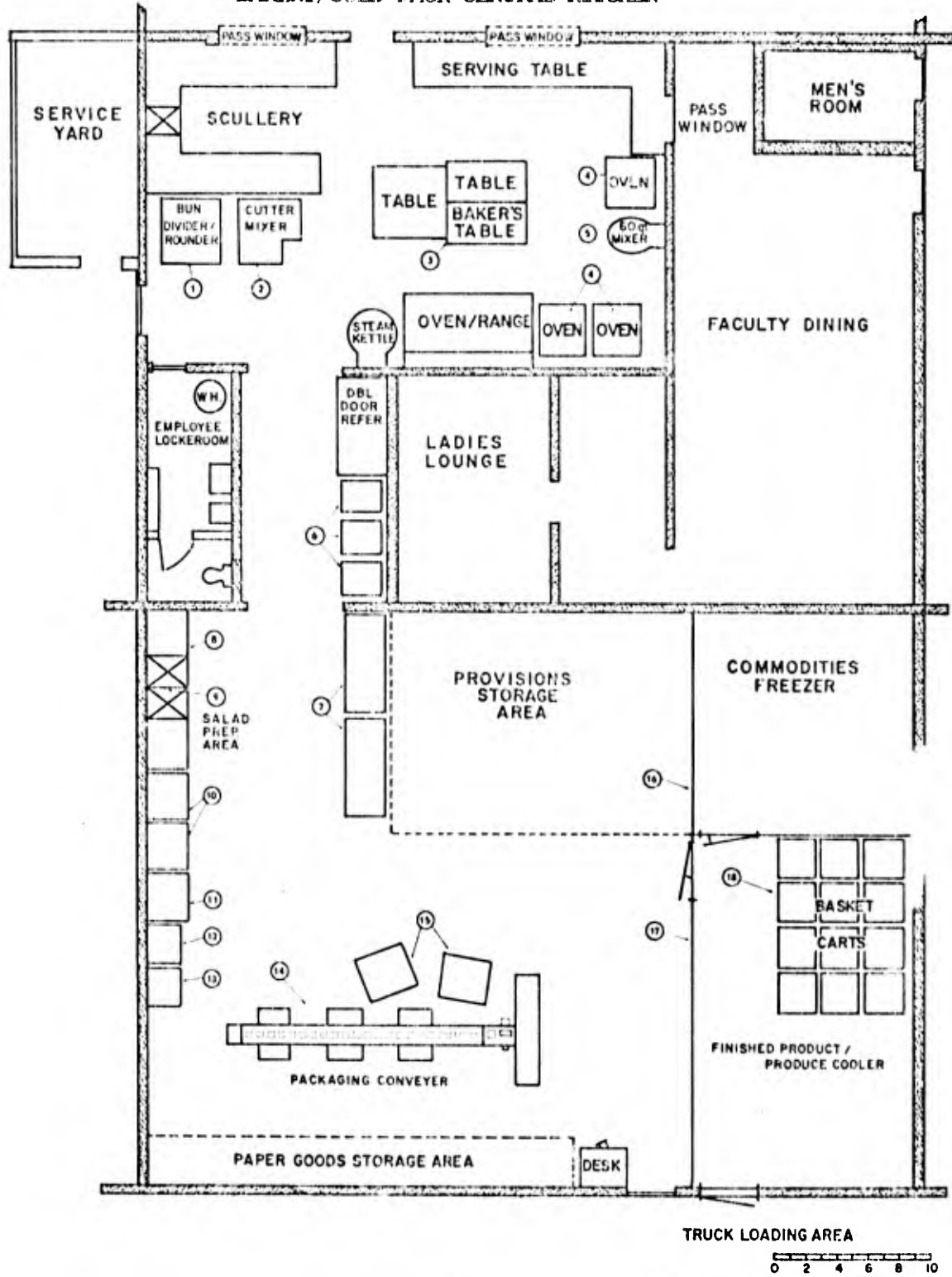
FIGURE 2. EXPANDED HIGHLAND SCHOOL KITCHEN
