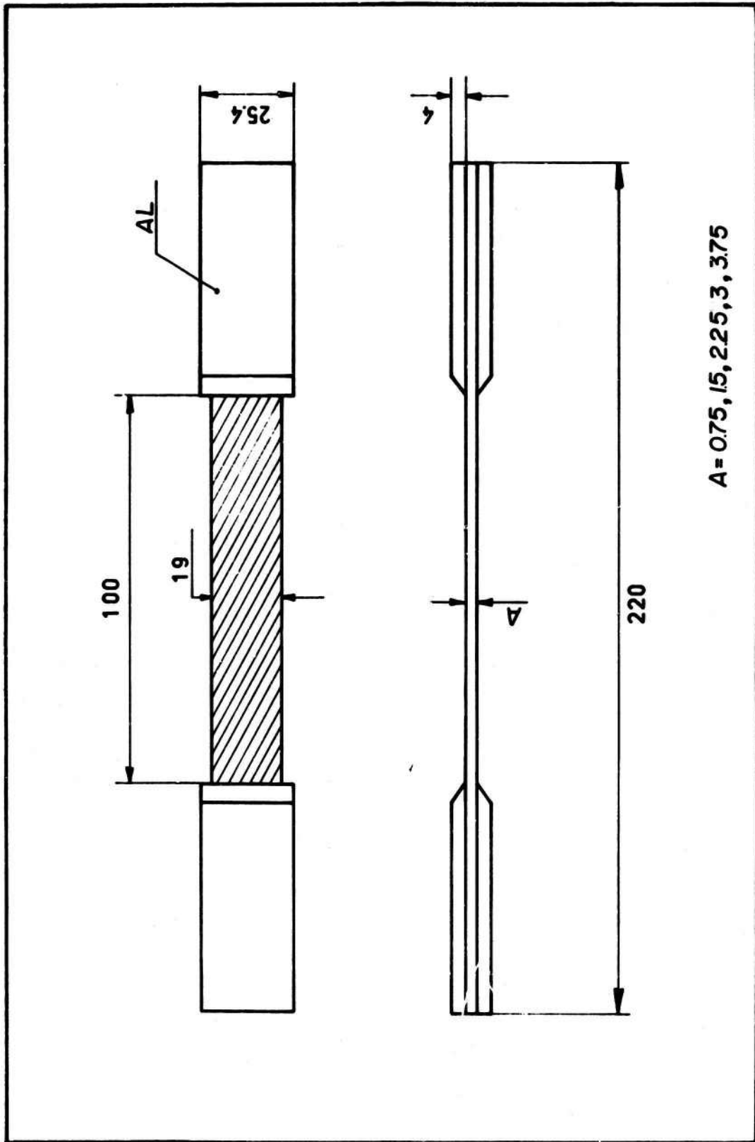
Fig. 4: Off-Axis Specimen.
