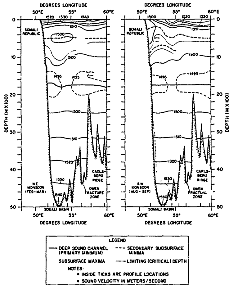
FIGURE A-4. SOUND VELOCITY CROSS-SECTIONS BETWEEN 9° AND 10° N, LATITUDE FOR NORTHEAST AND SOUTHWEST MONSOONS (SOMALI BASIN)
