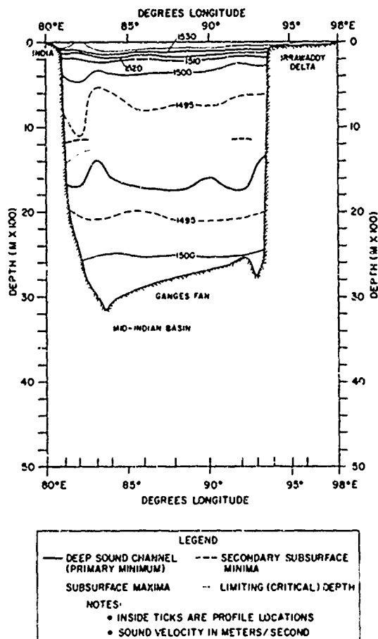
FIGURE A-3. SOUND VELOCITY CROSS-SECTION BETWEEN 15° AND 16° N. LATITUDE (BAY OF BENGAL) FOR NORTHEAST MONSOON (MAR)
