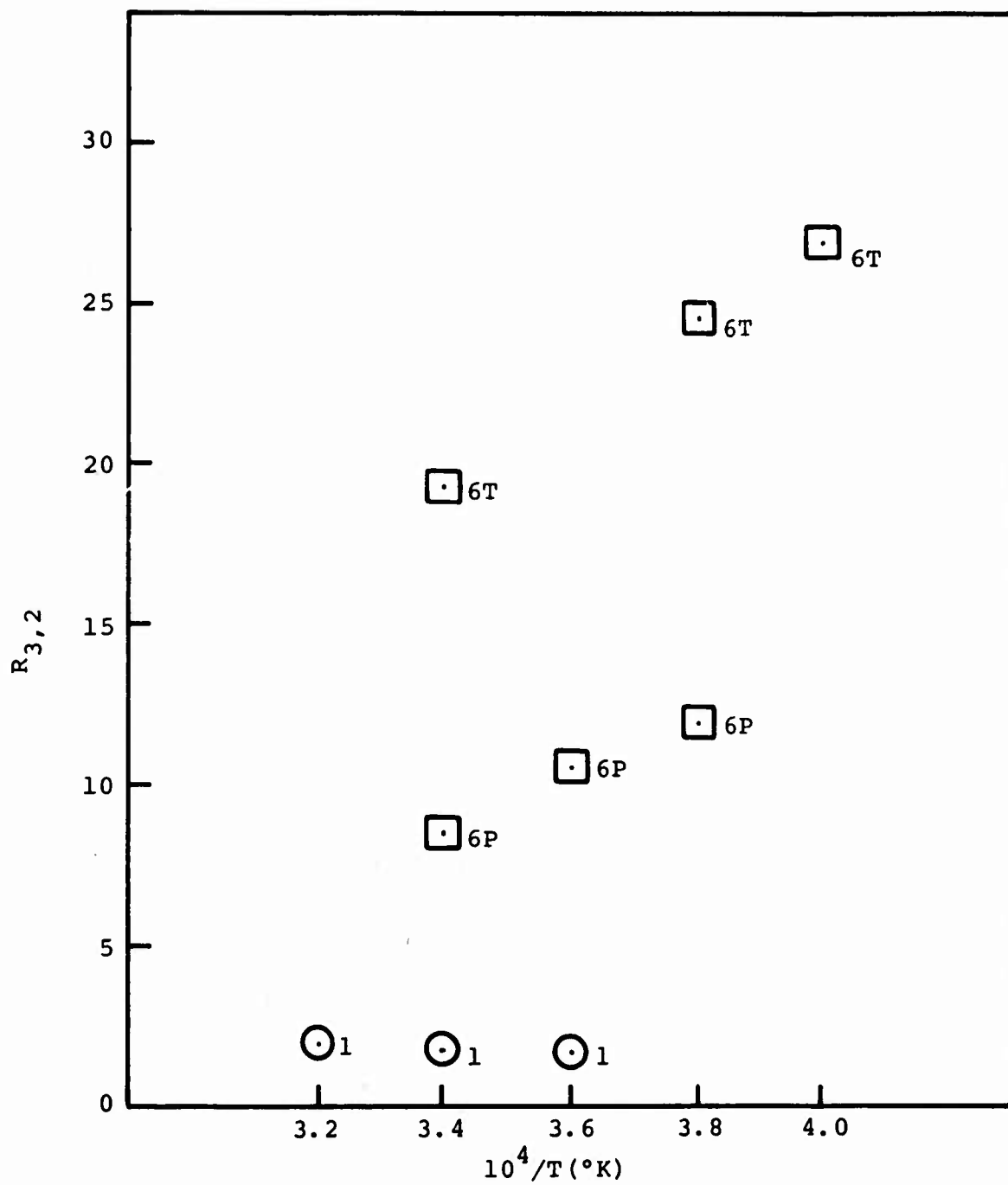
Figure 10. Plot of R_{3,2}^K and R_{3,2}^L vs. \frac{1}{T} for Pyrolytic Graphite. (Free vaporization from c-face)
