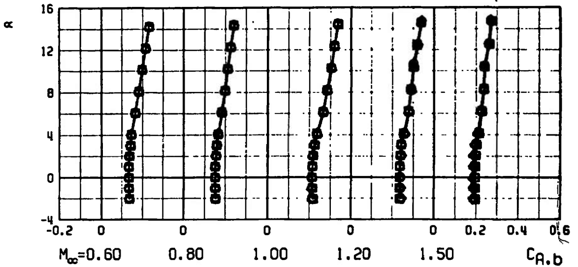
b. Forebody and Base Axial-Force Coefficients Fig. 10 Concluded
