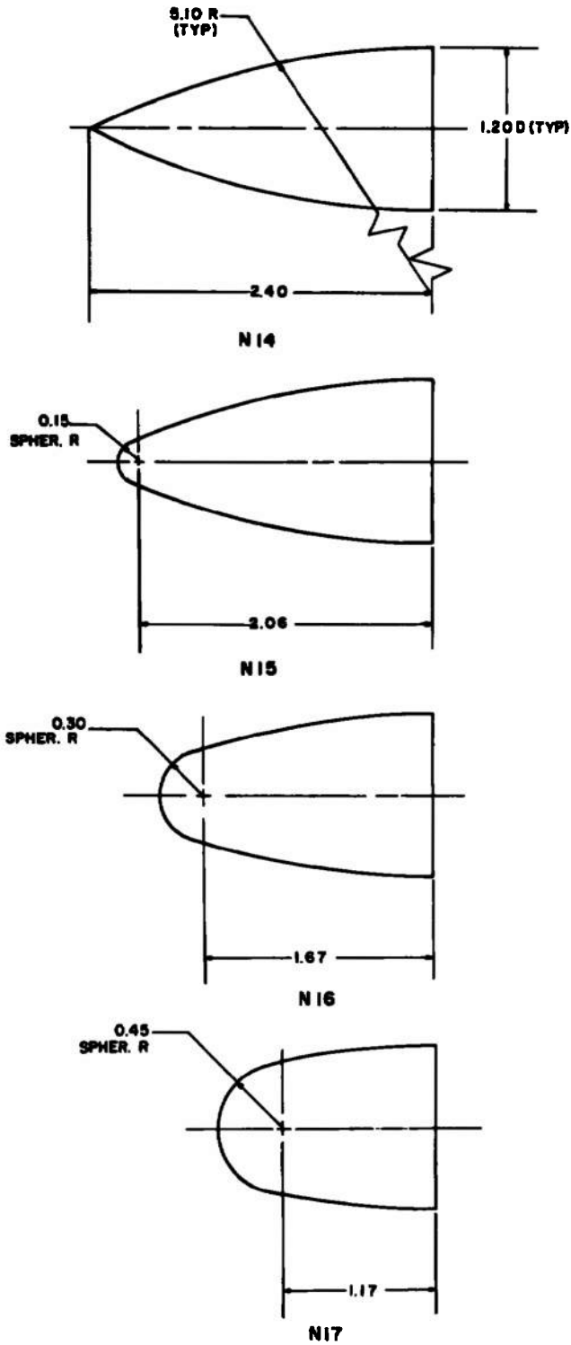
a. 2-cal Tangent Ogive Noses Fig. 4 Dimensional Sketches of Model Components
