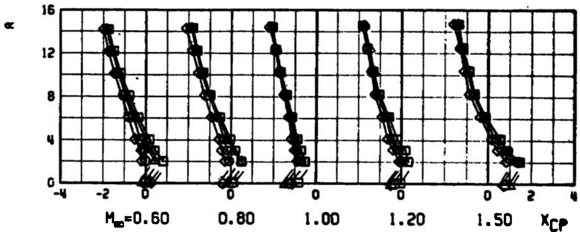
a. Normal-Force Coefficient and Center-of-Pressure Location Fig. 9 Aerodynamic Coefficients of 3-cal Noses on 9-cal Midbody
