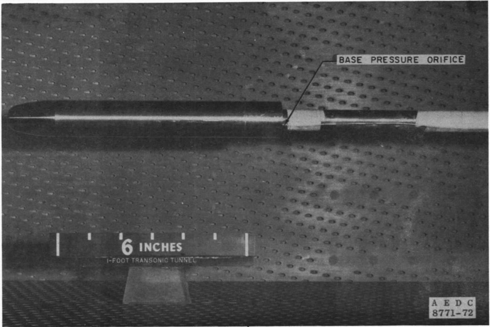
a. N17 M5 A17 Fig. 2 Installation Photographs
