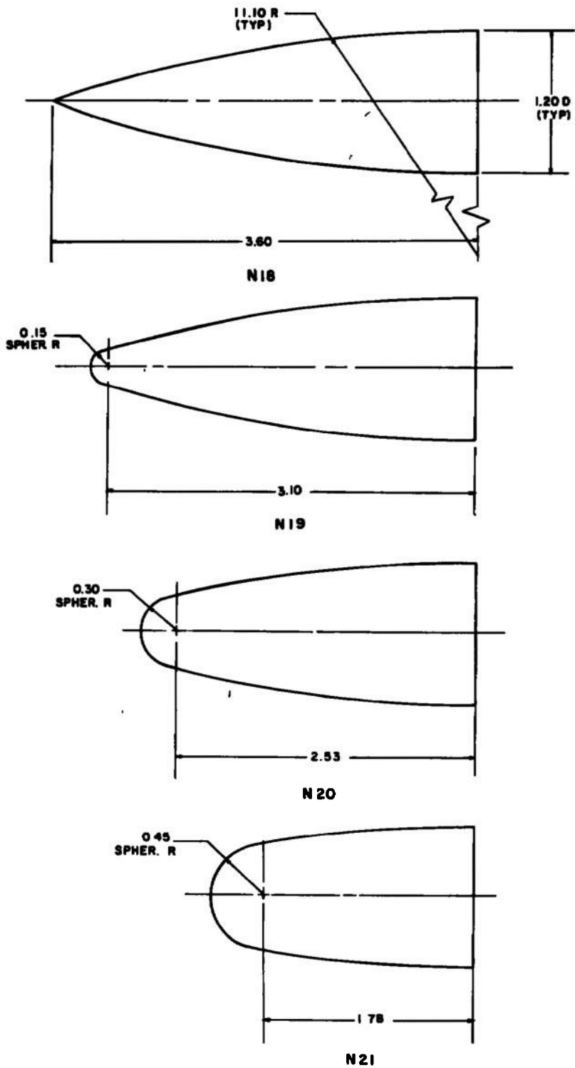
b. 3-cal Tangent Ogive Noses Fig. 4 Continued
