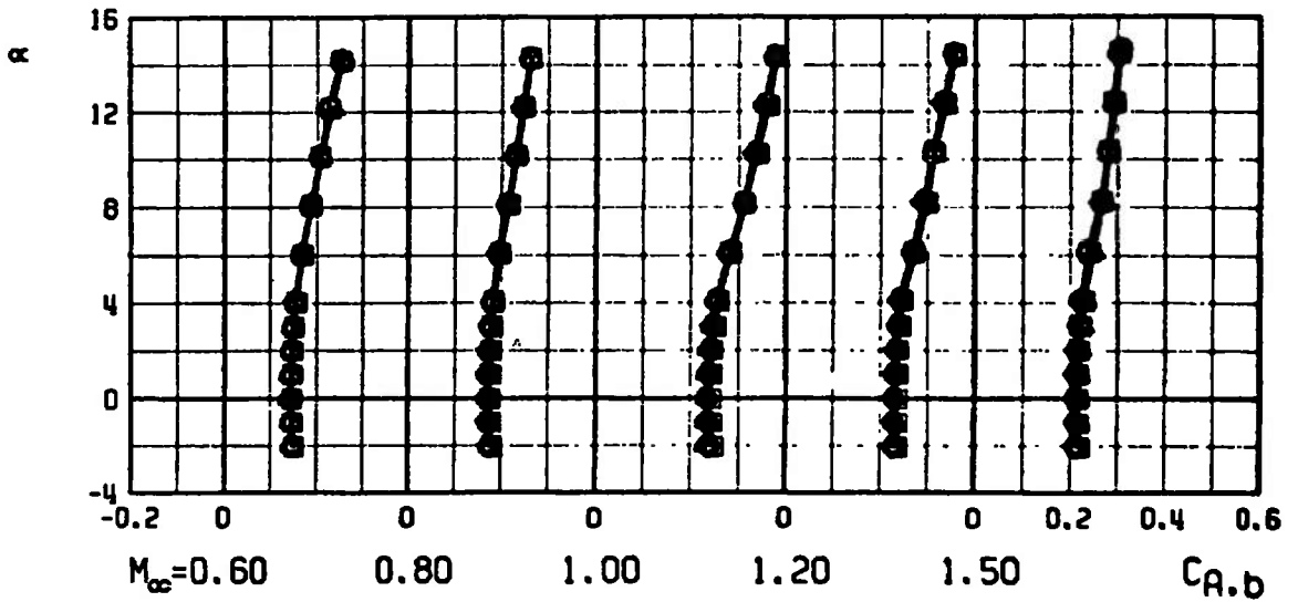
b. Forebody and Base Axial-Force Coefficients Fig. 6 Concluded
