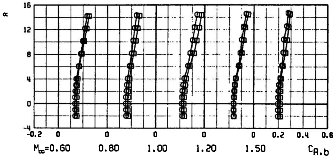
b. Forebody and Base Axial-Force Coefficients, Zero Bluntness Ratio Fig. 14 Continued
