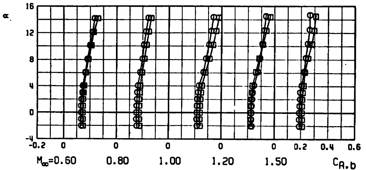
d. Forebody and Base Axial-Force Coefficient, 0.50 Bluntness Ratio Fig. 13 Concluded
