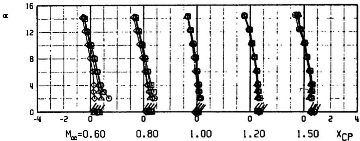
a. Normal-Force Coefficient and Center-of-Pressure Location Fig. 5 Aerodynamic Coefficients of 2-cal Noses on 5-cal Midbody
