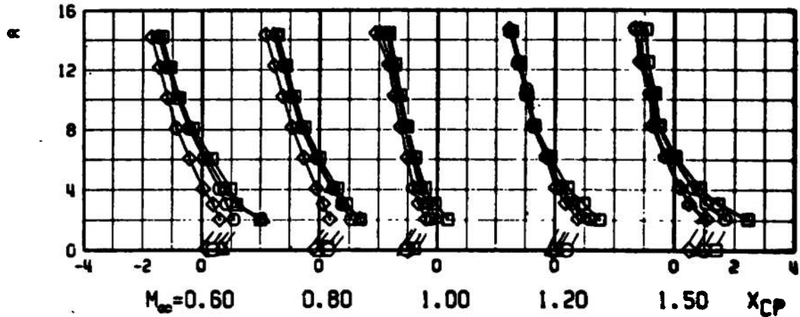
a. Normal-Force Coefficient and Center-of-Pressure Location Fig. 10 Aerodynamic Coefficients of 4-cal Noses on 9-cal Midbody
