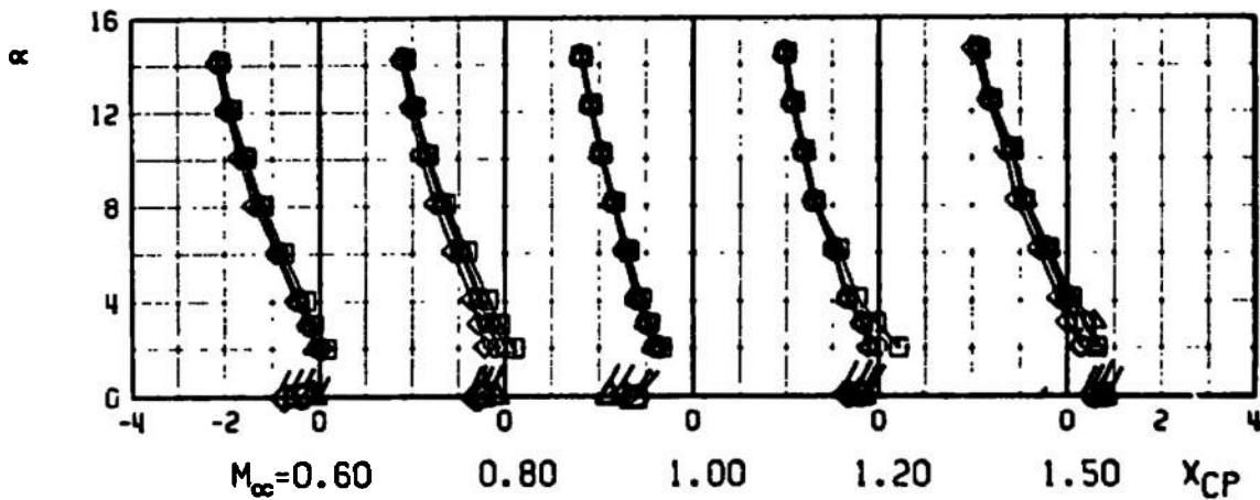
a. Normal-Force Coefficient and Center-of-Pressure Location Fig. 8 Aerodynamic Coefficients of 2-cal Noses on 9-cal Midbody
