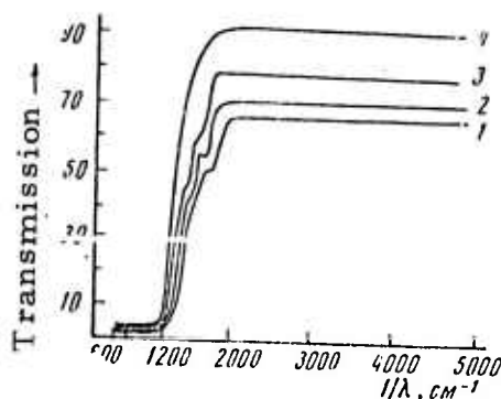
Fig. 1. IR transmission curves of 1 mm thick, spectral grade LiF samples after explosive processing. 1 - 30-50 \mu , 2 - 10-15 \mu , and 3 - 30-50 \mu , after two consecutive explosive moldings; 4 - original LiF single crystal.
