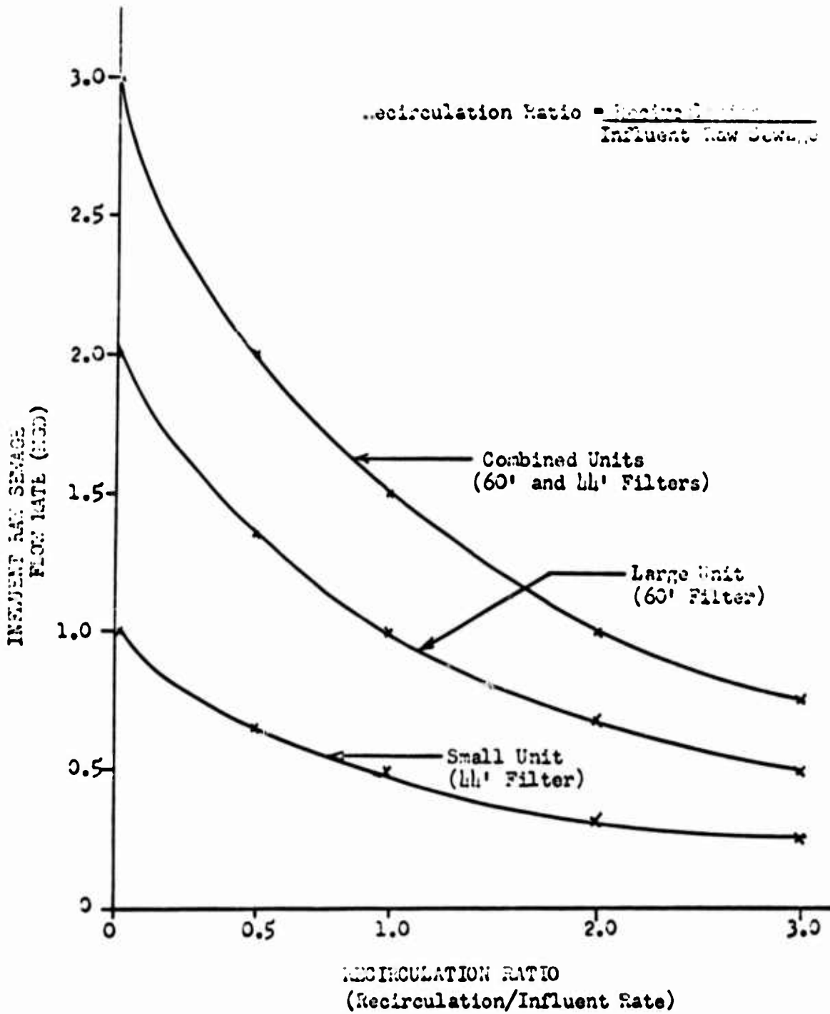
Figure 7 Maximum Allowable Recirculation Ratios
