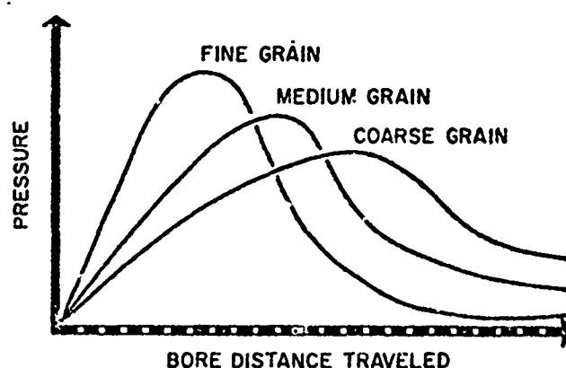
Figure 2. Pressure-travel curve illustrating the inverse relationship of grain size to quickness.
