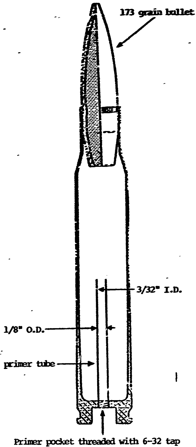
Figure 5. Construction of the forward primed cartridge case.
