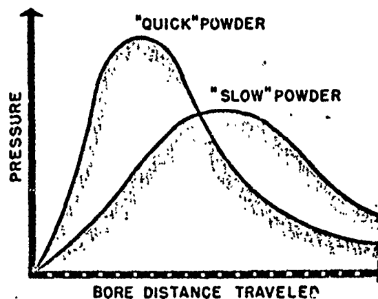
Figure 1. Characteristic pressure curves with weight of charge as a constant.
