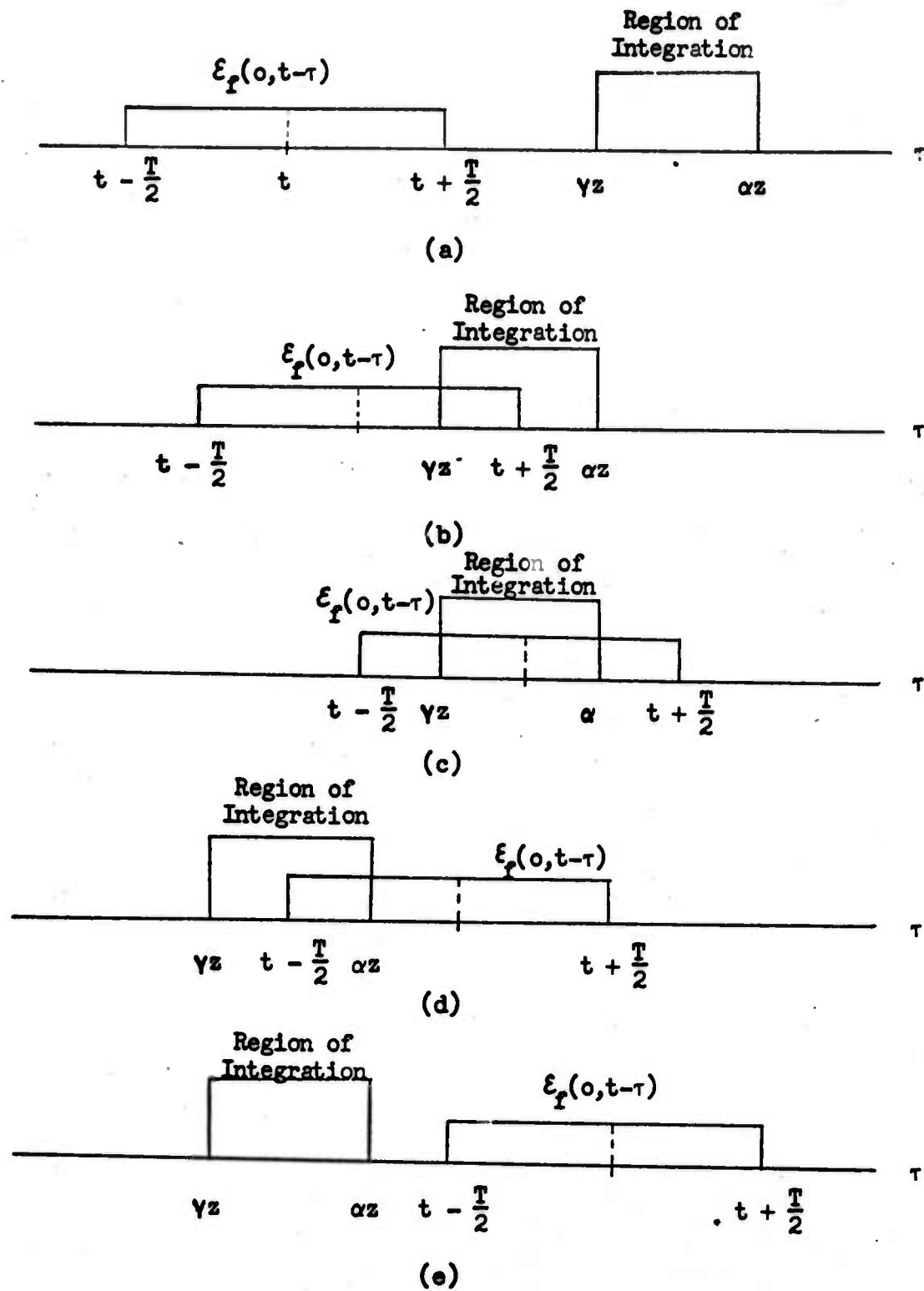
FIGURE A-IV. Convolution Integral Limits Relationship.
