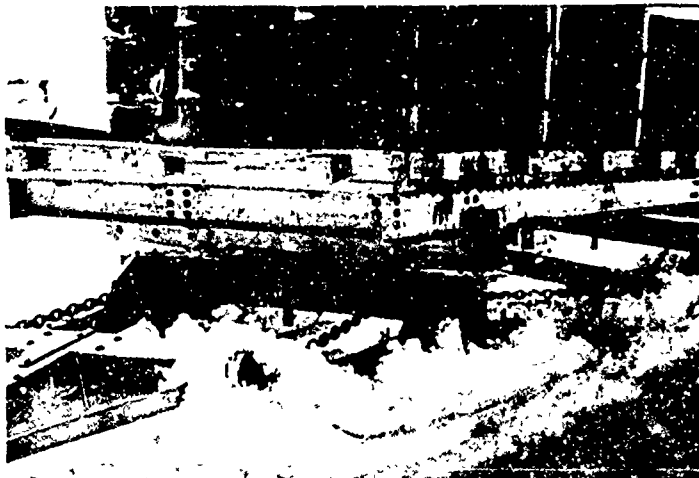
Figure 20. Snow frozen to runner.
