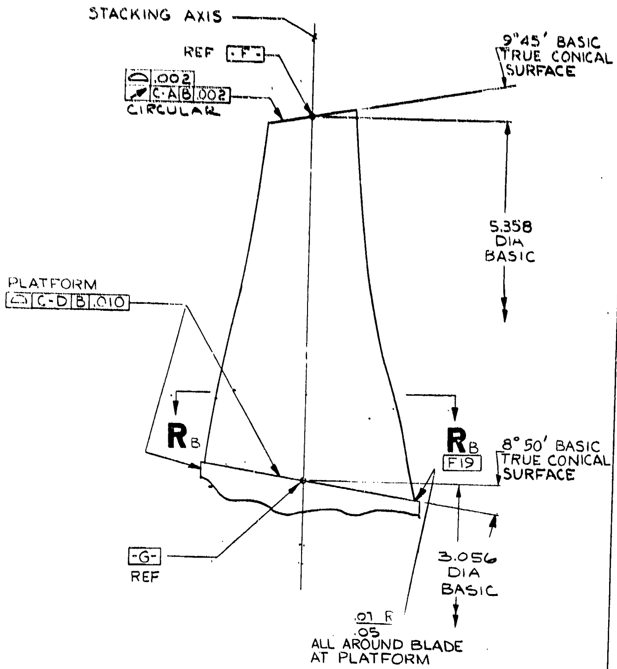
Figure 224. Axial Turbine.
