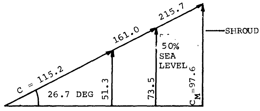
(b) REACTOR EXIT VELOCITY TRIANGLE
