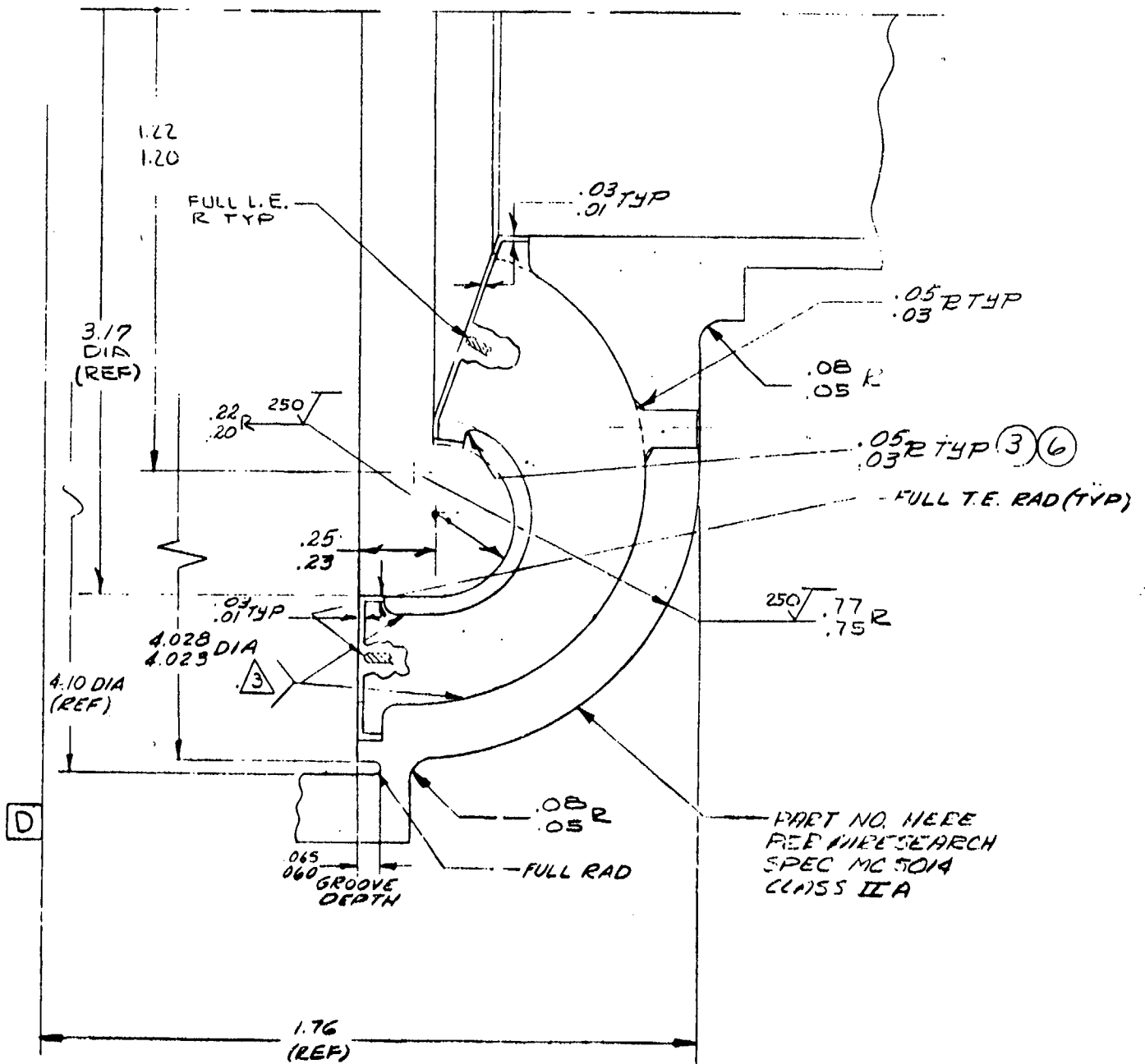
VIEW C SCALE 4/1
