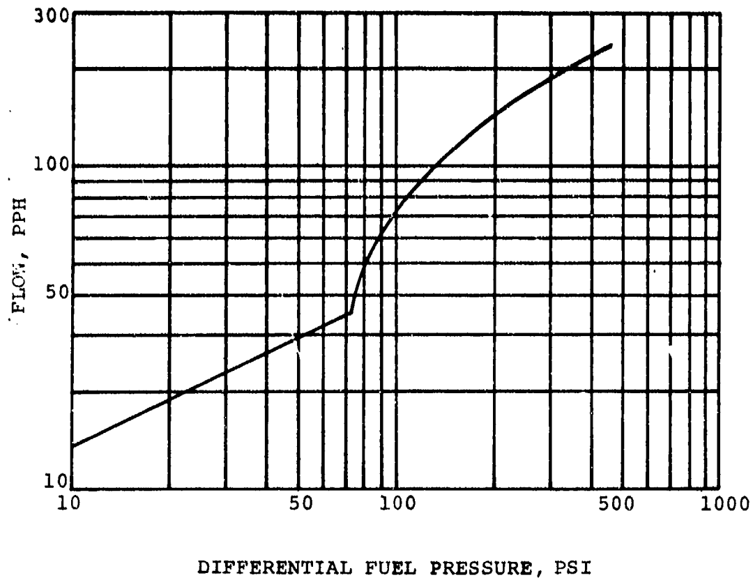
Figure 67. Fuel System Flow Calibration.
