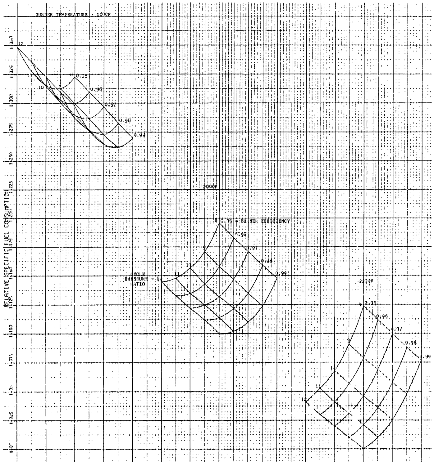
Figure 18. Burner Efficiency Parametric Data.
