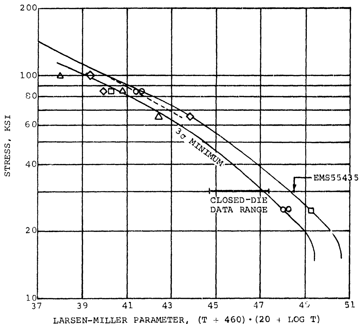
Figure 134. AF2-1DA Stress-Rupture Curve From AFML-TR-69-25, With AiResearch Data.
