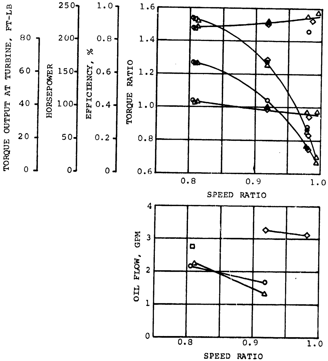
Figure 158. Steady-State Torque Converter Performance.
