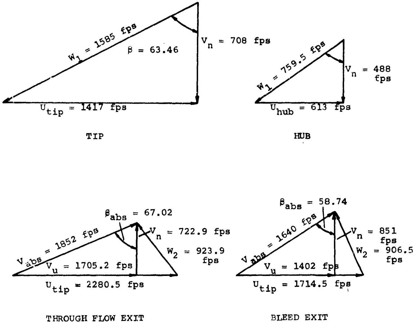
Figure 38. Centrifugal Compressor Vector Triangles of Inducer Leading Edge.
