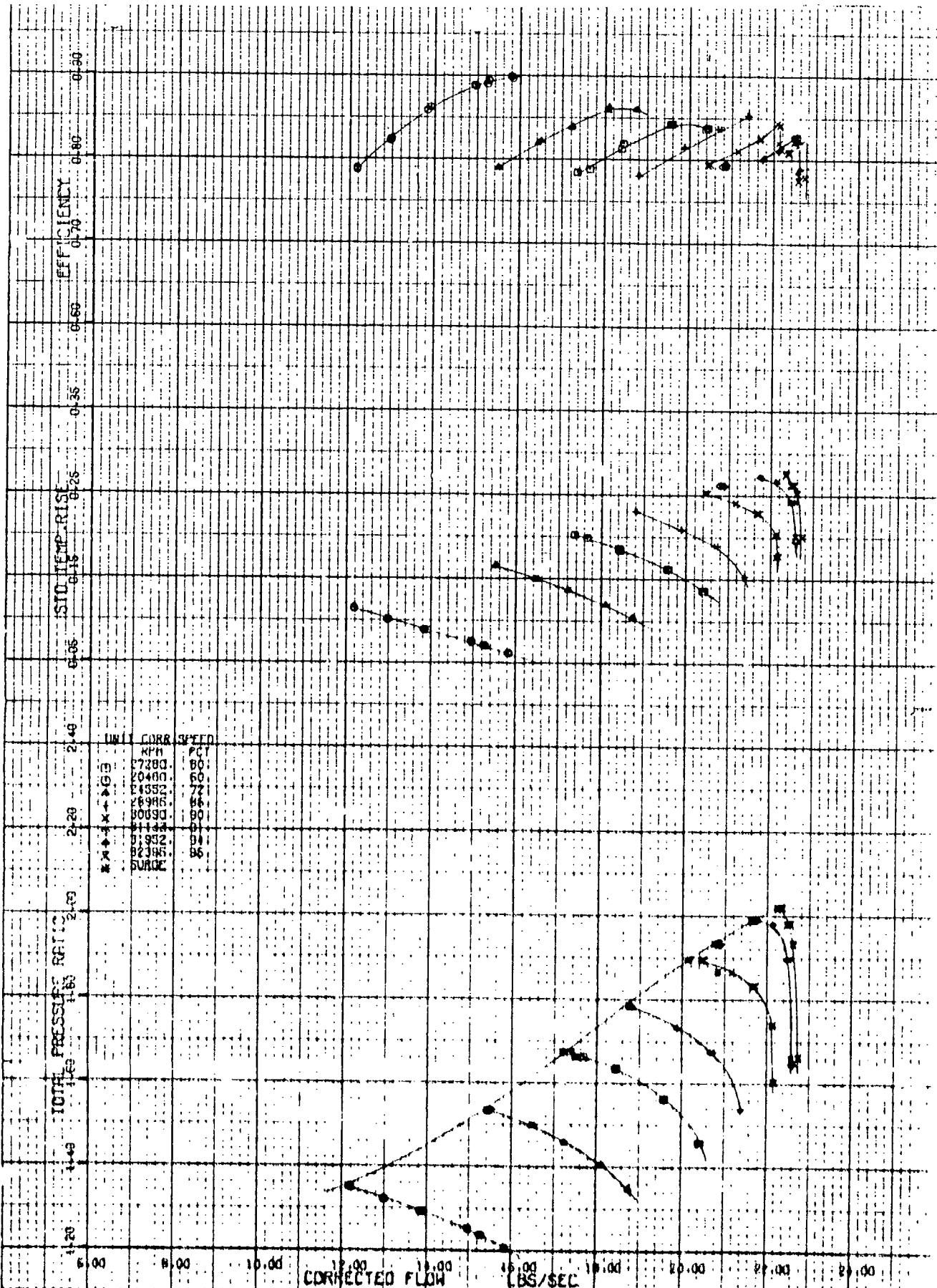
Figure 24. Axial - 2 Compressor Rotor Performance Map.
