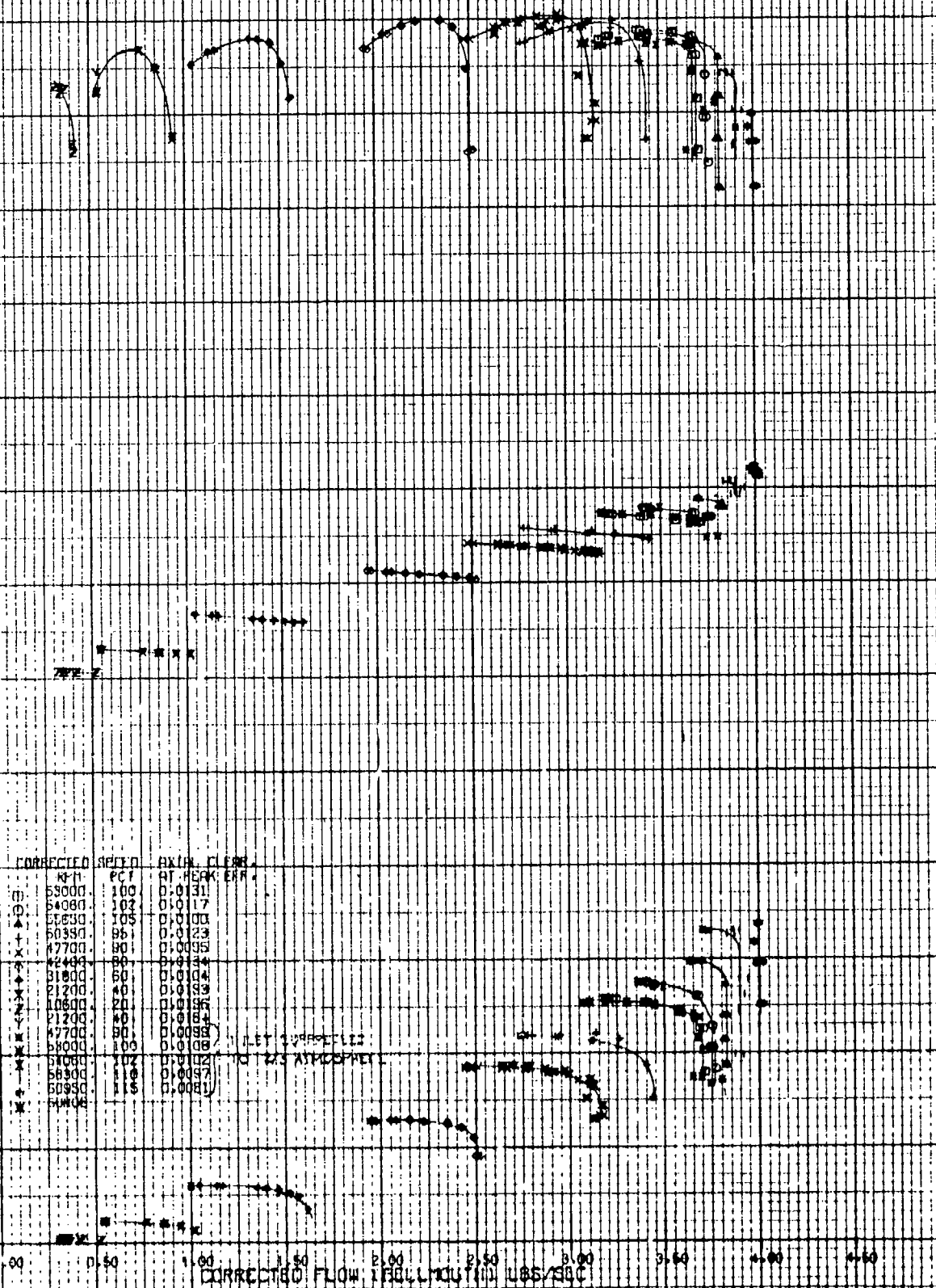
Figure 40. Centrifugal Compressor Performance Map.
