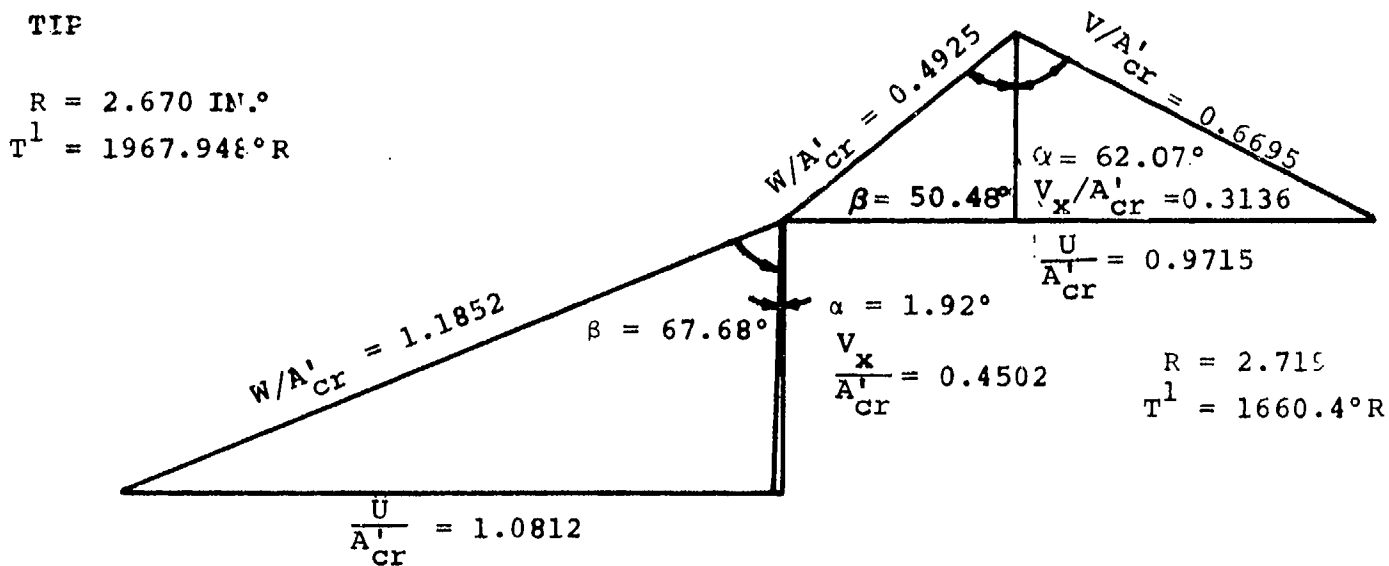
Figure 79. Axial Turbine Vector Diagrams
