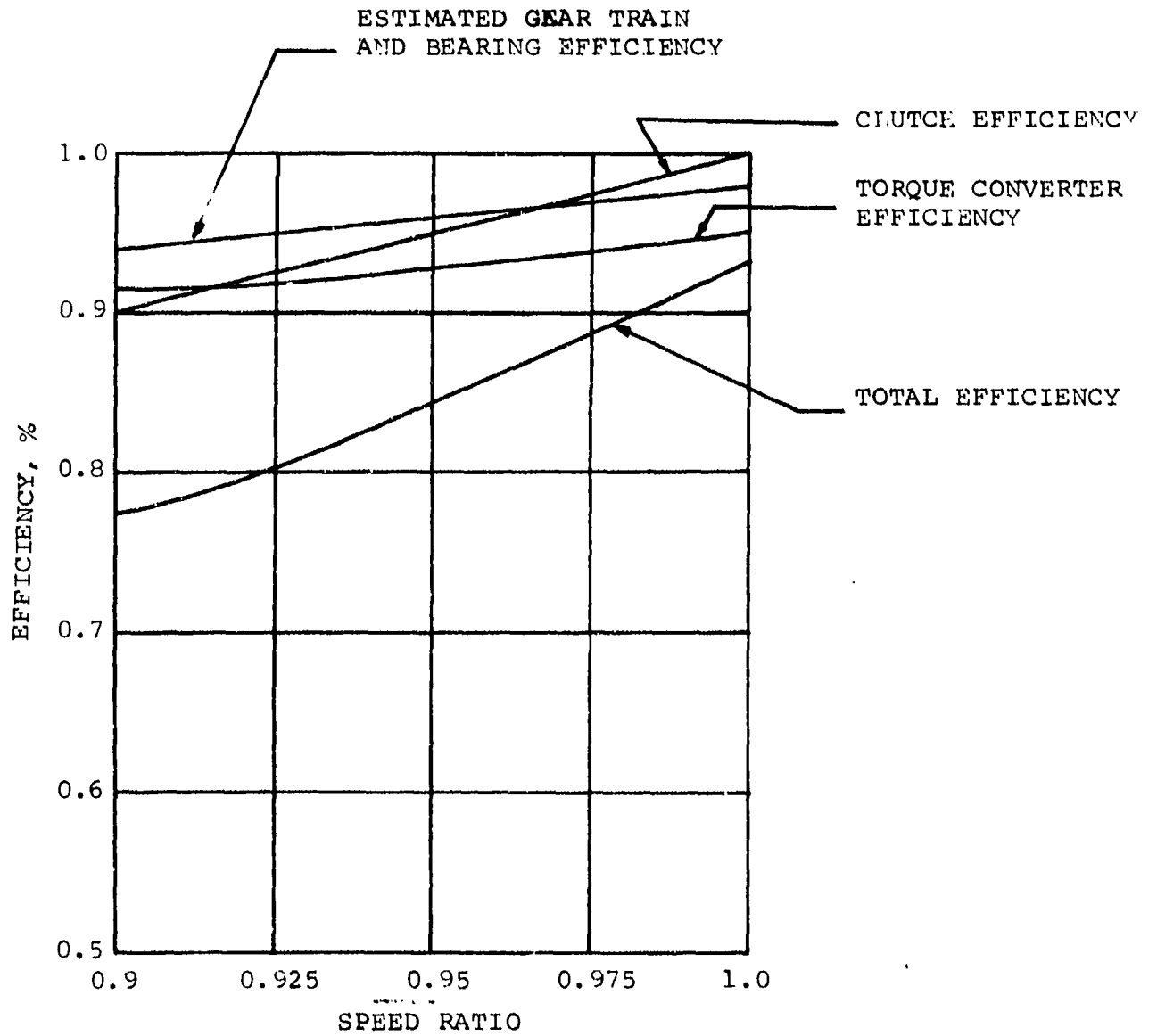
Figure 156. Estimated Lockup Torque Converter Efficiency.
