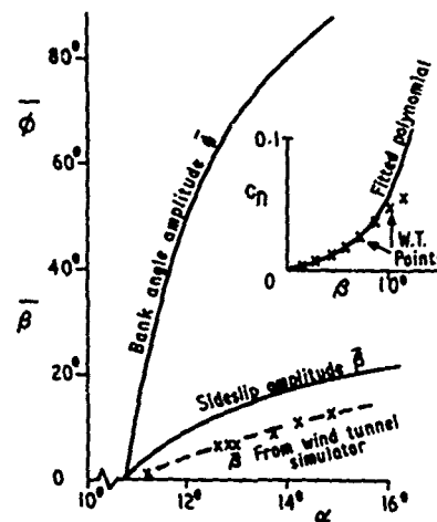
FIG. 7 RESULTS OF CALCULATION OF LIMIT CYCLE AMPLITUDE \beta AND \phi OF THE HP115 DUTCH ROLL AT HIGH INCIDENCE (FROM REF. 16)
