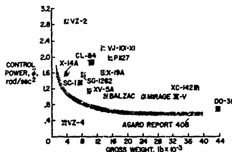
Fig. 5. Comparison of hover roll control values with AGARD 408 requirement.
