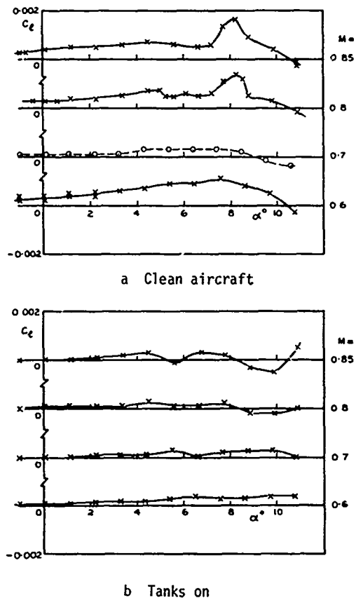
Fig.13 Rolling moment coefficients for aircraft B ( \beta = 0 )
