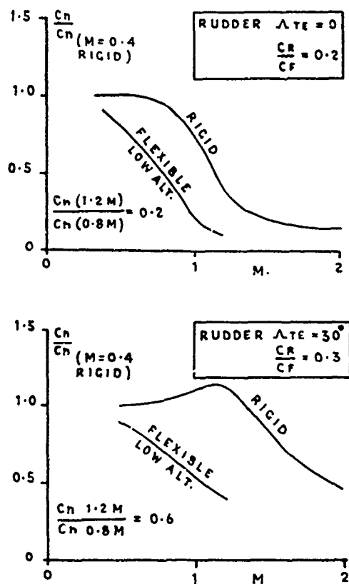
FIG. 26. TRANSONIC CHANGE IN RUDDER EFFECTIVENESS: EFFECT OF FIN & RUDDER GEOMETRY
