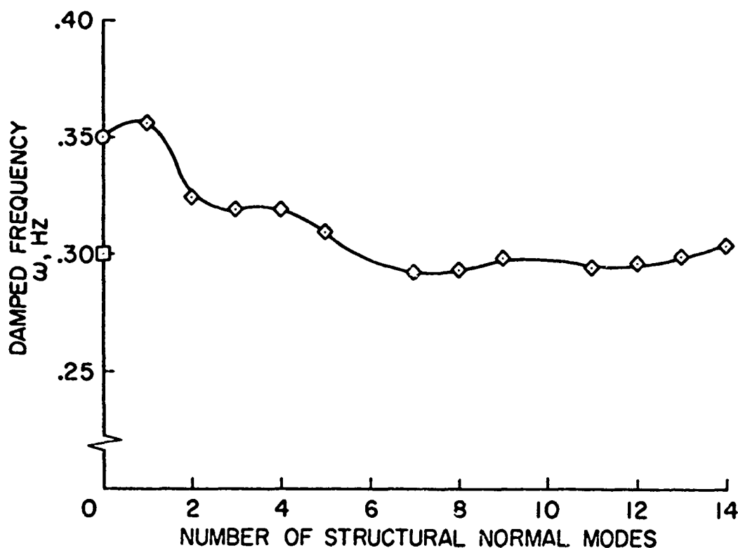
Fig. 8 Effect of number of normal modes on short-period damping and frequency, Boeing 707-320B.
