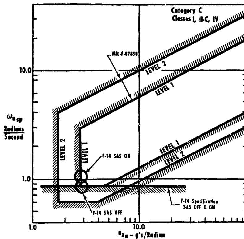
Figure 19 - Short Period Frequency Requirement
