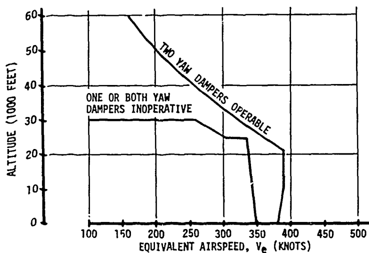
Figure 1 727 Operating Restrictions With One Yaw Damper Failed
