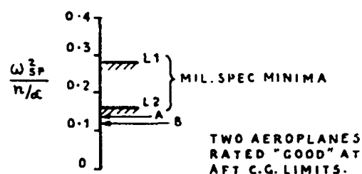
FIG. 3 LONGITUDINAL STABILITY REQUIREMENTS (U.S.A.F. MIL. SPEC.)
