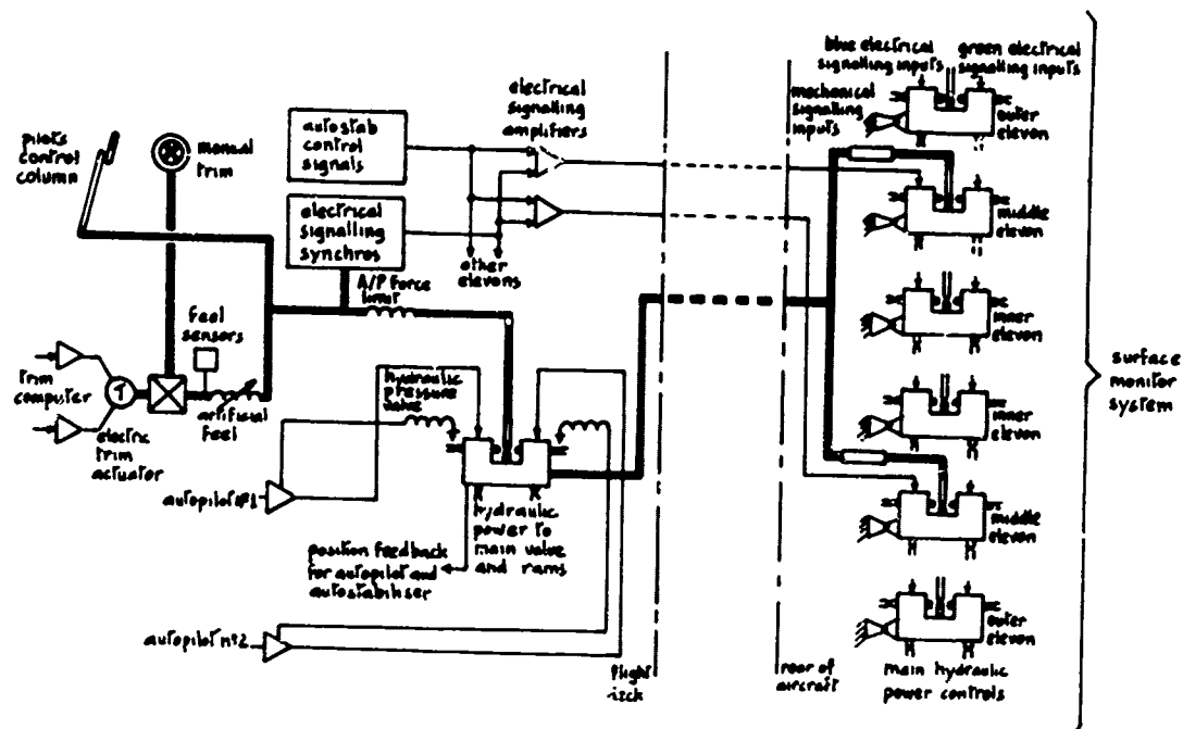
SCHEME SHOWING THE PRINCIPLES OF THE CONCORDE FLYING CONTROL SYSTEM
