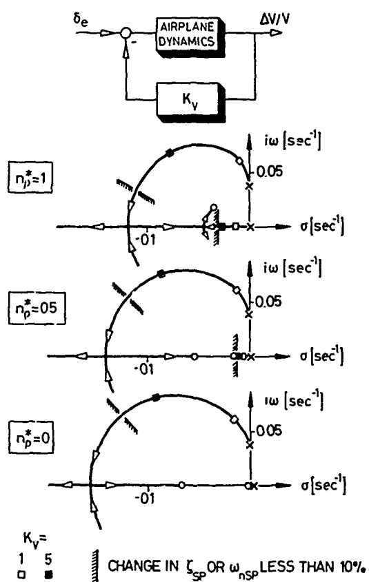
FIG.13: THRUST EFFECTS ON THE STABILIZATION OF THE PHUGOID AND HEIGHT MODE BY SPEED FEEDBACK TO MOMENT
