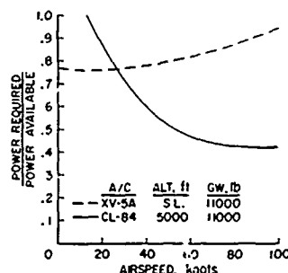
Fig. 2. Comparison of power required curves for the XV-5A and CL-84 aircraft.
