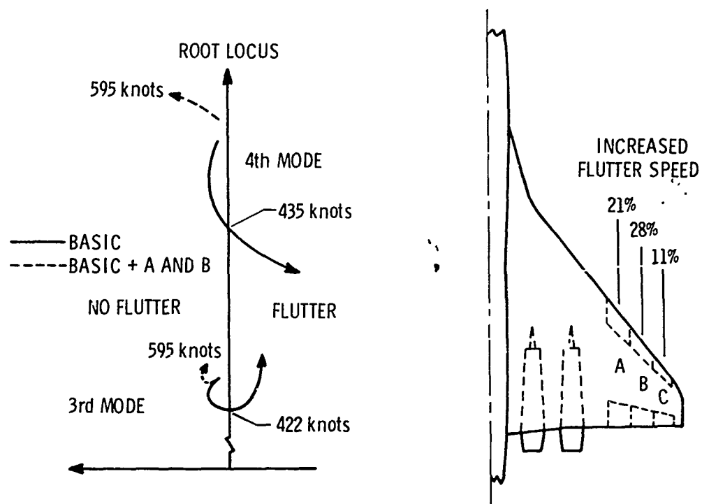
Fig.3 Calculated effectiveness of aerodynamic energy concept flutter suppression systems
