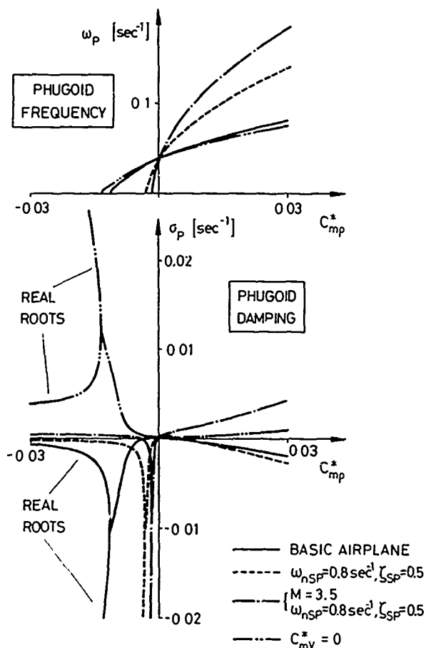
FIG.11: EFFECT OF C_{mp}^* ON THE PHUGOID MODE (PARAMETER: \omega_{nSP} , M , C_{mv}^* )
