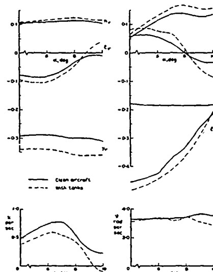
Fig.16 Lateral characteristics of aircraft B ( M = 0.85 )
