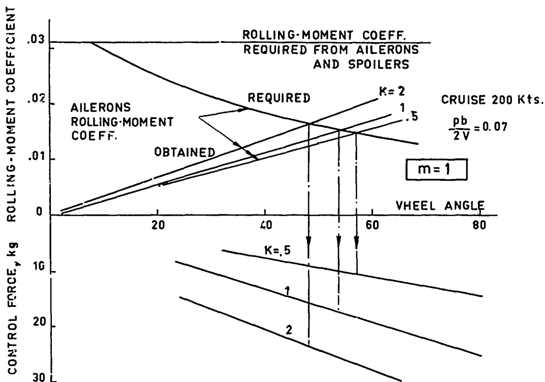
FIG.17- DEFINITION OF AILERON SPRING-TAB CHARACTERISTICS.
