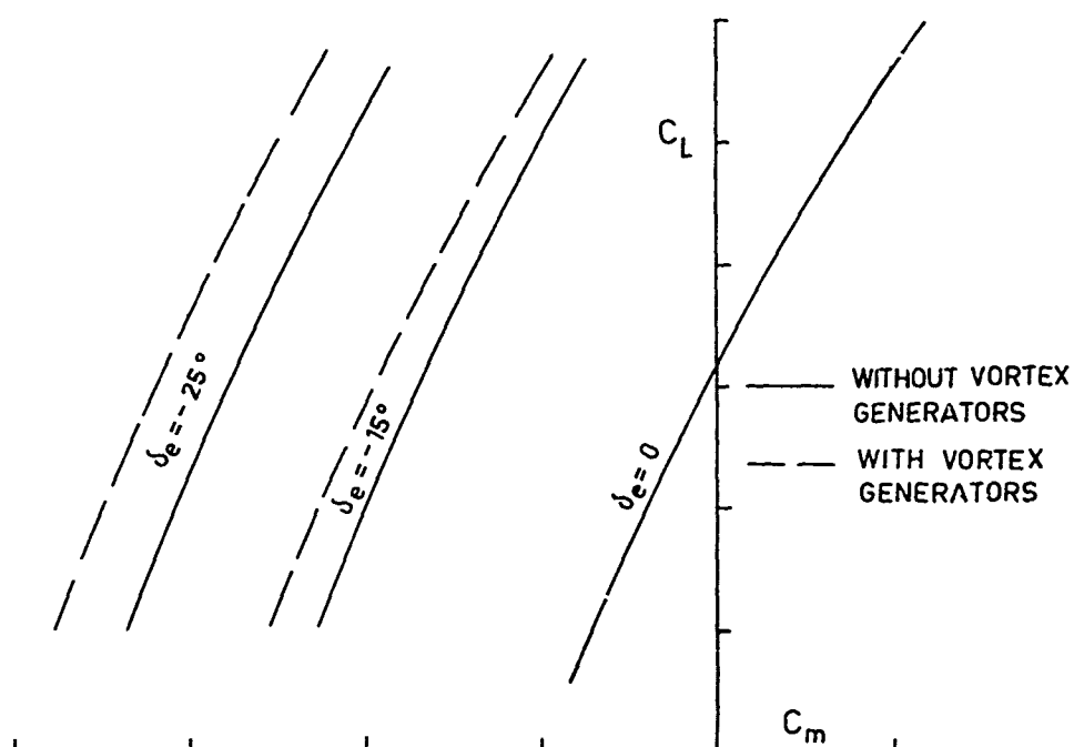
FIG.11 - EFFECT OF VORTEX GENERATORS UNDER TAILPLANE ON ELEVATOR EFFECTIVENESS
