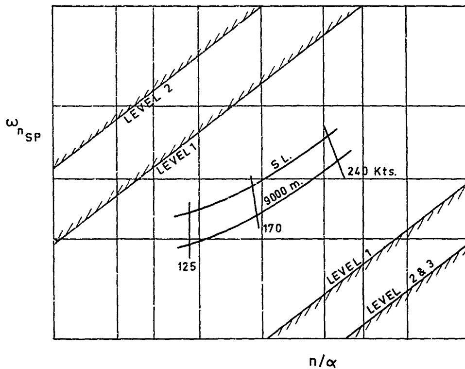
FIG. 2-G.222 SHORT-PERIOD CHARACTERISTICS (CRUISE CONF.-CONTROL FIXED)
