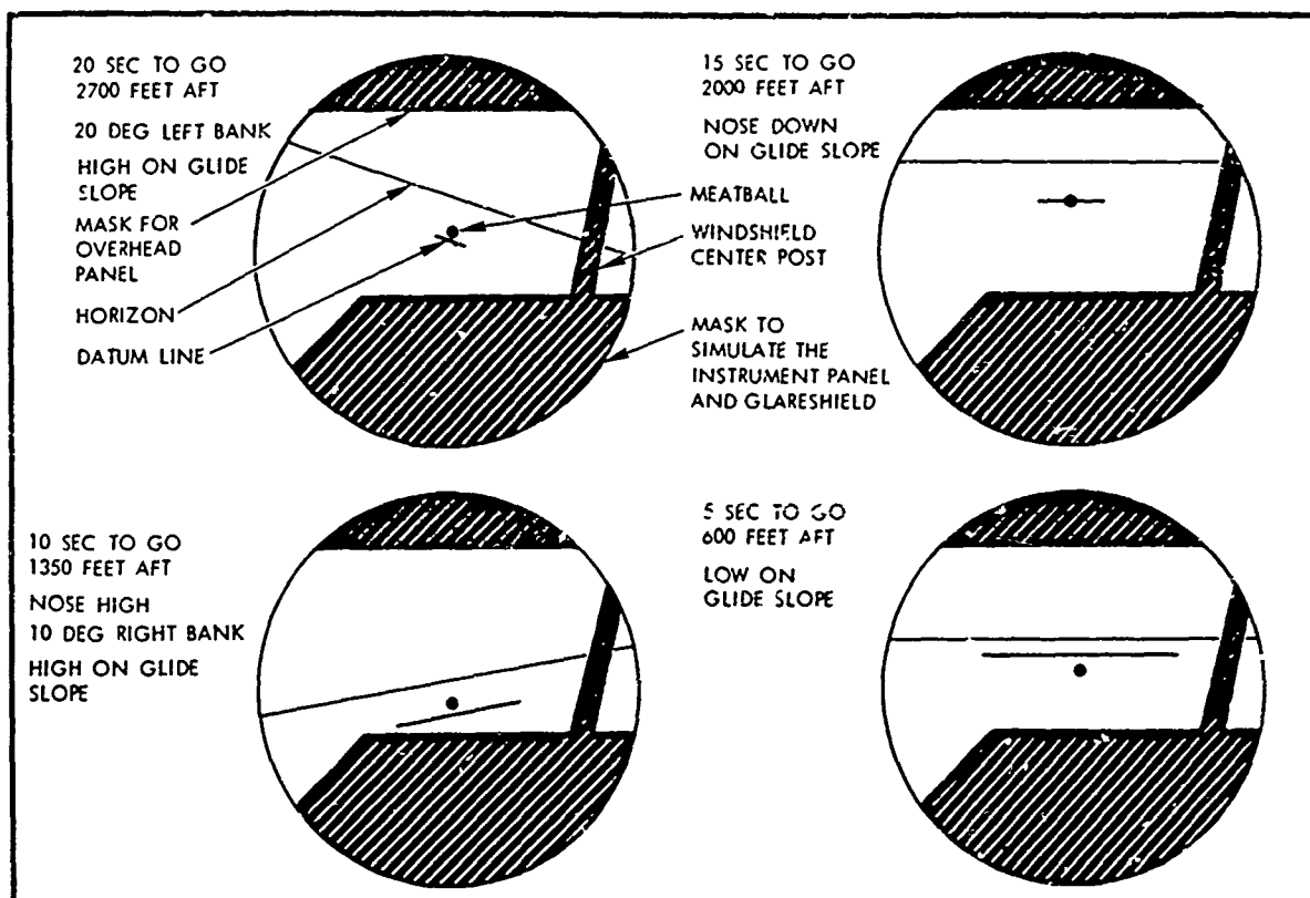
Figure 5 - Lockheed Initial Simulator Display
