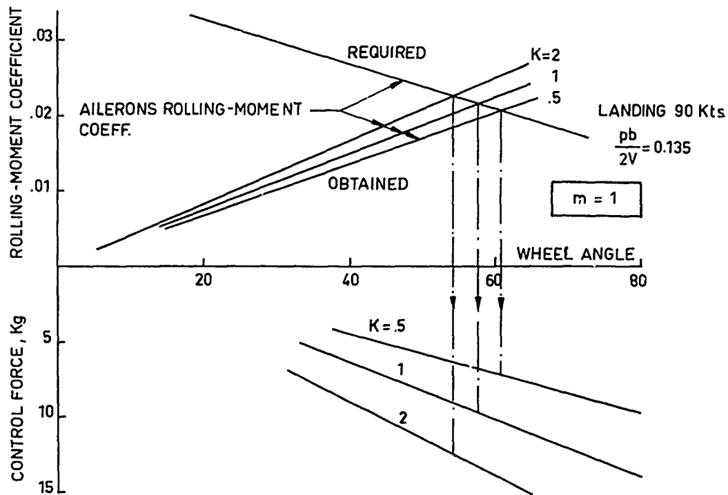
FIG. 19-DEFINITION OF AILERON SPRING-TAB CHARACTERISTICS
