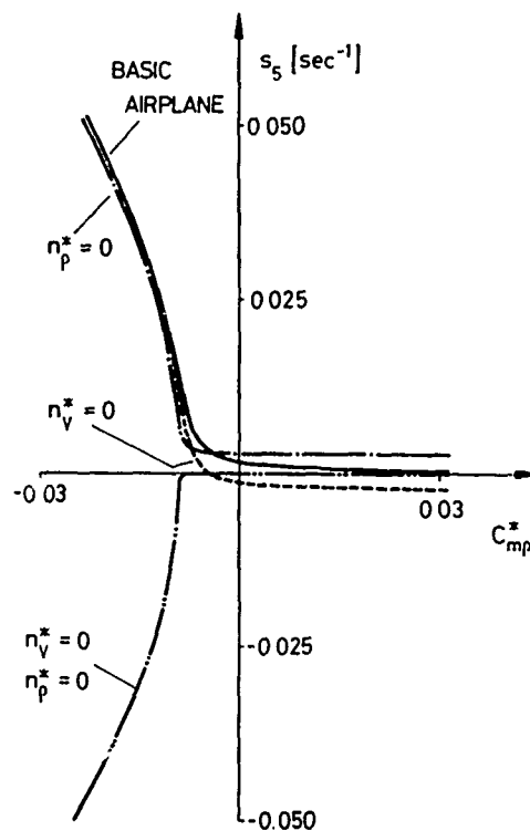
FIG.10: EFFECT OF C_{mp}^* ON THE HEIGHT MODE (PARAMETER: n_p^* , n_v^* )
