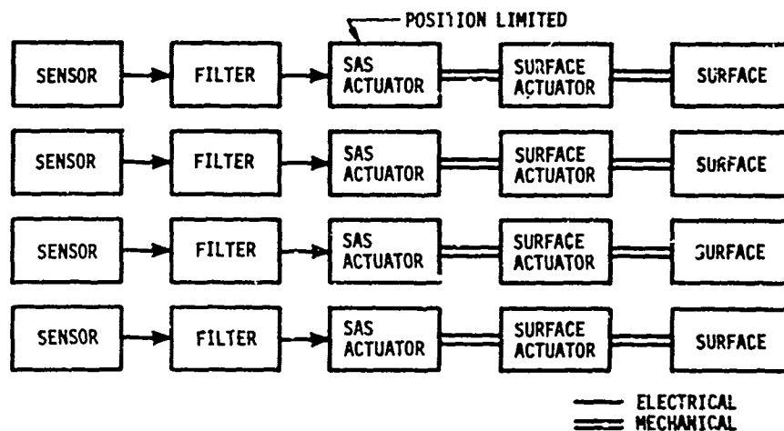
Figure 4 System Mechanization Using Split Control Surfaces
