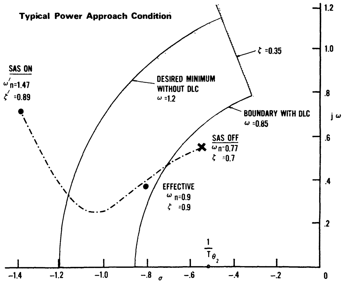
Figure 20 - F-14 Short - Period Dynamics
