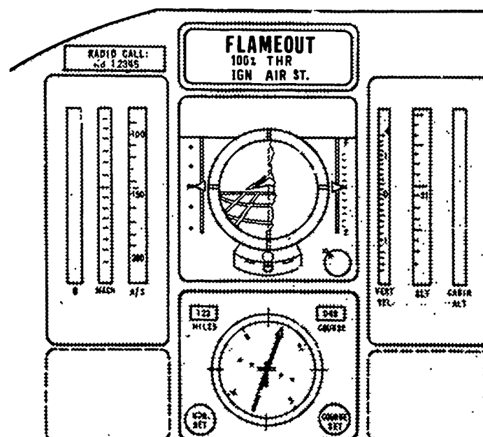
FIG. 2 HOT MESSAGE AND ADVICE PANEL.
