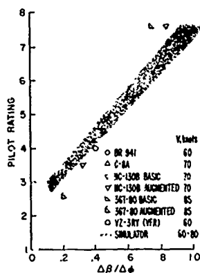
Fig. 7. Relation of turn entry coordination and pilot rating.
