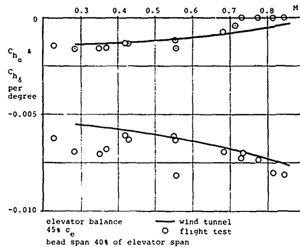
Fig. 8 Hinge moment characteristics of F28 elevator
