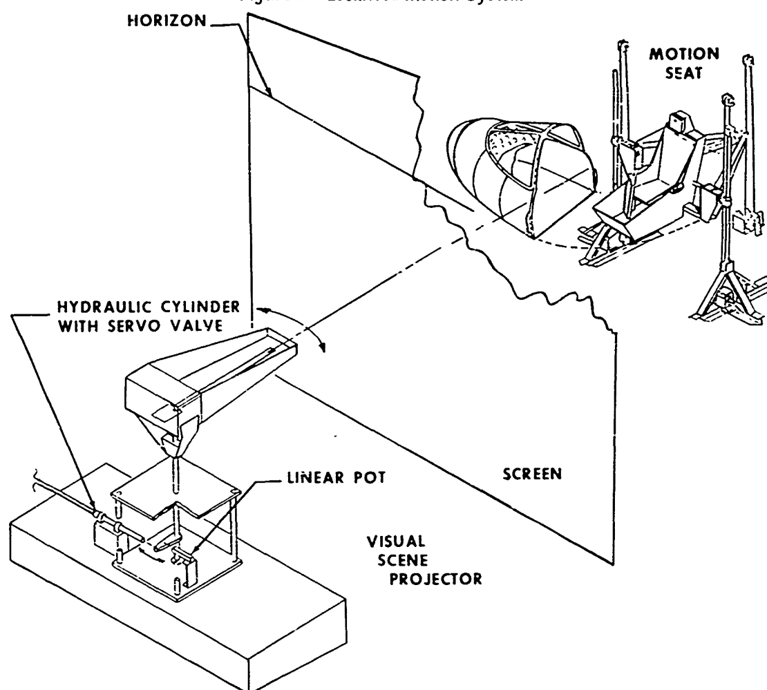
Figure 8 - Grumman Simulation
