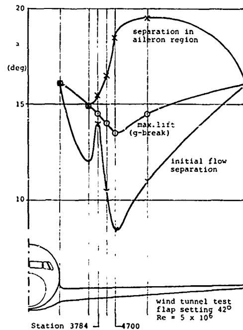
Fig. 13 Effect of span wise fence location on progression of flow separation
