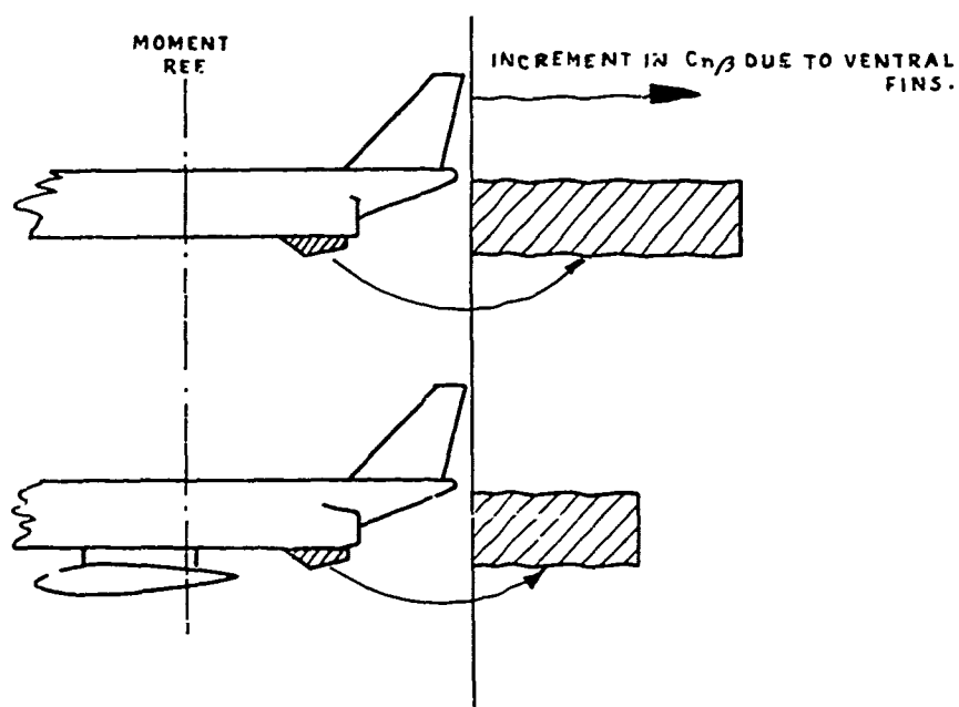
FIG. 22. COMPARISON OF SINGLE AND TWIN FIN CONTRIBUTIONS TO DIRECTIONAL STABILITY.
