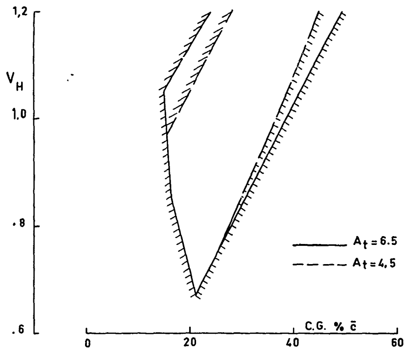
FIG. 4- INFLUENCE OF HORIZONTAL TAIL ASPECT RATIO ON CENTER OF GRAVITY LIMITS
