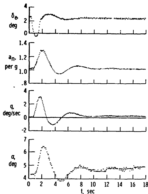
Figure 10. Typical XB-70-1 flight data of pull-up and release maneuver M = 0.75 , h_p = 7,650 m (25,100 ft).
