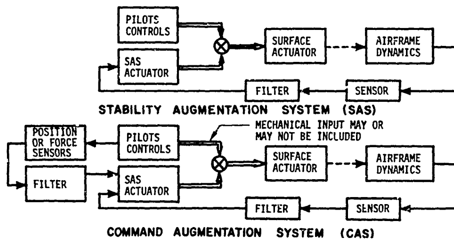
Figure 8 Stability Augmentation And Command Augmentation Systems
