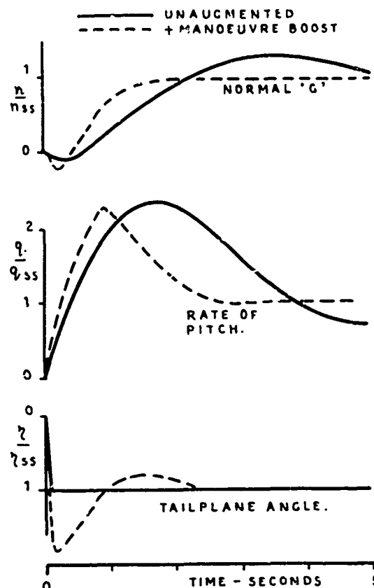
FIG. 4. EFFECT OF MANOEUVRE BOOST ON TRANSIENT RESPONSE TO TAILPLANE.
