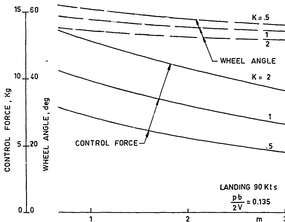
FIG. 22- SYNTESIS OF AILERON SPRING-TAB TYPICAL CHARACTERISTICS
