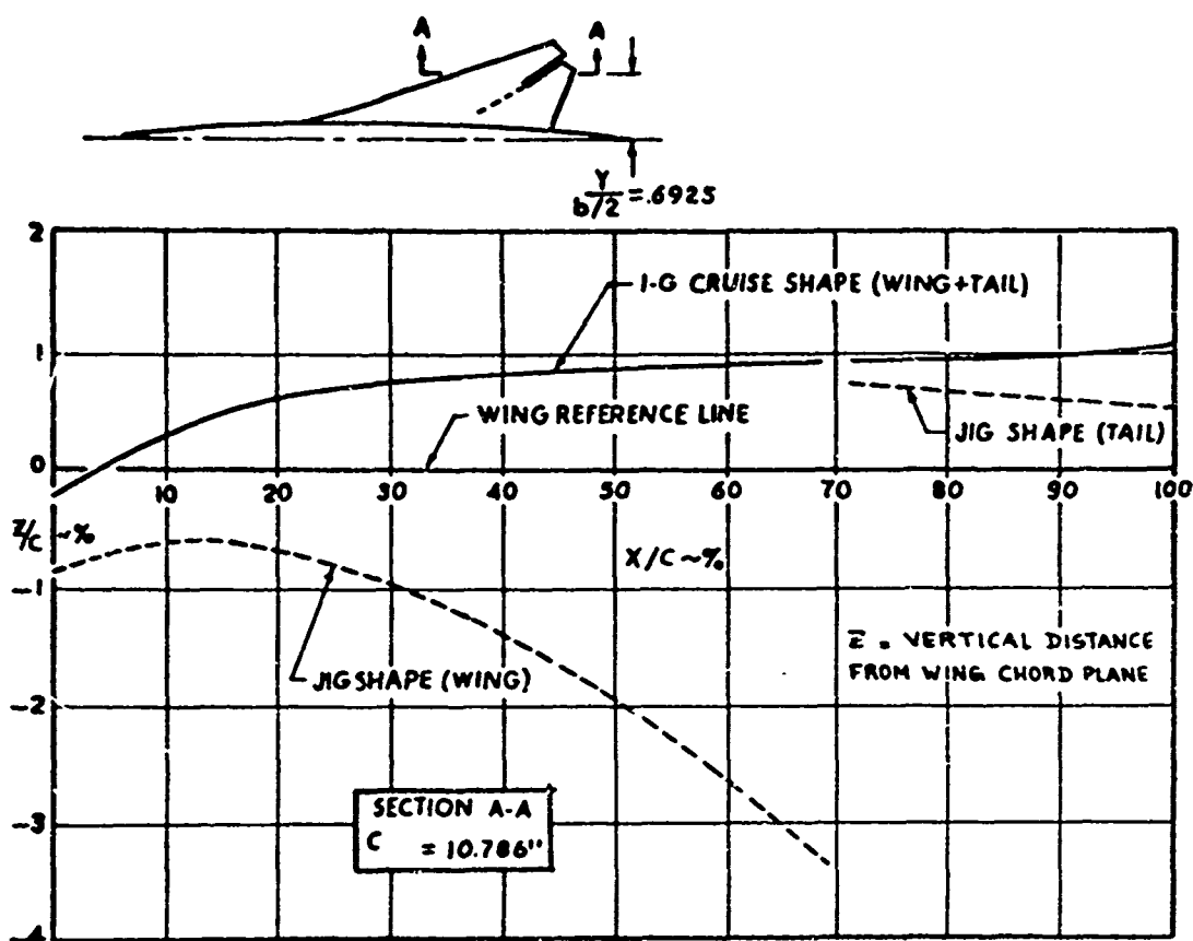
FIGURE 9 EXAMPLE OF JIG SHAPE AND CRUISE SHAPE
