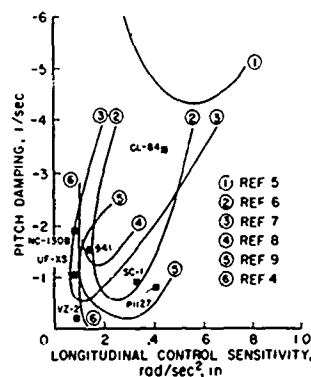
Fig. 1. Comparison of 3.5 pilot rating boundaries from piloted simulator and flight tests.
