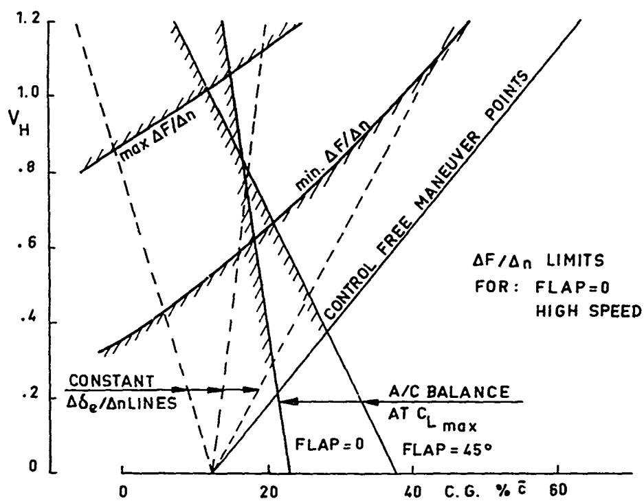
FIG. 3- CENTER OF GRAVITY LIMITS VERSUS HORIZONTAL TAIL VOLUME
