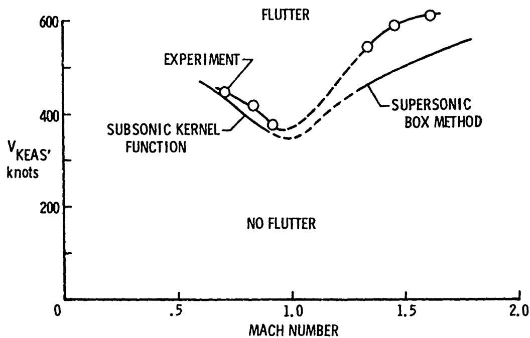
Fig.2 Comparison of measured and calculated SST model flutter boundaries
