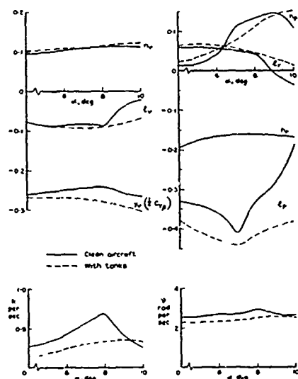
Fig.15 Lateral characteristics of aircraft B ( M = 0.6 )
