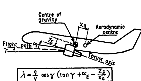
FIG. 9 FACTORS INFLUENCING GLIDE PATH STABILITY IN FLIGHT UNDER SPEED CONSTRAINT
