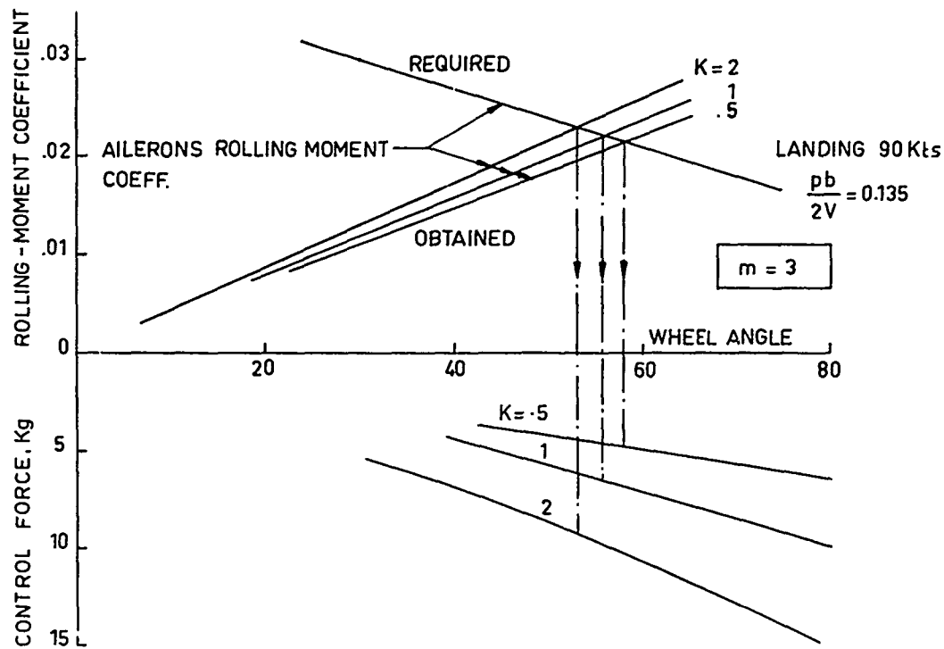
FIG. 20- DEFINITION OF AILERON SPRING -TAB CHARACTERISTICS
