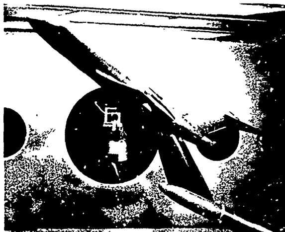
Fig. 10 F28 wind tunnel model at extreme angle of incidence
