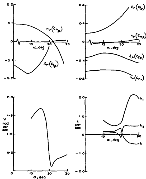
Fig.14 Lateral characteristics of aircraft A
