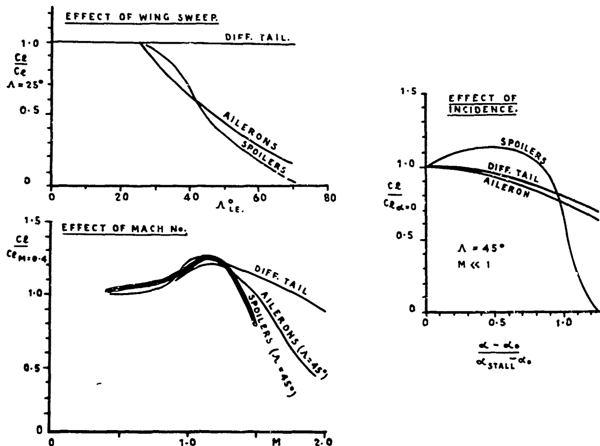
FIG. 12 VARIATION OF CONTROL EFFECTIVENESS WITH SWEEP, MACH NO. AND INCIDENCE FOR ALTERNATIVE ROLL CONTROLS
