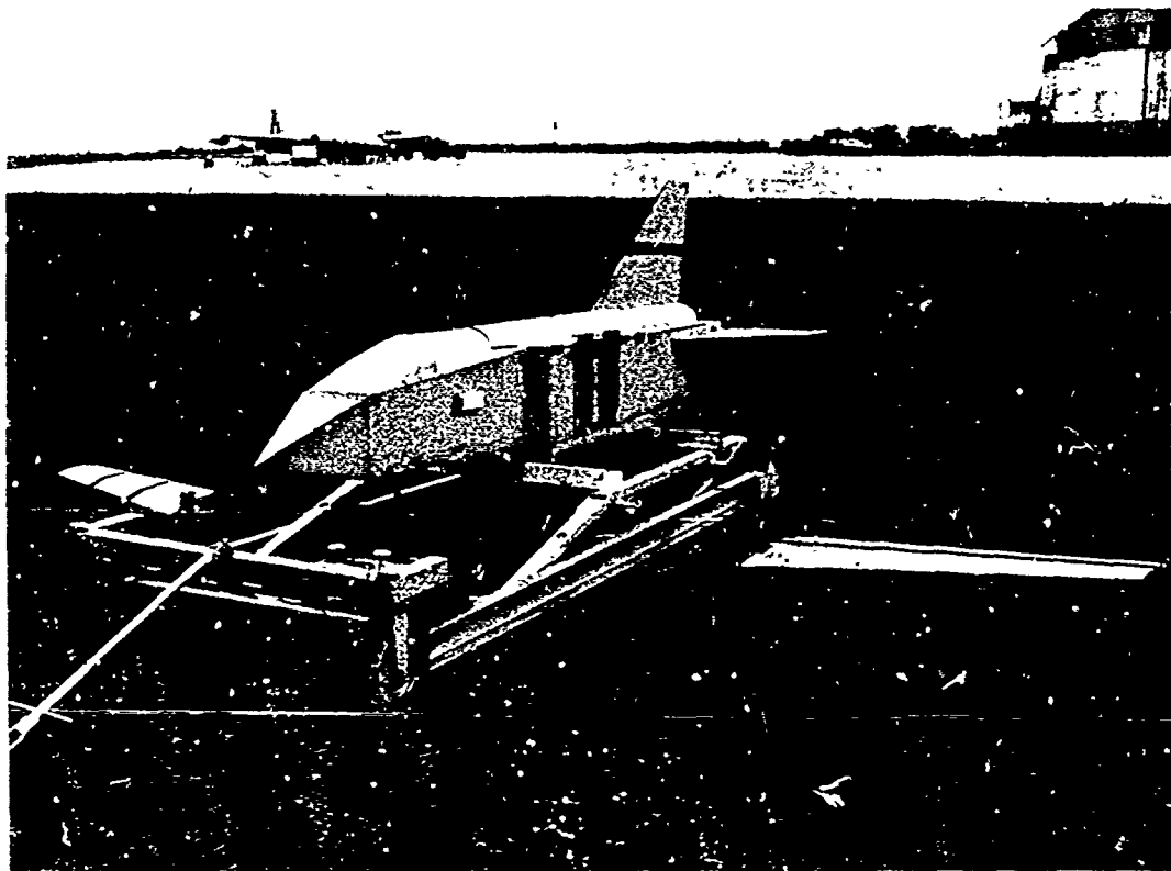
fig. 6 Model handling trolley
