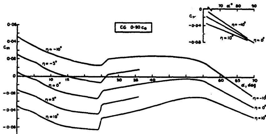
Fig.4 Pitching moment characteristics assumed for the slender-wing aircraft
