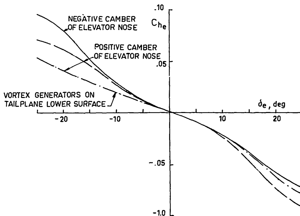
FIG.10 - INFLUENCE OF ELEVATOR NOSE CAMBER AND VORTEX GENERATORS ON HINGE MOMENT BEHAVIOUR
