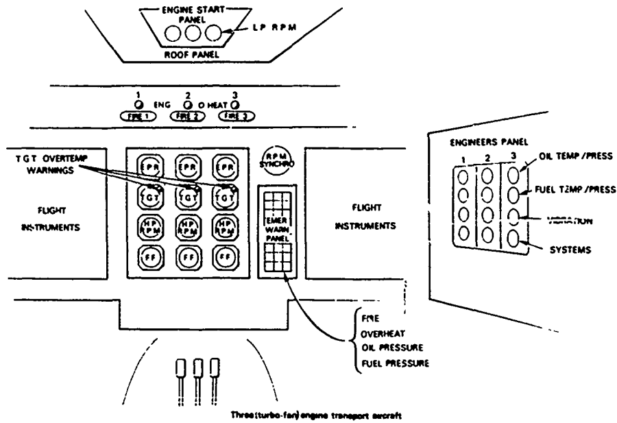
FIG. 3 RECOMMENDED ENGINE INSTRUMENTS PANELS LAYOUT FOR CURRENT AIRCRAFT.
