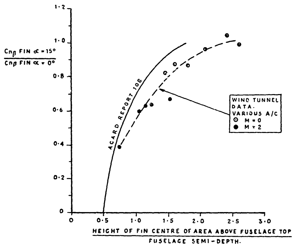
FIG. 20 EFFECTS OF ANGLE OF ATTACK ON FIN CONTRIBUTION TO DIRECTIONAL STABILITY
