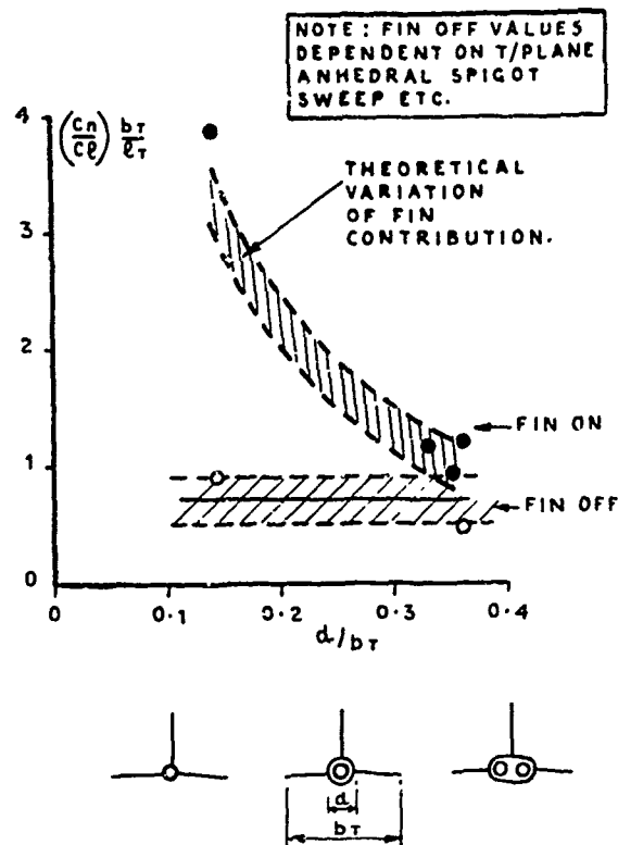
FIG. 15. EFFECT OF AFTERBODY WIDTH ON YAWING MOMENT DUE TO DIFFERENTIAL TAIL. \alpha=0 ; \delta_H=0 ; M < 1 .
