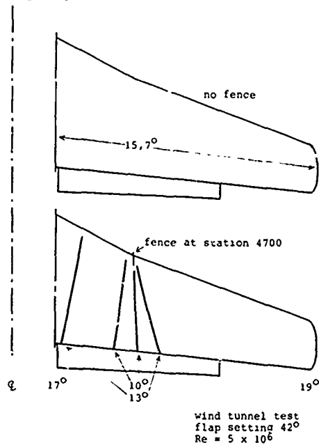
Fig. 12 Effect of fence on progression of flow separation
