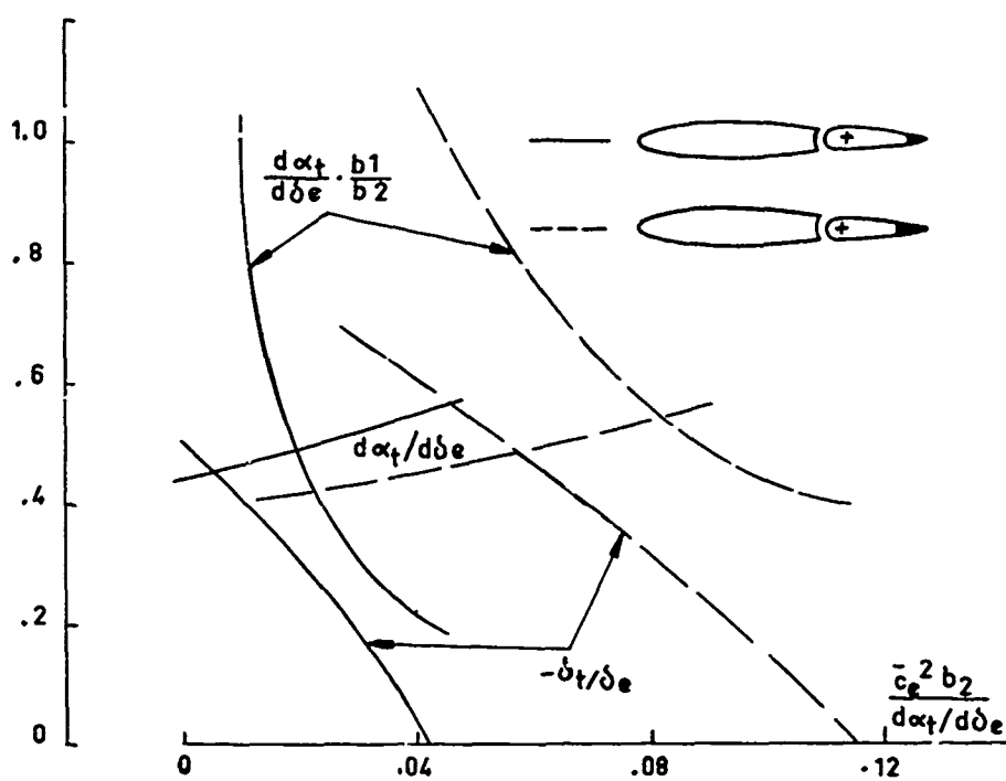
FIG. 7 - TWO-DIMENSIONAL CONFIGURATION INFLUENCE ON ELEVATOR EFFECTIVENESS AND FLOATING TENDENCY
