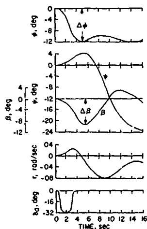
Fig. 6. Time history of the response of the NC-130B to a step bank maneuver; V = 70 knots
