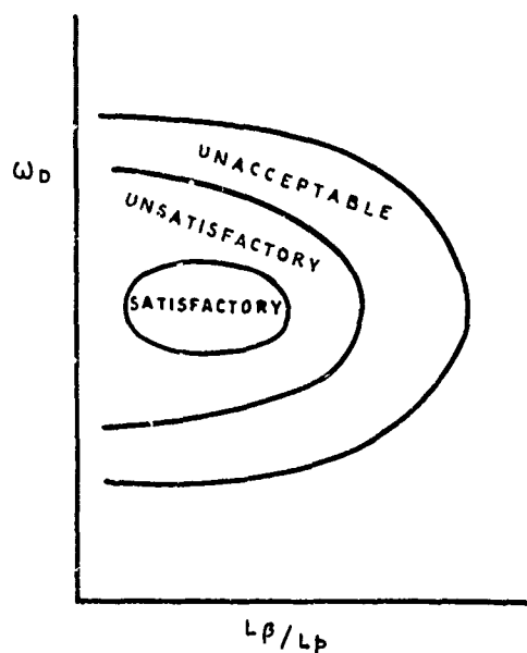
FIG. 24. A POSSIBLE CRITERION FOR LATERAL HANDLING QUALITIES IN TURBULENCE.
