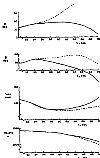
Fig.11 Late recovery action ( \alpha_r = 28^\circ and parachute deployed at 53 seconds)
