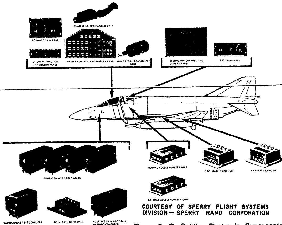
Figure 9 Fly-By-Wire Electronic Components
