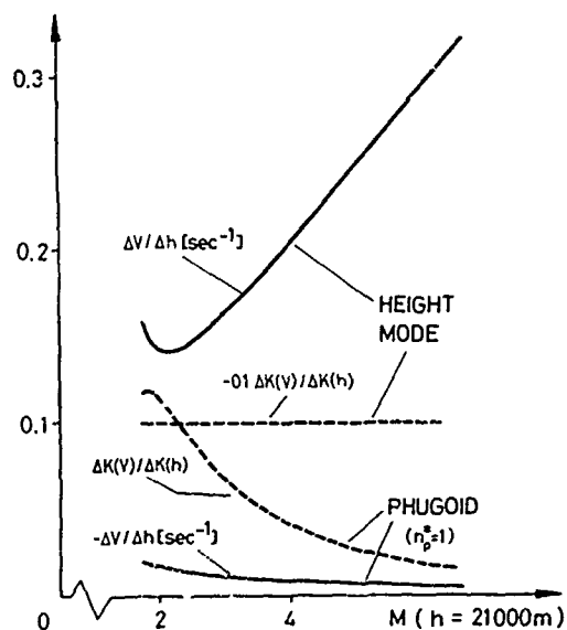
FIG. 7: SPEED-HEIGHT-RATIO AND AERODYNAMIC-FORCES-RATIO OF THE PHUGOID AND HEIGHT MODE
