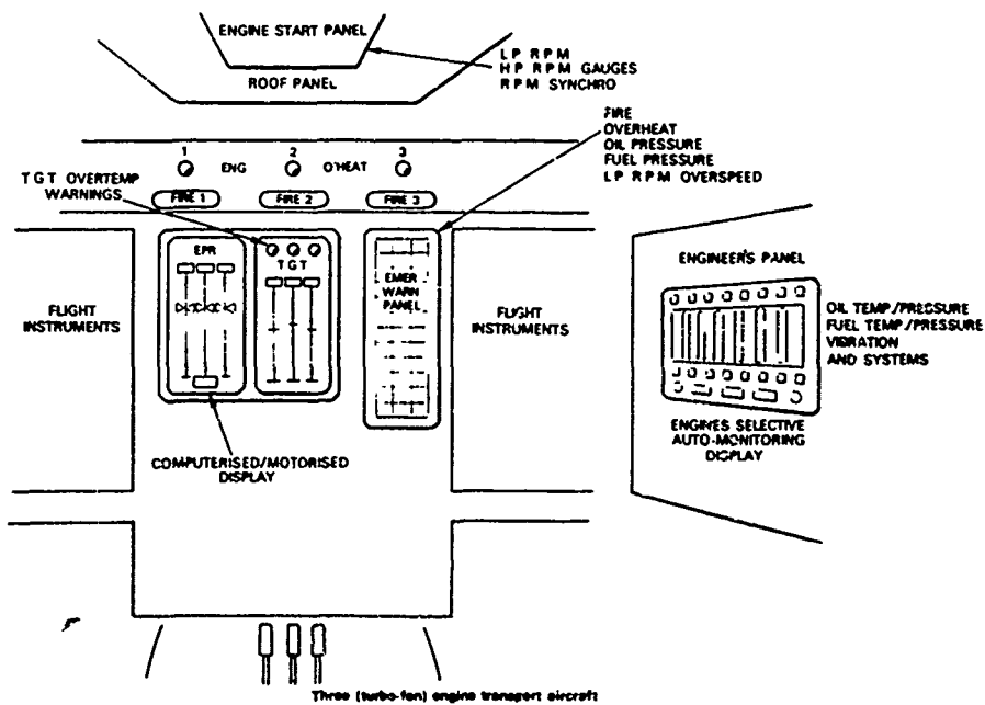
FIG. 4 PROPOSED ENGINE INSTRUMENTS PANELS LAYOUT FOR FUTURE AIRCRAFT.
