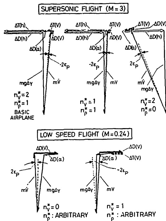
FIG. 8: TIME VECTOR DIAGRAM OF THE PHUGOID FOR SUPERSONIC AND LOW SPEED FLIGHT (POLYGON OF FLIGHT PATH TANGENTIAL FORCES)
