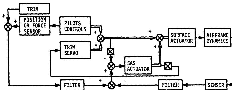
Figure 10 Two Methods Of Reducing Transients During Reversion To Mechanical Control
