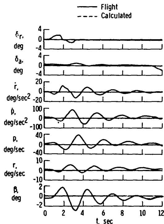
Figure 6 Comparison of flight and calculated time histories of a high aspect ratio, swept-wing airplane.
