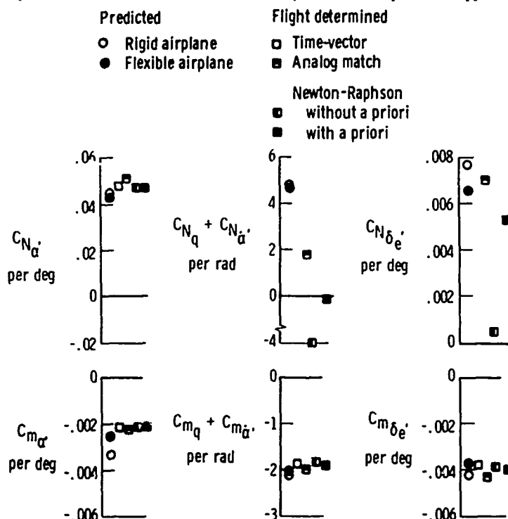
Figure 11. Comparison of predicted and flight-determined XB-70 longitudinal derivatives at Mach 0.75.
