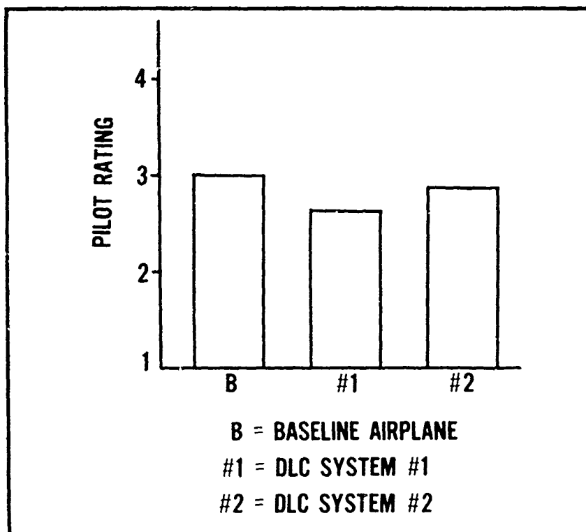
Figure 14 - S-3 Direct Lift Control Evaluation-Moving Base Simulator
