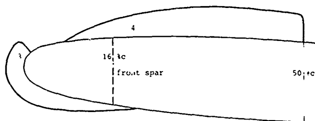
KINK SECTION OF WIND TUNNEL MODEL (STATION 4700)
