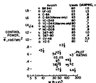
Fig. 4. Roll control power values for STOL aircraft.
