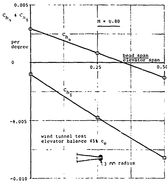
Fig. 7 Influence of bead on elevator hinge moment derivatives
