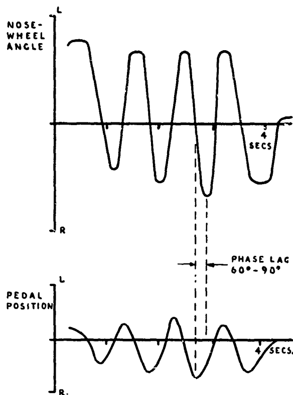
FIG. 28. EXAMPLE OF PILOT-INDUCED STEERING OSCILLATION DUE TO EXCESSIVE PHASE LAG IN RESPONSE.
