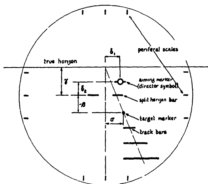
FIG. 6 IMAGE SEEN BY THE PILOT DURING LANDING (N A D).
