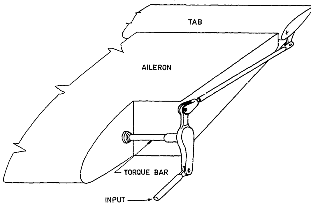
FIG.14- SKETCH OF AILERON SPRING-TAB
