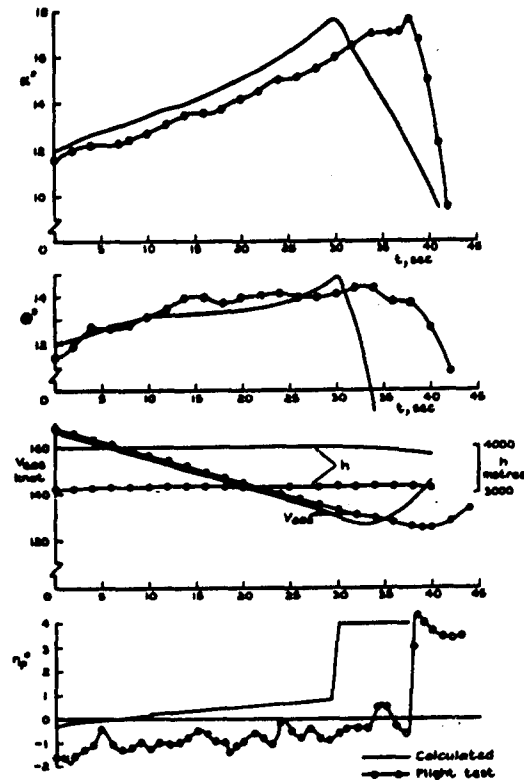
Fig.7 Comparison of calculated motion (WT data) with flight test results.
