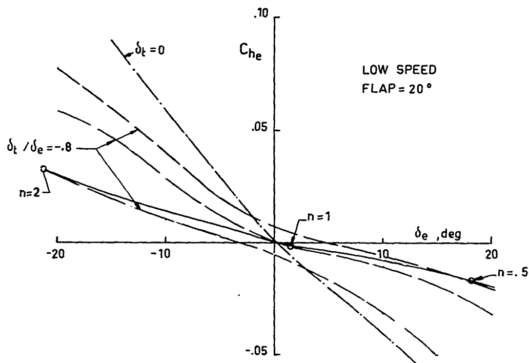
FIG. 9 - TYPICAL ELEVATOR HINGE MOMENT CHARACTERISTICS
