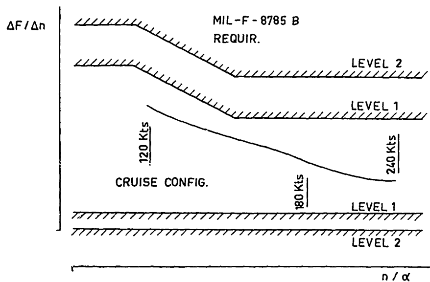
FIG. 8 - CONTROL FORCE GRADIENT VARIATIONS WITH SPEED
