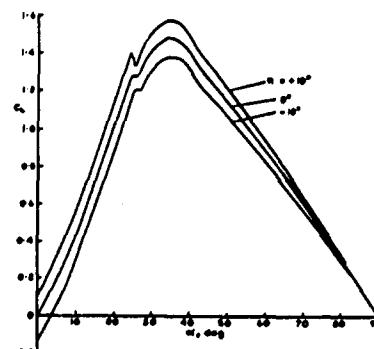
Fig.3 Lift characteristics assumed for the slender-wing tailless aircraft
