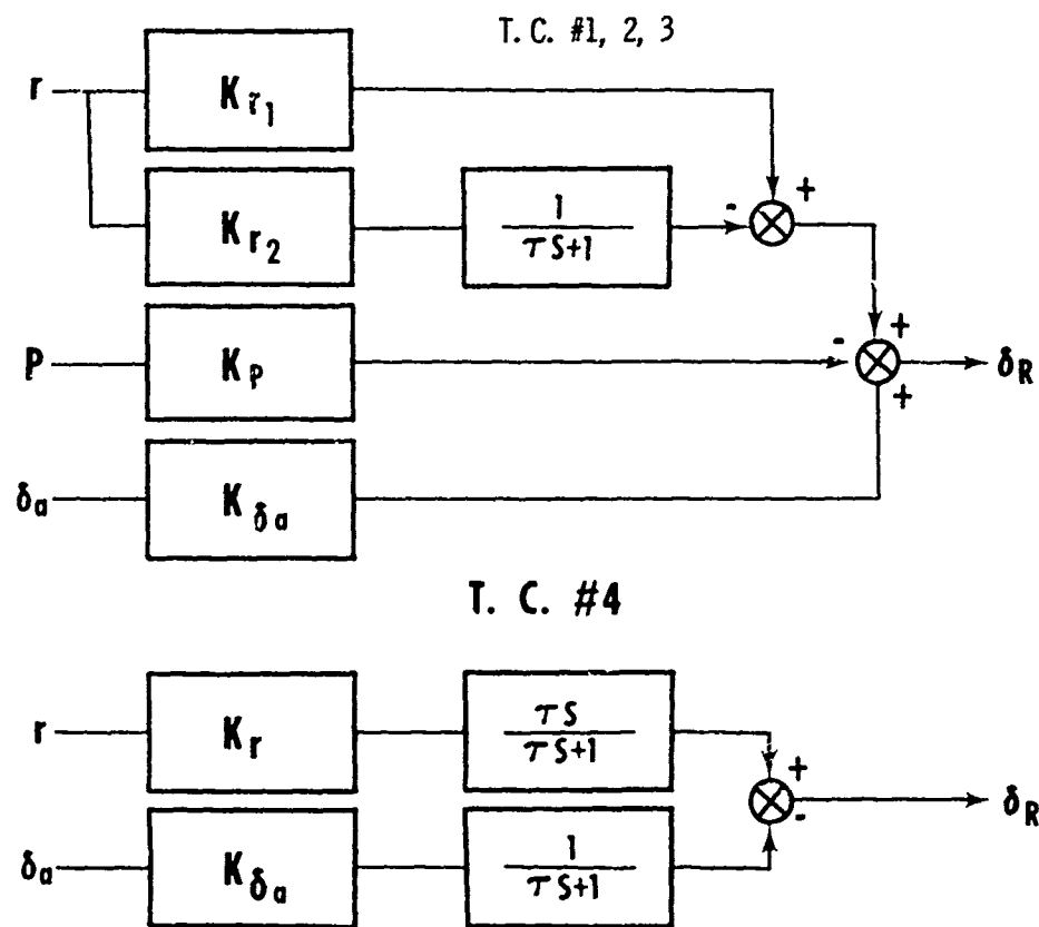
Figure 17 - Turn-Coordinator Mechanizations
