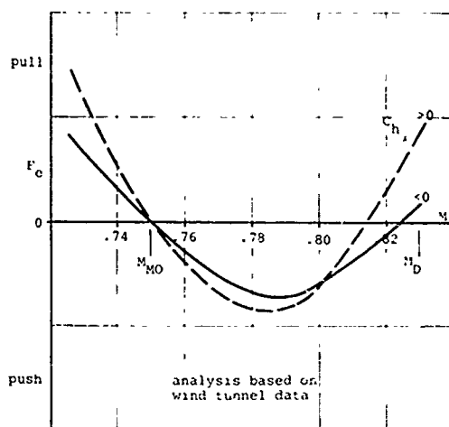
Fig. 5 Effect of C_{h_\alpha} -sign on transonic phenomena
