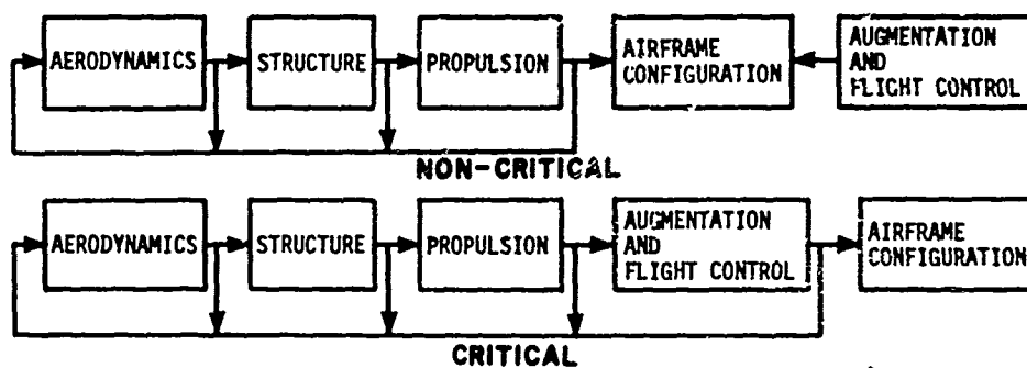
Figure 3 Design Cycle For Non-Critical And Critical Flight Control System Designs
