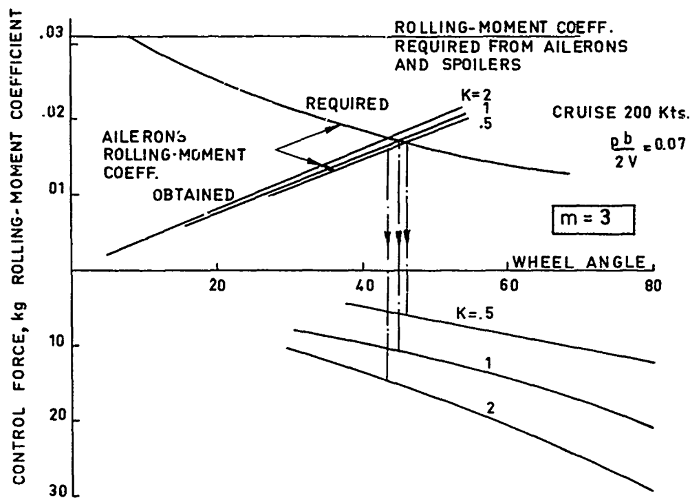
FIG.18 - DEFINITION OF AILERON SPRING-TAB CHARACTERISTICS
