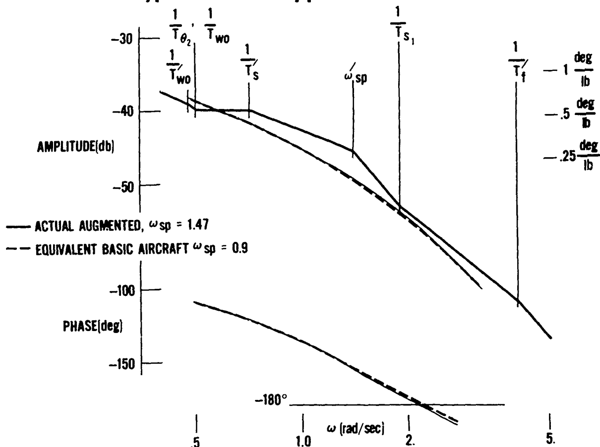
Figure 21 - F-14 Pitch Attitude to Stick Force Transfer Function
