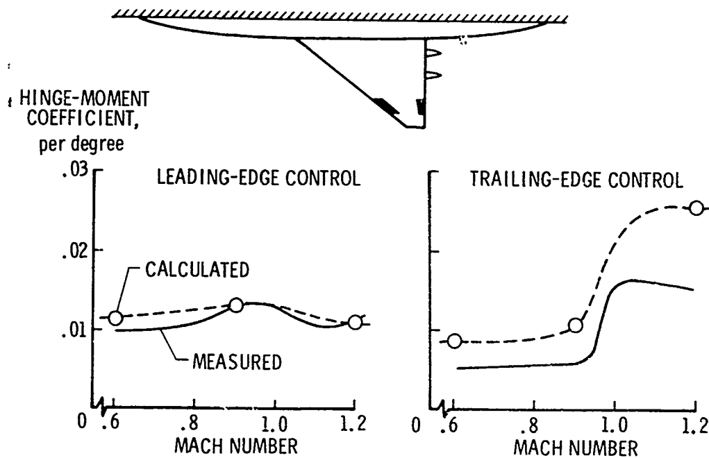
Fig.6 Comparison of measured and calculated static hinge moment coefficients
