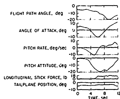
Fig. 3. Attitude divergence characteristics; P.1127 85 knots.
