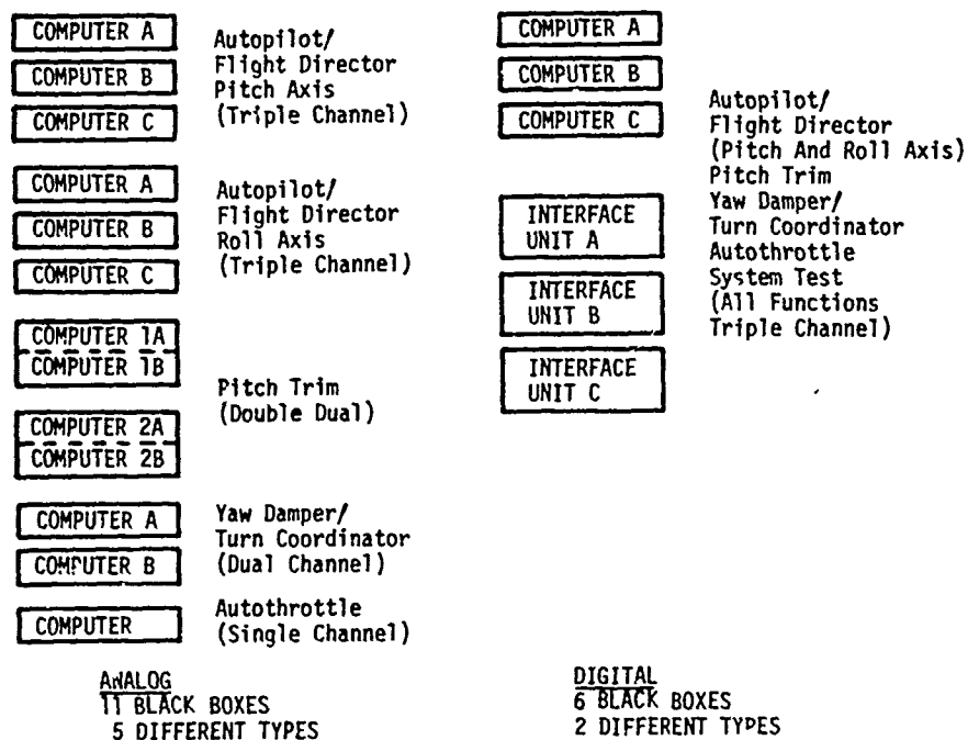
Figure 12 Comparison Of Hardware Complexity For A Typical Automatic Flight Control System
