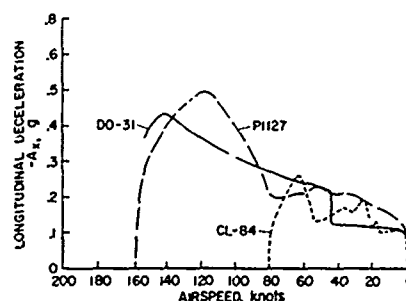
Fig. 9. Decelerating transition characteristics for several V/STOL aircraft.
