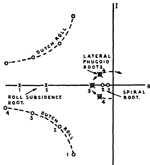
FIG. 19. LATERAL PHUGOID ONSET WITH REDUCING FIN SIZE ON SLENDER AEROPLANE WITH HIGH C_{dp} & HIGH \frac{C_{np}}{C_{dp}} (ROOT LOCUS PLOT.)
