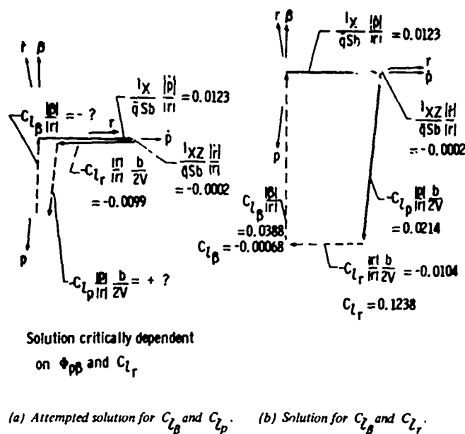
Figure 7 Graphical time-vector solution for rolling-moment derivatives of a light, twin-engine, propeller-driven airplane.
