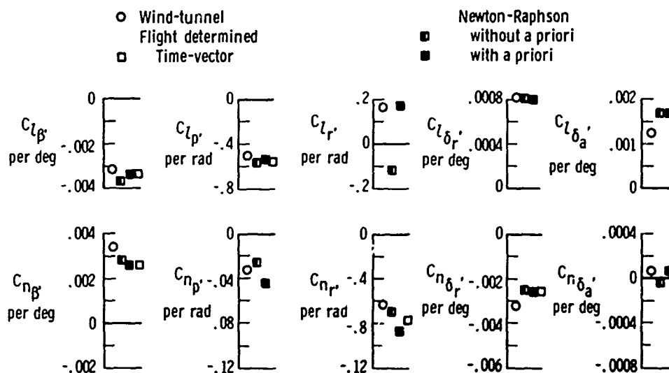
Figure 5 Comparison of predicted and flight-determined lateral-directional derivatives for a high aspect ratio, swept-wing airplane.
