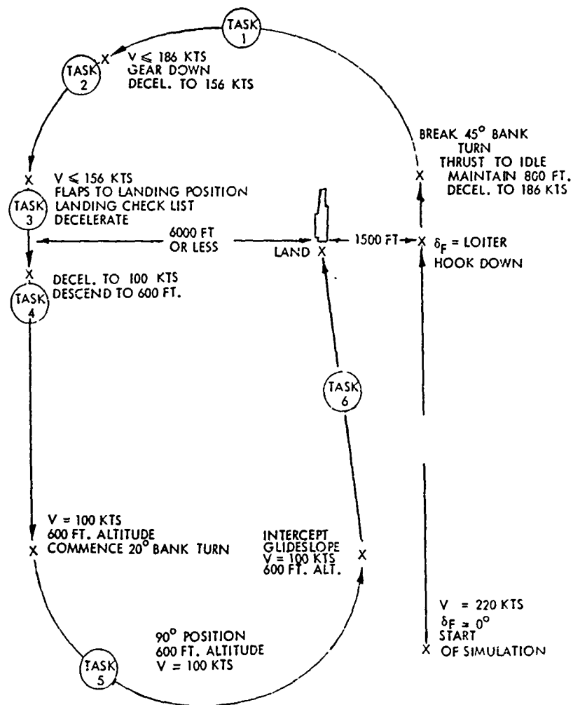
Figure 13 - Circling Approach Profile
