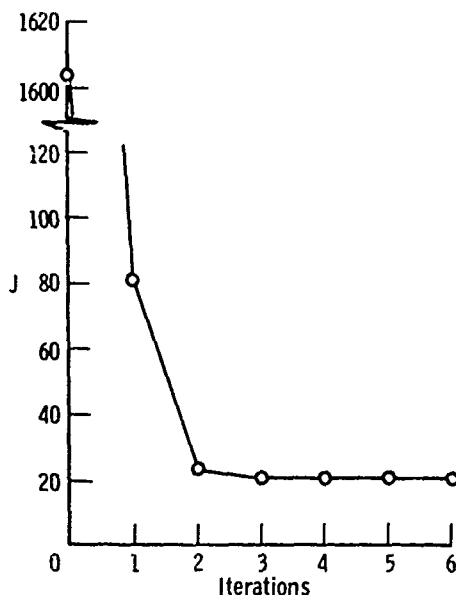
Figure 1. Convergence of fit error for the modified Newton-Raphson method (from ref. 6).
