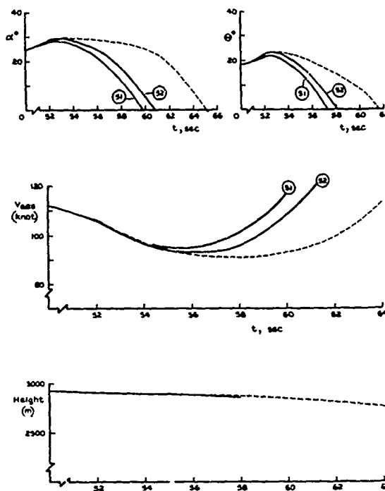
Fig.10 The effect on the recovery motion of deployment of a parachute at the instant indicated ( \alpha_r = 26^\circ )
