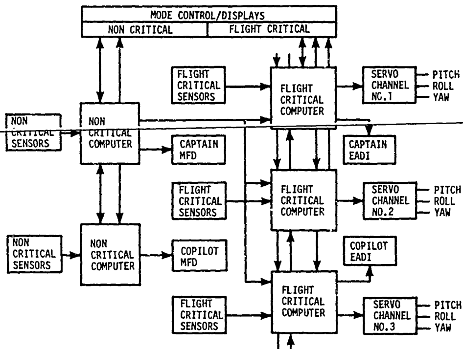
Figure 11 System Organization By Critical And Non-Critical Navigation, Guidance And Control Functions
