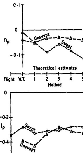
FIG. 3 COMPARISON WITH EXPERIMENT OF ROLLING MOMENT DERIVATIVES ESTIMATED BY VARIOUS METHODS
