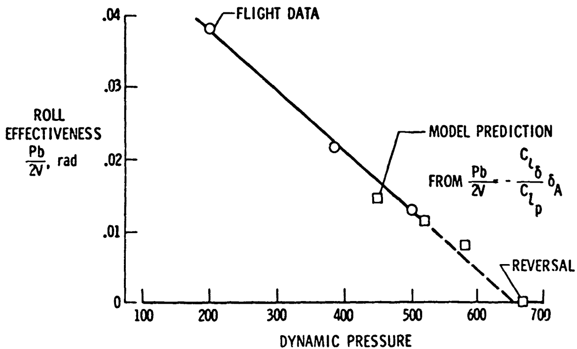
Figure 15 Comparison of flight measurement and model predicted aileron effectiveness.
