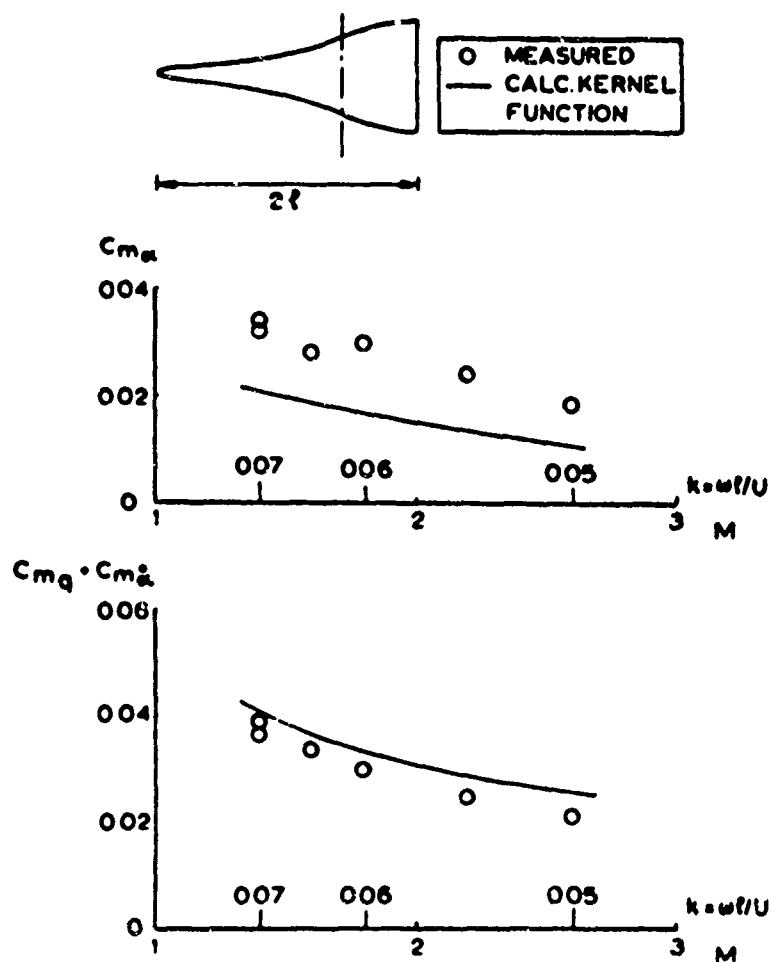
FIG. 3 PITCHING MOMENT ON OGEE WING DUE TO OSCILLATION ABOUT AXIS AT 71% OF ROOT CHORD (REF. 27).
