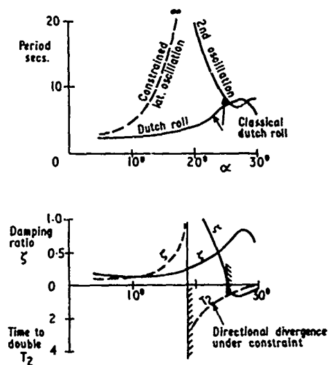
FIG. 8 CLASSICAL DUTCH ROLL AND BANK CONSTRAINED MODE FOR BAC 221 AIRCRAFT
