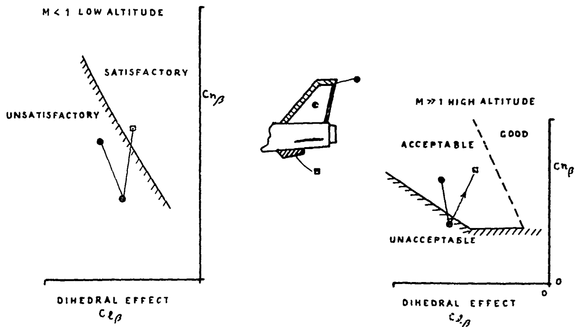
FIG. 21 EFFECTS OF ADDITIONAL BASIC FIN AREA COMPARED WITH VENTRAL FIN OF SAME AREA ON STABILITY AND HANDLING QUALITIES.
