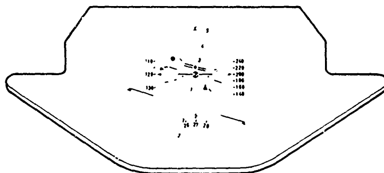
FIG. 5 IMAGE SEEN BY THE PILOT DURING LANDING (C S F).
