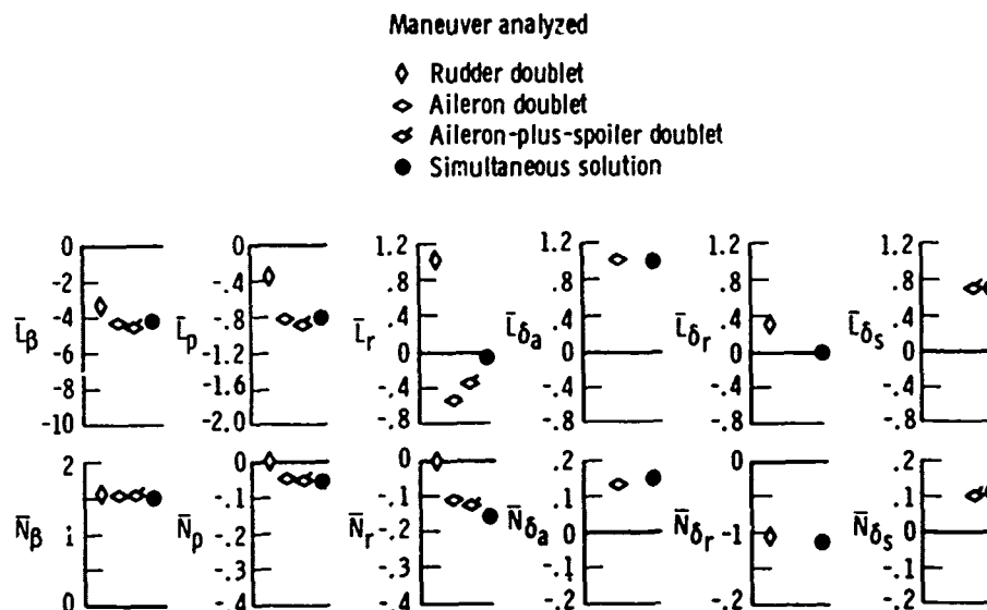
Figure 3. A comparison of derivatives from maneuvers analyzed separately and simultaneously by the modified Newton-Raphson method without a priori. Convair 990, M = 0.80 , h_p = 10,670 m (35,000 ft)
