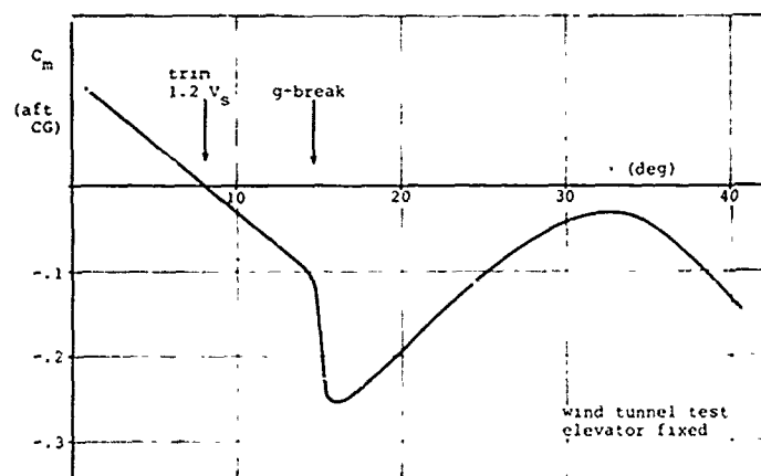
Fig. 9 F28 pitching moment characteristics
