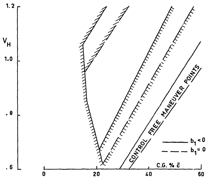
FIG. 5 - INFLUENCE OF b_1 ON CENTER OF GRAVITY LIMITS
