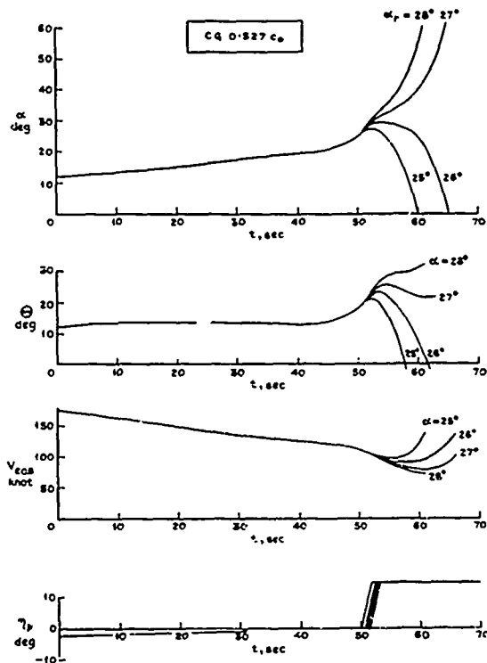
Fig.9 Response of aircraft with modified pitching moment characteristics to elevator input shown
