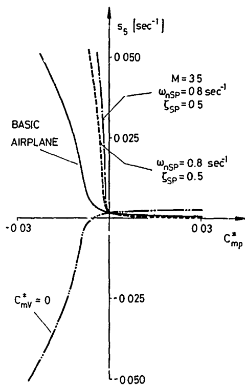
FIG.9: EFFECT OF C_{mp}^* ON THE HEIGHT MODE (PARAMETER: \omega_{nSP} , M , C_{mv}^* )
