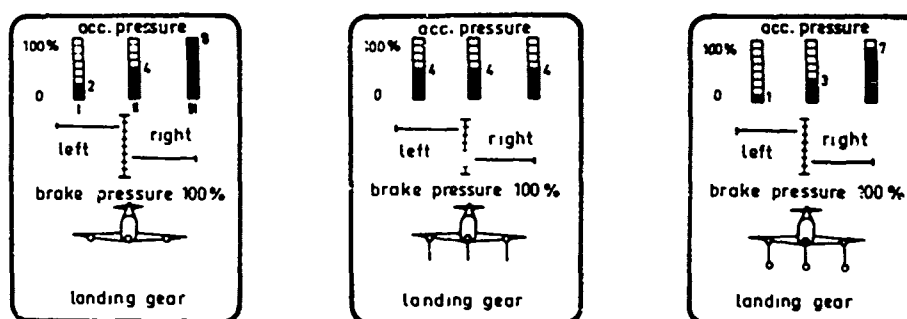
FIG. 13 EXAMPLE OF A DISPLAY FOR THE HYDRAULIC SYSTEM.
