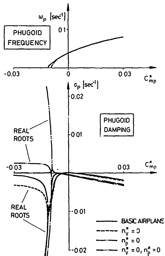
FIG.12: EFFECT OF C_{mp}^* ON THE PHUGOID (PARAMETER: n_p^* , n_v^* )
