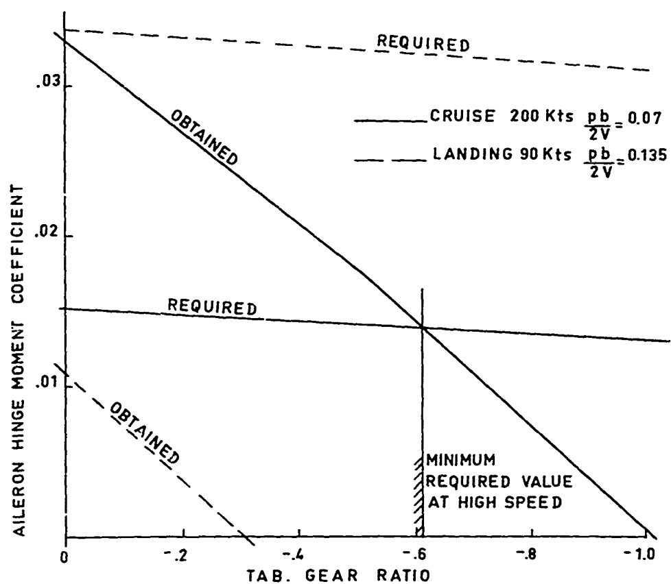
FIG. 13 - REQUIRED AND OBTAINED AILERON HINGE MOMENT VERSUS TAB GEAR RATIO.
