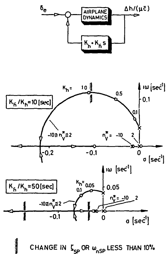
FIG.14: THRUST EFFECTS ON THE STABILIZATION OF THE PHUGOID AND HEIGHT MODE BY FEEDBACK OF HEIGHT AND RATE OF HEIGHT TO MOMENT
