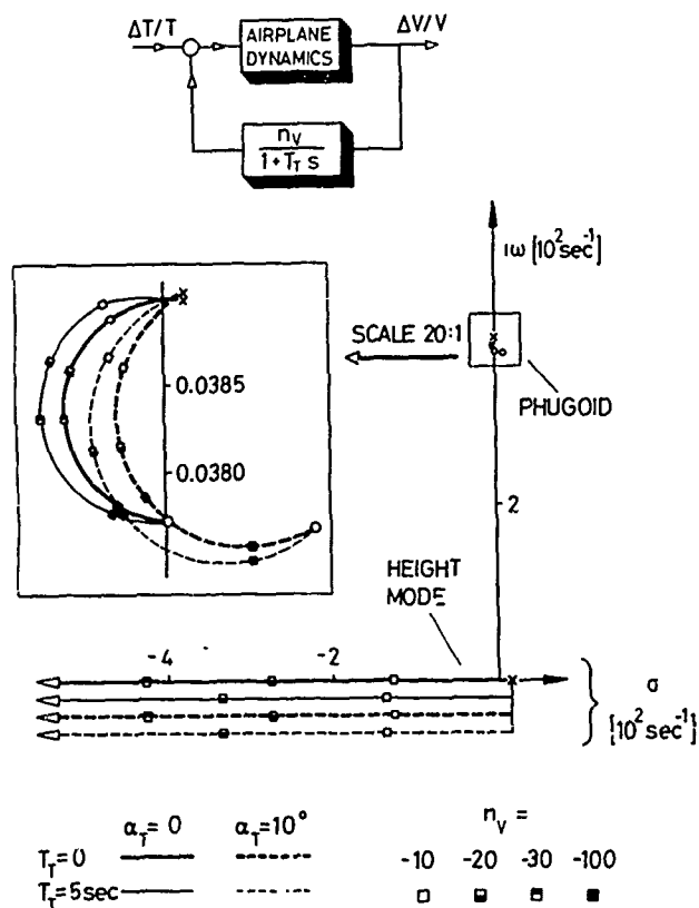
FIG. 5: EFFECT OF SPEED FEEDBACK TO THRUST ON THE PHUGOID AND HEIGHT MODE IN SUPERSONIC FLIGHT ( M=3 )
