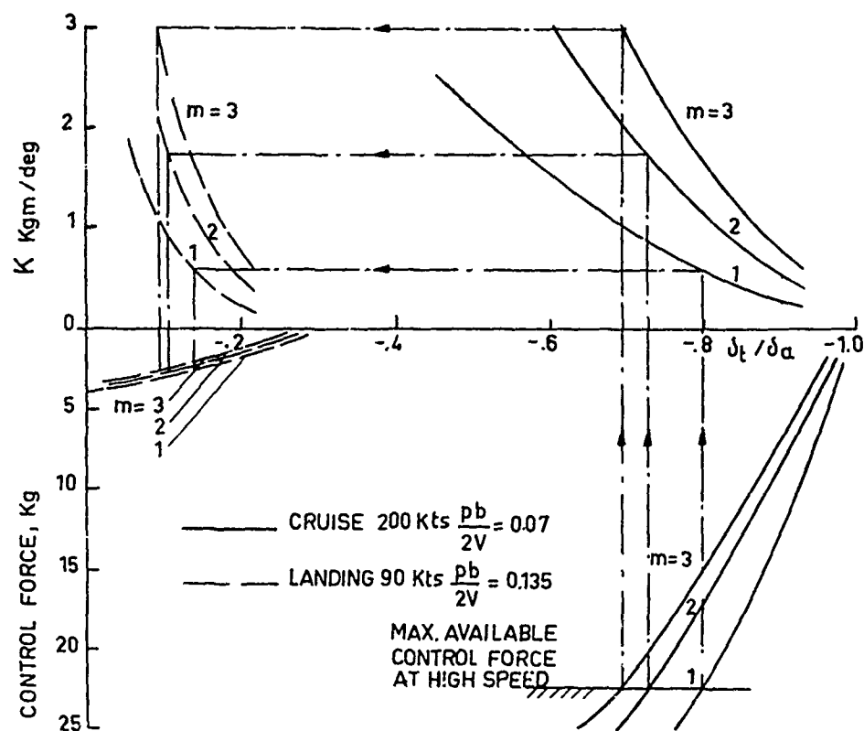
FIG.15- DEFINITION OF AILERON SPRING-TAB CHARACTERISTICS SIMPLIFIED CALCULATIONS
