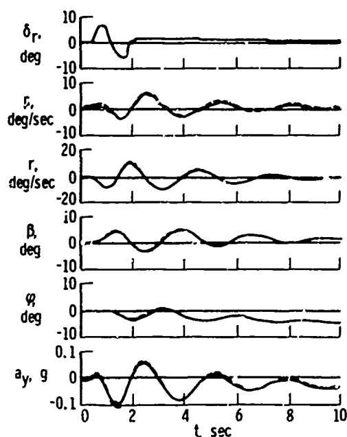
Figure 9. Comparison of flight and calculated time histories of a light, twin-engine, propeller-driven airplane.
