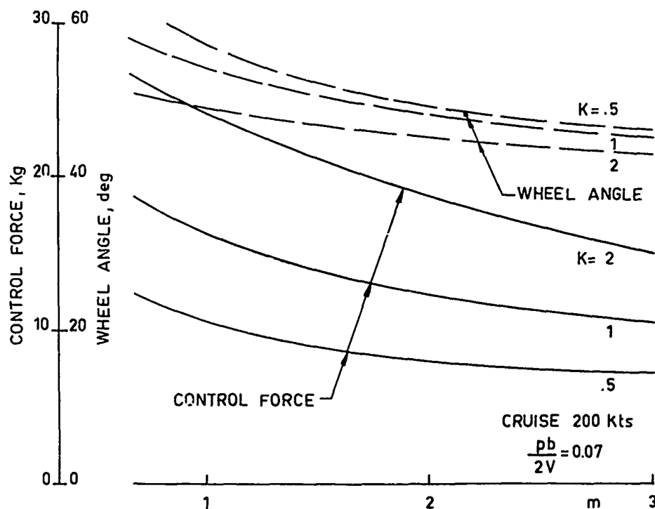
FIG. 21- SYNTESIS OF AILERON SPRING-TAB TYPICAL CHARACTERISTICS
