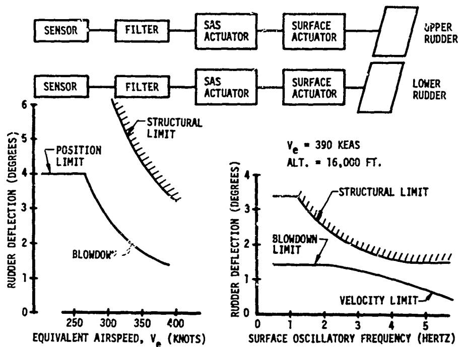
Figure 2 Yaw Dampar Authority
