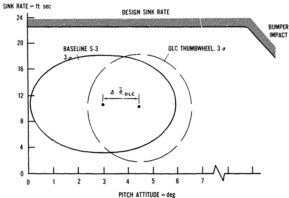
Figure 15 - S-3 Conditions at Touchdown - Moving Base Simulation
