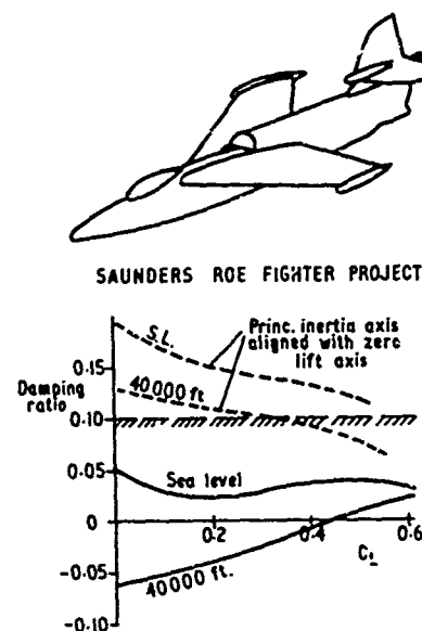
FIG. 4 PREDICTION OF DUTCH ROLL CHARACTERISTICS OF AN AIRCRAFT PROJECT REVEALING TOTALLY UNACCEPTABLE BEHAVIOUR
