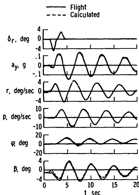
Figure 4. Comparison of Convair 990 flight and calculated time histories of a rudder-doublet maneuver. M = 0.80 , h_p = 10,670 m (35,000 ft).
