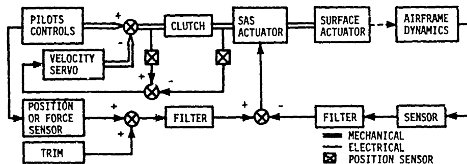
Figure 9 Fly-By-Wire Electronic Components
