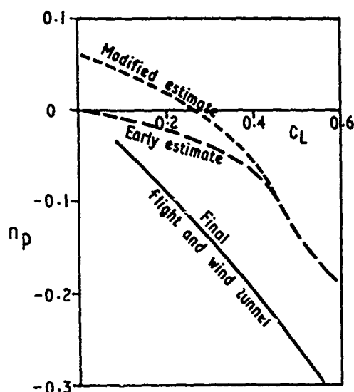
FIG. 6 COMPARISON OF EARLY ESTIMATES AND LATER FLIGHT AND WIND TUNNEL DATA FOR THE DERIVATIVE n_p .
