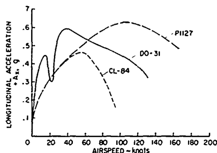
Fig. 8. Accelerating transition characteristics for several V/STOL aircraft.
