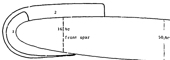
KINK SECTION OF WIND TUNNEL MODEL (STATION 4700)
