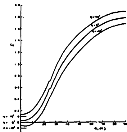
Fig.2 Drag characteristics assumed for the slender-wing aircraft
