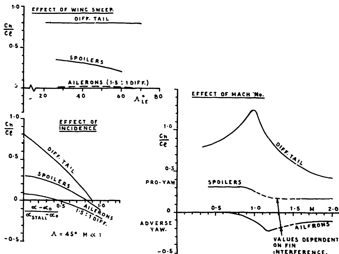
FIG. 13 VARIATION OF YAWING MOMENT DUE TO ROLL CONTROL WITH SWEEP, MACH NO. AND INCIDENCE FOR ALTERNATIVE ROLL CONTROLS
