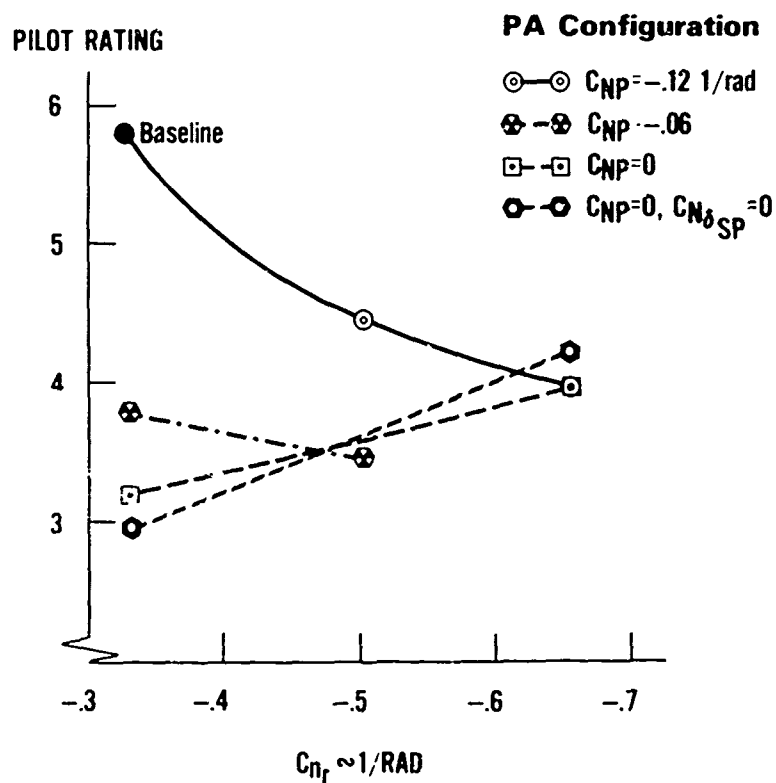
Figure 16 - S-3 Lateral Directional Parametric Study
