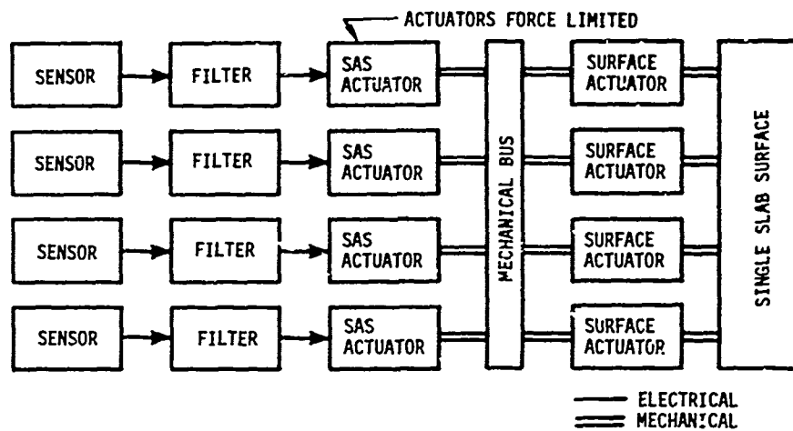
Figure 5 System Mechanization Using Single Control Surfaces
