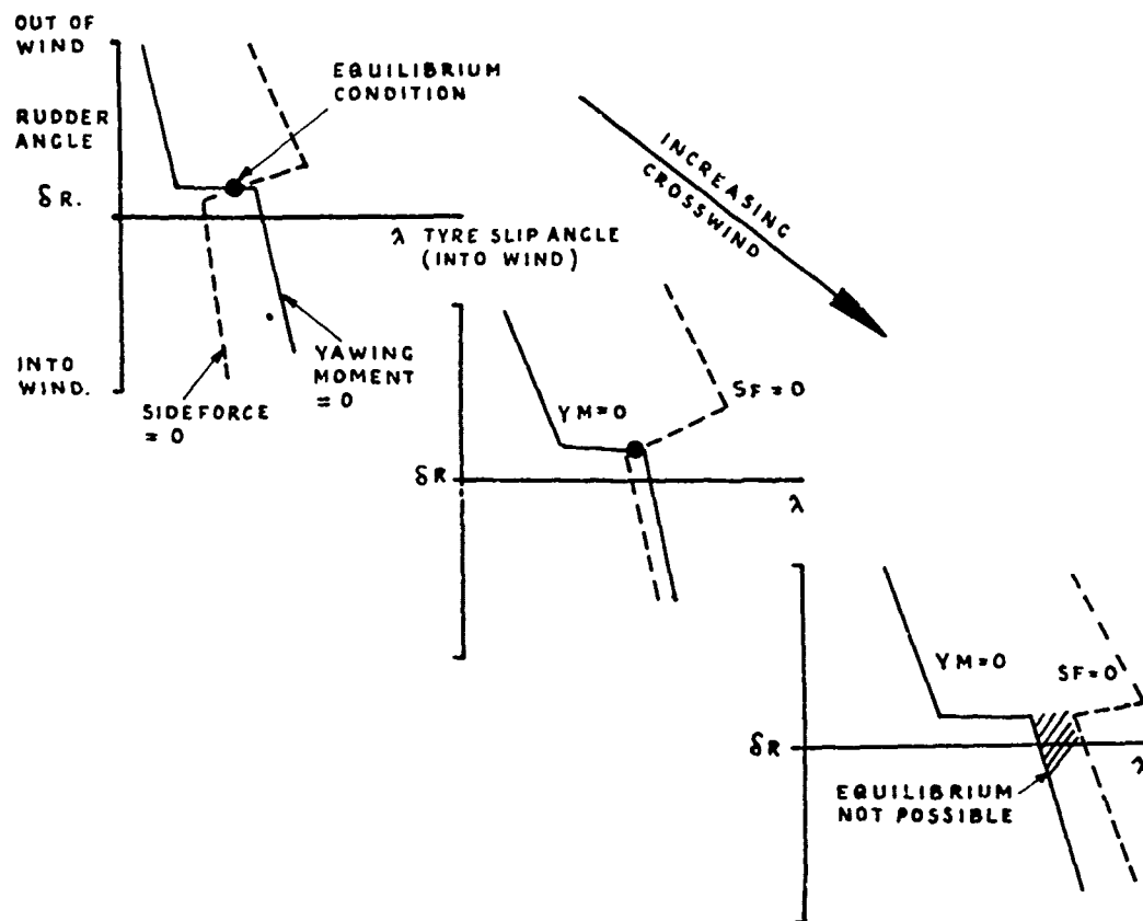
FIG. 29. CROSSWIND LANDING GROUND ROLL EQUILIBRIUM CONDITIONS
