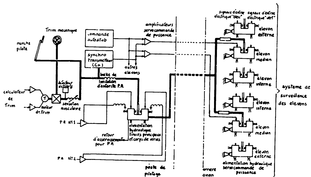
SCHEME SHOWING THE PRINCIPLES OF THE CONCORDE FLYING CONTROL SYSTEM
