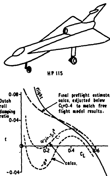
FIG. 5 PREFLIGHT PREDICTIONS OF DUTCH ROLL STABILITY OF THE H.P. 115
