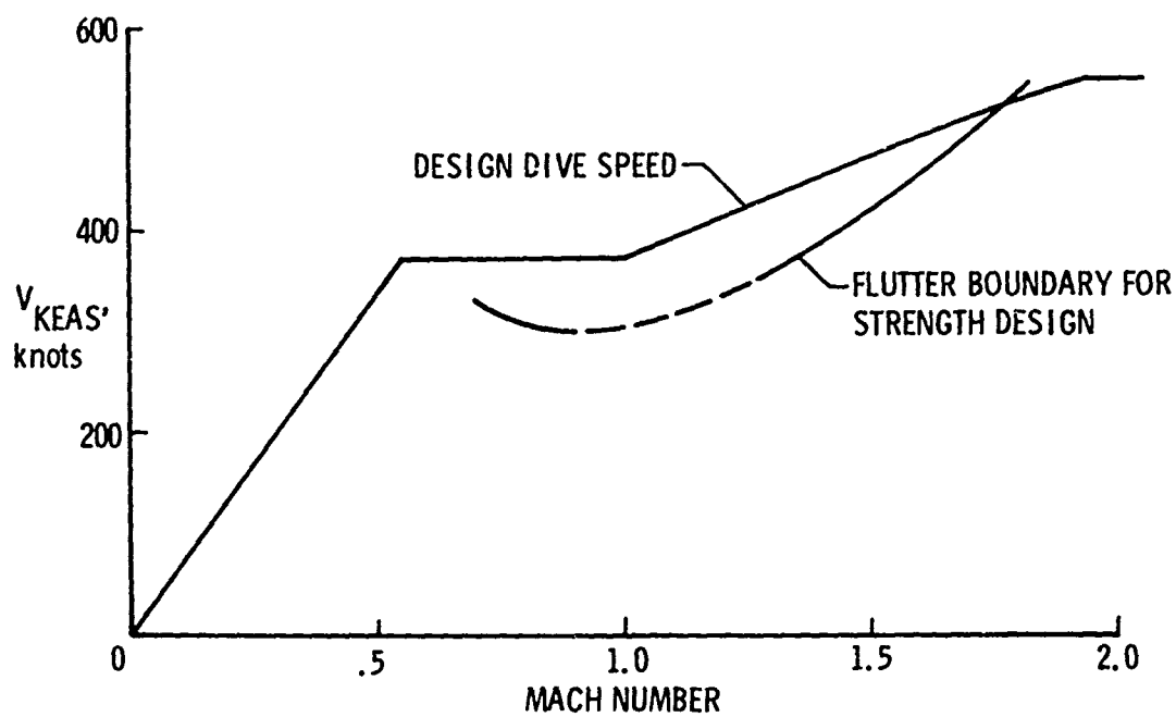
Fig.1 Flutter prevention considerations for the US SST
