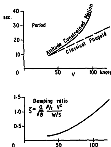
FIG. 10 LONGITUDINAL MOTION IN THE STOL REGIME WITH PITCH ATTITUDE CONSTRAINT BY ELEVATOR CONTROL
