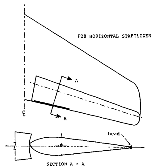
Fig. 6 F28 tailplane and final elevator configuration
