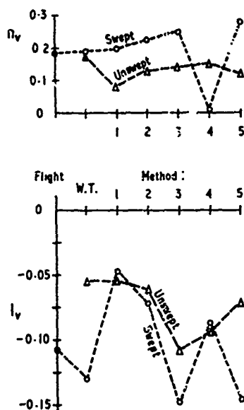
FIG. 2 COMPARISON WITH EXPERIMENT OF LATERAL DERIVATIVES ESTIMATED BY VARIOUS THEORETICAL METHODS
