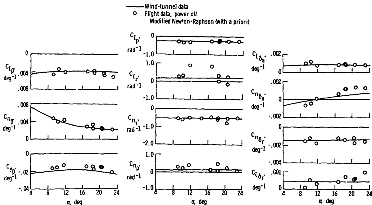
Figure 2. Comparison of flight-determined derivatives with wind-tunnel data for the HL-10 lifting body.
