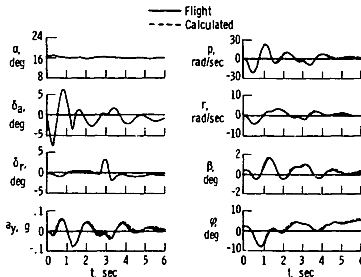
Figure 12. Comparison of flight and calculated (with a priori) time histories of the HL-10 lifting body with stability augmentation system on. Control inputs—aileron and rudder doublets
