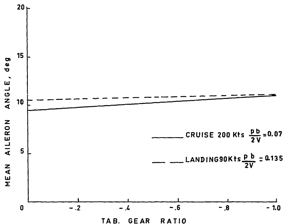
FIG. 12 - REQUIRED AILERON ANGLE VERSUS TAB GEAR RATIO
