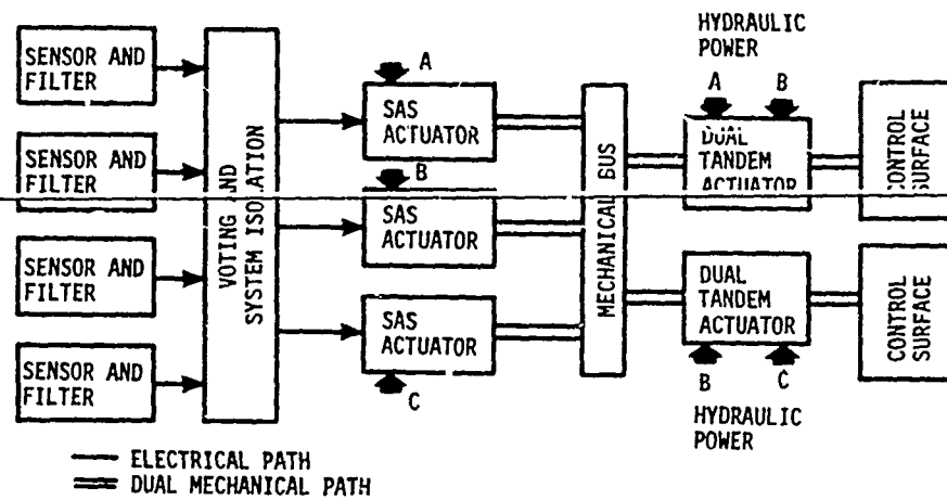
Figure 7 Redundancy Levels For Flight Critical Applications
