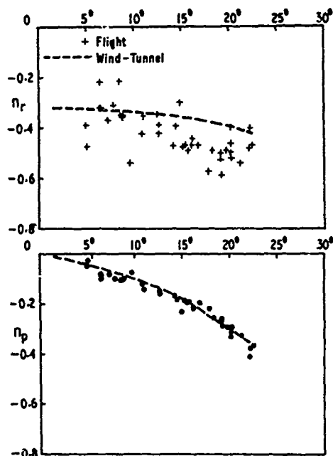
FIG. 1 YAWING MOMENT DERIVATIVES OF HPIIS FROM ANALYSIS OF DUTCH ROLLS
