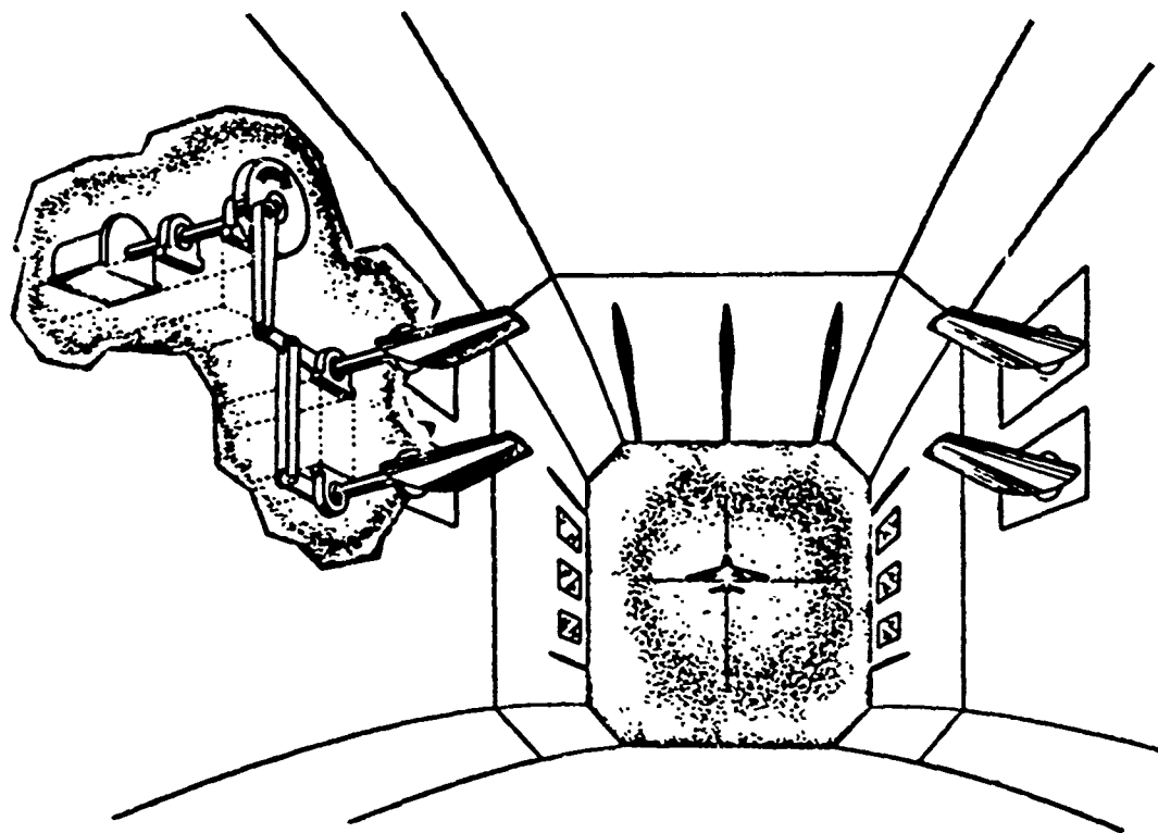
Figure 13 Langley transonic dynamics tunnel airstream oscillator. View looking downstream toward model with cutaway showing schematic of mechanism.
