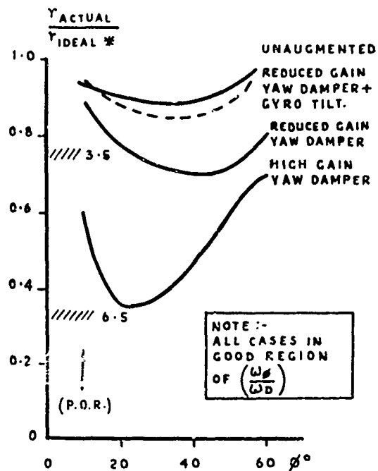
FIG. 25. TURN ENTRY MANOEUVRE PILOT COMMENTS RELATED TO RATE OF YAW DEVELOPMENT.
