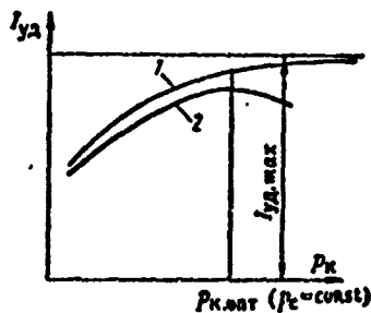
Fig. 9.9. Dependence of specific impulse of the chamber (1) and engine (2) with exhausting of the working fluid, after operation in the turbine, into the atmosphere on the pressure p_K ( p_c = \text{const} ).
