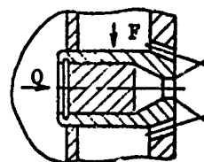
Fig. 12.8. Two-component combination injector.
