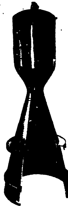
Fig. 12.3. Chamber of the RD-107 "Vostok" LPRE.
