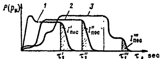
Fig. 14.1. Change in thrust (pressure p_k ) for various types of start-ups and shutdowns of an LPRE: 1 - abrupt ("full-flow") start; shutdown without final stage; 2 - start with preliminary stage; shutdown without final stage; 3 - start with preliminary and intermediate stages; shutdown through final stage.
