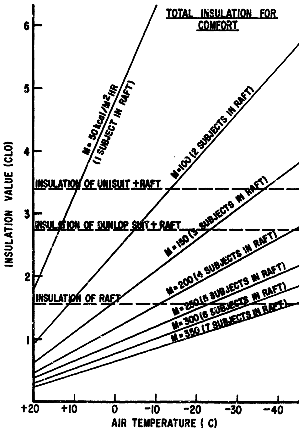
FIGURE 9. PREDICTIVE CLO VALUES REQUIRED FOR COMFORT IN A 7-MAN LIFE RAFT. THE AVERAGE METABOLIC RATE OF 50 Kcal/M 2 HR IS BASED ON DATA OBTAINED IN THIS STUDY.
