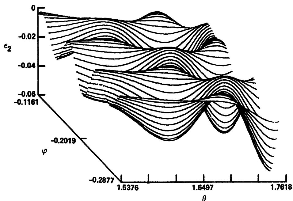
Figure 4.4. Azimuth Component of Nonradial Power, \epsilon_2 , at Sample Point 1
