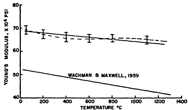
Figure 13. Young's Modulus of TYCO c-Axis Sapphire as a Function of Temperature. (The modulus of 30^{\circ} sapphire rods is included for reference, Reference 26. The dotted line indicates a second possible curve connecting the data points.)
