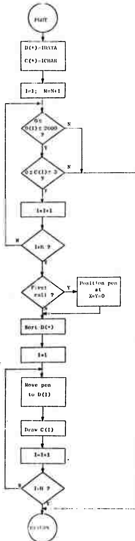
Fig. 4 Flowchart for PLOT Program
