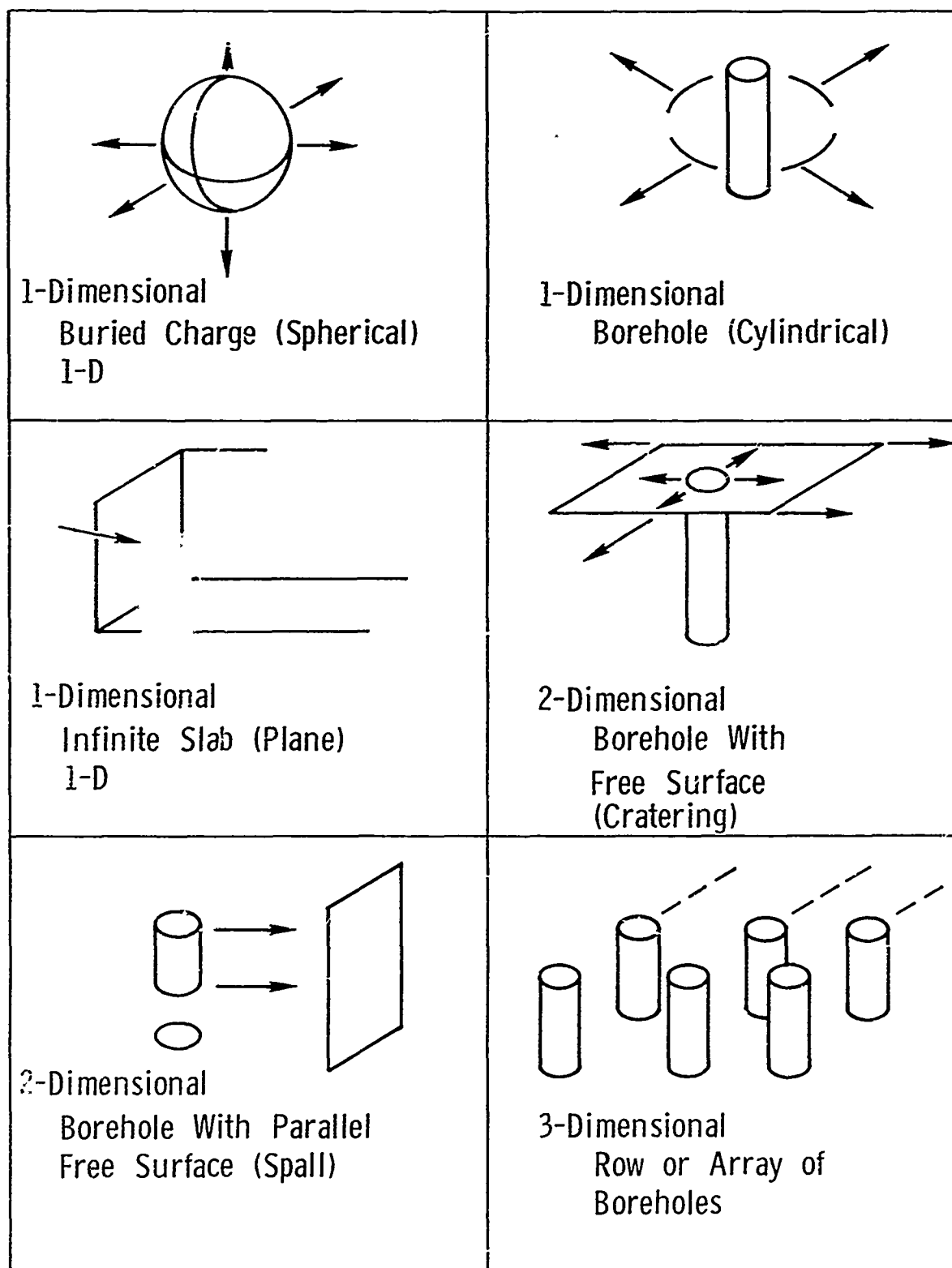
Figure 4 Material geometries.
