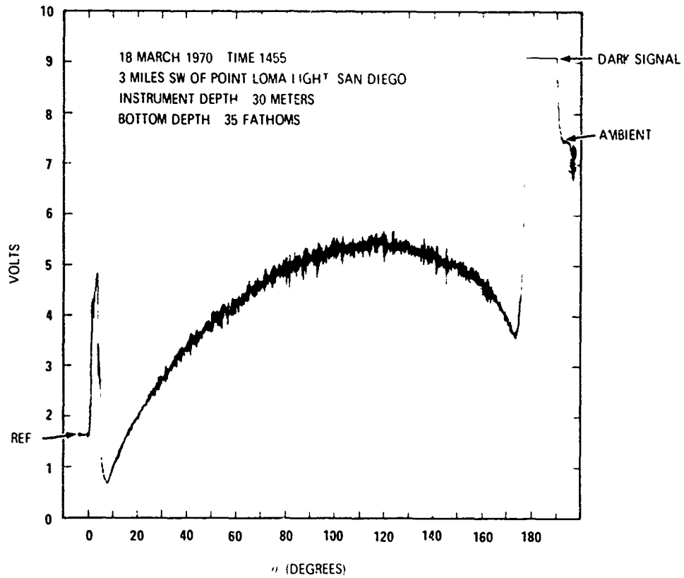
Figure 6. Sample of Signal Output Obtained with General Angle Scattering Meter.
