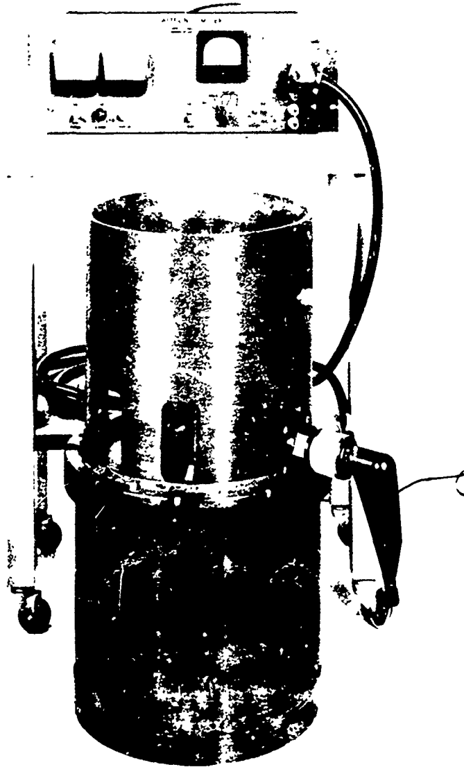
Figure 4. General Angle Scattering Meter.
