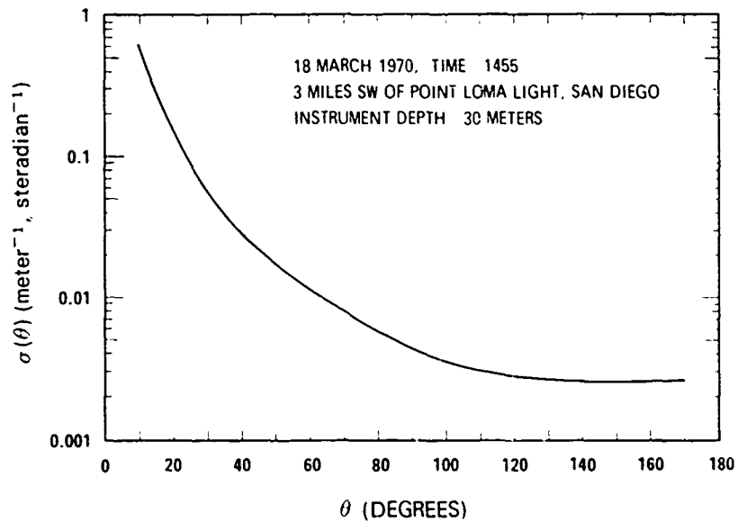
Figure 7. Sample of Final Data Obtained with General Angle Scattering Meter.
